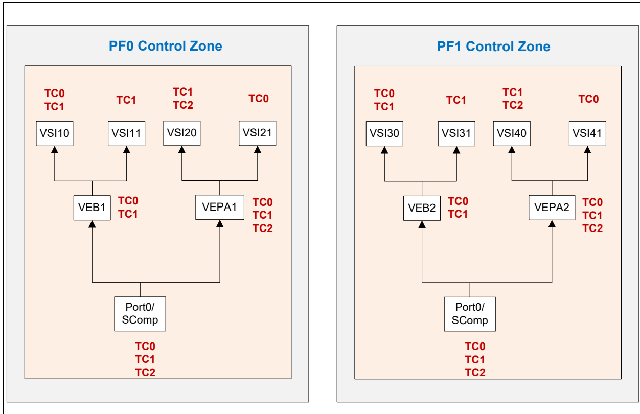
Figure 7-82. Software Control Zone in SFP Mode
