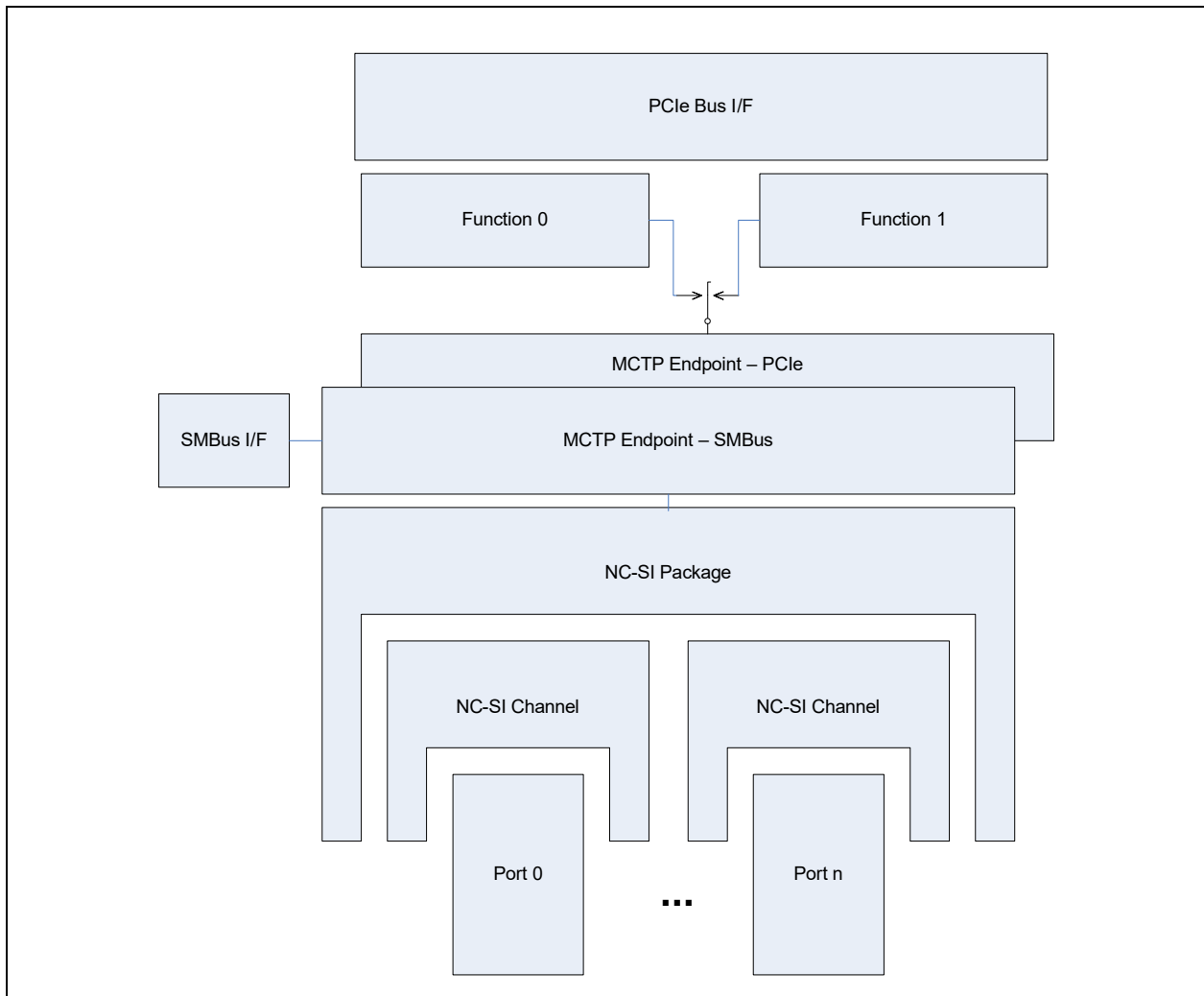
Figure 9-13. MCTP endpoints topology
