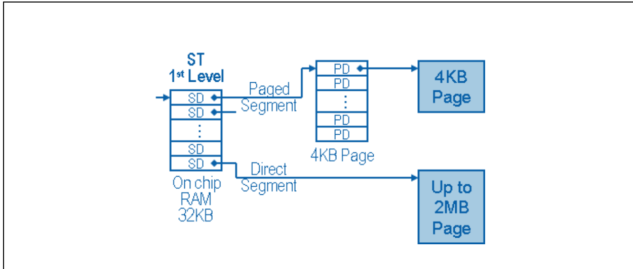
Figure 7-91. Host Memory Cache Direct Segment
