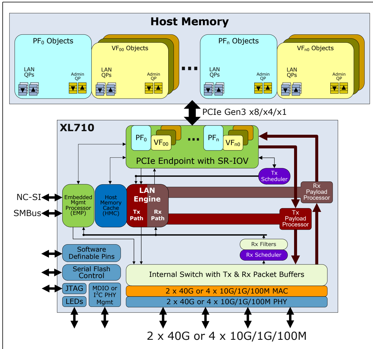
Figure 1-8. Fortville block diagram
