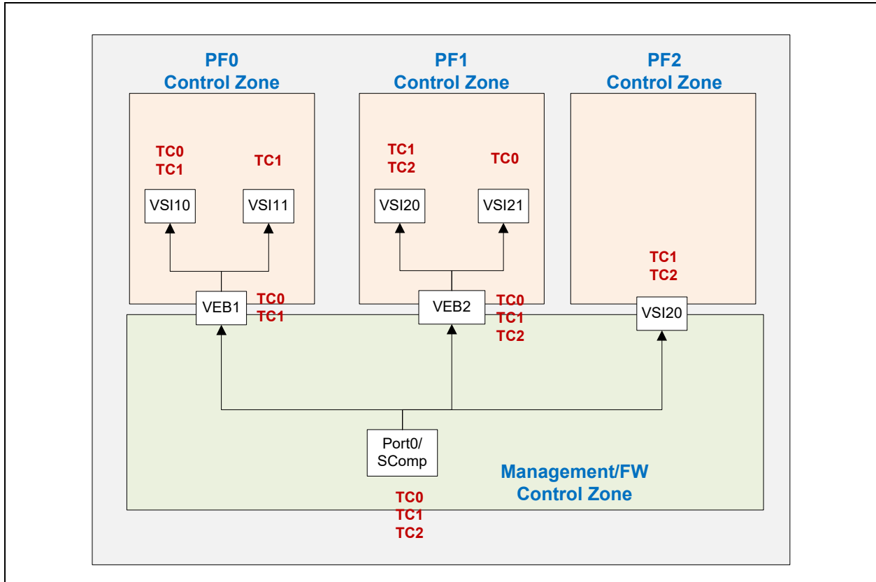
Figure 7-83. Software Control Zone in MFP Mode
