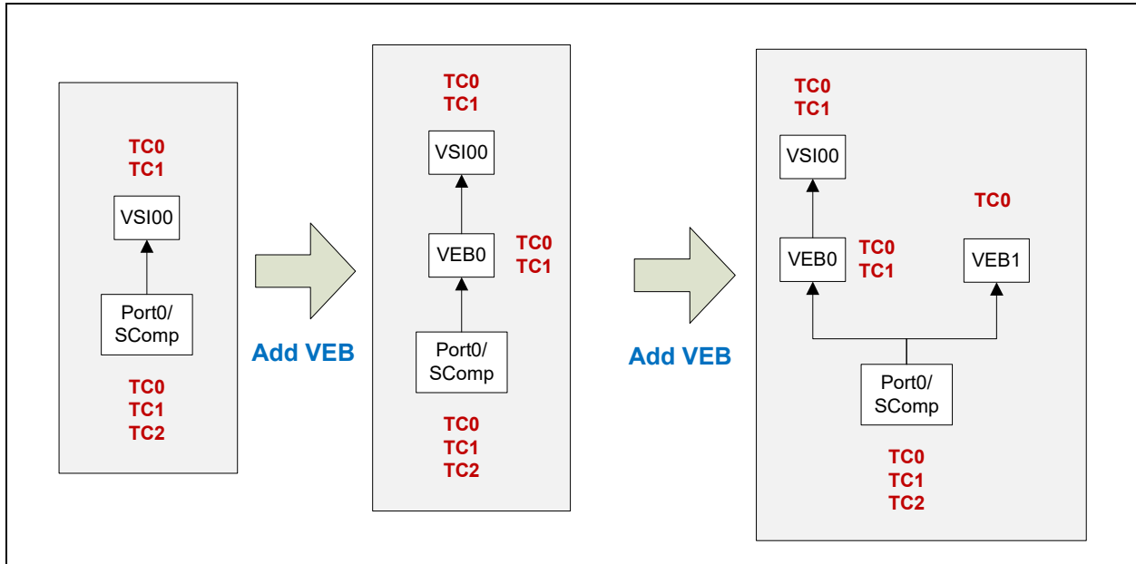
Figure 7-80. Adding VEB/PA
