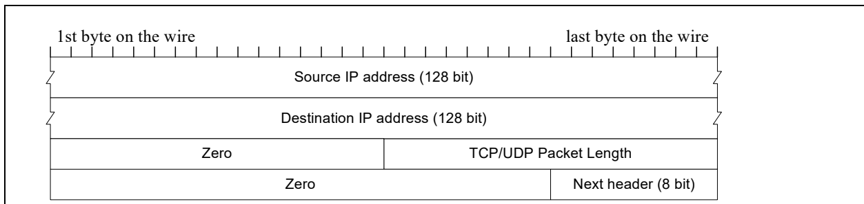
Figure 7-25. IPv6 pseudo header for TCP/UDP checksum
