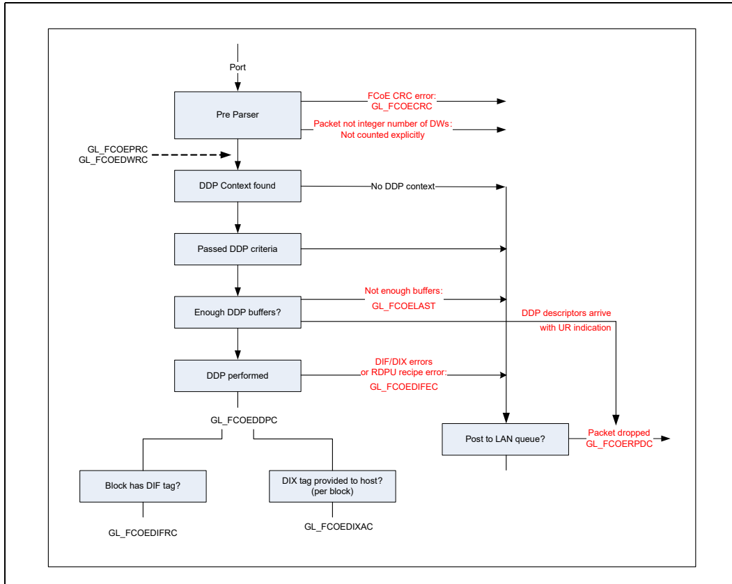
Figure 7-93. FCoE function statistics
