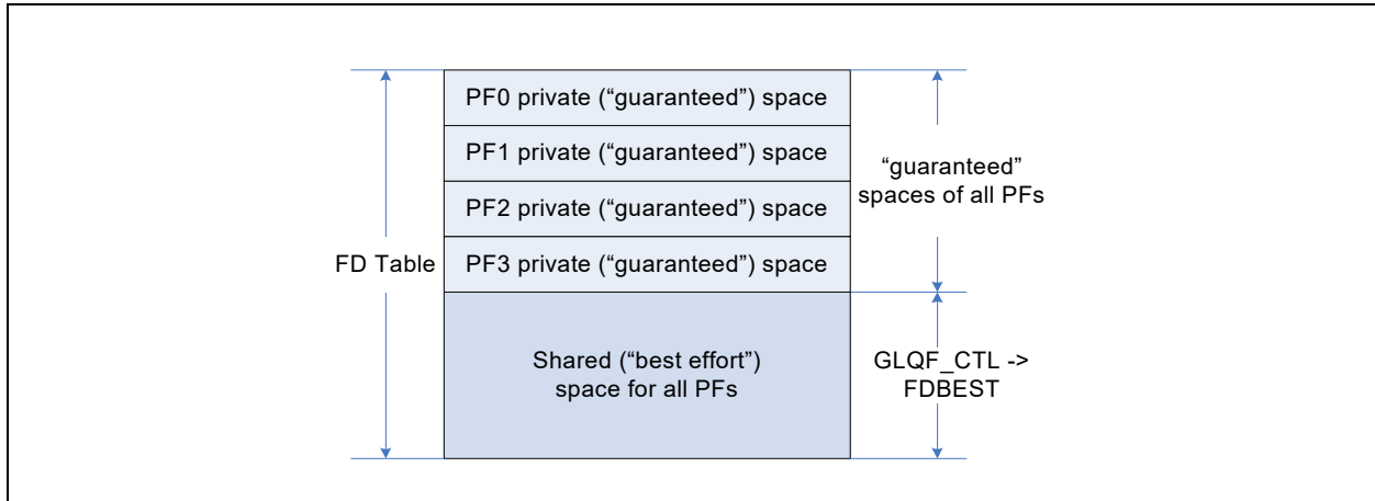
Figure 7-5. FD table allocation (example for 4 x PFs: PF0 ... PF3)
