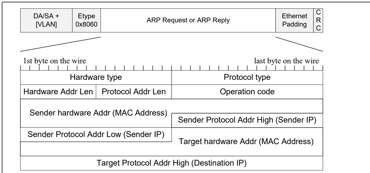
Figure 7-22. ARP packet format
