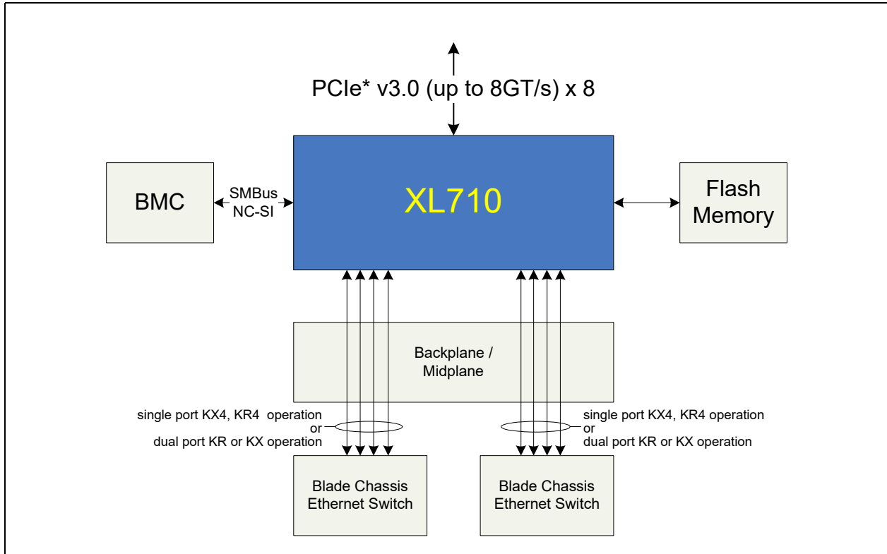
Figure 1-4. Typical blade system dual-redundant star configuration
