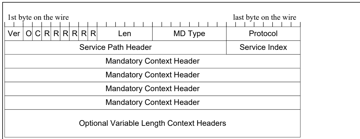
Figure 7-33. NSH header structure
