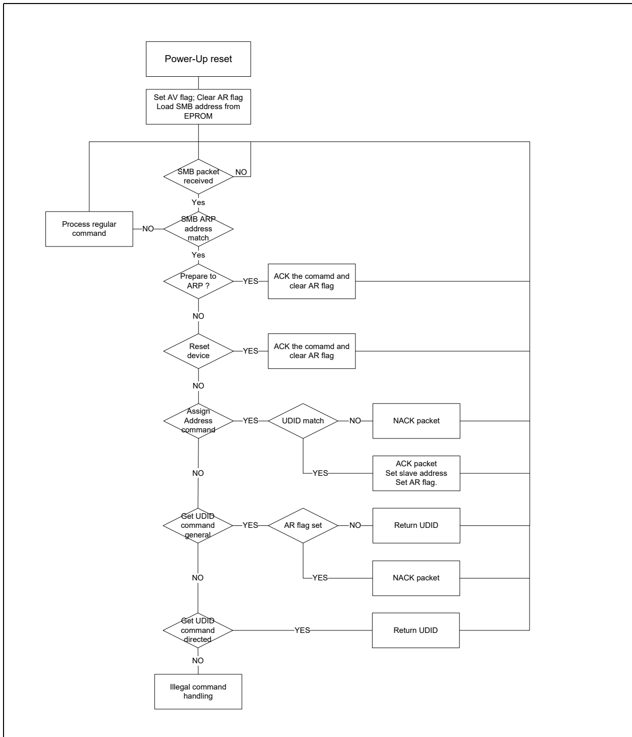
Figure 9-4. SMBus ARP flow
