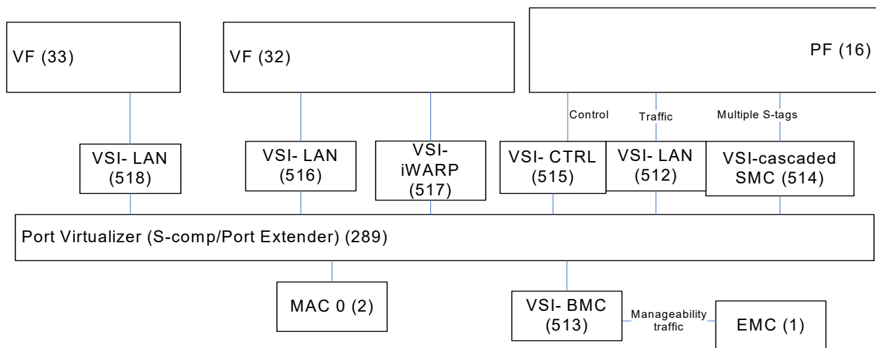
Figure 7-56. Port Virtualizer
