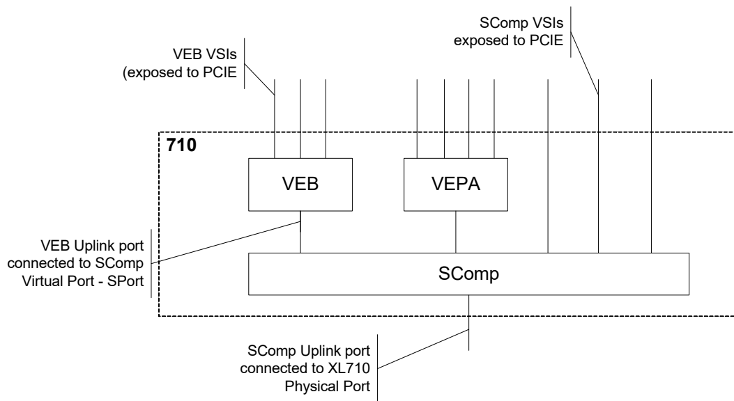
Figure 7-72. Hierarchy of Switching Elements
