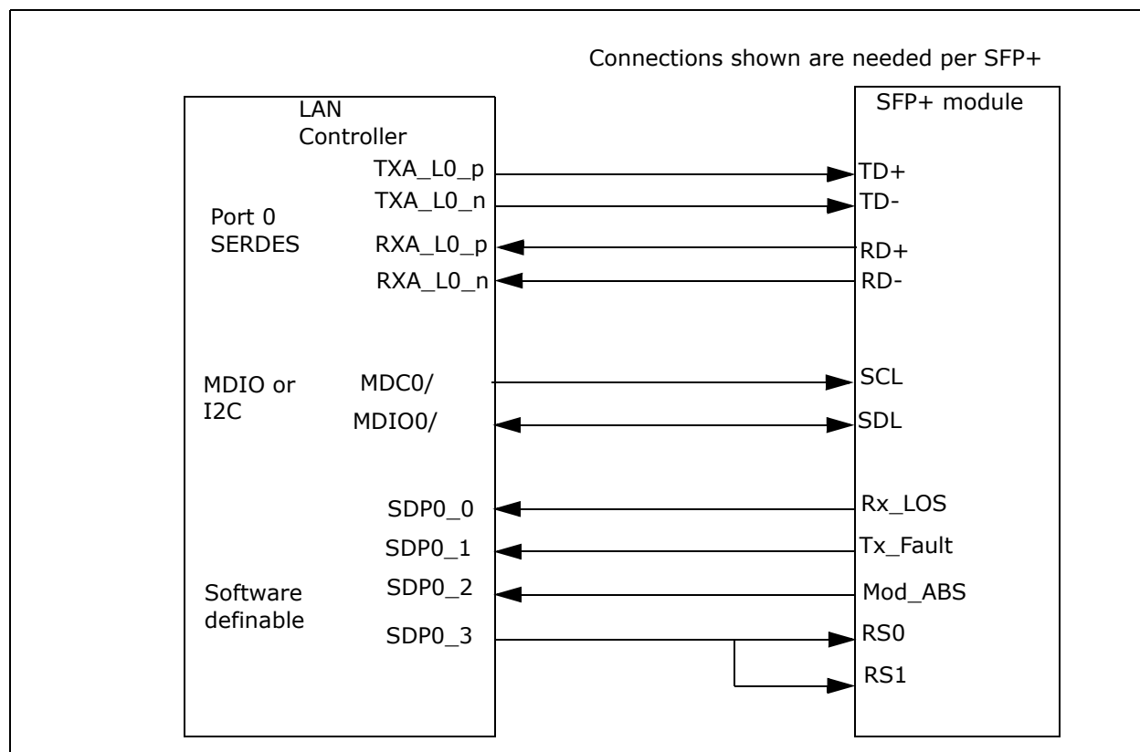
Figure 3-3. Fortville SDP connections to SFP+ module
