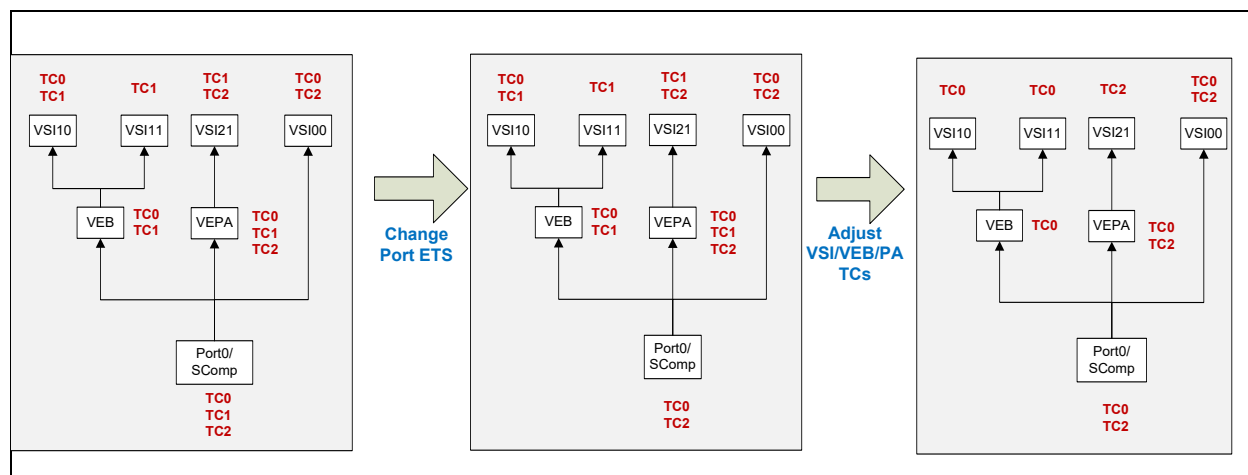
Figure 7-85. Change Physical Port ETS
