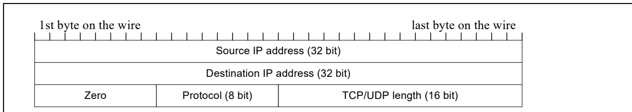
Figure 7-24. IPv4 pseudo header for TCP/UDP checksum
