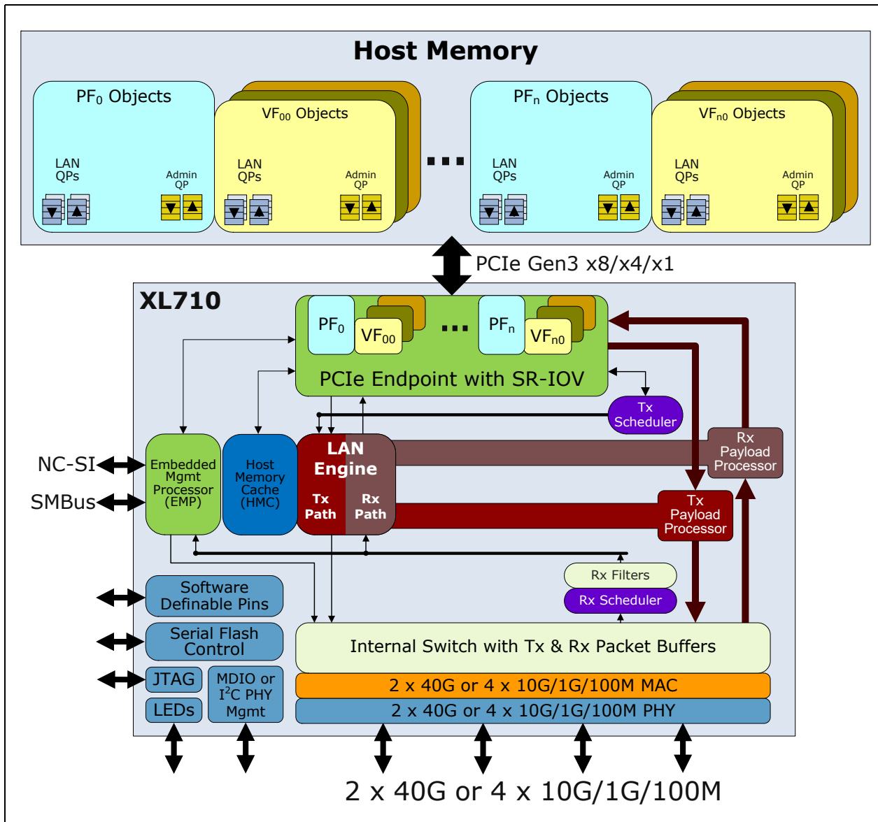
Figure 1-7. Fortville block diagram
