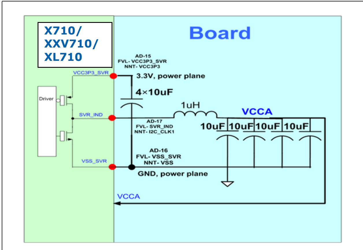
Figure 13-2. Fortville analog SVR board connectivity schematic illustration
