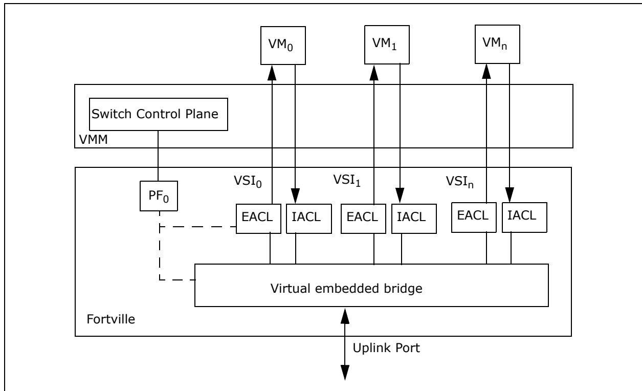
Figure 7-51. Switch control plane
