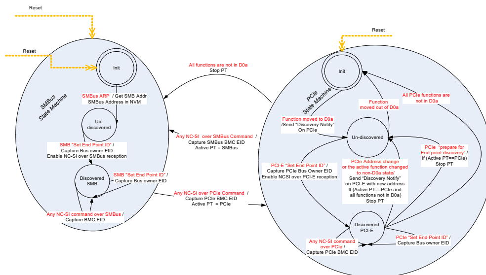
Figure 9-14. MCTP bus transition state machine
