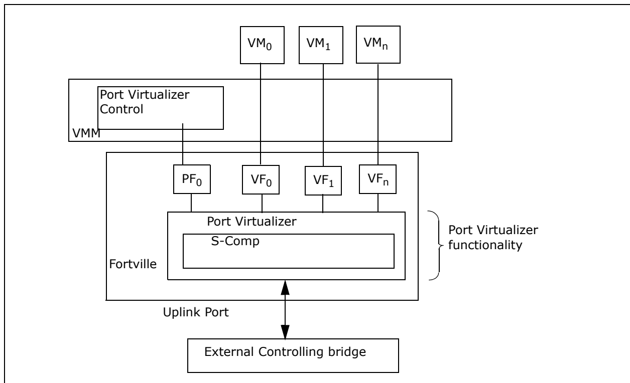
Figure 7-37. External switching configuration – port virtualizer
