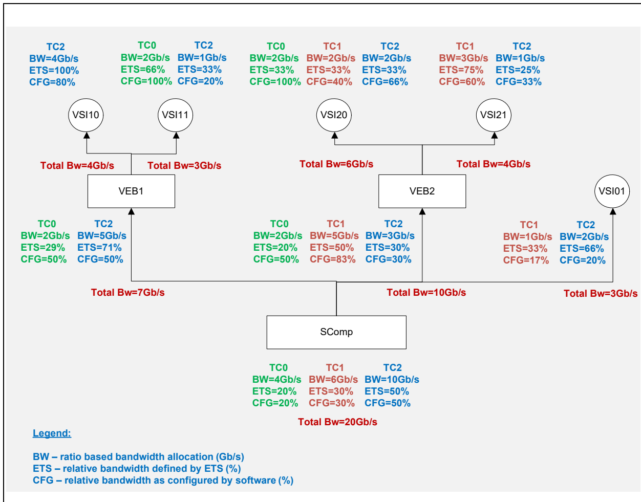
Figure 7-87. ETS-Based Scheme: Relative Bandwidth Calculation Example
