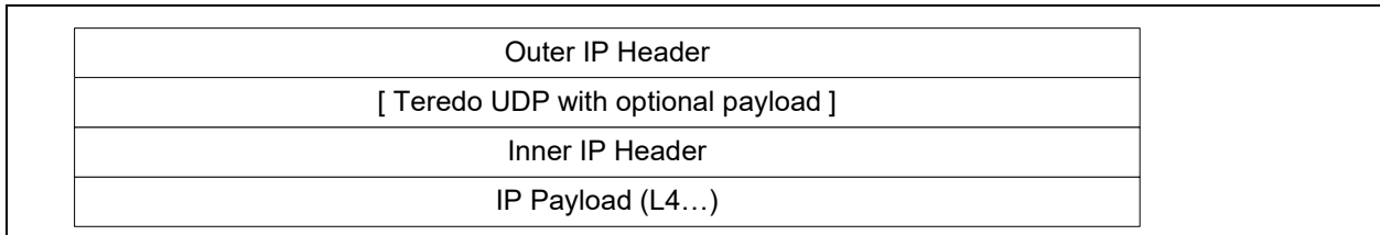
Figure 7-29. IP / Teredo tunneling
