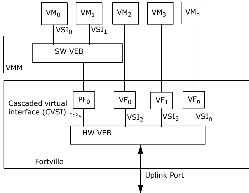
Figure 7-40. Cascaded VEB
