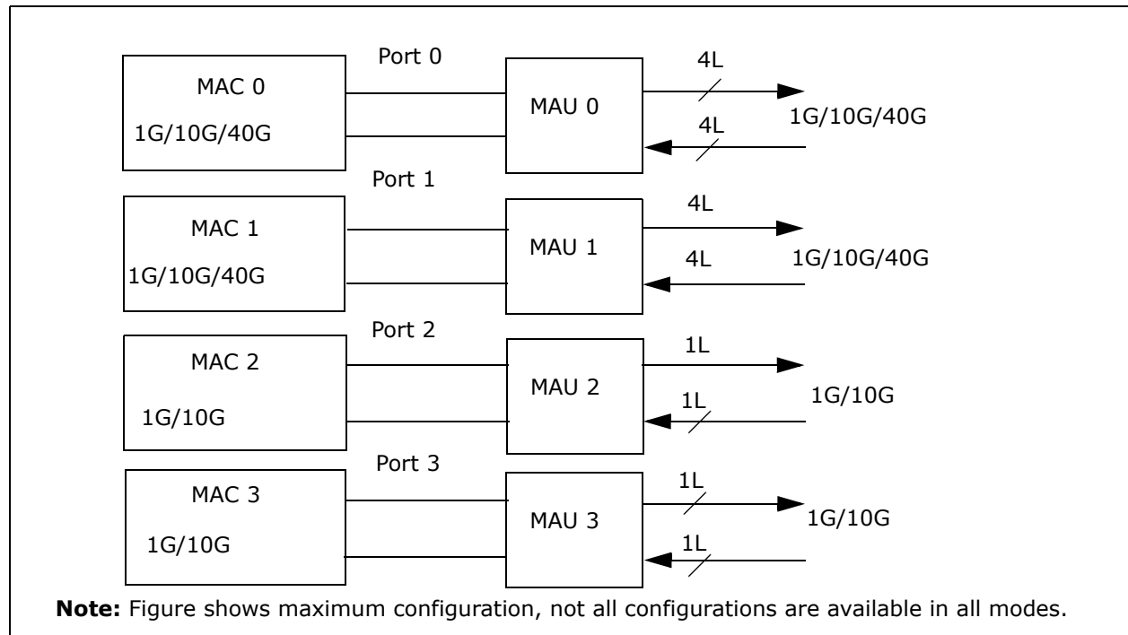
Figure 3-5. Fortville MAC and MAUI interfaces
