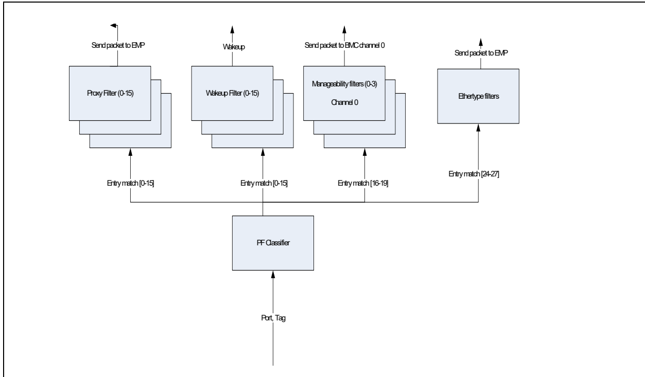
Figure 7-50. Out-of-band filtering operation
