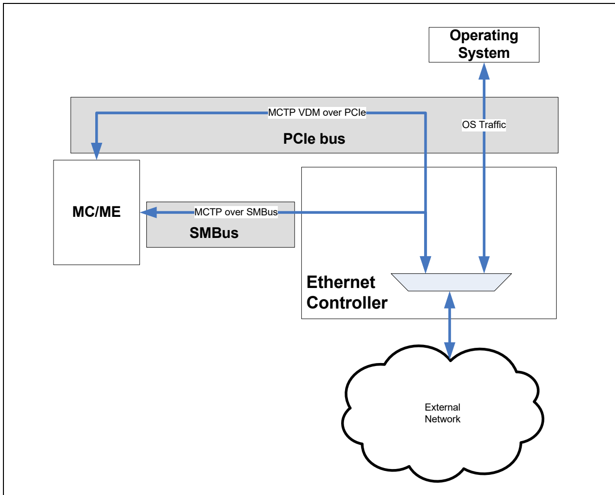
Figure 9-12. X710/XXV710/XL710 MCTP connections
