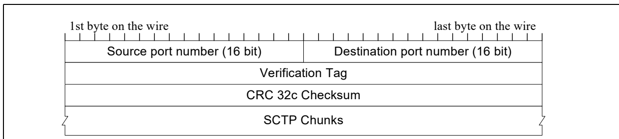
Figure 7-27. SCTP packet format
