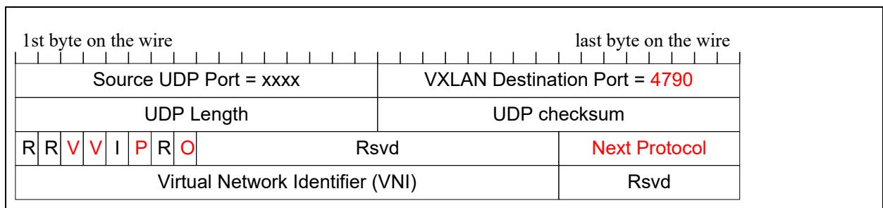
Figure 7-32. VXLAN-GPE header structure
