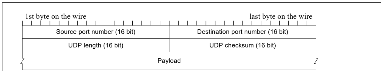
Figure 7-23. UDP packet format
