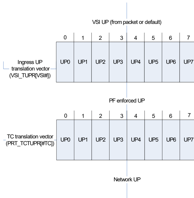
Figure 7-10. Example: Non-VLAN aware, non-DCB aware operating system
