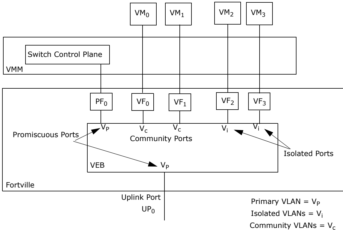
Figure 7-52. PVLAN configuration
