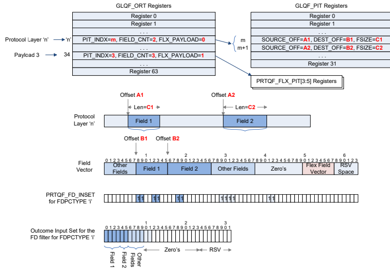
Figure 7-2. Input set example for an FD filter
