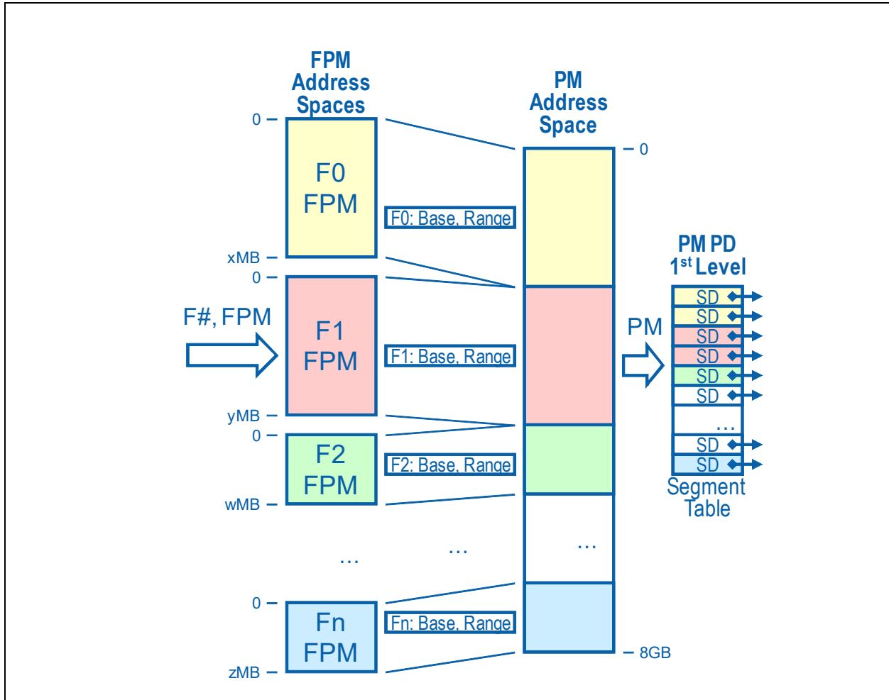
Figure 7-89. Host Memory Cache FPM Space
