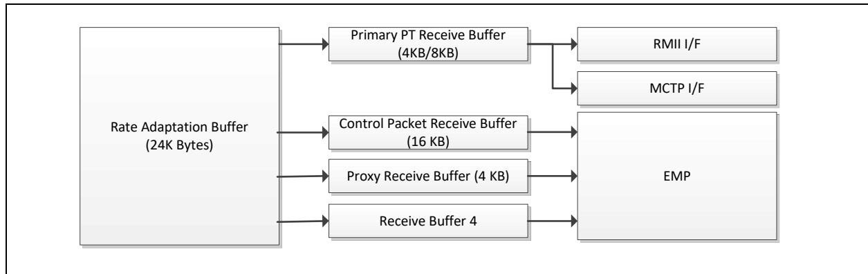
Figure 9-2. EMP Receive buffers
