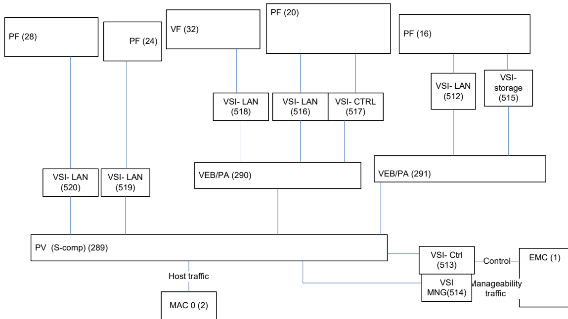
Figure 7-57. Port Virtualizer + VEB/VEPA
