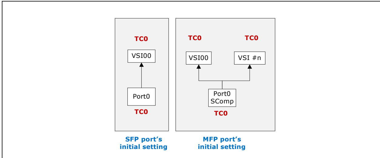
Figure 7-86. Initial setting in SFP (one initial VSI/Port) and MFP (one initial VSI/PF)
