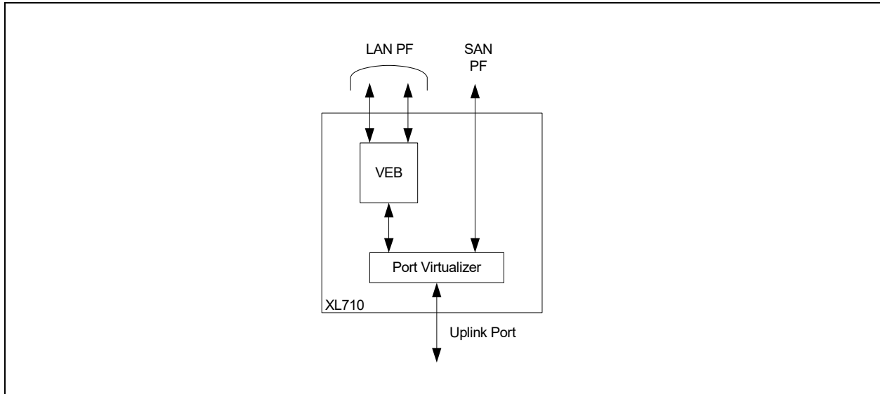
Figure 7-38. Internal switch configuration - LAN and SAN PFs
