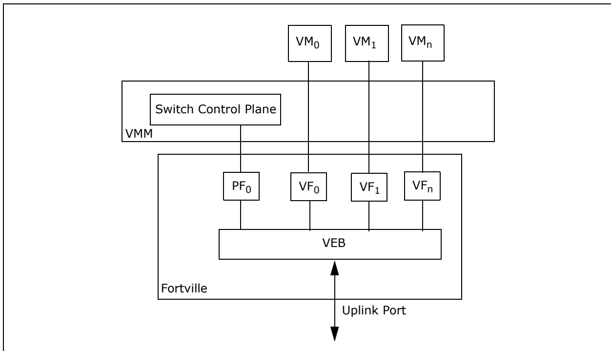
Figure 7-35. Internal switching configuration – hardware VEB
