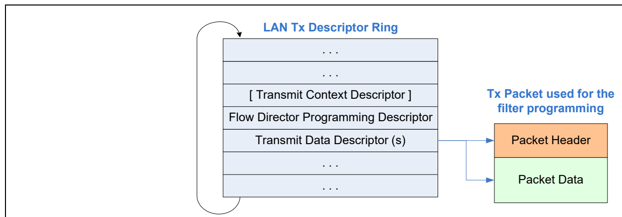
Figure 7-4. Flow director filter programming
