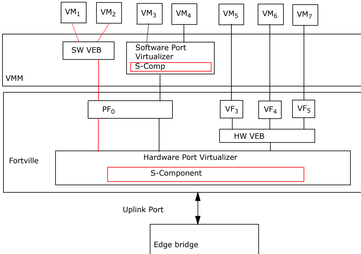
Figure 7-42. Cascaded VEB and port virtualizer
