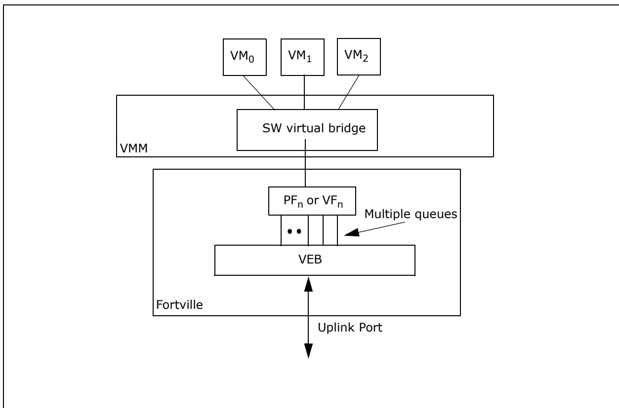
Figure 7-34. Internal switching configuration – software VEB
