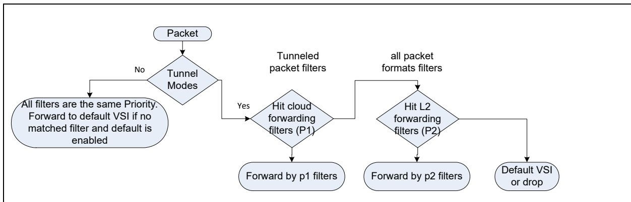
Figure 7-47. Cloud forwarding filters priority
