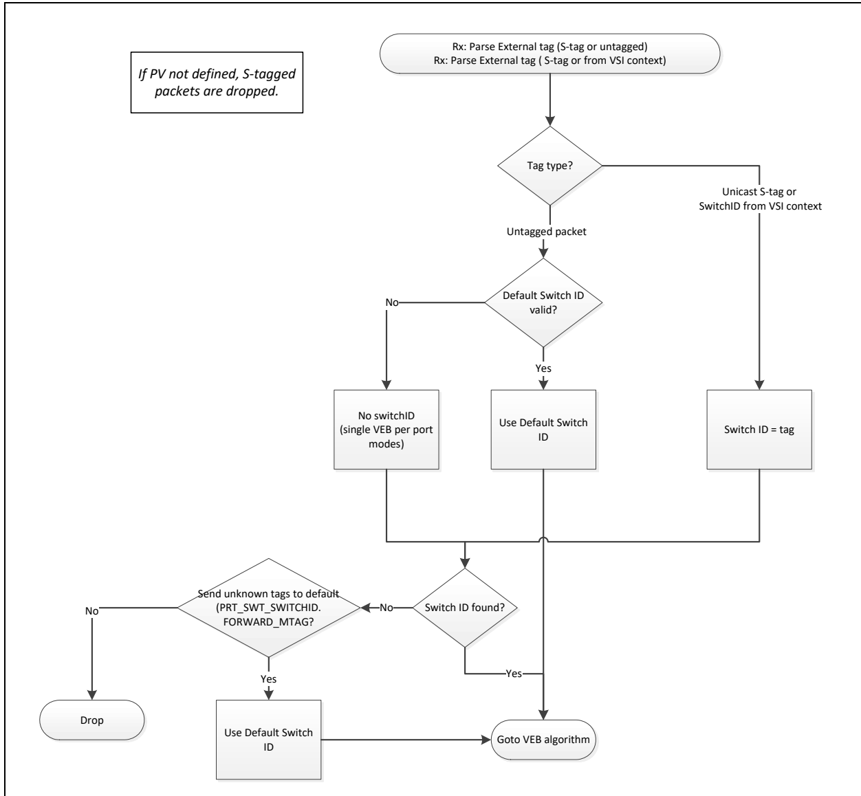
Figure 7-44. Port virtualizer flow
