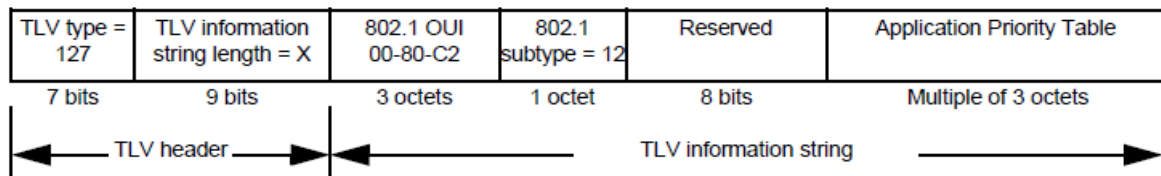
Figure 7-69. Application Priority Table TVL format
