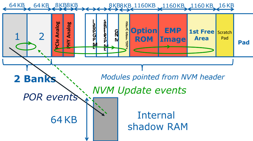
Figure 3-9. Flash high level map
