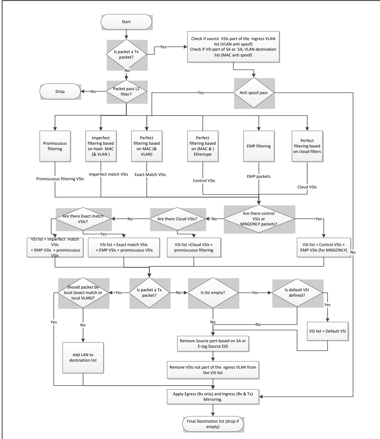
Figure 7-48. Cloud VEB flow diagram
