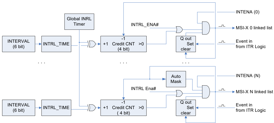
Figure 7-62. Interrupt rate limit (top-level description)
