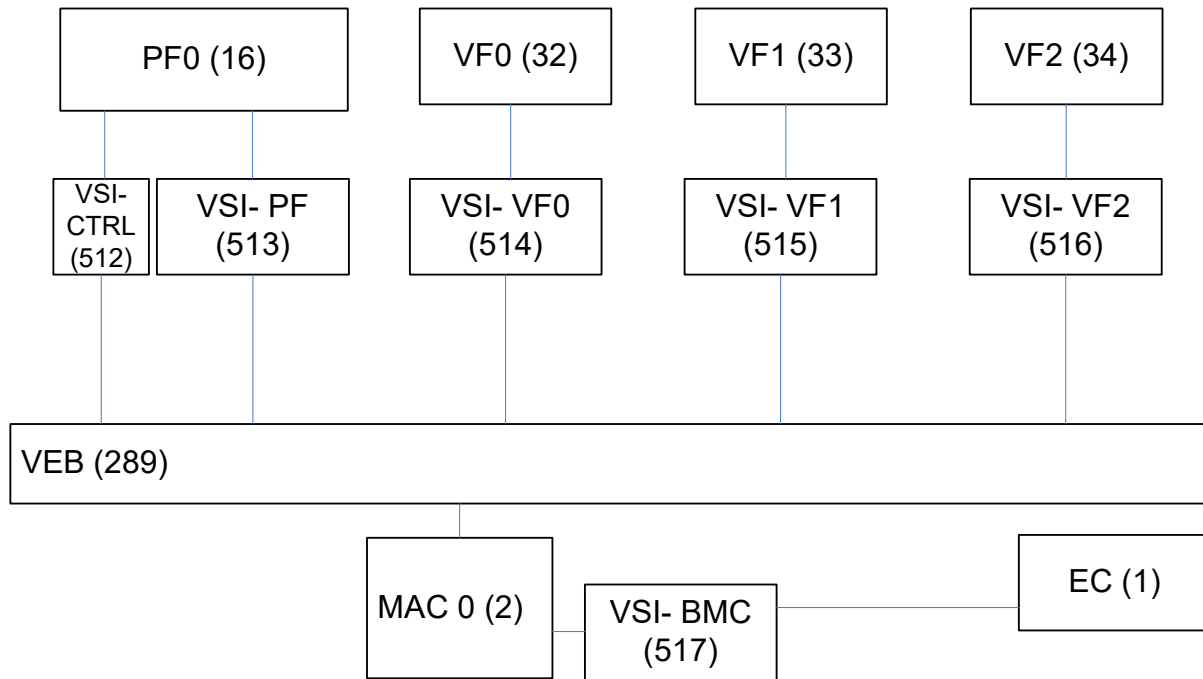
Figure 7-53. Switching structure Example
