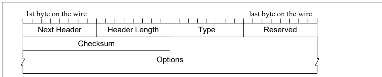
Figure 7-21. IPv6 mobility header
