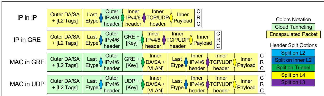
Figure 7-28. Tunneled packet formats
