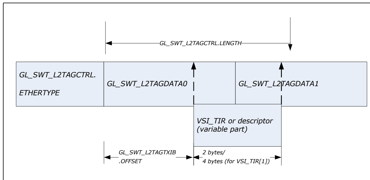
Figure 7-9. Tag insertion
