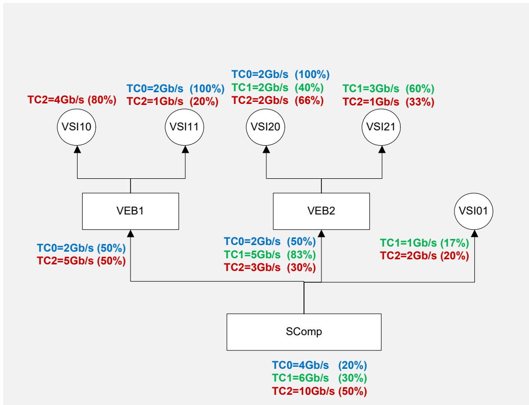
Figure 7-78. ETS-Based Bandwidth Configuration Example
