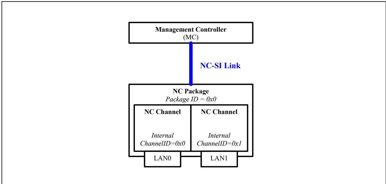
Figure 9-8. Single NC package, two NC channels
