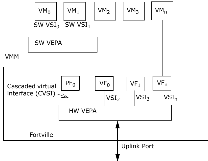
Figure 7-41. Cascaded VEPA
