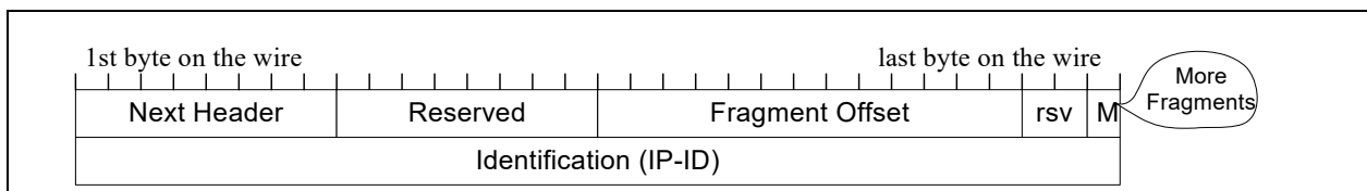
Figure 7-19. IPv6 fragment header
