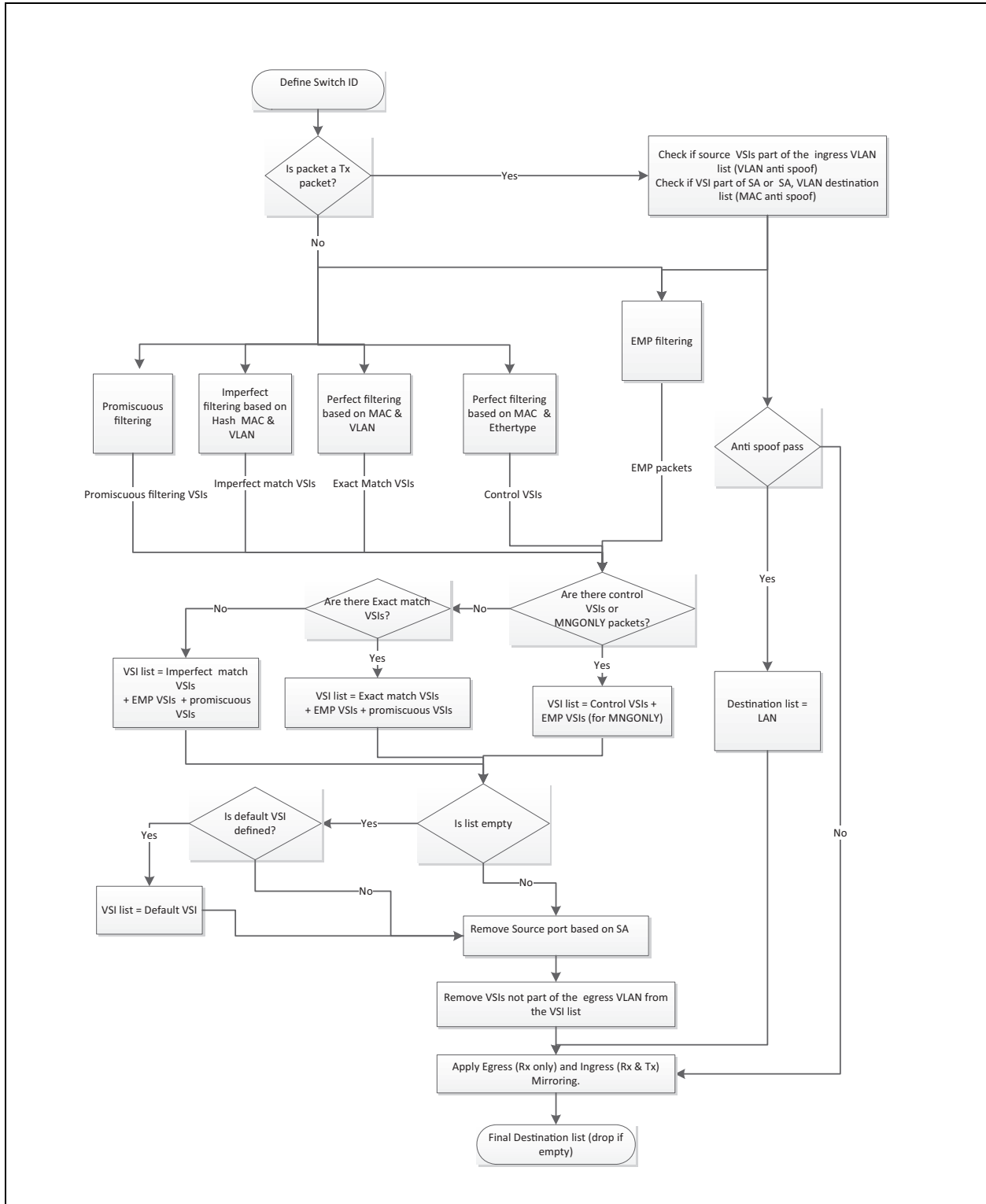
Figure 7-49. VEBA flow diagram
