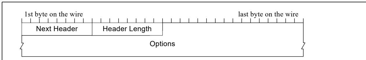
Figure 7-20. IPv6 destination options
