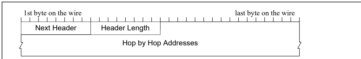
Figure 7-17. IPv6 hop-by-hop extension header
