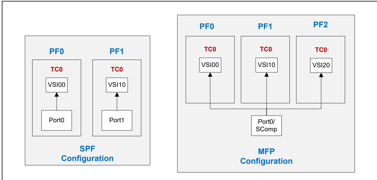
Figure 7-79. Default VSI Configuration
