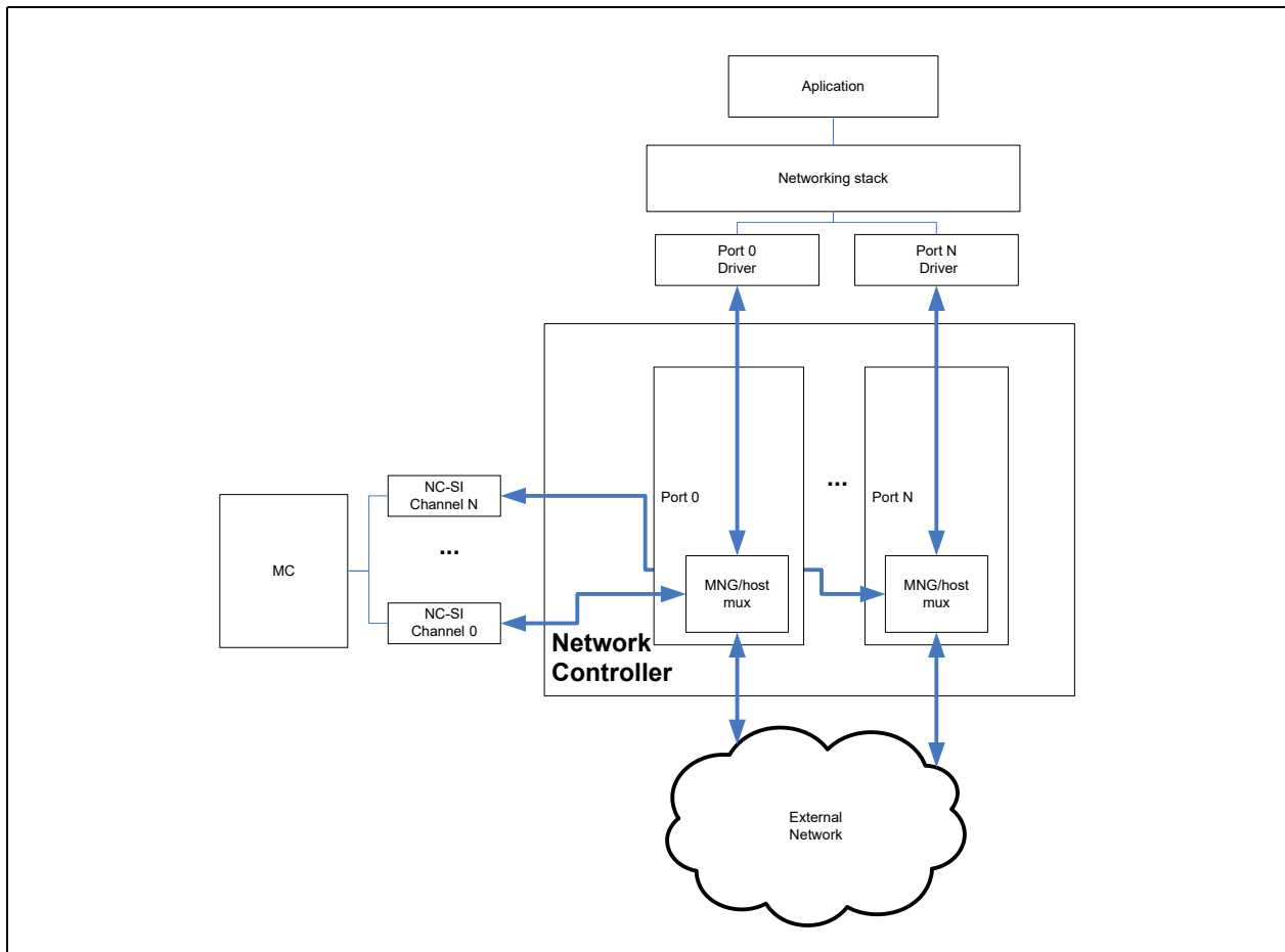
Figure 9-6. Operating System-to-MC flow
