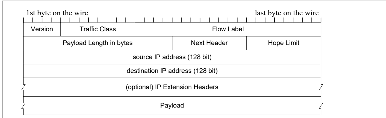
Figure 7-16. IPv6 datagram
