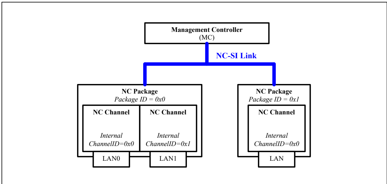
Figure 9-9. Two NC packages (left, with two NC channels and right, with one NC channel)
