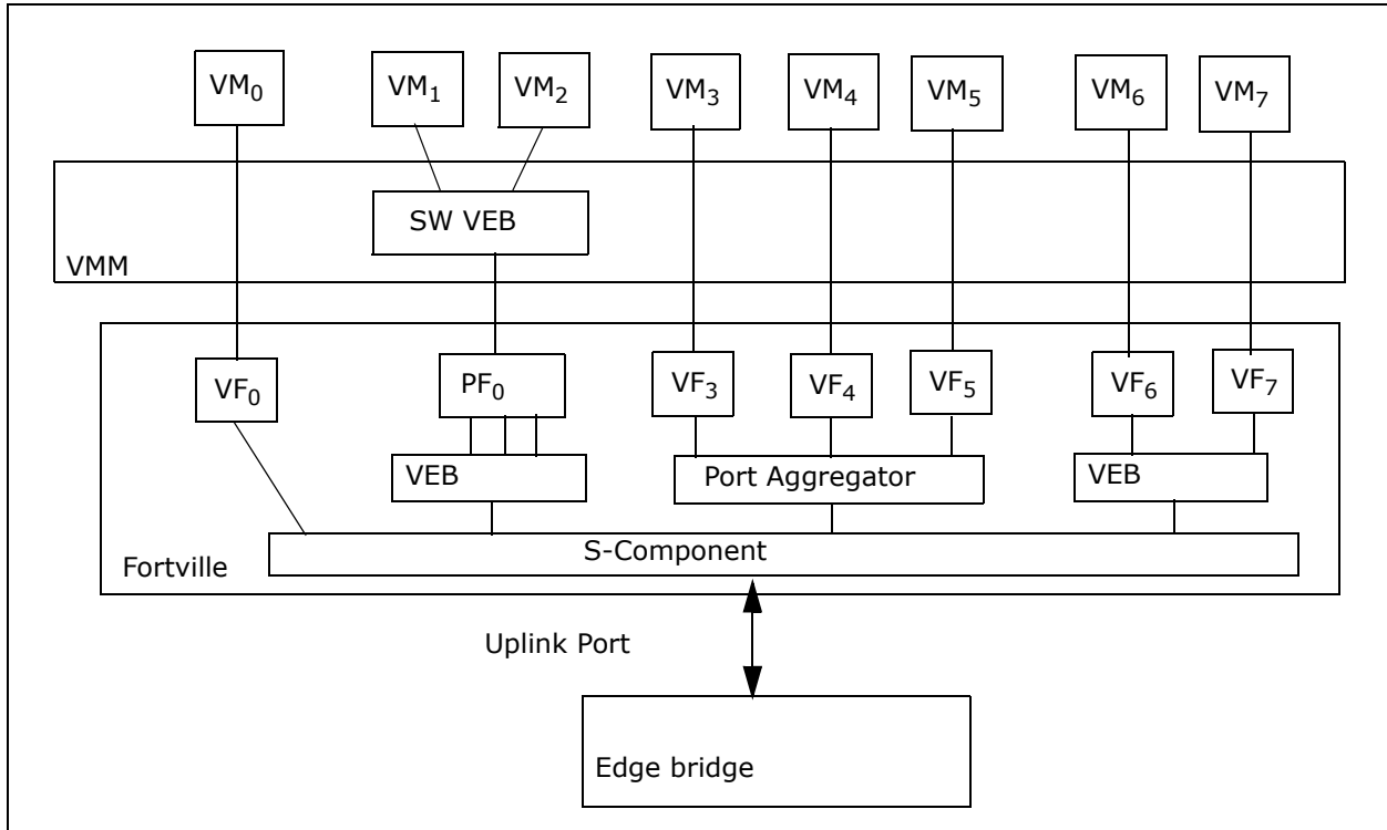
Figure 7-39. Cascaded VEB
