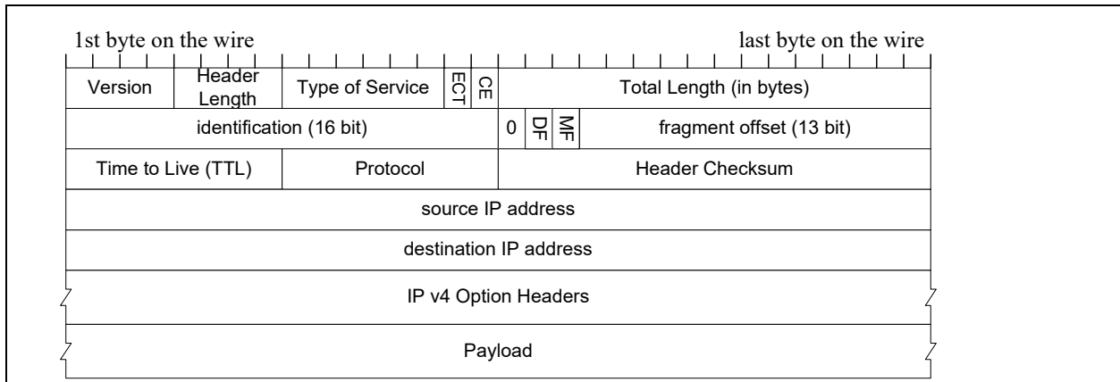
Figure 7-15. IPv4 datagram
