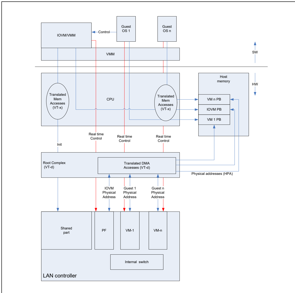
Figure 7-64. SR-IOV Based System
