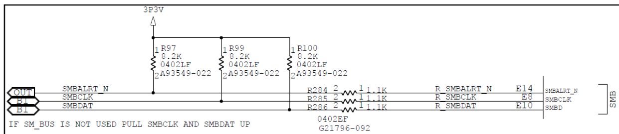
Figure 14-3. SMBus Connections
