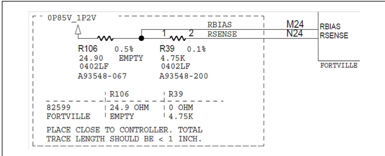
Figure 13-23. Fortville Bias Circuit
