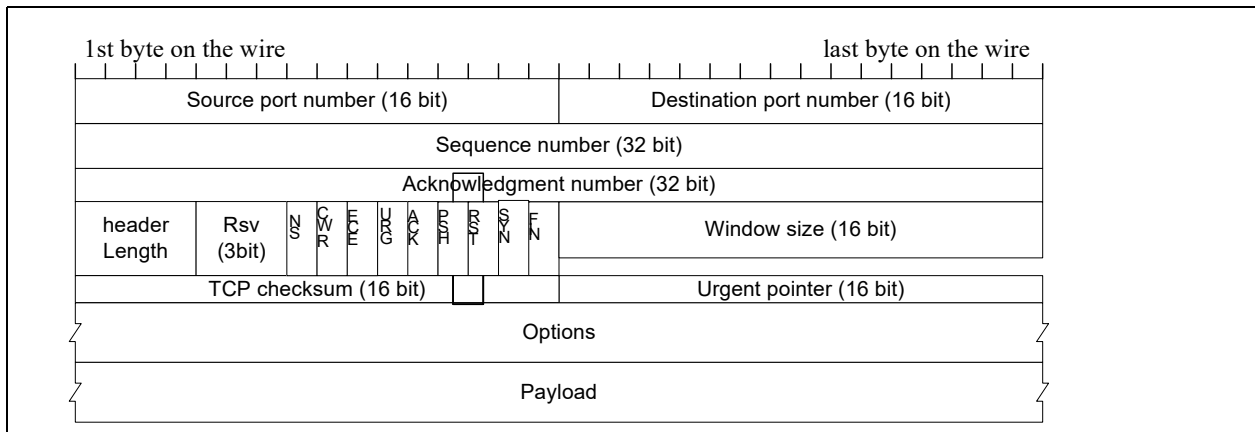
Figure 7-26. TCP packet format
