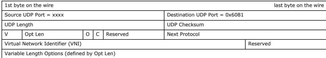
Figure 7-31. Geneve header structure
