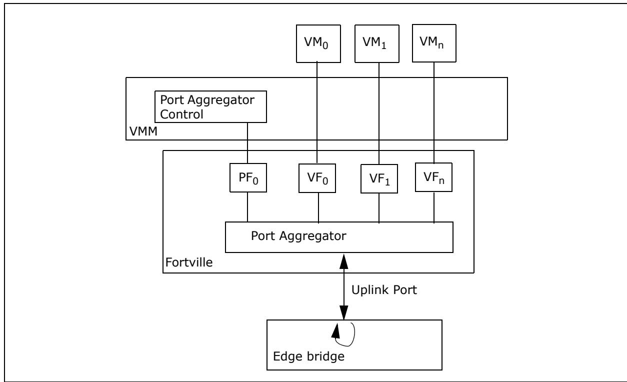
Figure 7-36. External switching configuration – virtual port aggregator
