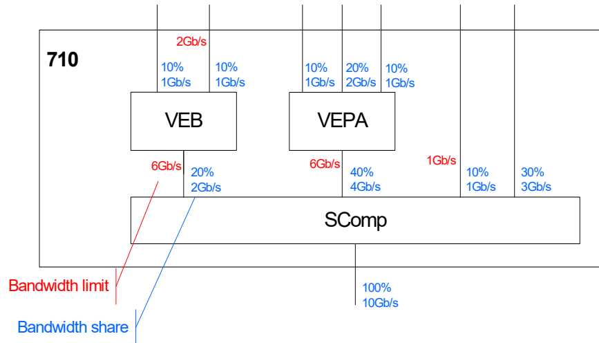
Figure 7-75. Example of Limiting Maximum Bandwidth
