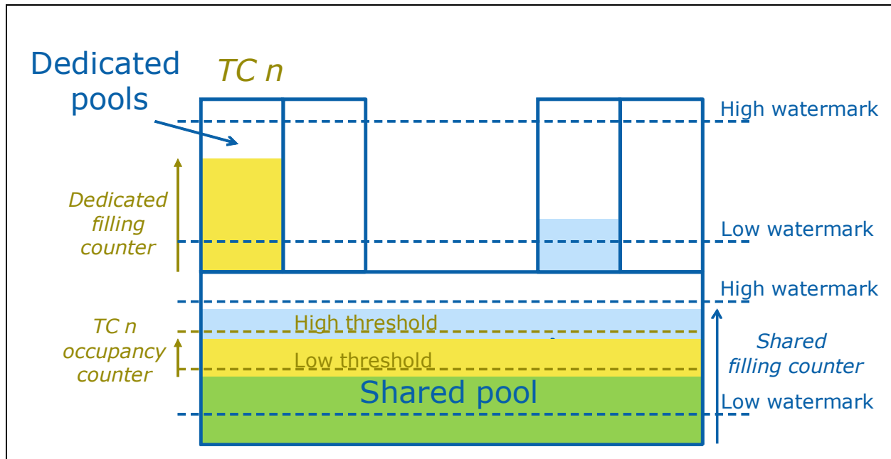
Figure 7-65. Normal Partitioning of the Per Port Rx Packet Buffer
