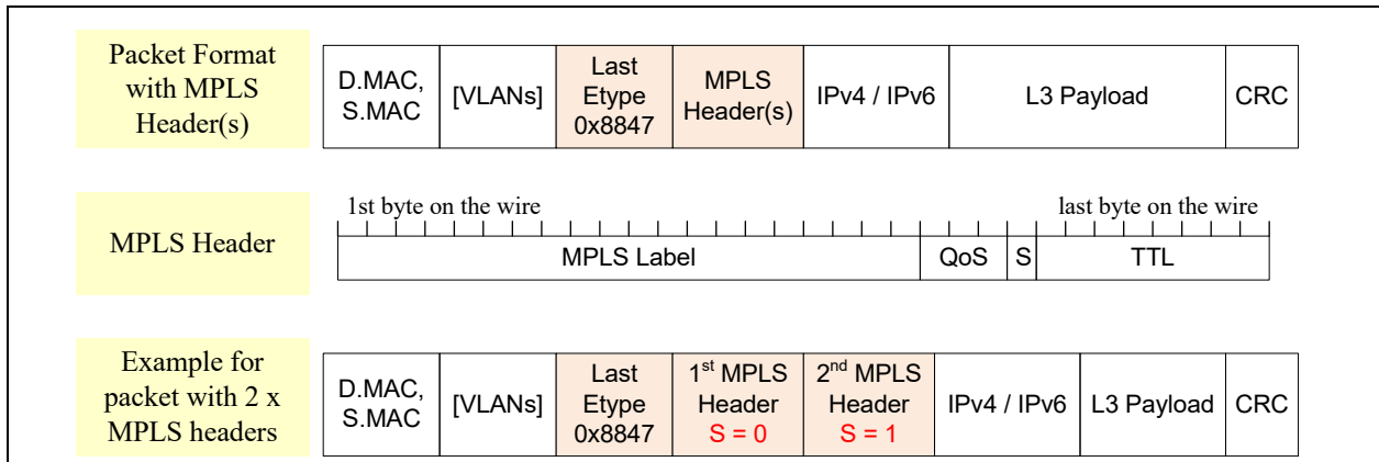
Figure 7-14. MPLS header
