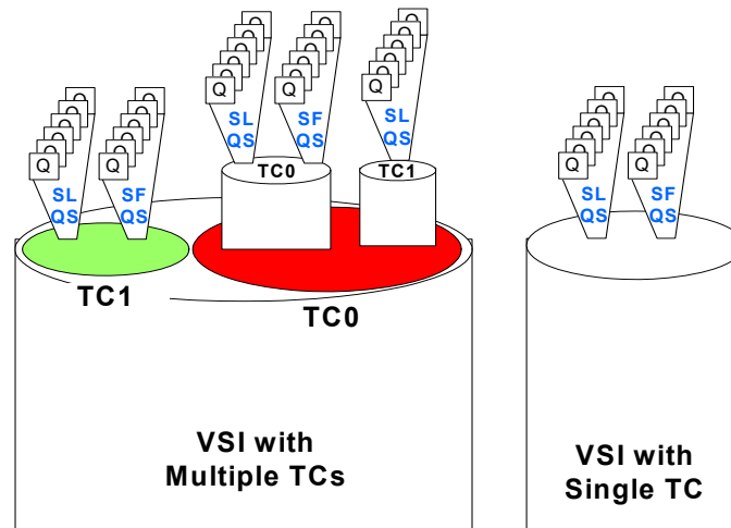
Figure 7-76. Queue Set Assignment Diagram
