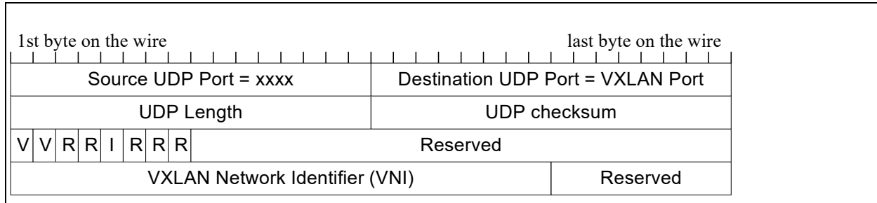
Figure 7-30. VXLAN header structure
