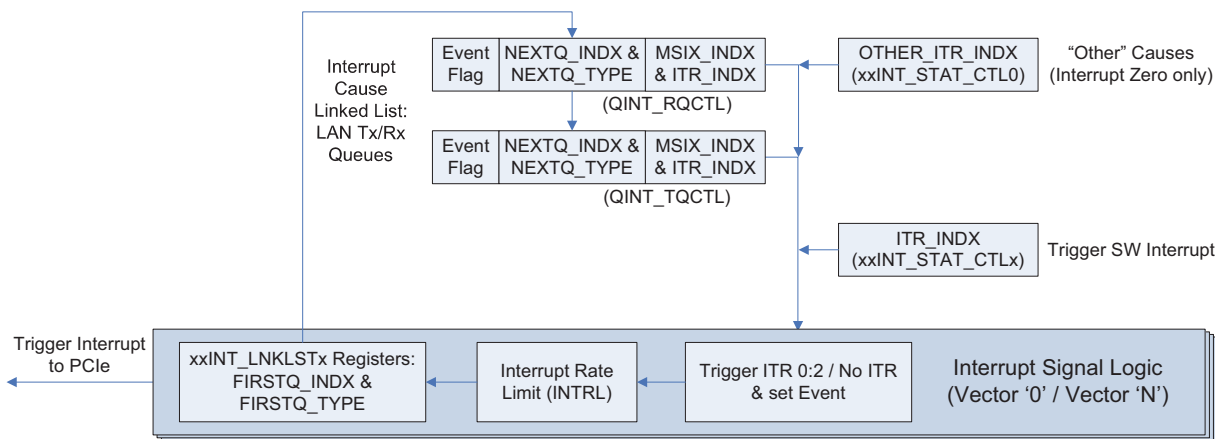
Figure 7-60. Mapping interrupt causes to interrupt signaling
