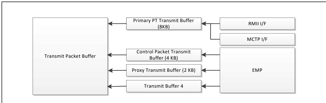
Figure 9-3. EMP Transmit buffers
