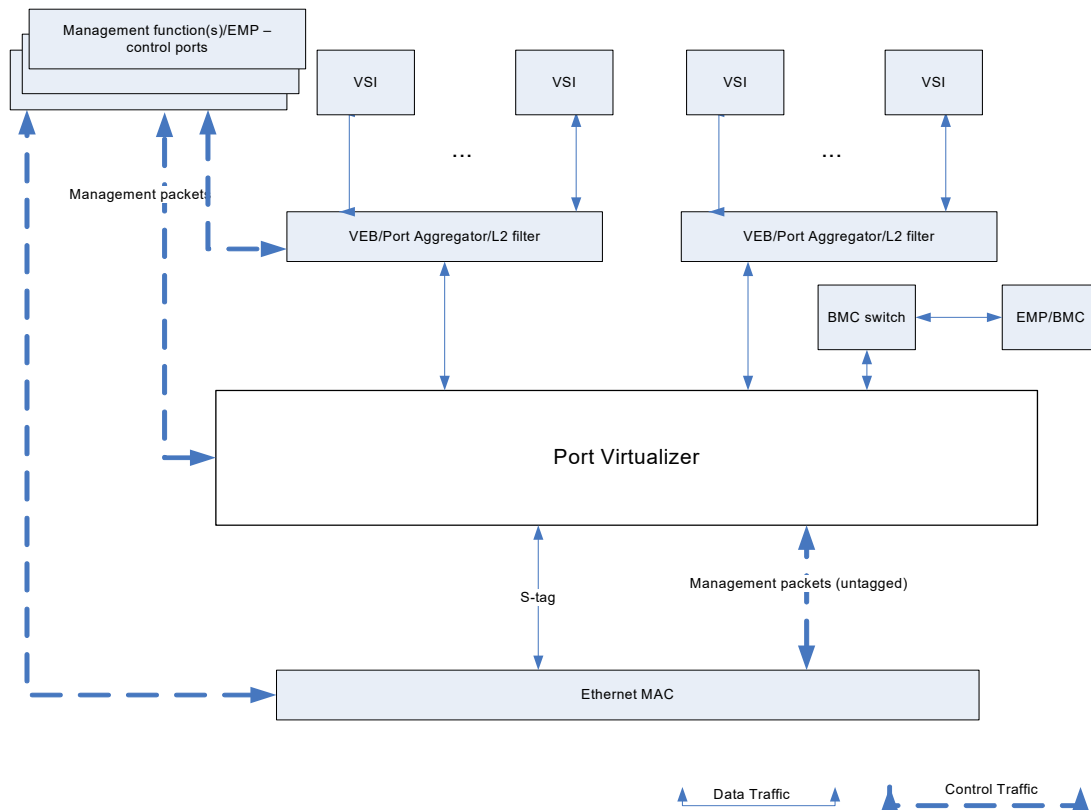
Figure 7-43. Switching elements per port
