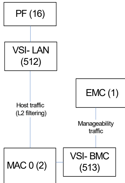
Figure 7-54. Switch Configuration - Basic L2
