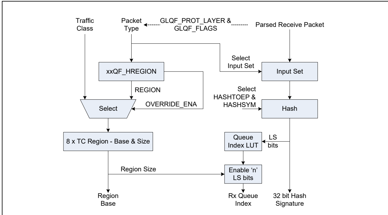
Figure 7-3. RSS block diagram
