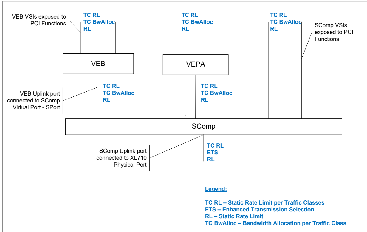
Figure 7-73. Fortville Bandwidth Management Attributes
