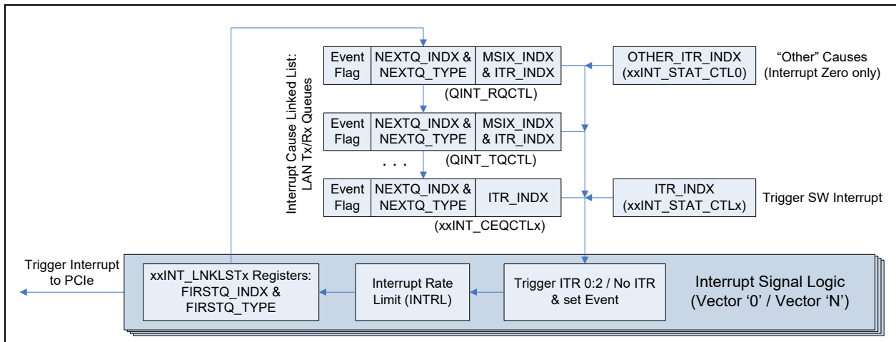
Figure 7-61. Mapping Interrupt Causes to Interrupt Signaling
