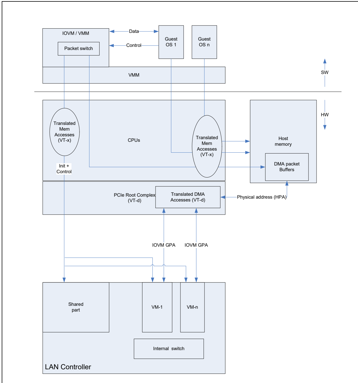
Figure 7-63. VMDq System
