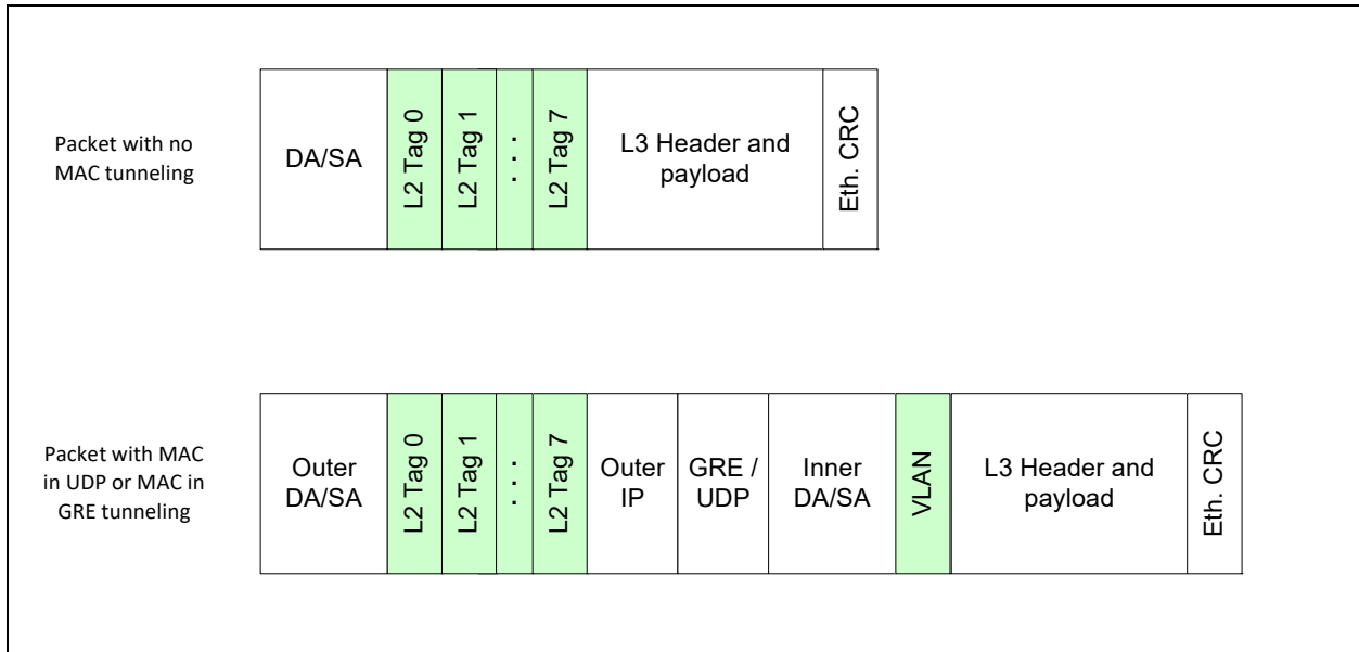
Figure 7-7. L2 tags order
