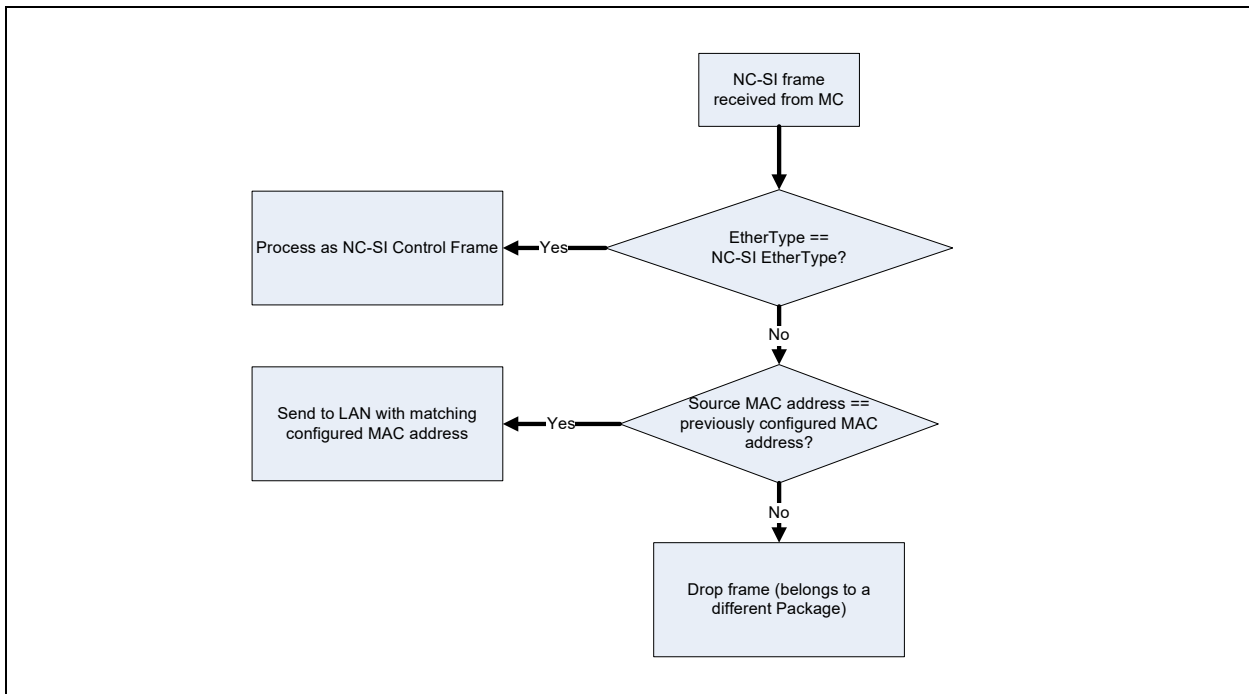
Figure 9-10. NC-SI frames receive flow for the NC
