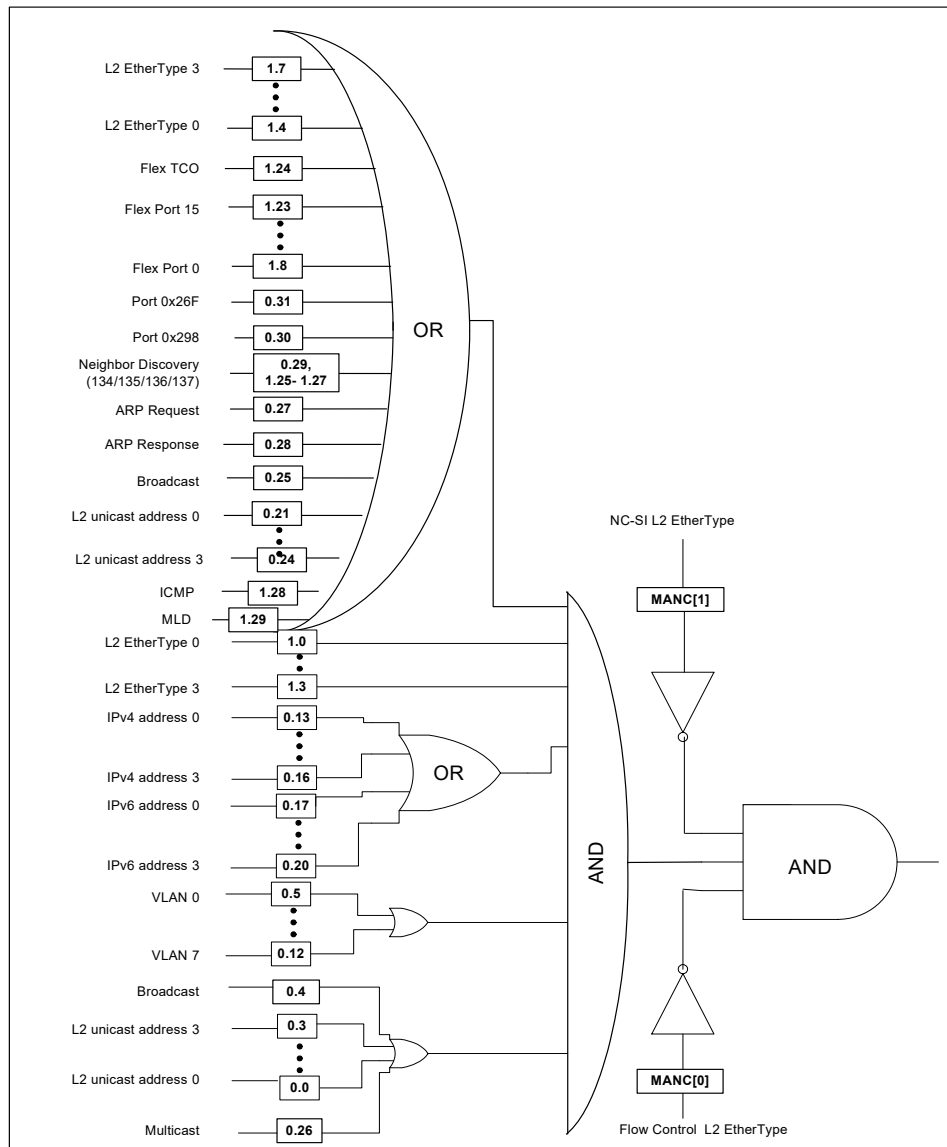
Figure 9-5. Manageability decision filters
