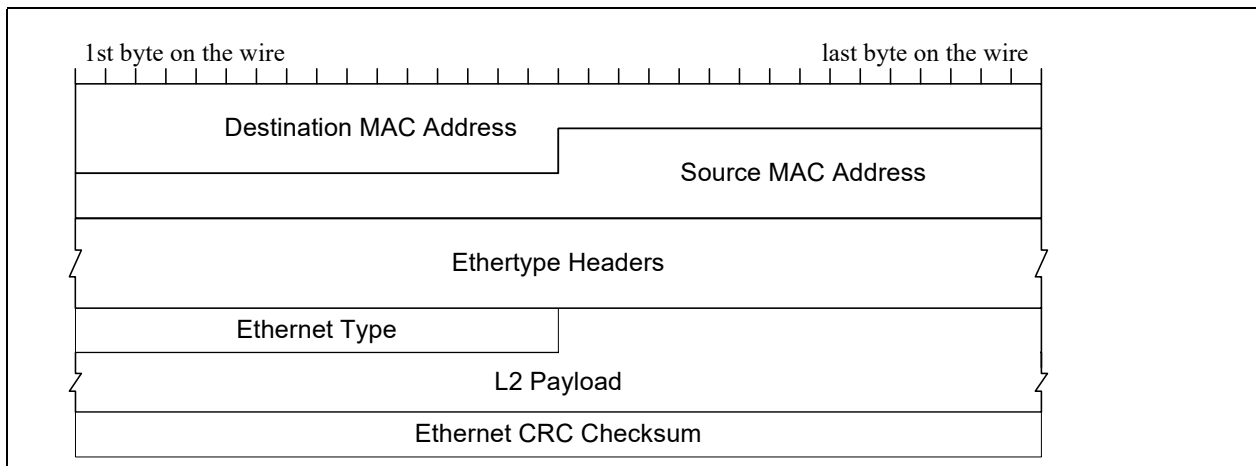
Figure 7-12. Standard L2 Frame format
