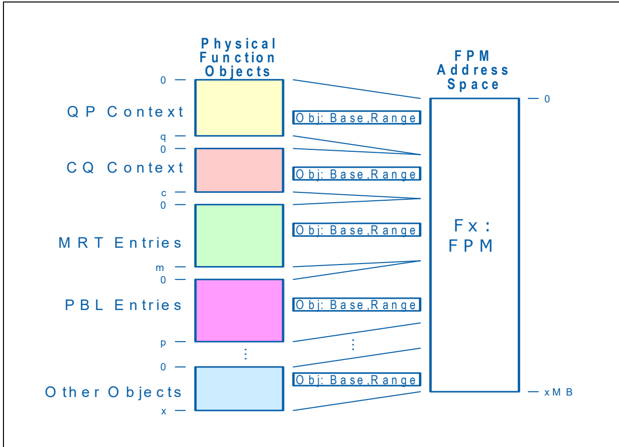
Figure 7-90. Host Memory Cache FPM Object Access
