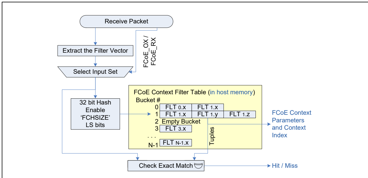
Figure 7-6. FCoE Context Filter Table
