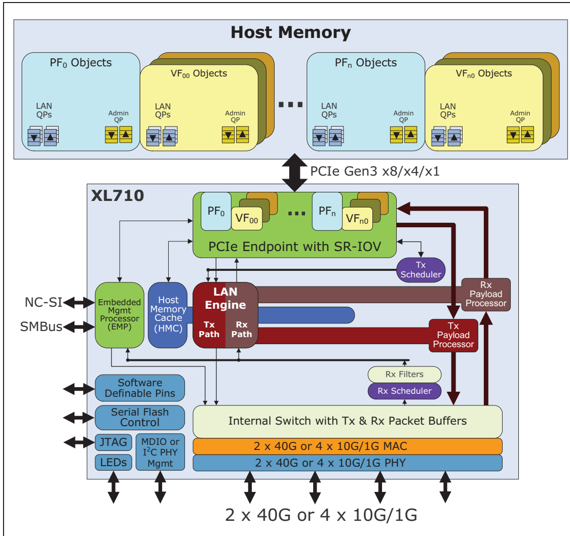
Figure 1-5. Fortville block diagram
