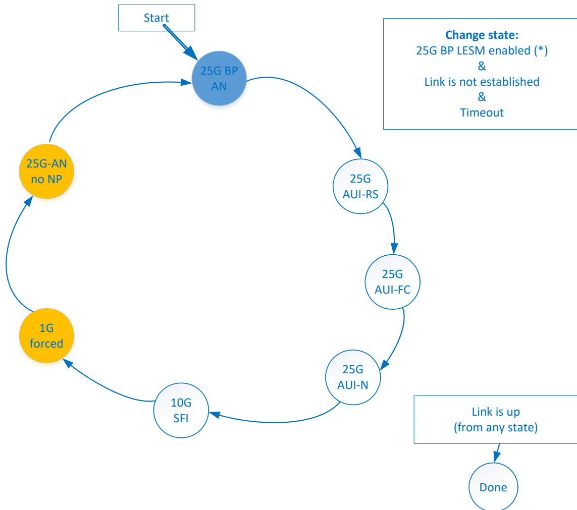
Figure 3-7. 25 GbE Backplane LESM Diagram
