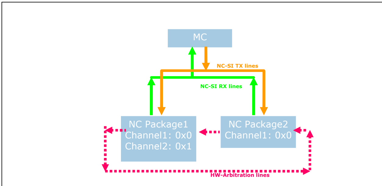
Figure 9-11. Multi-NC environment
