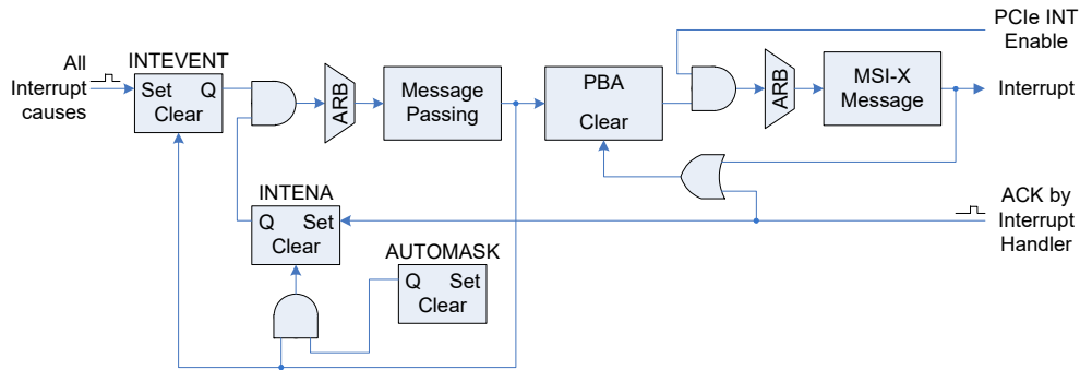
Figure 7-59. Conceptual interrupt logic
