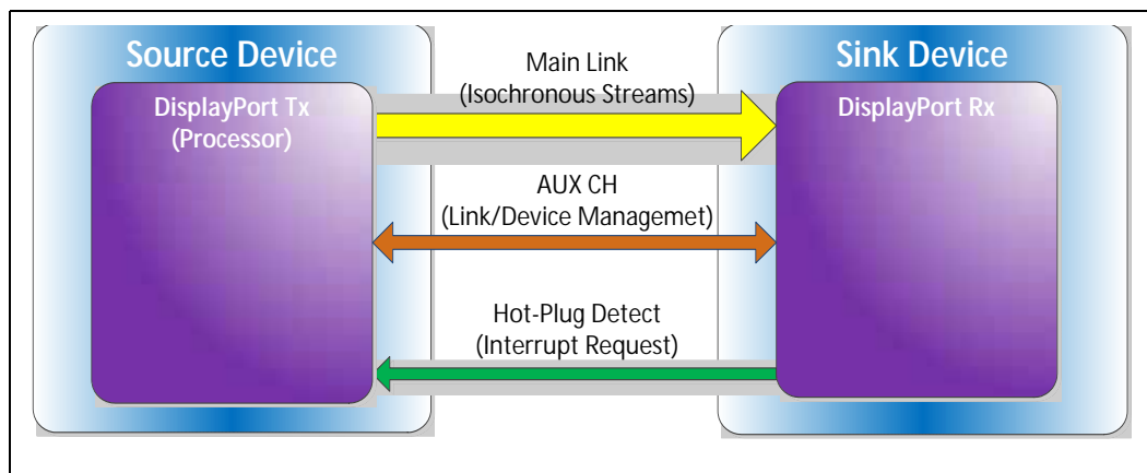
Figure 2-6. DisplayPort* Overview
