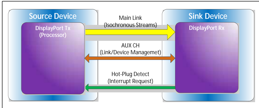
Figure 2-7. DisplayPort* Overview
