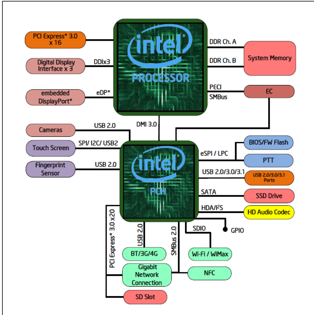
Figure 1-1. H-Processor Line Platforms
