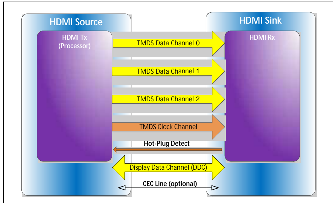
Figure 2-8. HDMI * Overview
