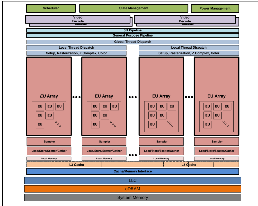
Figure 2-5. Gen 9 LP Block Diagram
