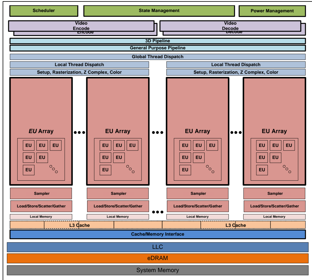
Figure 2-6. Gen 9 LP Block Diagram
