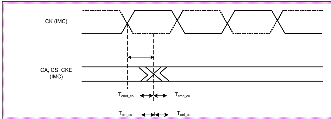
Figure 7-5. DDR Data Setup and Hold Timing Waveform
