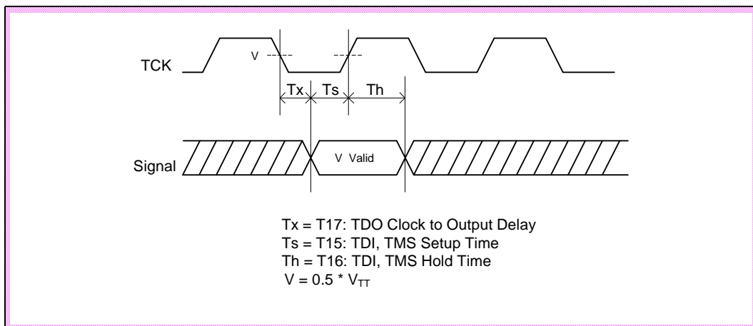
Figure 7-6. TAP Valid Delay Timing Waveform
