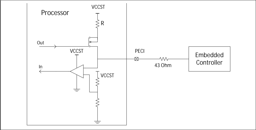
Figure 2-11. Example for PECE EC Connection
