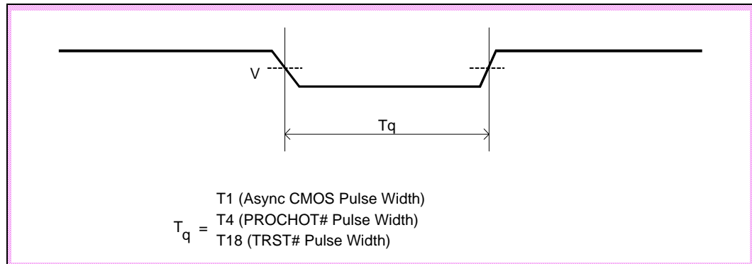
Figure 7-7. Test Reset (TRST#), Async Input, and PROCHOT# Output Timing Waveform
