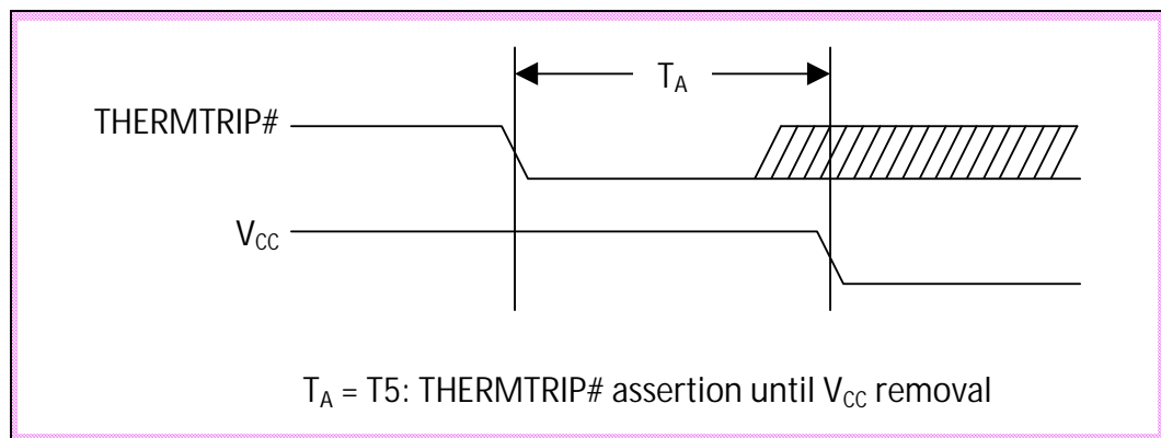
Figure 7-8. THERMTRIP# Power Down Sequence
