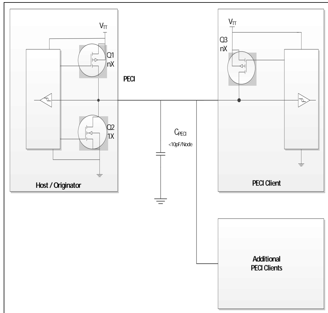
Figure 2-10. Example for PECE Host-Clients Connection
