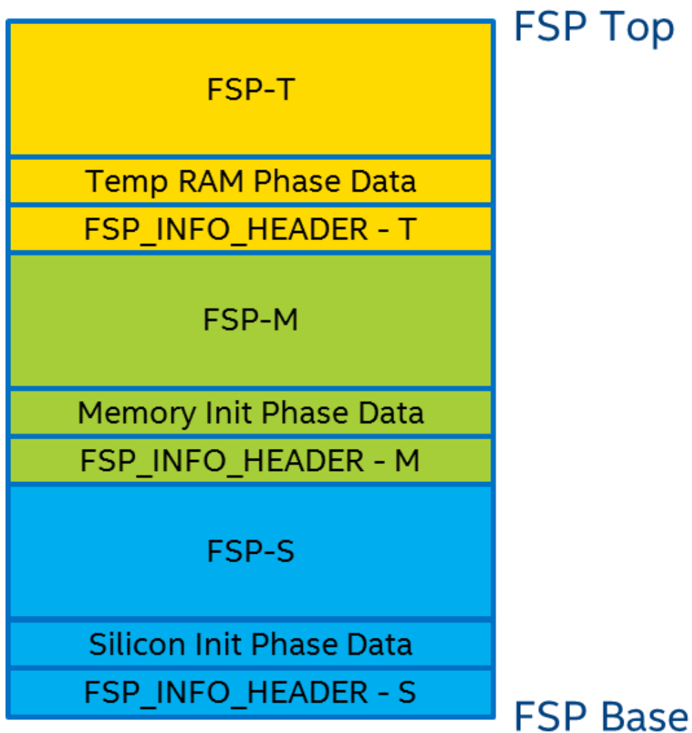
Figure 2: Intel® FSP Component Layout View
