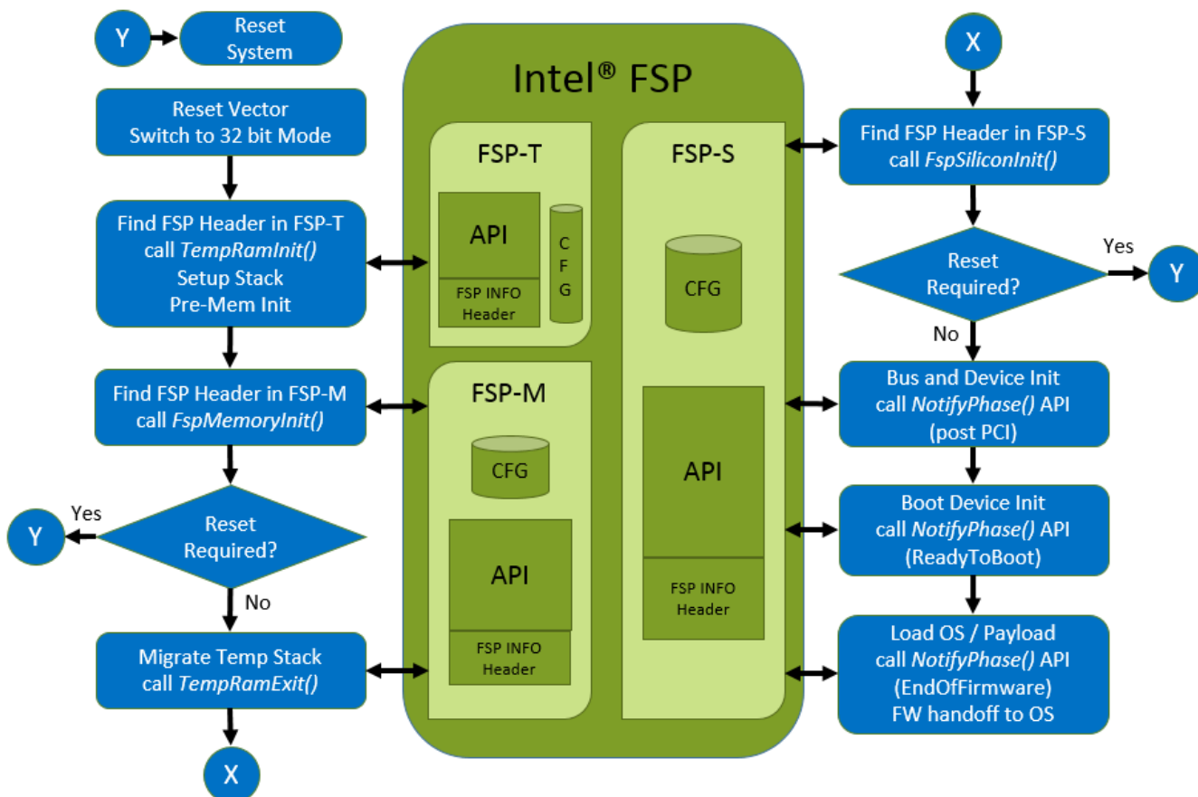
Figure 4: API Mode Boot Flow
