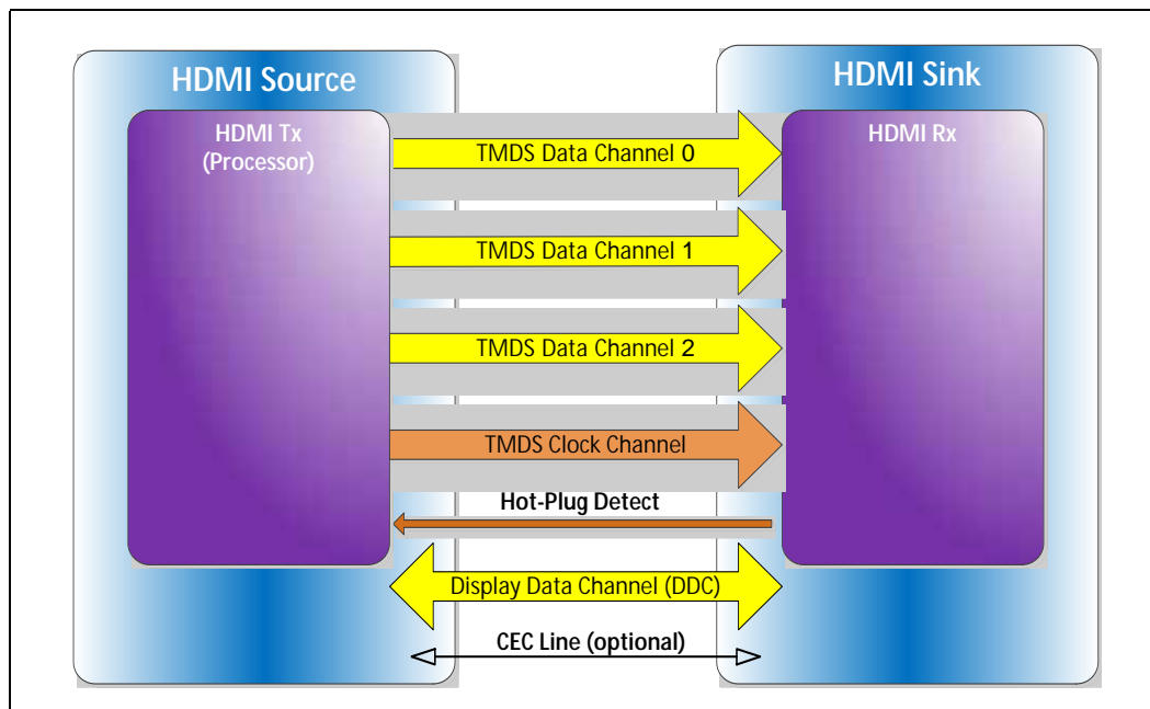
Figure 2-7. HDMI* Overview
