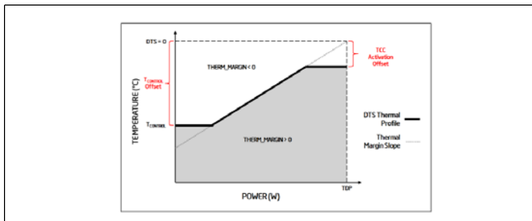
Figure 5-8. Digital Thermal Sensor (DTS) 1.1 Definition Points
