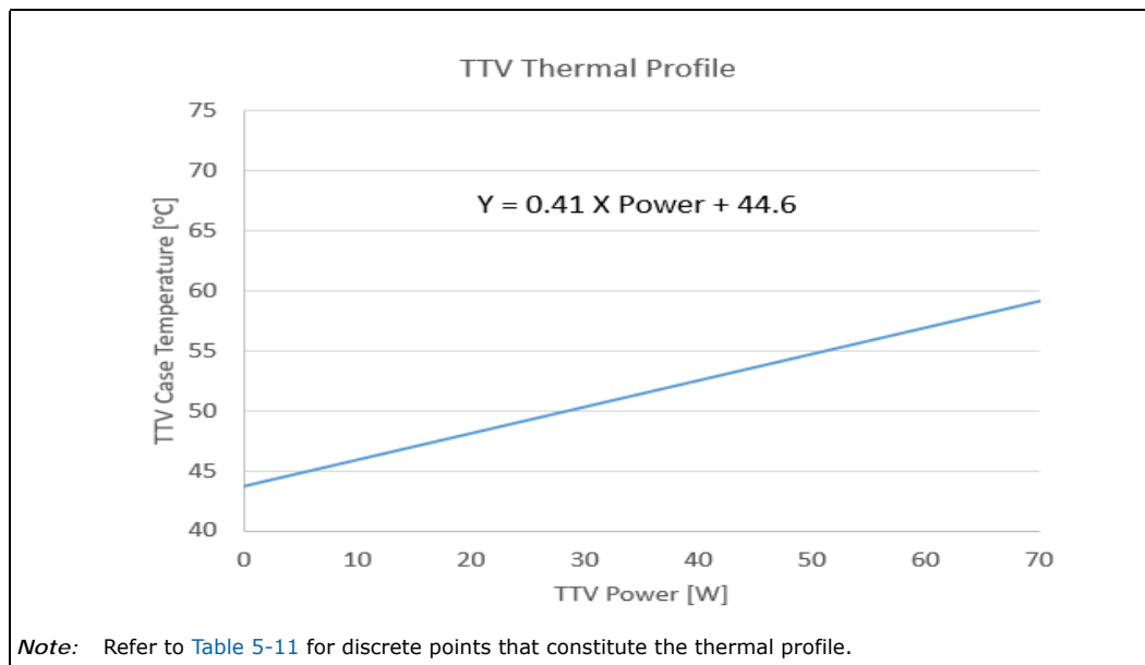
Figure 5-3. Thermal Test Vehicle Thermal Profile for PCG 2015C Processor
