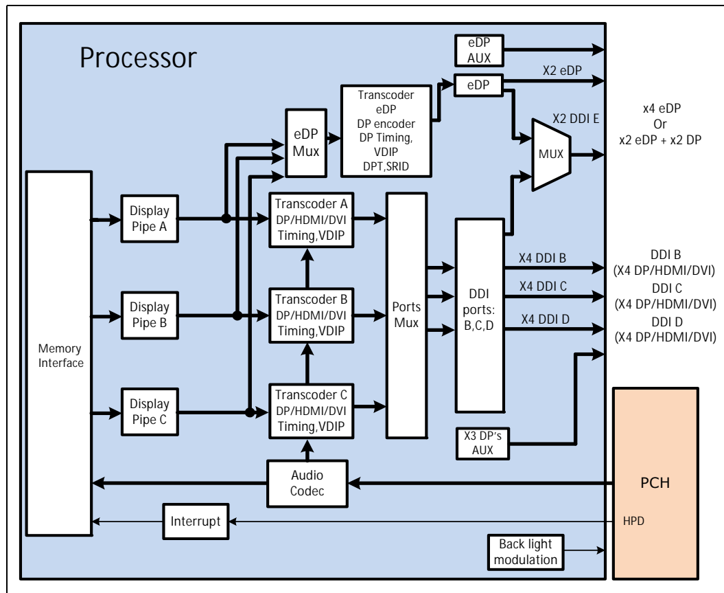
Figure 2-5. Processor Display Architecture (With Three DDI Ports as an Example)
