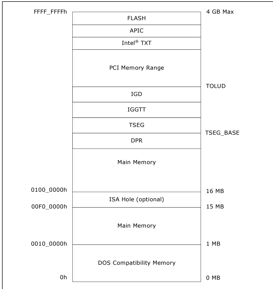
Figure 2-5. Main Memory Address Range
