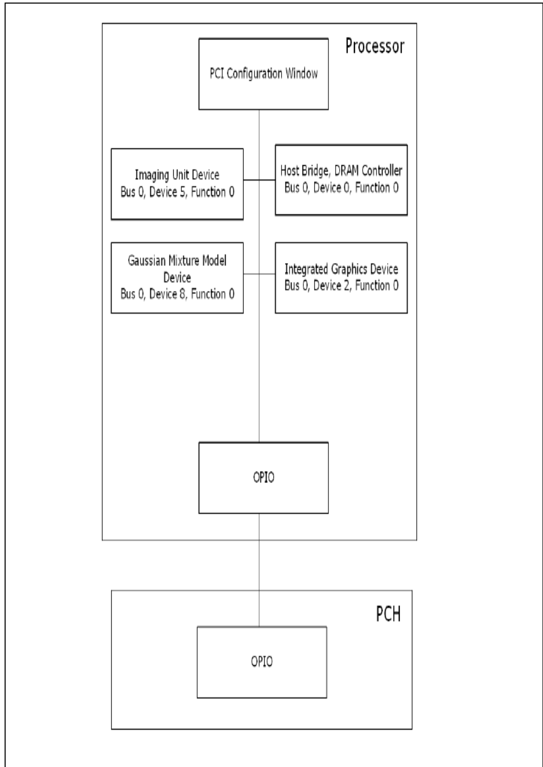
Figure 2-1. Conceptual Platform PCI Configuration Diagram
