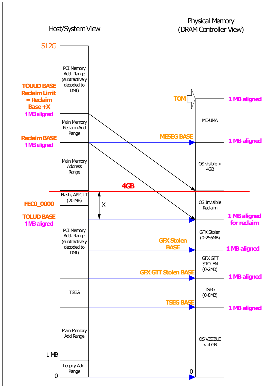
Figure 2-2. System Address Range Example
