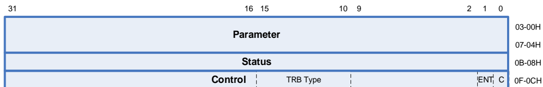
Figure 4-13: TRB Template
