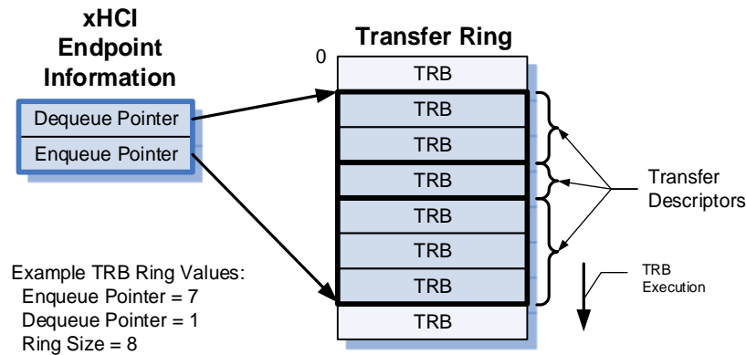
Figure 3-4: Transfer Ring 2
