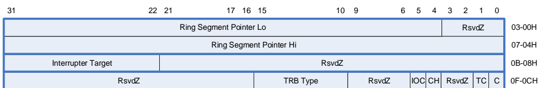
Figure 6-38: Link TRB
