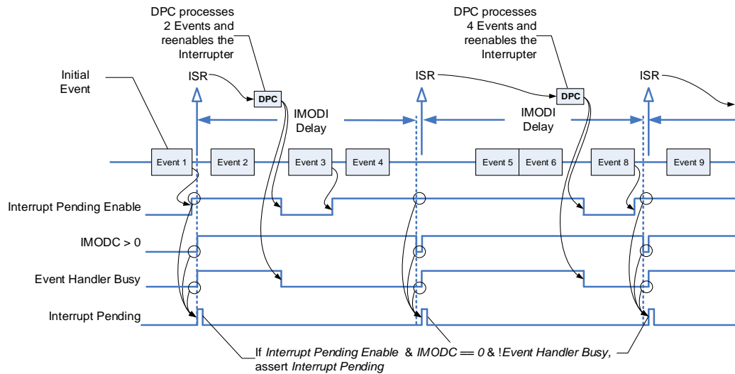
Figure 4-23: Heavy load, interrupts moderated
