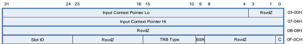
Figure 6-27: Evaluate Context Command TRB
