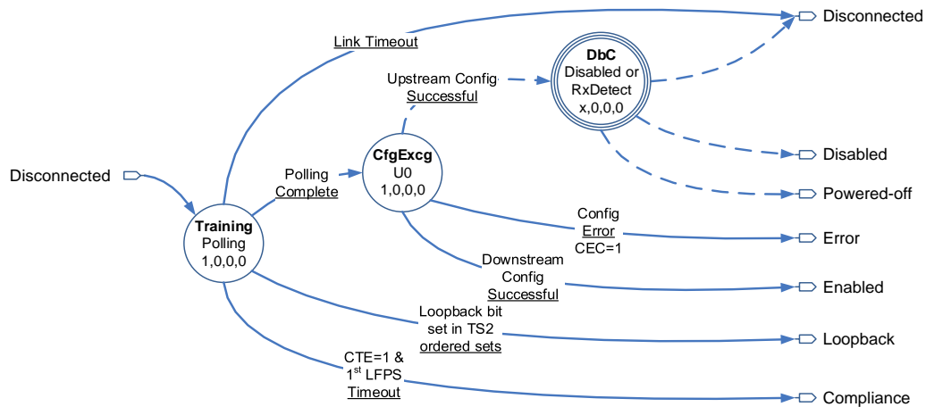
Figure 4-28: USB3 Root Hub Port Polling Substate Diagram
