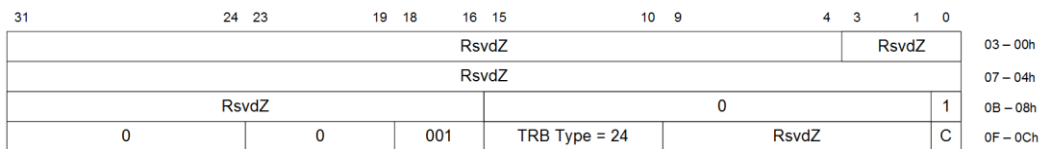
Figure 7-17: Get Extended Property - Get Supported Resource Subtype
