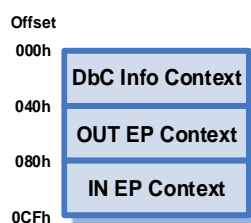
Figure 7-10: Debug Capability Context Data Structure
