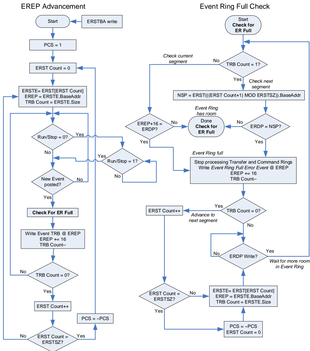
Figure 4-12 describes the algorithm the xHC employs for advancing its internal Event Ring Enqueue Pointer (EREP). The left side of the figure describes the EREP Advancement algorithm. The right side of the figure describes the algorithm for checking if the Event Ring is full.
