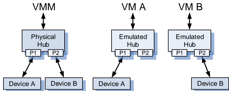
Figure 8-2: Emulated Hub Device Attachment Example
