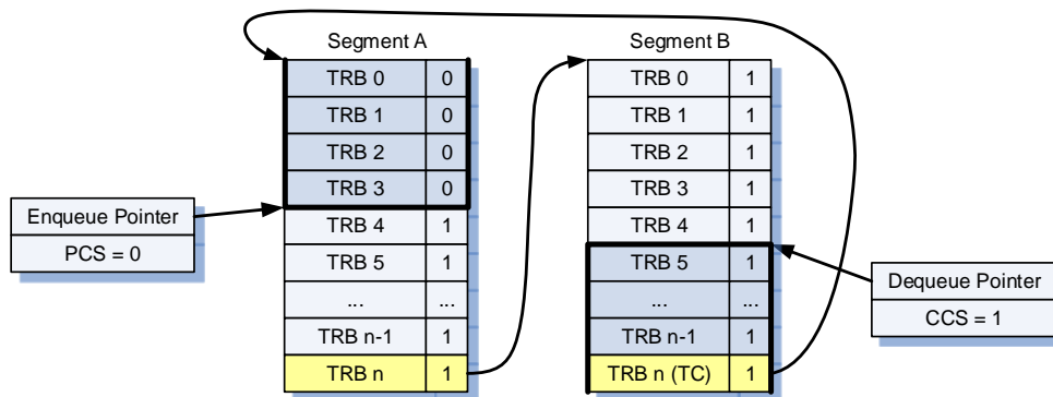
Figure 4-9: Initial State of Transfer Ring
