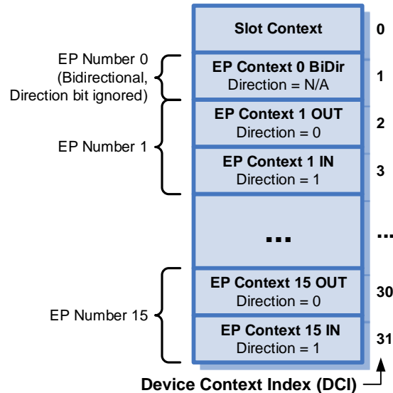
Figure 4-4: Endpoint Context Addressing
