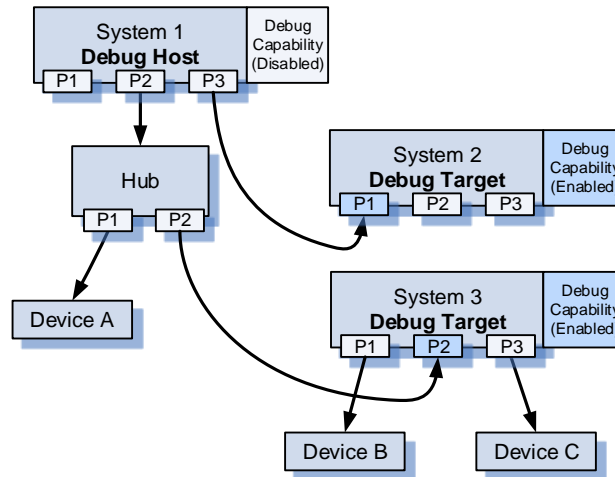
Figure 7-4: Example Debugging Topology
