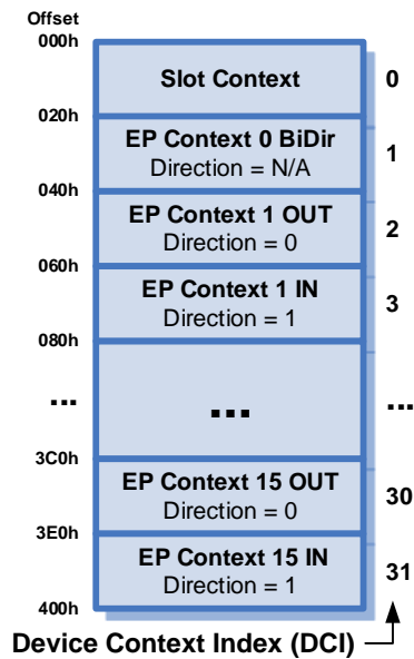
Figure 6-1: Device Context Data Structure
