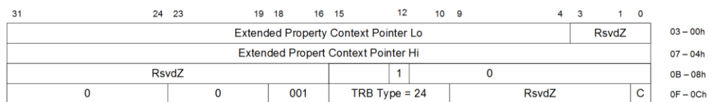
Figure 7-25: Get Time Stamp Command SubType
