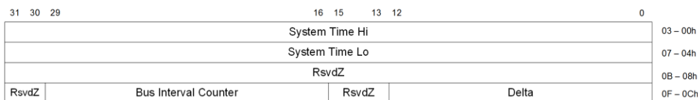
Figure 7-27: Extended Property Context with Get Time Stamp Results
