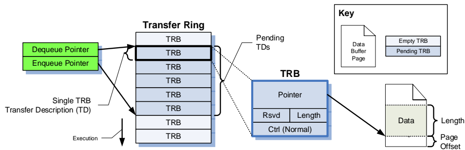
Figure 3-6: Simple Transfer Example
