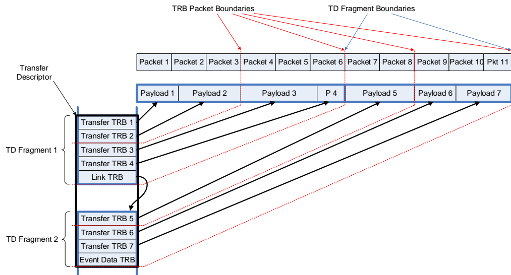
Figure 4-16: TRB Packet Boundary Example
