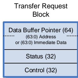
Figure 3-5: Transfer Request Block
