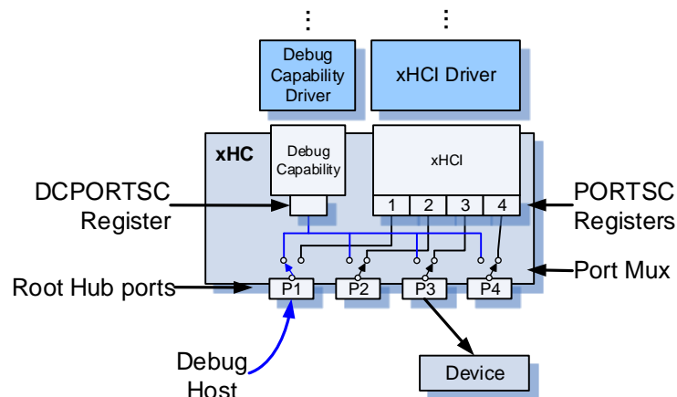
Figure 7-7: Debug Port Multiplexing
