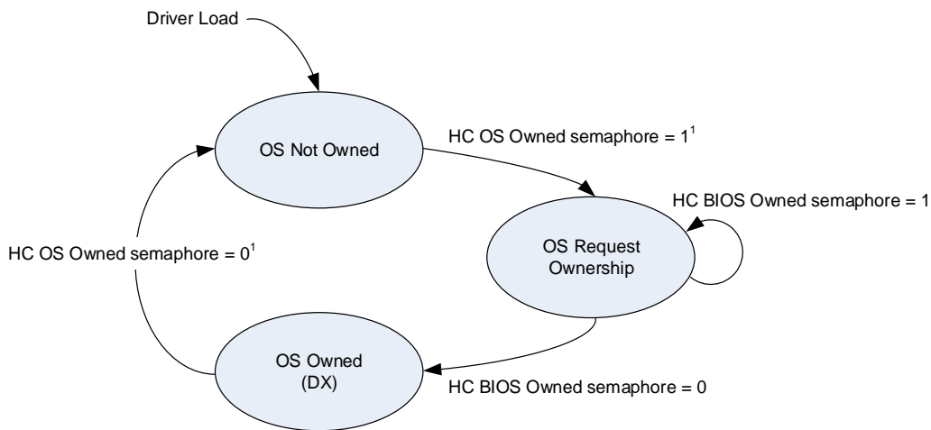
Figure 4-37: OS Ownership State Machine
