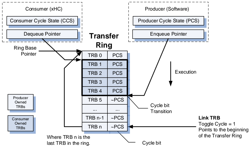
Figure 4-6: Index Management
