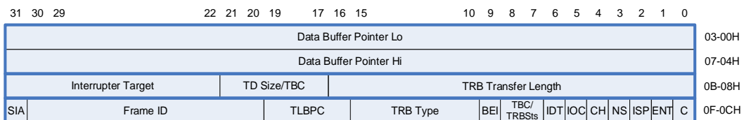
Figure 6-12: Isoch TRB
