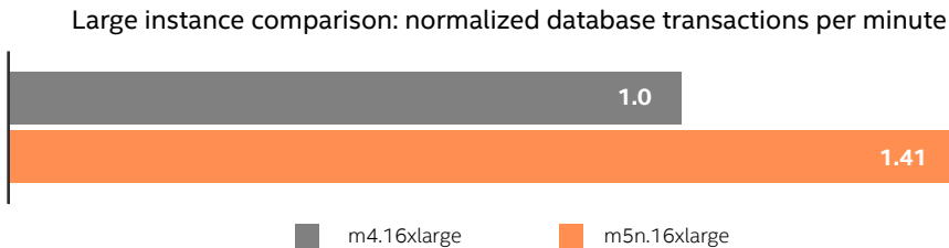
Figure 3. HammerDB test results comparing performance of the M5n instance type to M4 instance type with 64 vCPUs and 100GB database size.
