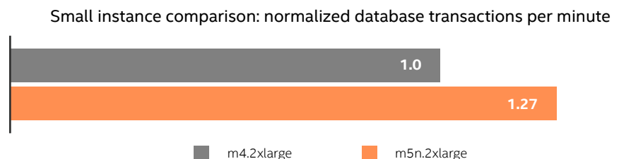
Figure 1. HammerDB test results comparing performance of the M5n instance type to M4 instance type with 8 vCPUs and 20GB database size.
