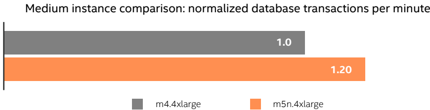
Figure 2. HammerDB test results comparing performance of the M5n instance type to M4 instance type with 16 vCPUs and 50GB database size.
