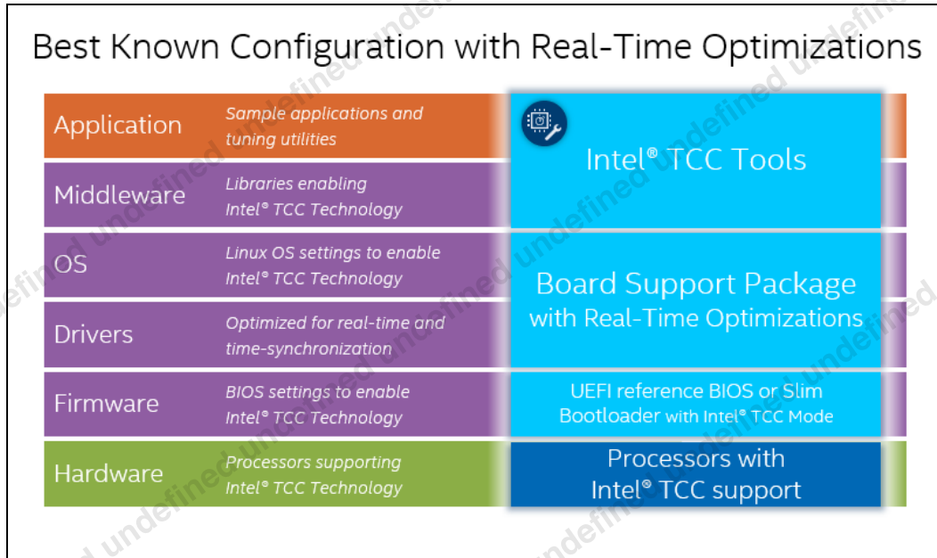
Figure 1. Intel® TCC Reference Software Stack
