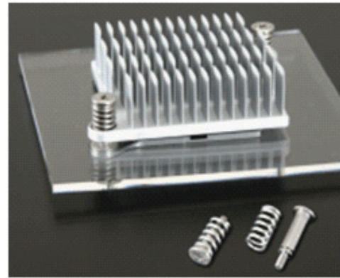
Shoulder screws
