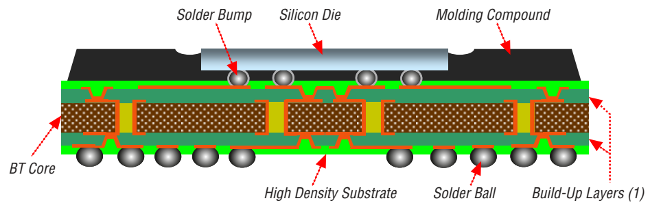
Figure 2. Cross-Sectional View of an TCFCBGA Package
