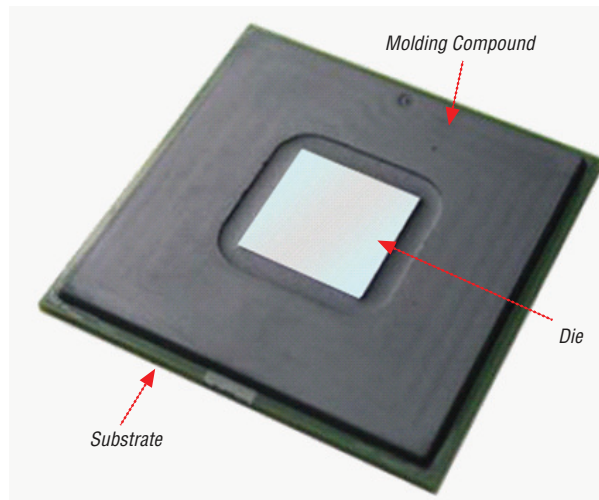
Figure 1. Package Construction of a TCFCBGA
