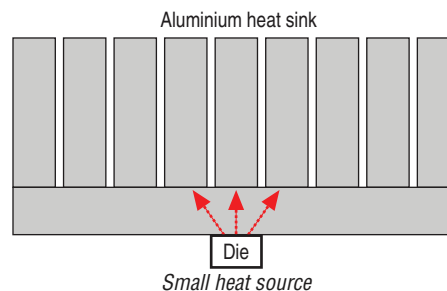
Figure 12. Small Heat Source with Aluminium Heat Sink
