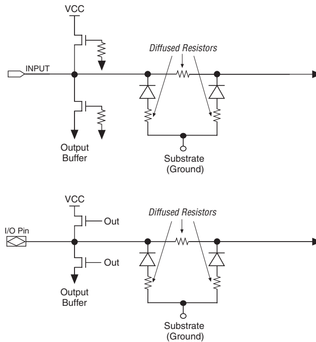
Figure 2. Altera Device Input Protection Structures
