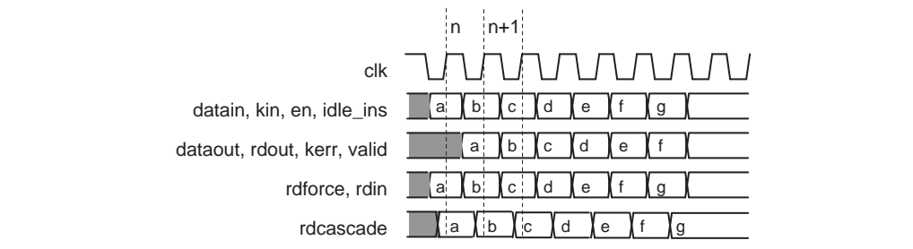
Figure 3-6. Encoder Timing Diagram—One Cycle Latency
