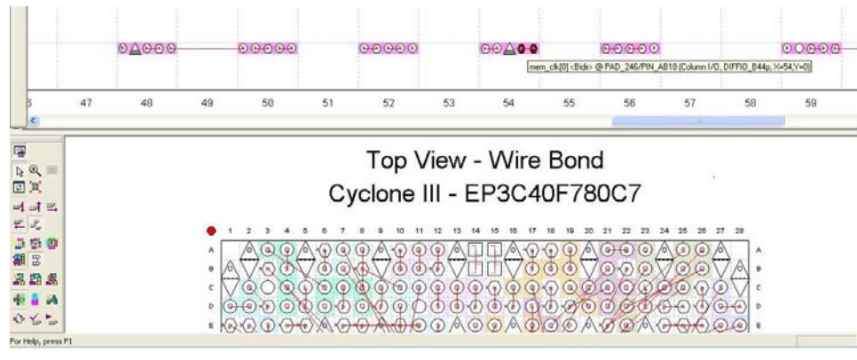
Figure 2-5. Correct Placement of mem_clk[0] and mem_clk_n[0] in Cyclone III and Cyclone IV Devices.
