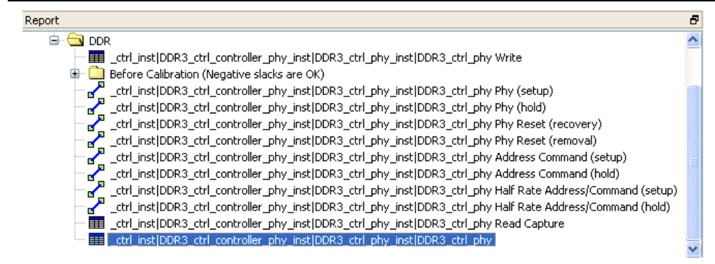
Figure 1-8. DDR Timing Report in the TimeQuest Window Report Pane
