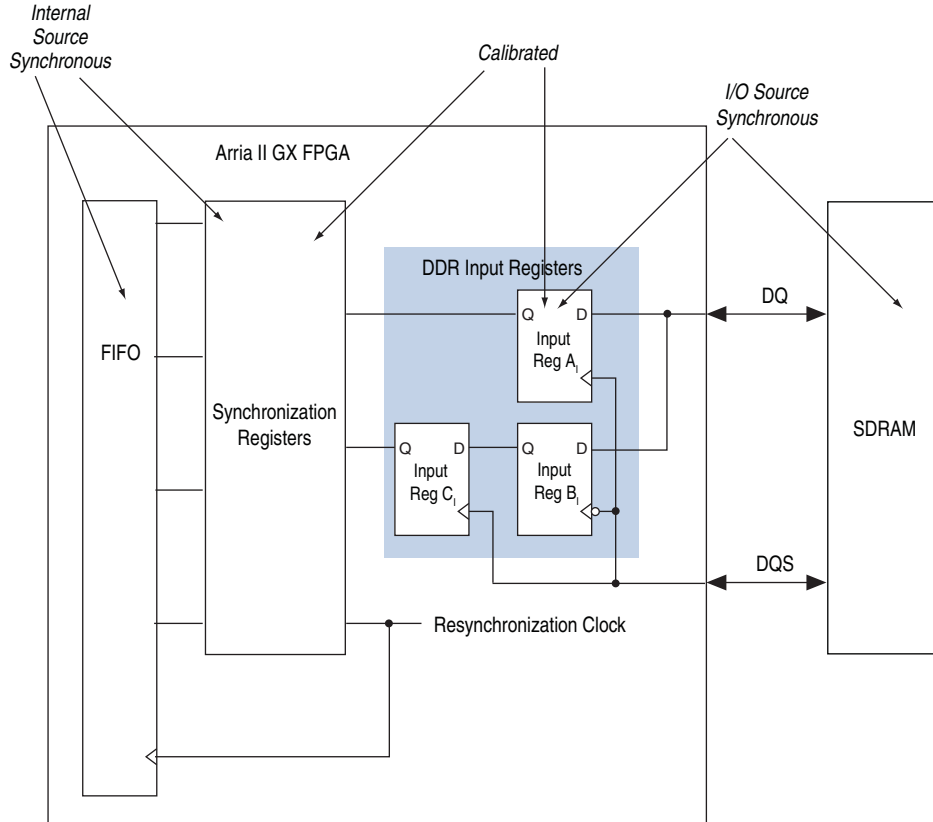
Figure 1-1. Arria II GX Devices Input Data Path Registers and Circuit Types in SDRAM Interface
