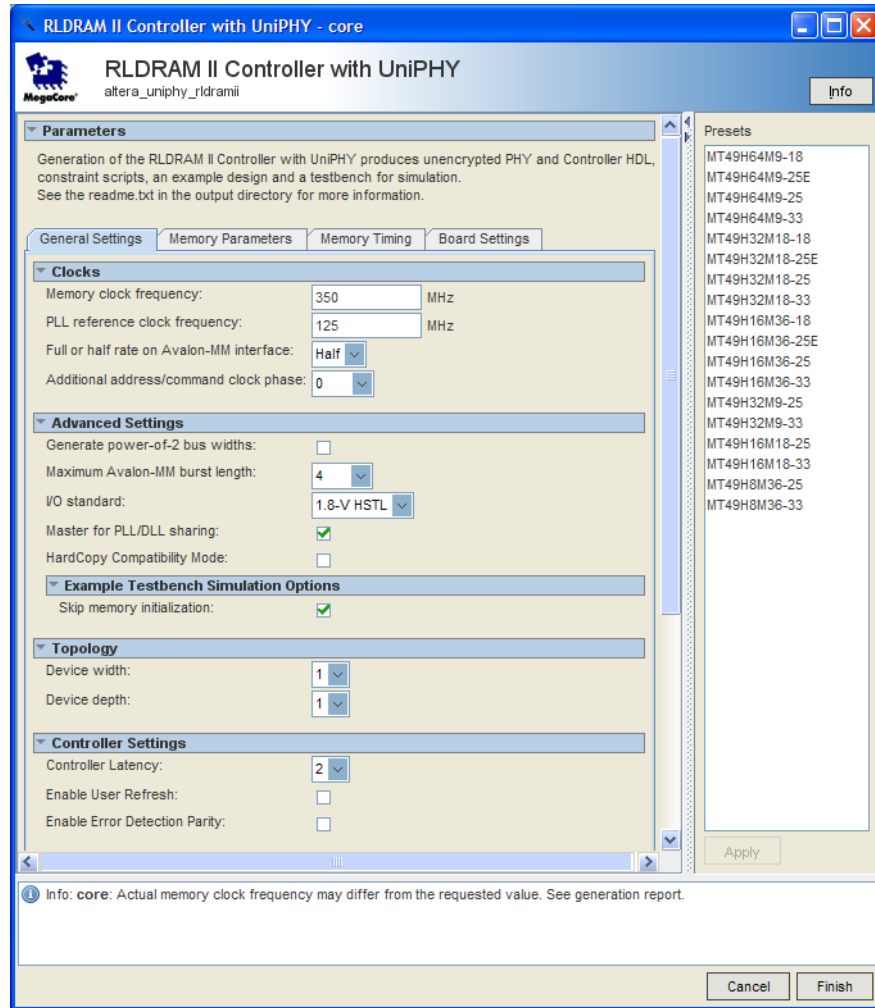
Figure 2-2. Presets
