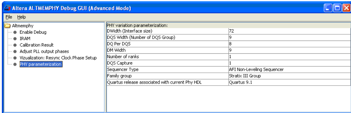
Figure 4-9. PHY Parameterization
