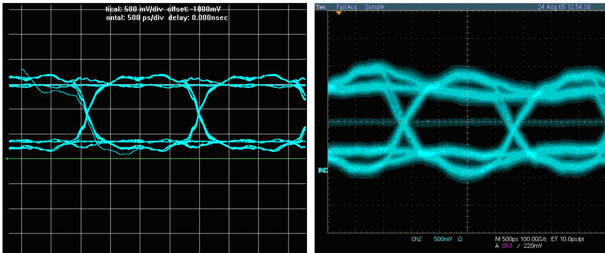
Figure 1-28. Simulation and Board Measurement, FPGA Writing to Memory
