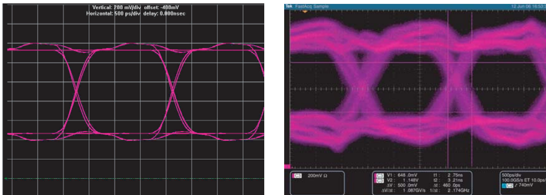
Figure 3-16. HyperLynx Simulation and Board Measurement of the Signal at the FPGA When Reading From Slot 1 With Both Slots Populated (Note 1)
