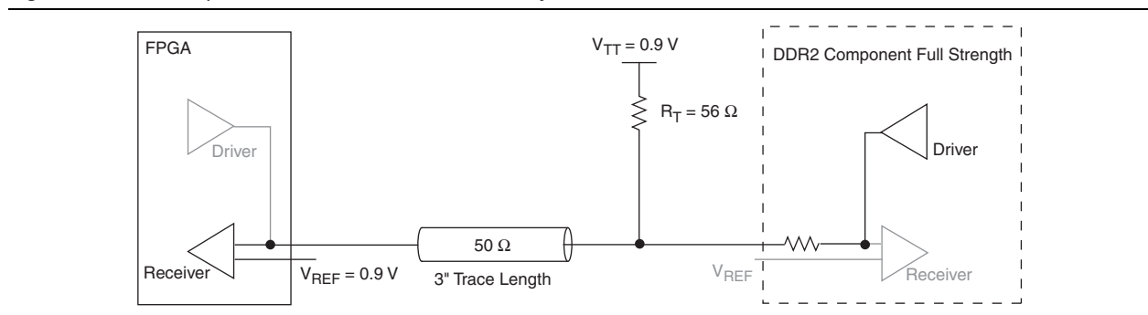
Figure 3-20. Read Operation from DDR2 SDRAM Memory with Class I Termination
