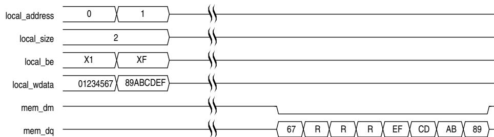
Figure 6-4. Partial Write for HPC—Full Rate
