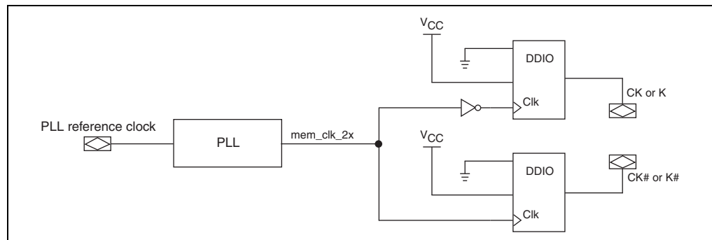
Figure 1-15. DDIO Configuration
