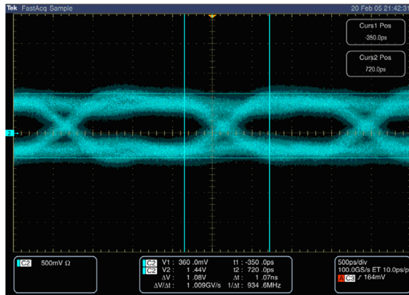
Figure 1-22. Board Measurement, FPGA Reading from Memory
