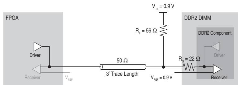
Figure 1-23. Class I Termination Scheme with Memory-Side Series Resistor
