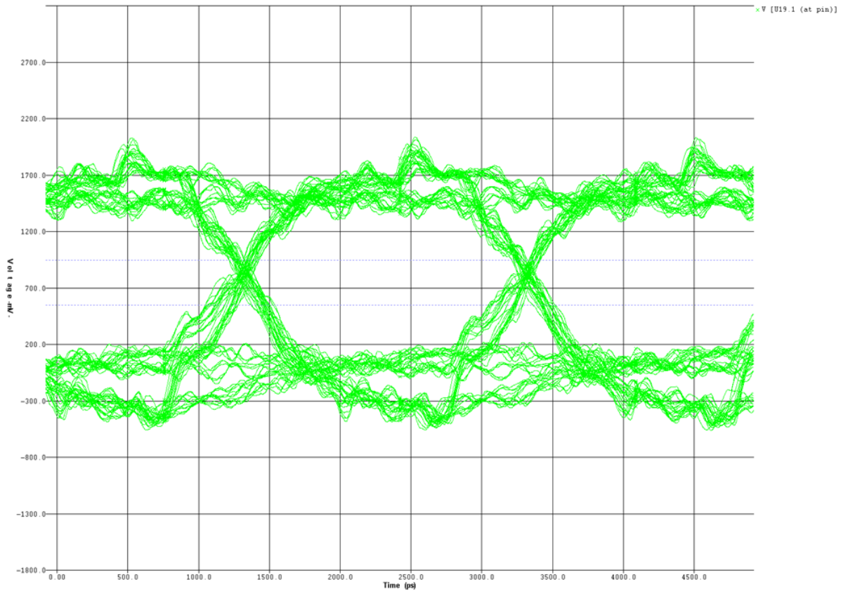
Figure 4-14. Read Data Simulation at 250 MHz with No Far-End Termination
