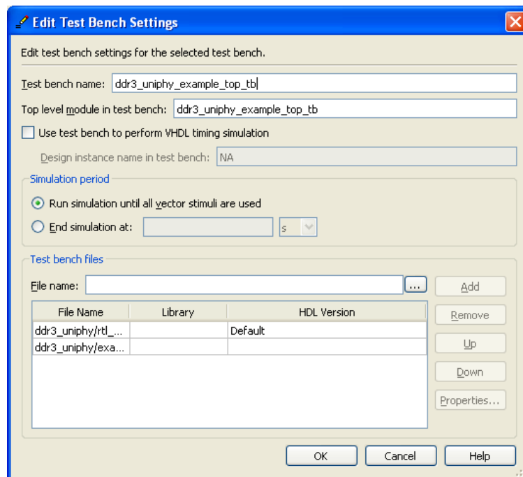
Figure 3–2. Testbench Settings
