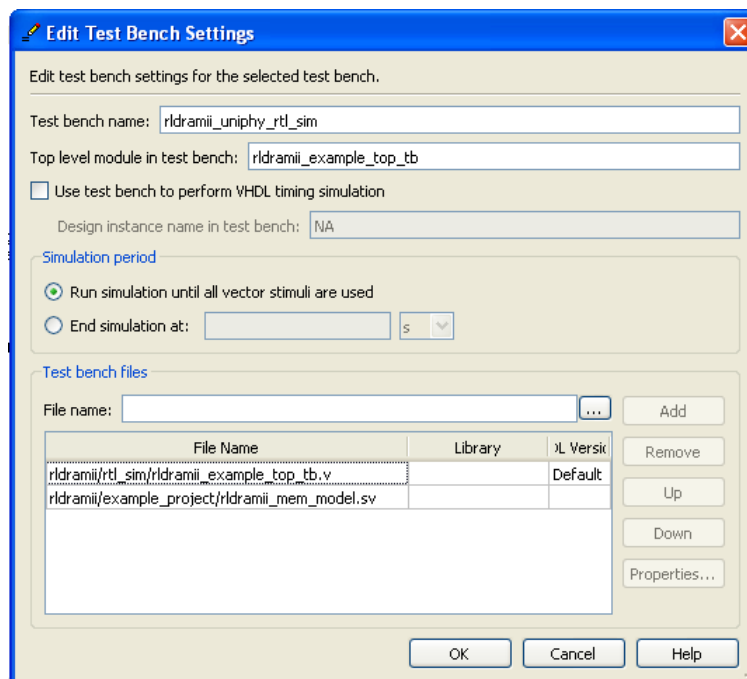
Figure 4-4. Testbench Settings
