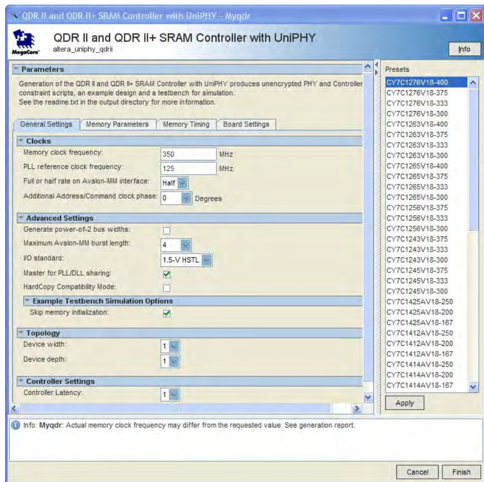
Figure 2-2. Presets
