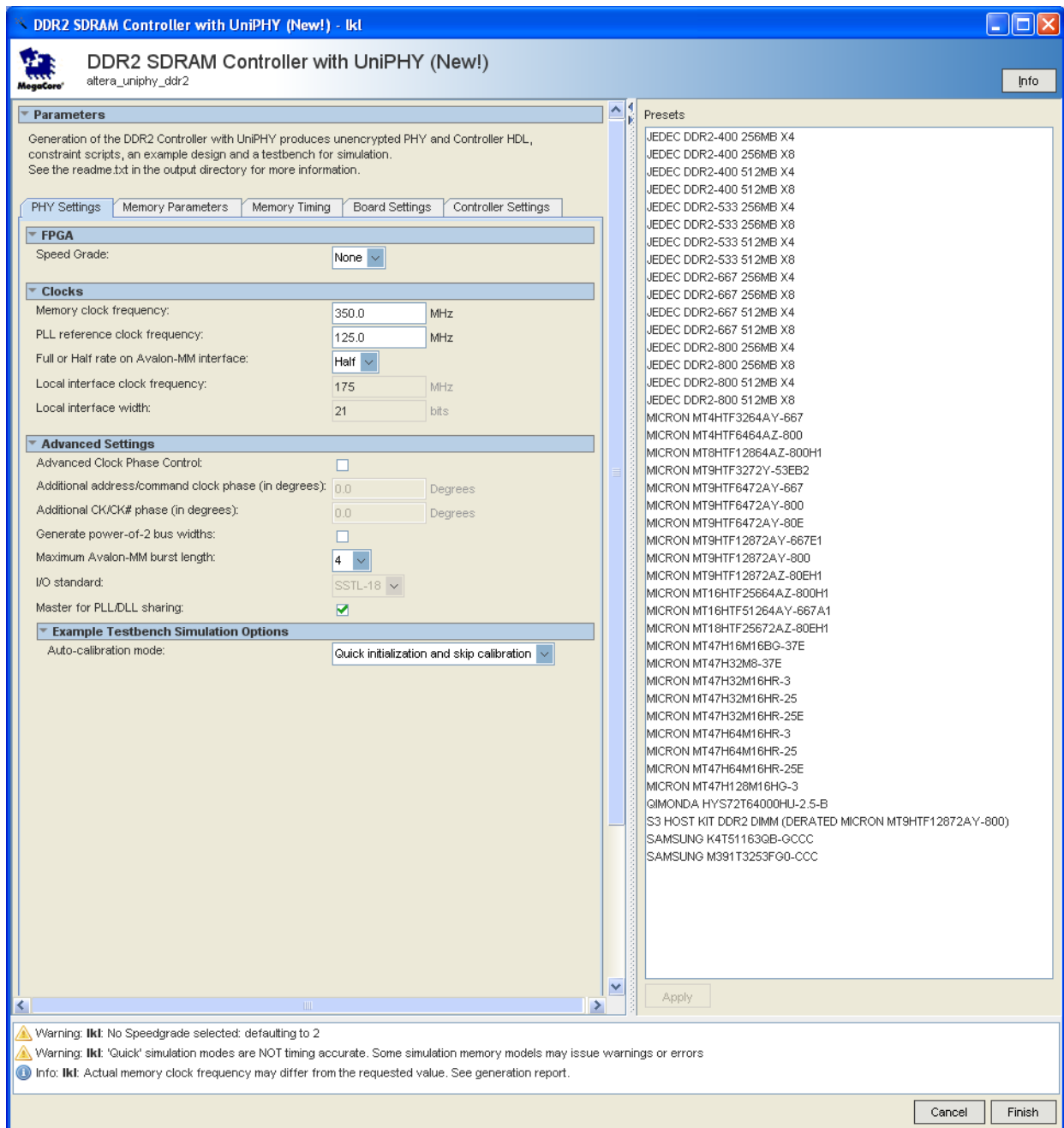
Figure 2-2. Presets
