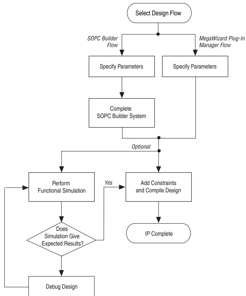
Figure 2-1. Design Flows
