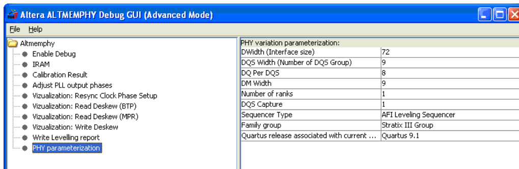
Figure 4-20. PHY Parameterization
