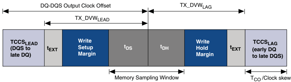
Figure 1-7. Timing Budget for Write Data Timing Path
