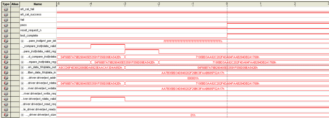
Figure 2-7. SignalTap II Example RLDRAM II Design Analysis
