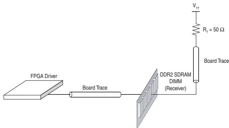
Figure 1-2. Fly-By Placement of a Parallel Resistor
