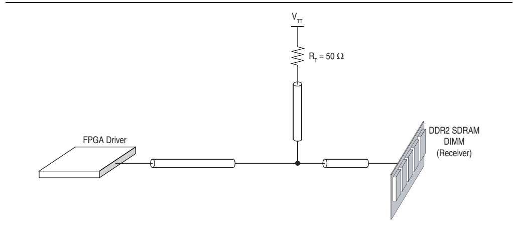
Figure 1-3. Non-Fly-By Placement of a Parallel Resistor
