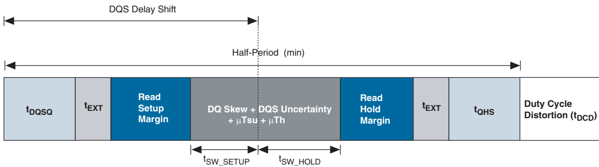
Figure 1-6. Timing Budget for Read Data Timing Path
