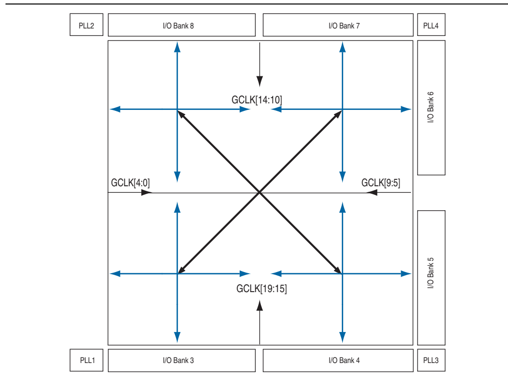
Figure 1-3. PLL and DLL Locations in Cyclone IV GX Devices
