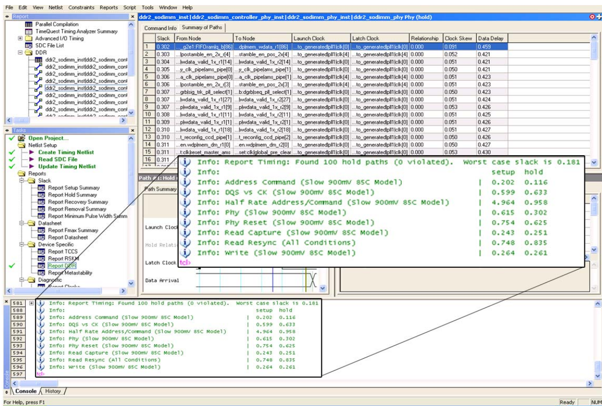
Figure 2-7. Timing Margin Report in the TimeQuest Timing Analyzer
