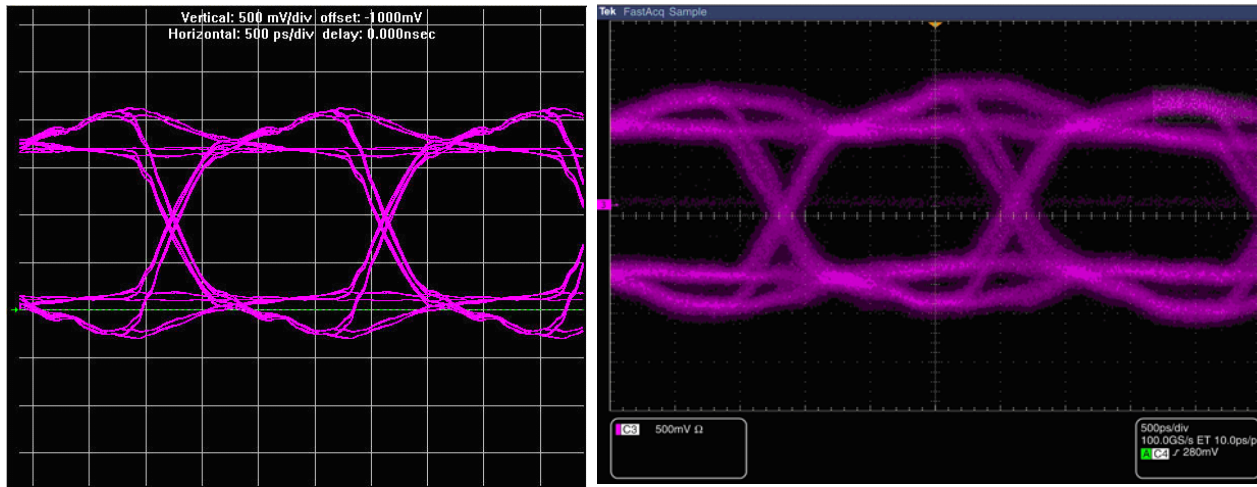
Figure 1-24. HyperLynx Simulation and Board Measurement, FPGA Writing to Memory
