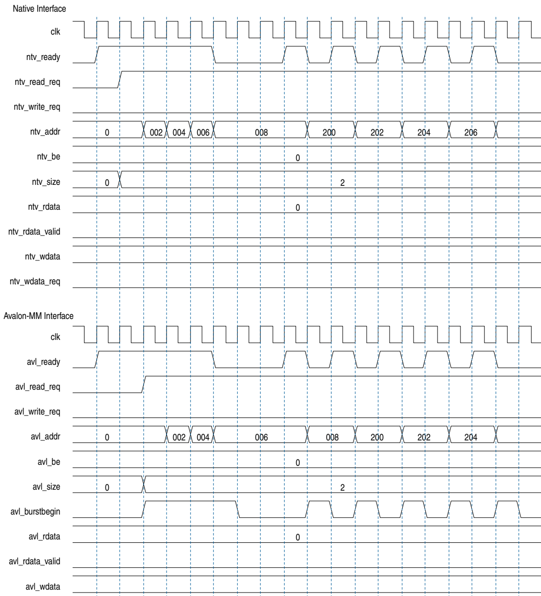
Figure 1-2. Read Commands
