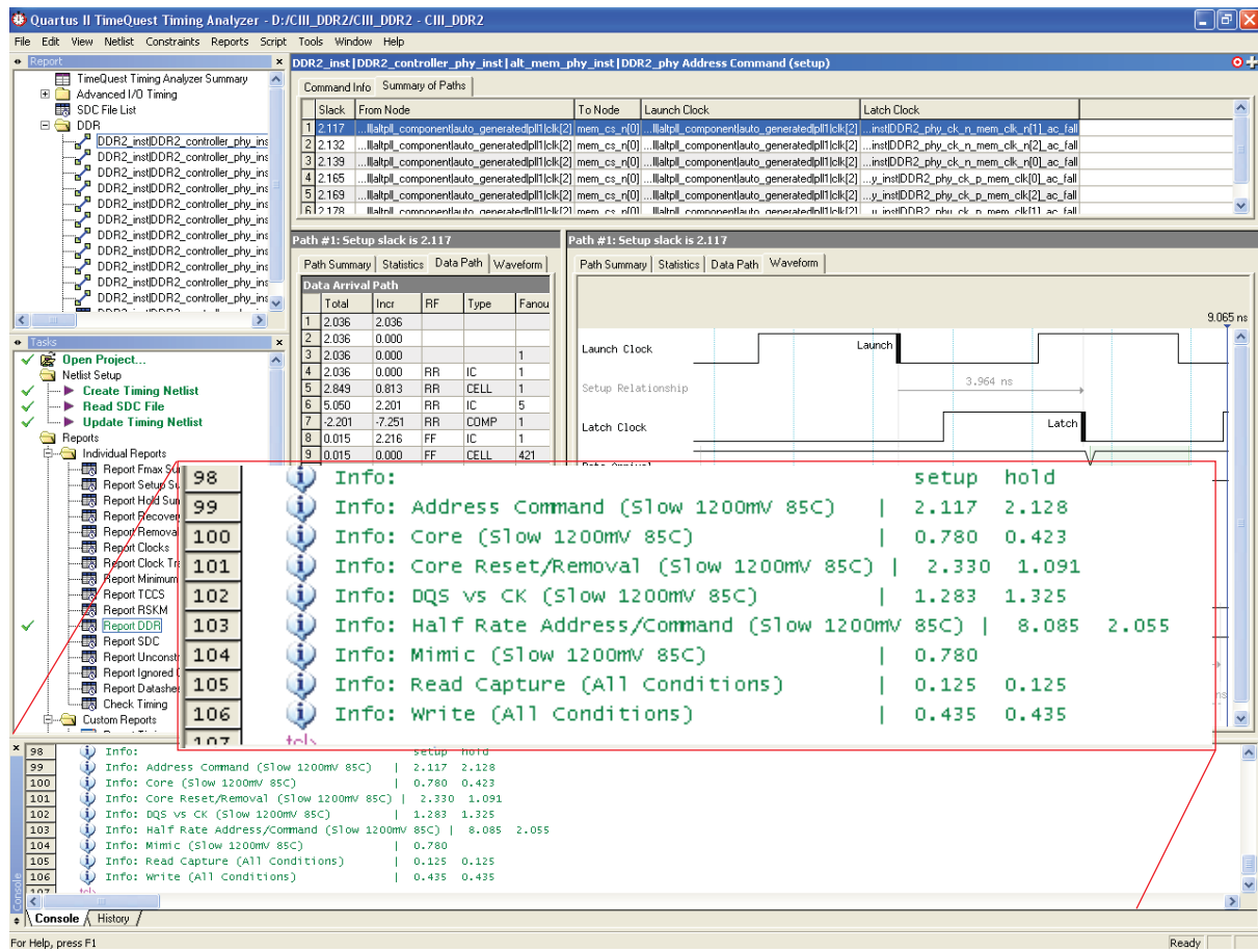
Figure 3-18. Timing Margin Reported After Adjusting clk2
