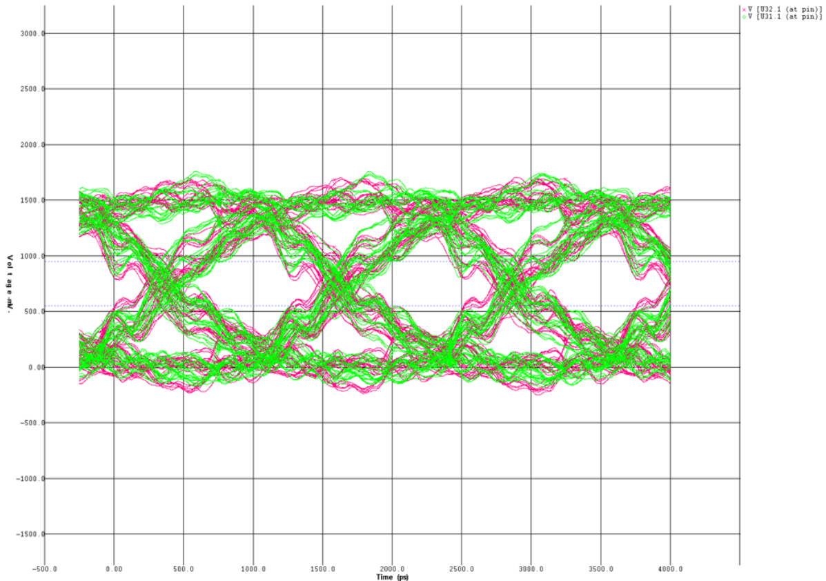
Figure 4-11. Address Simulation Using Stratix IV Class I HSTL-15 50 \Omega Calibration Driver and No Termination
