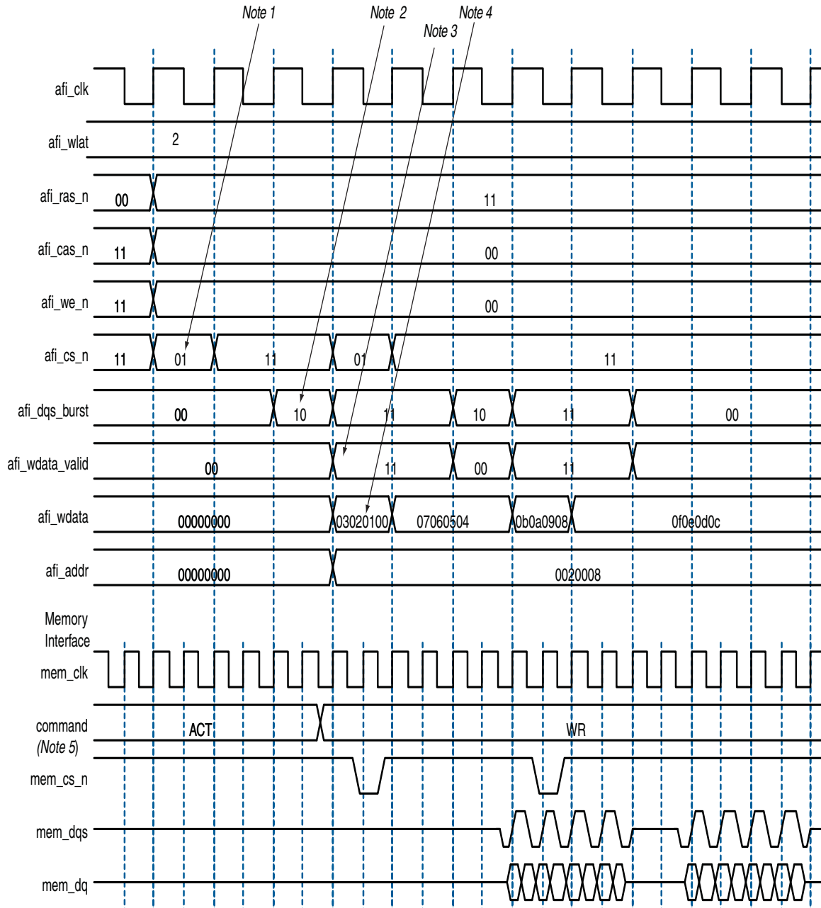
Figure 5-10. Word-Aligned Writes
