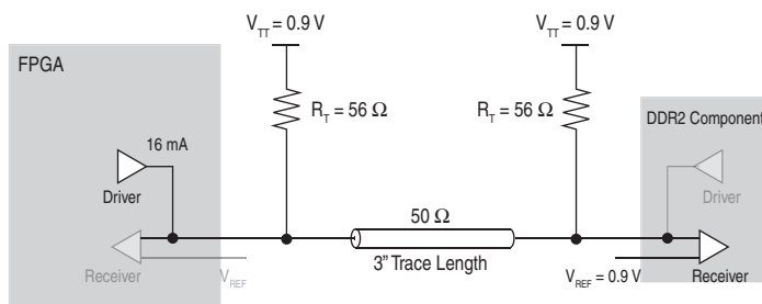
Figure 1-36. Class II Termination Scheme without Memory-Side Series Resistor
