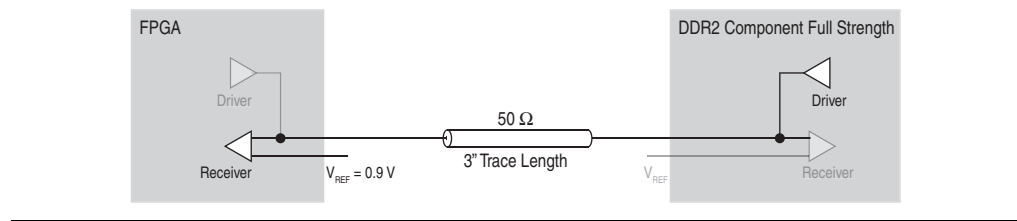
Figure 1-33. No-Parallel Termination Scheme, FPGA Reading from Memory
