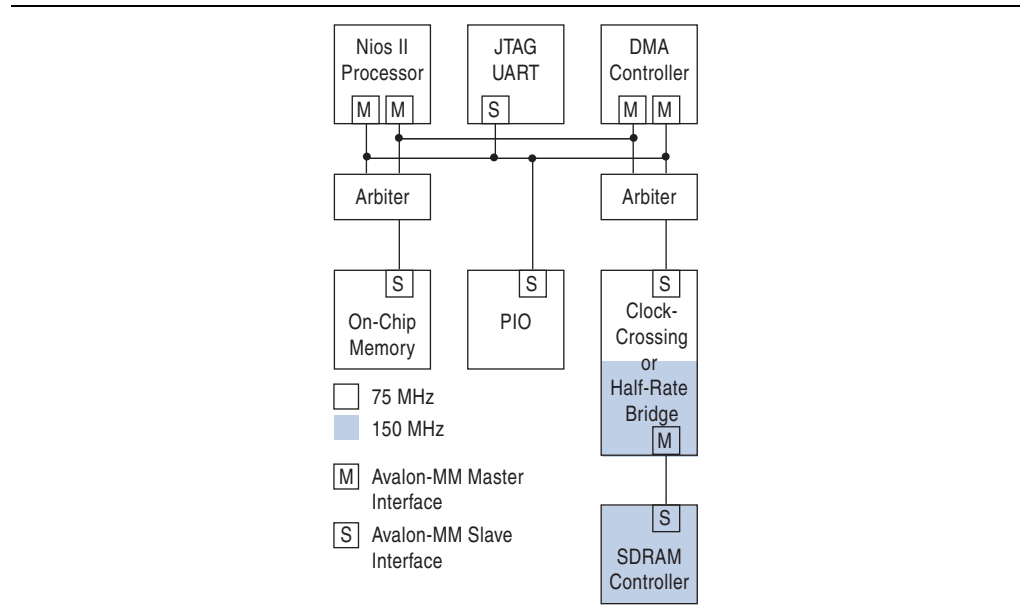
Figure 6-2. Clock Crossing Bridge
