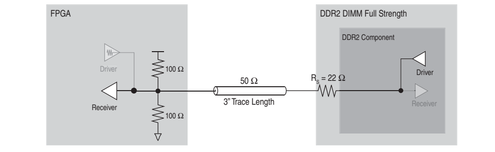
Figure 1-11. Dynamic Parallel OCT Scheme with Memory-Side Series Resistor
