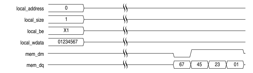
Figure 6-5. Partial Burst for HPC
