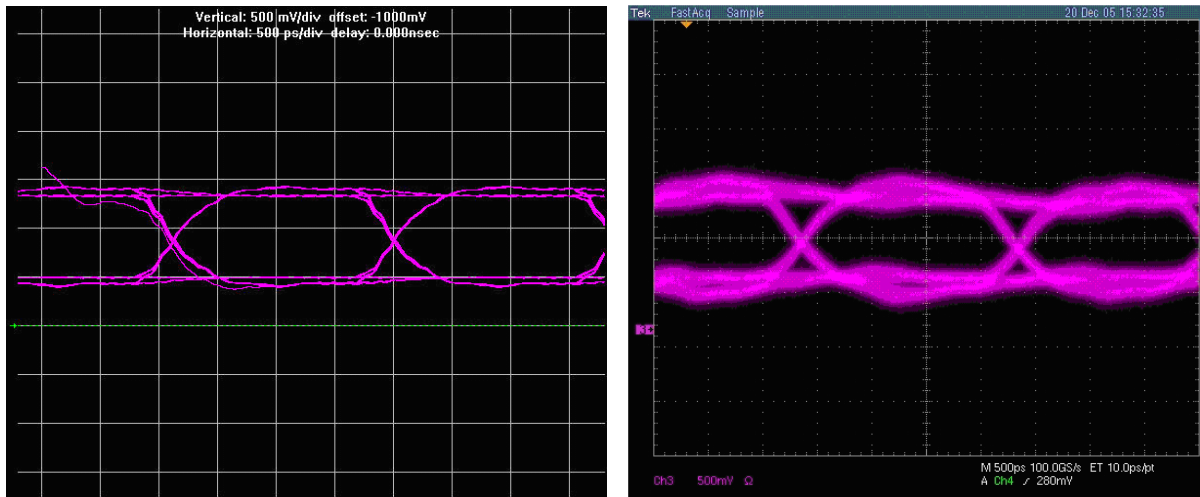
Figure 1-16. HyperLynx Simulation and Measurement, FPGA Writing to Memory
