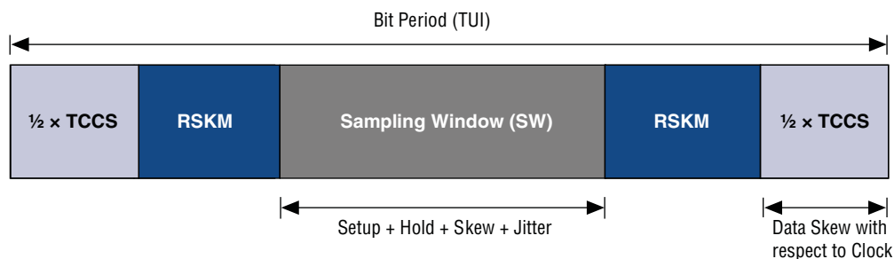
Figure 1-4. Sample Timing Budget Diagram
