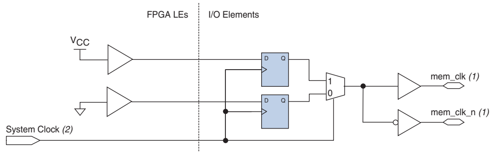
Figure 1-14. DIDO Configuration with Signal Splitter
