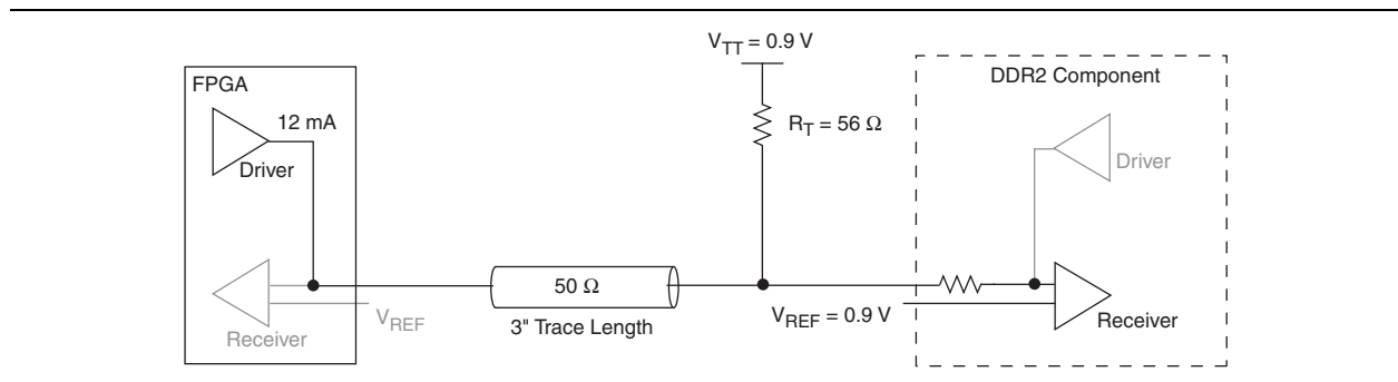
Figure 3-19. Write Operation to DDR2 SDRAM Memory with Class I Termination
