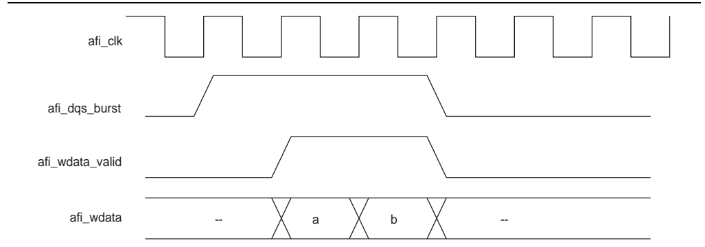
Figure 5-7. Full-Rate Write
