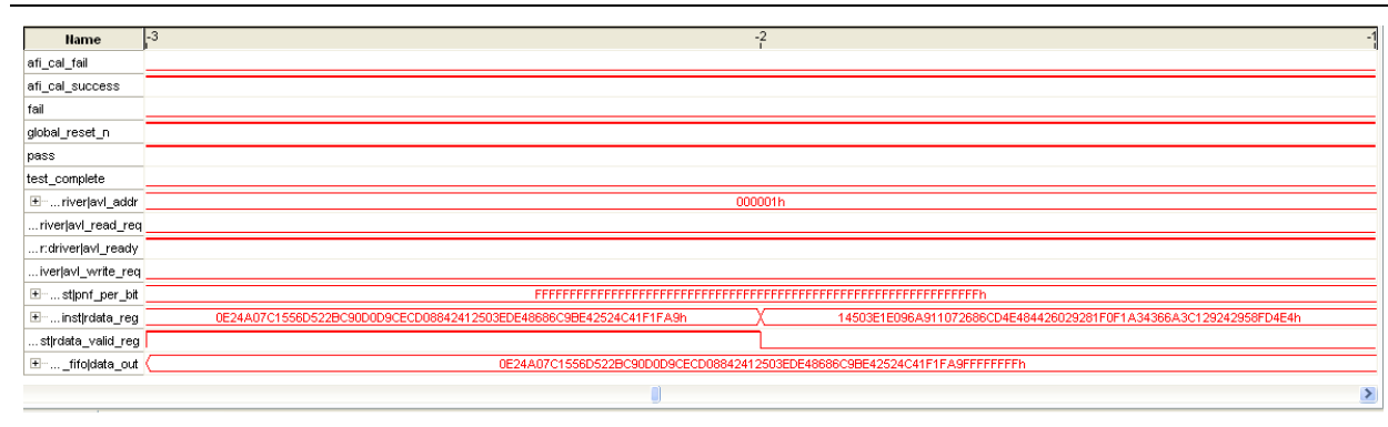
Figure 3-6. SignalTap II Example DDR3 SDRAM with UniPHY Design Analysis
