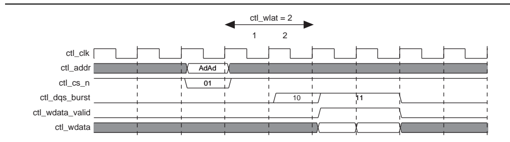
Figure 5-25. Timing for ctl_dqs_burst , ctl_wdata_valid , Address, and Command—Half-Rate Design
