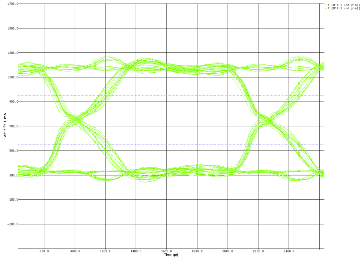
Figure 4-4. Write Data Simulation at 400 MHz with Fly-By 50 \Omega Parallel Termination to V_{TT}
