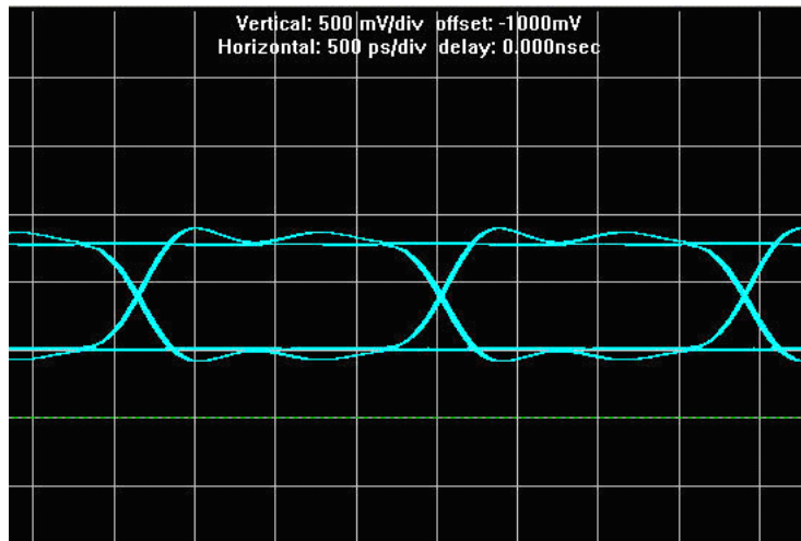
Figure 1-21. HyperLynx Simulation, FPGA Reading from Memory
