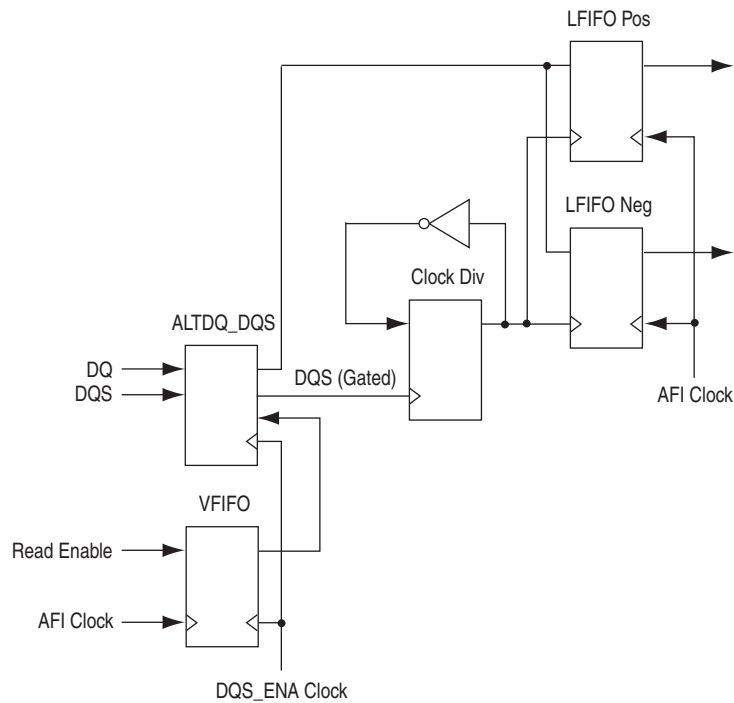
Figure 6-4. Read Datapath
