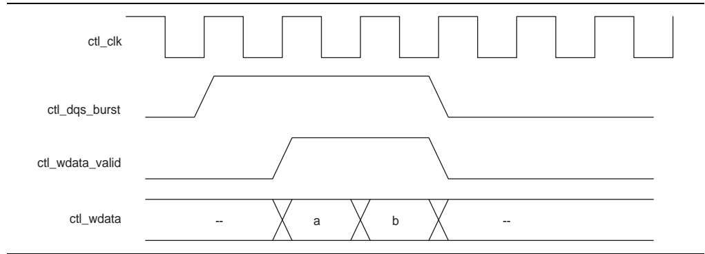
Figure 5-16. Full-Rate Write
