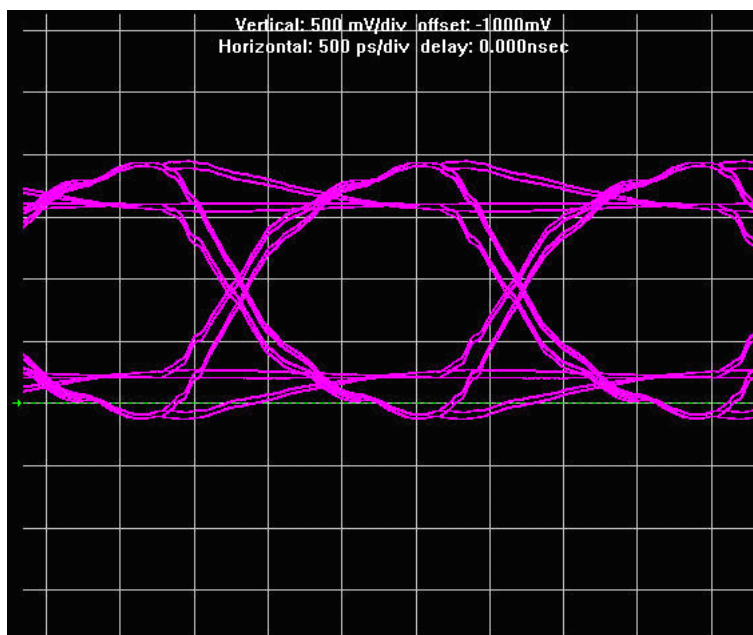
Figure 1-18. HyperLynx Simulation, FPGA Writing to Memory
