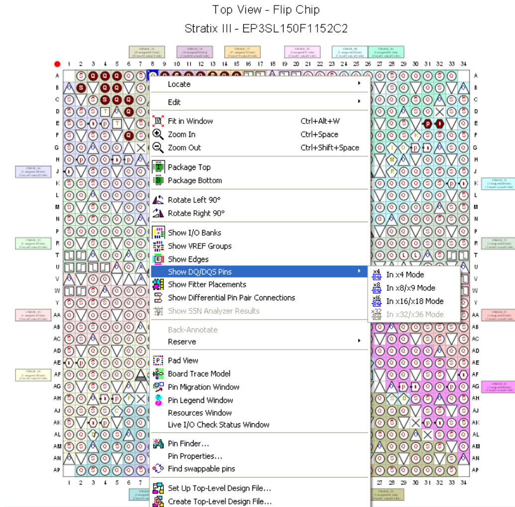
Figure 1-1. Quartus II Pin Planner, Show DQ/DQS Pins, In \times 16/\times 18 Mode
