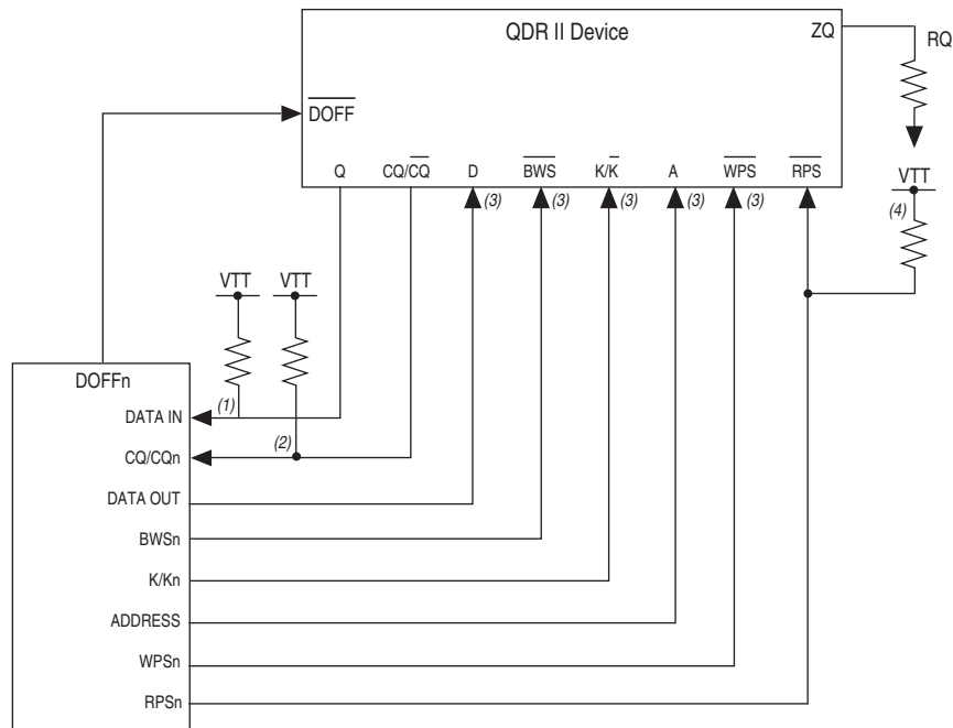
Figure 4-1. Configuration With A Single QDR II SRAM Component
