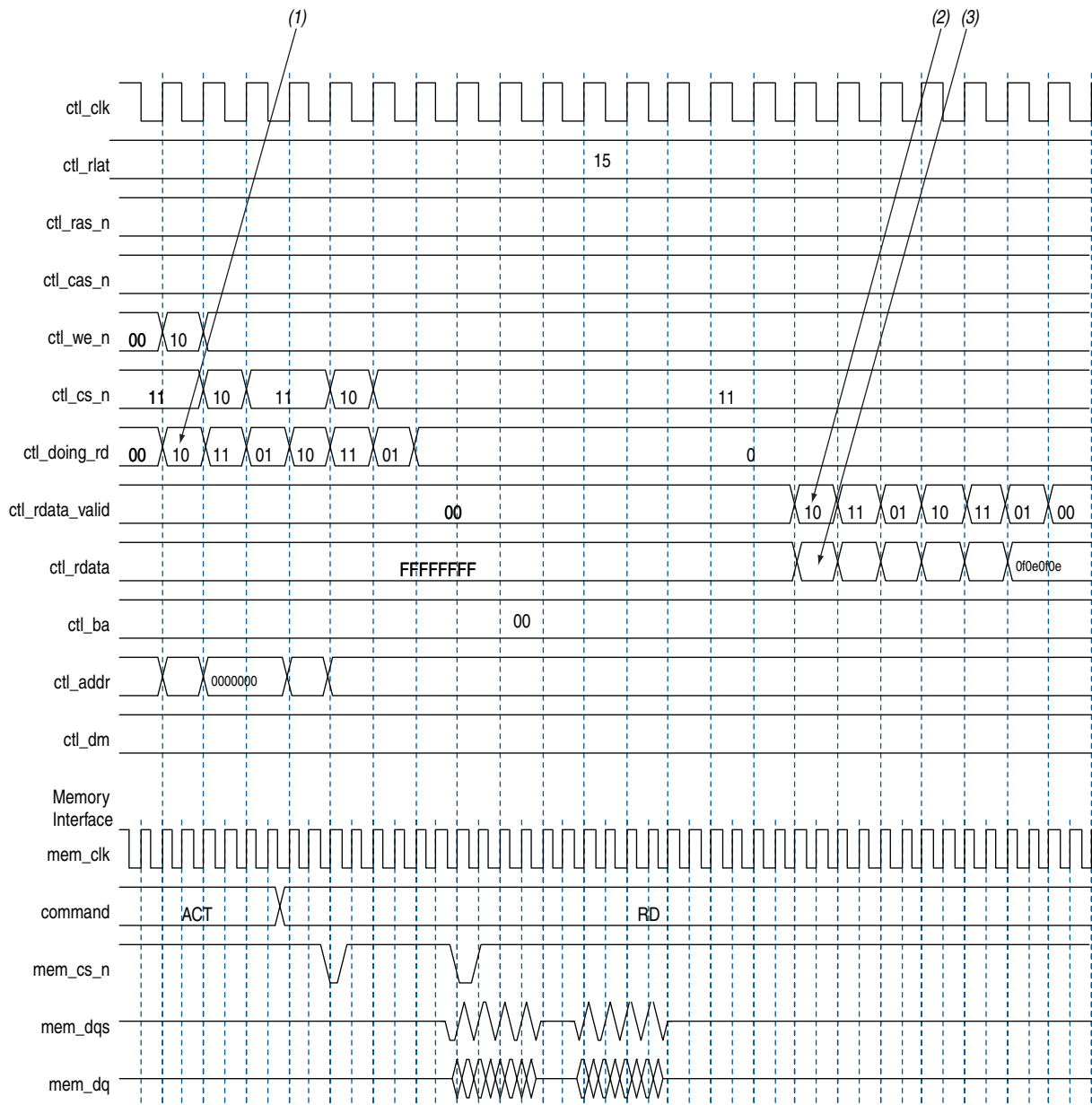
Figure 5-20. Word-Unaligned Reads
