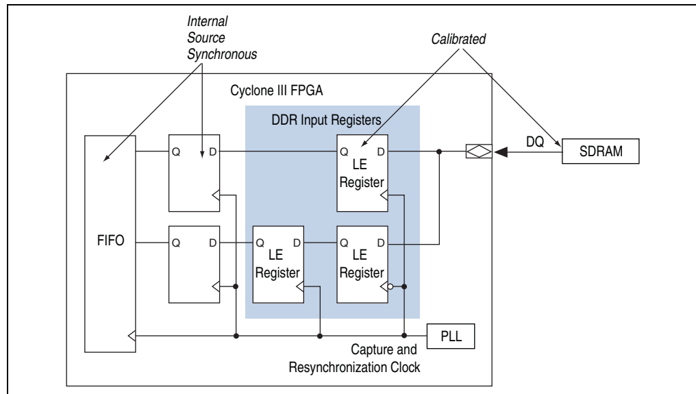
Figure 1-3. Cyclone III Input Data Path Registers and Circuit Types in SDRAM Interface
