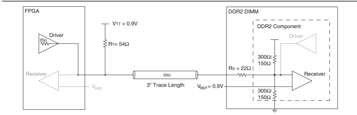
Figure 3-8. Double Parallel Termination Scheme (Class II) Using ODT on DDR2 SDRAM DIMM with Memory-side Series Resistor
