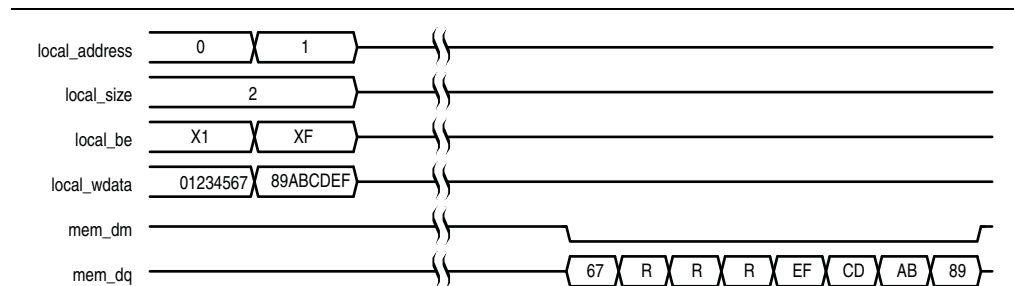
Figure 5-3. Partial Write for the Controller—Full Rate
