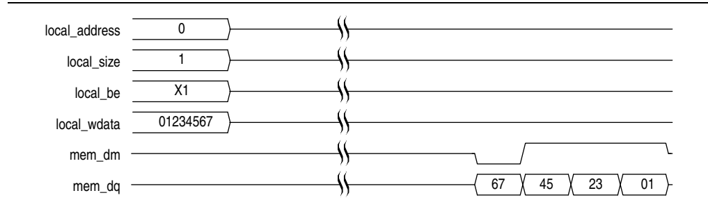
Figure 7-4. Partial Burst for HPC II
