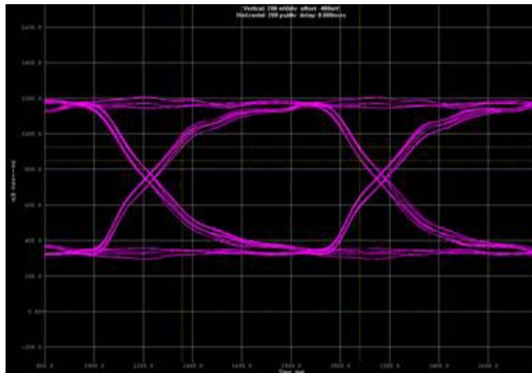
Figure 2-7. Simulated Write-Eye Diagram of a DDR3 SDRAM DIMM Using a 60-Ω ODT Setting
