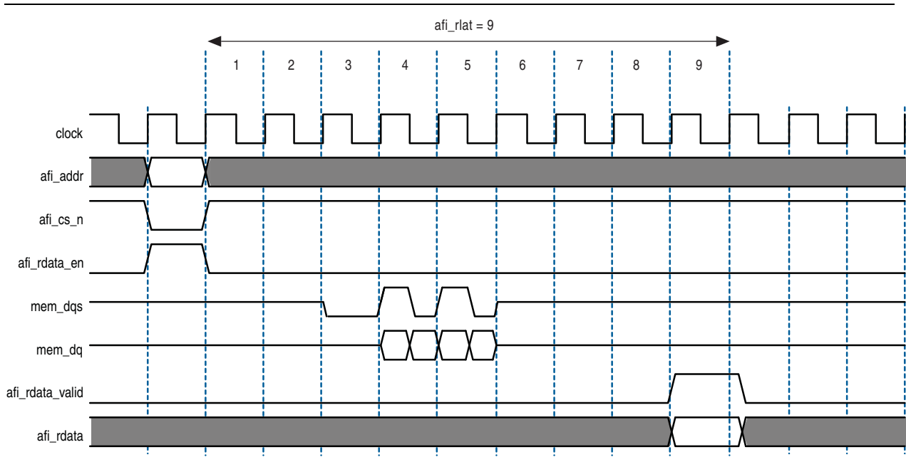
Figure 5-8. Full-Rate Reads
