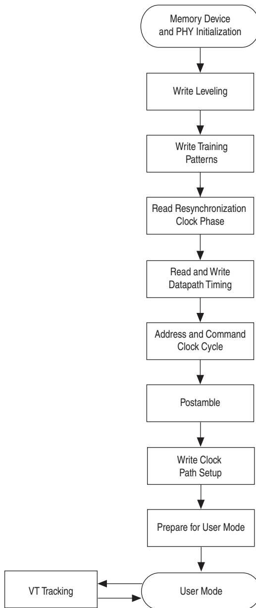
Figure 5-5. Calibration Flow—DDR3 SDRAM (with leveling)
