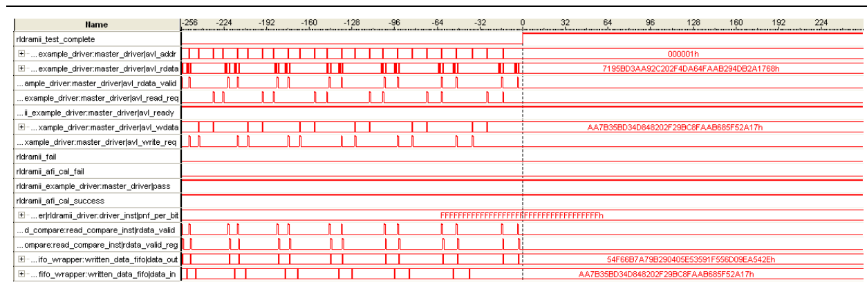
Figure 4-8. SignalTap II Example RLDRAM II Design Analysis
