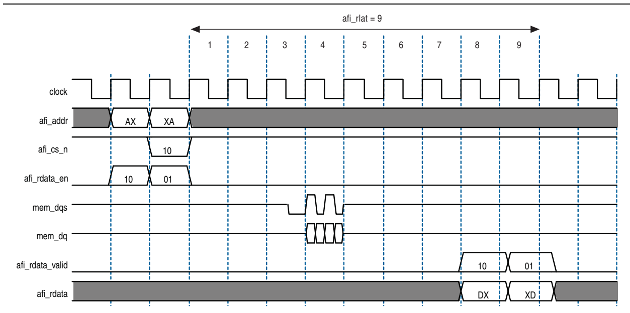
Figure 6-10. Half-Rate Reads
