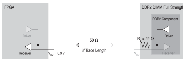
Figure 1-31. No-Parallel Termination Scheme, FPGA Reading from Memory
