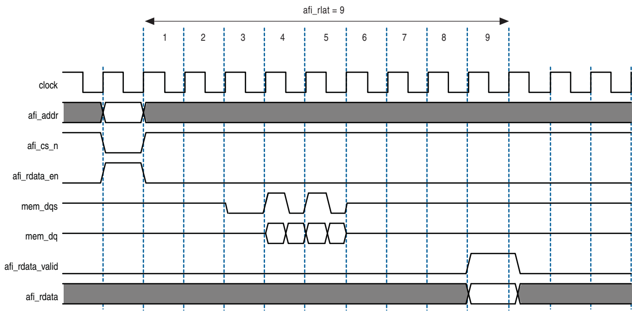
Figure 5-8. Full-Rate Reads
