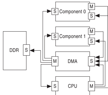
Figure 6-5. A Single Master Accessing Memory with DMA Controller
