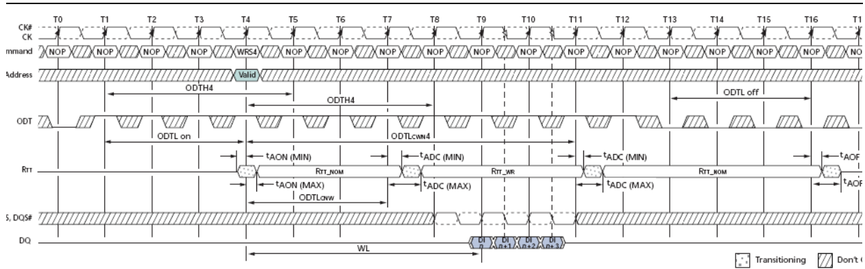
Figure 2-3. Dynamic ODT: Behavior with ODT Asserted Before and After the Write (Note 1)
