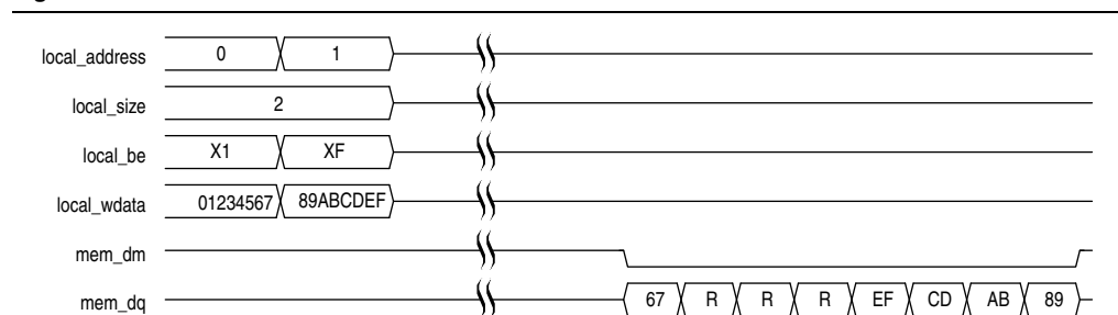
Figure 7-3. Partial Write for HPC II
