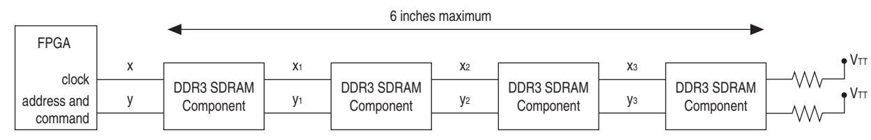
Figure 2-23. DDR3 SDRAM Component Routing Guidelines
