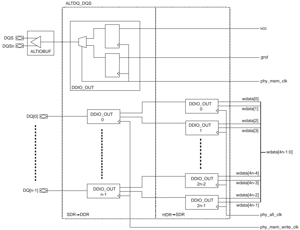
Figure 5-3. Write Datapath
