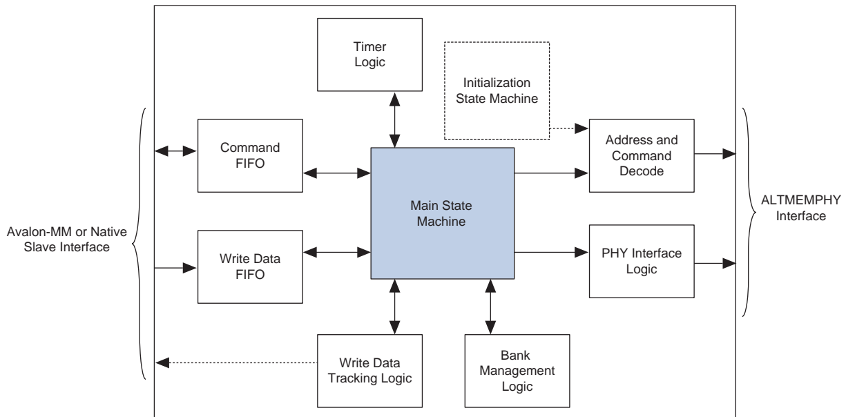
Figure 6-2. DDR3 SDRAM HPC Architecture Block Diagram
