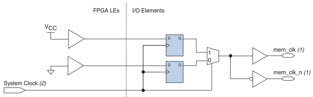
Figure 1-16. DIDO Configuration with Signal Splitter
