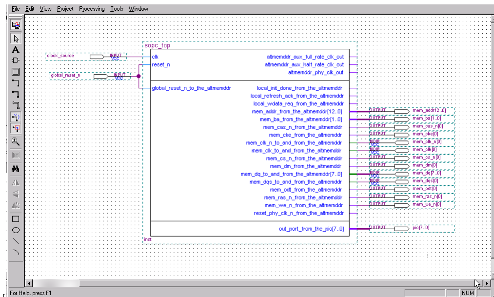
Figure 6-14. Quartus II Top-Level Project
