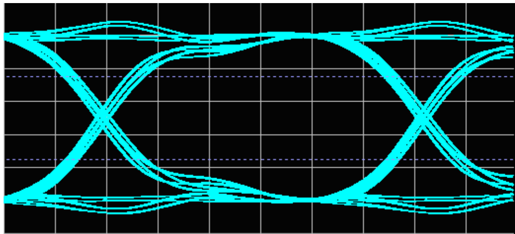
Figure 2. HyperLynx Simulation FPGA Writing to Memory
