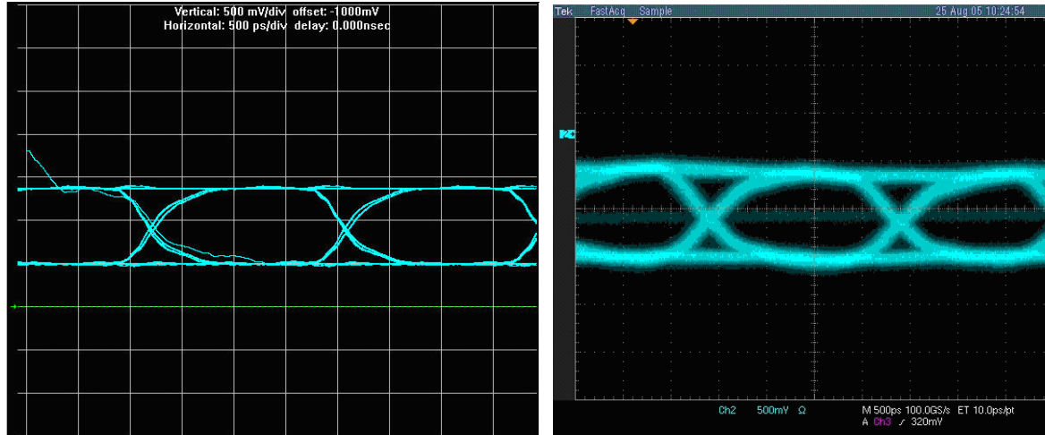
Figure 1-14. HyperLynx Simulation and Measurement, FPGA Writing to Memory
