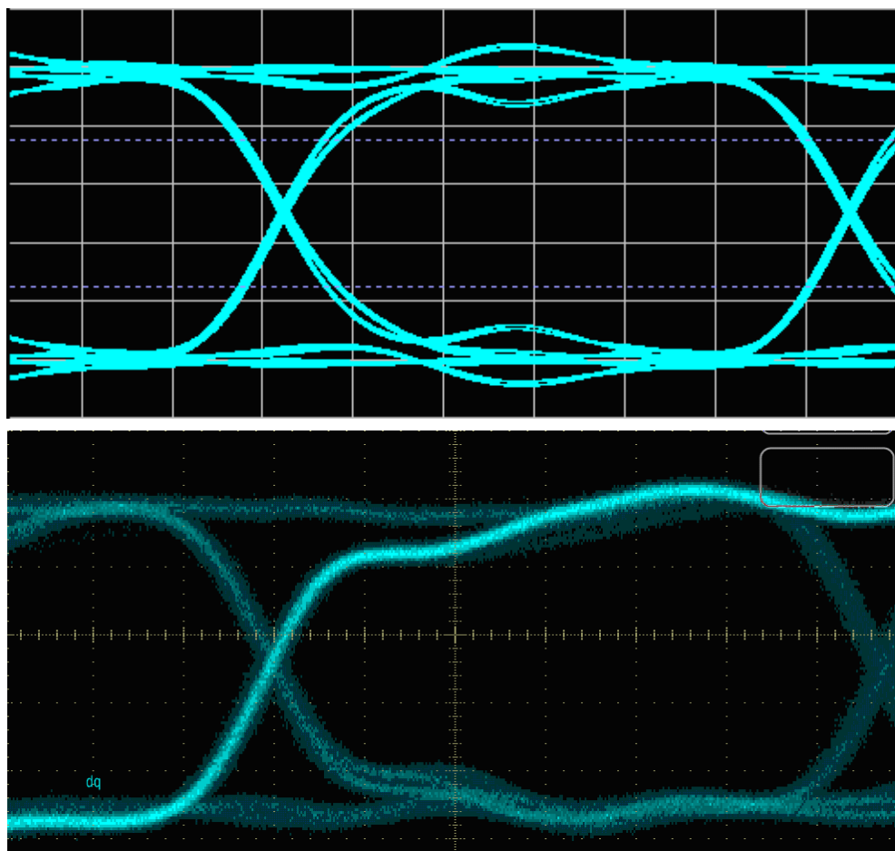
Figure 1-12. Hyperlynx Simulation and Board Measurement, FPGA Reading from Memory
