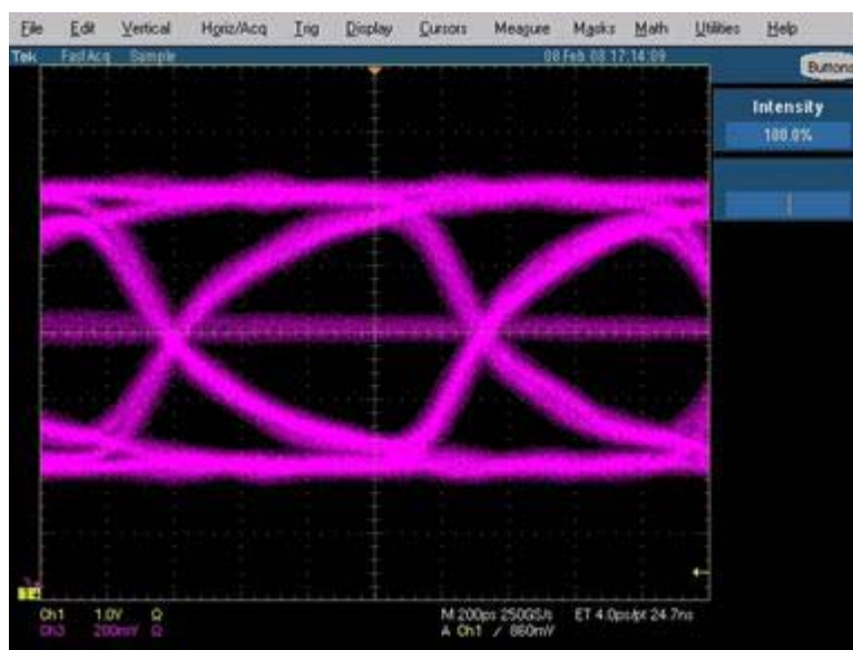
Figure 2-8. Measured Write-Eye Diagram of a DDR3 SDRAM DIMM Using the 60-Ω ODT Setting
