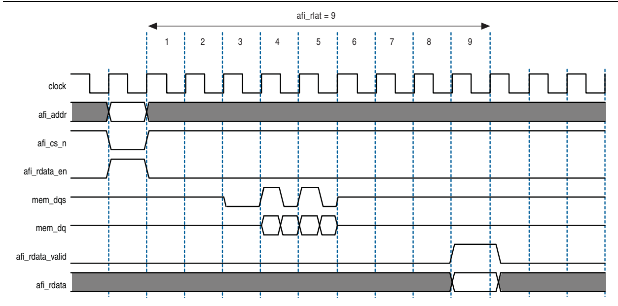
Figure 6-9. Full-Rate Reads
