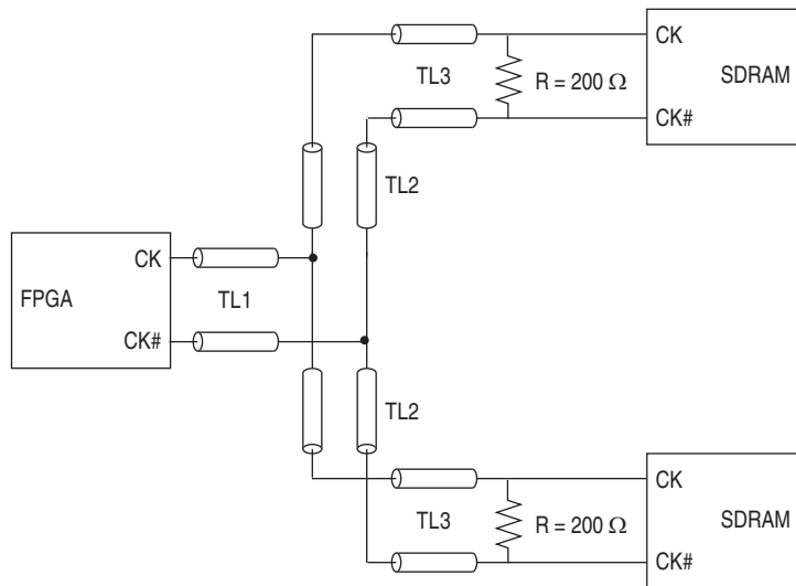
Figure 2-26. Placement of the Termination Resistor—End of Each Segment
