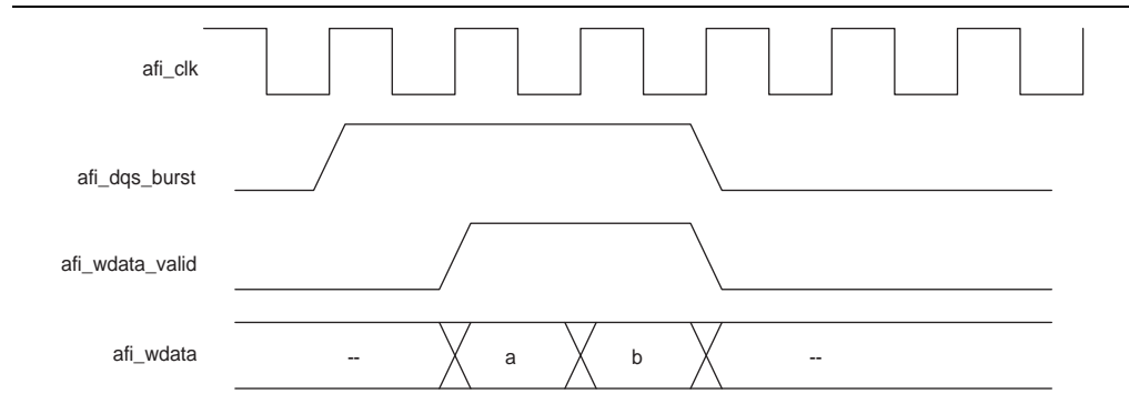
Figure 5-7. Full-Rate Write
