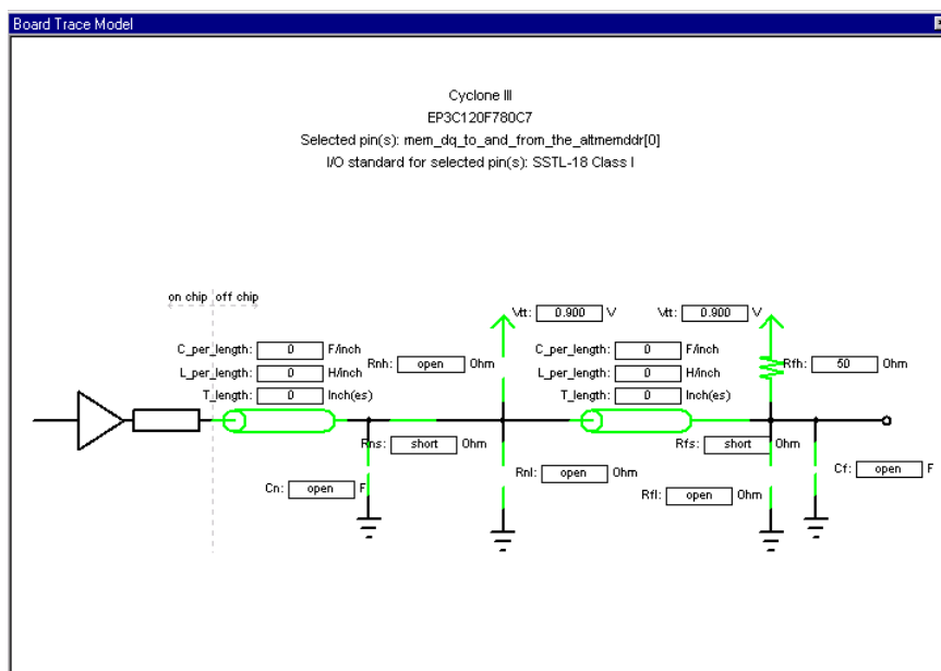
Figure 6-18. Board Trace Model
