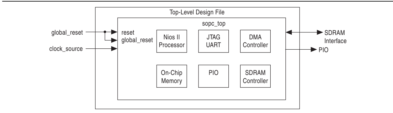
Figure 6-12. SOPC Builder Top-Level Block Diagram
