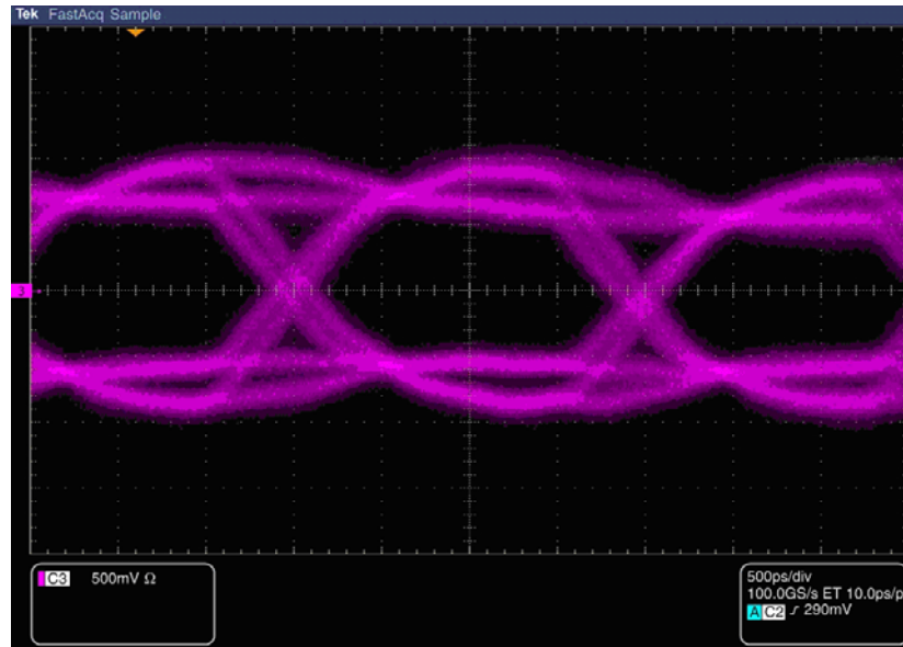
Figure 1-19. Board Measurement, FPGA Writing to Memory
