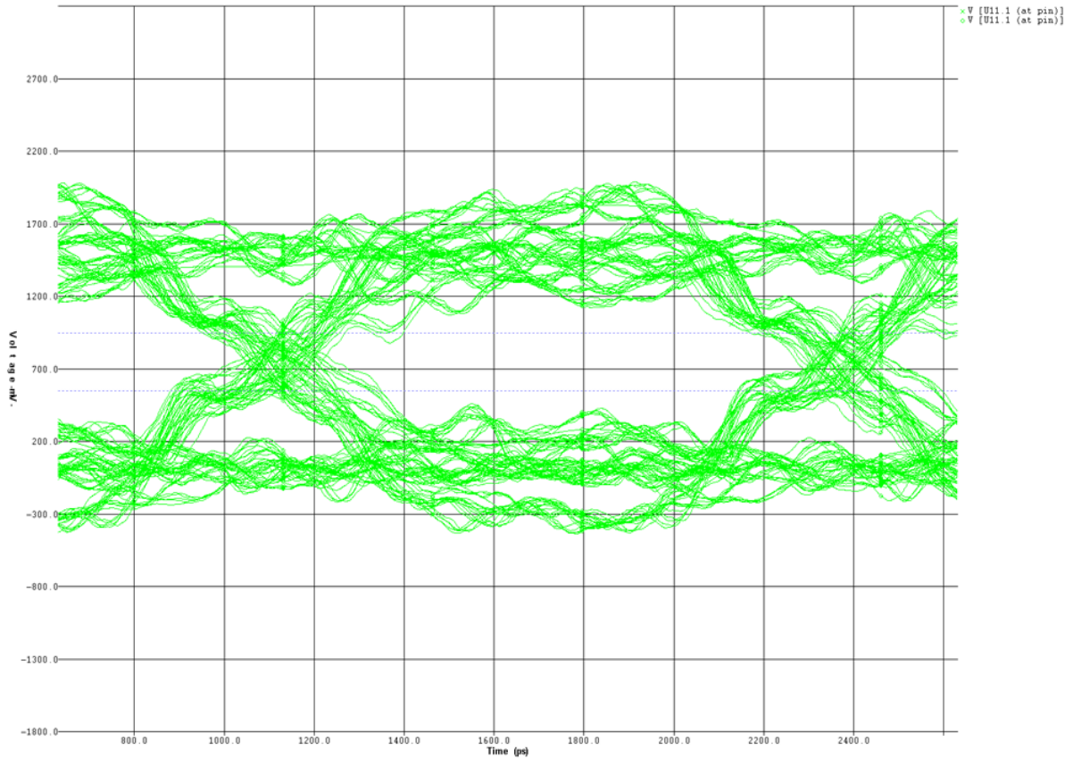
Figure 4-5. Write Data Simulation at 400 MHz with No Far-End Termination
