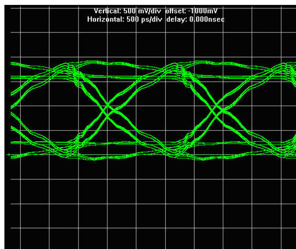
Figure 1-40. HyperLynx Simulation with a 16-mA Drive Strength Setting on the FPGA
