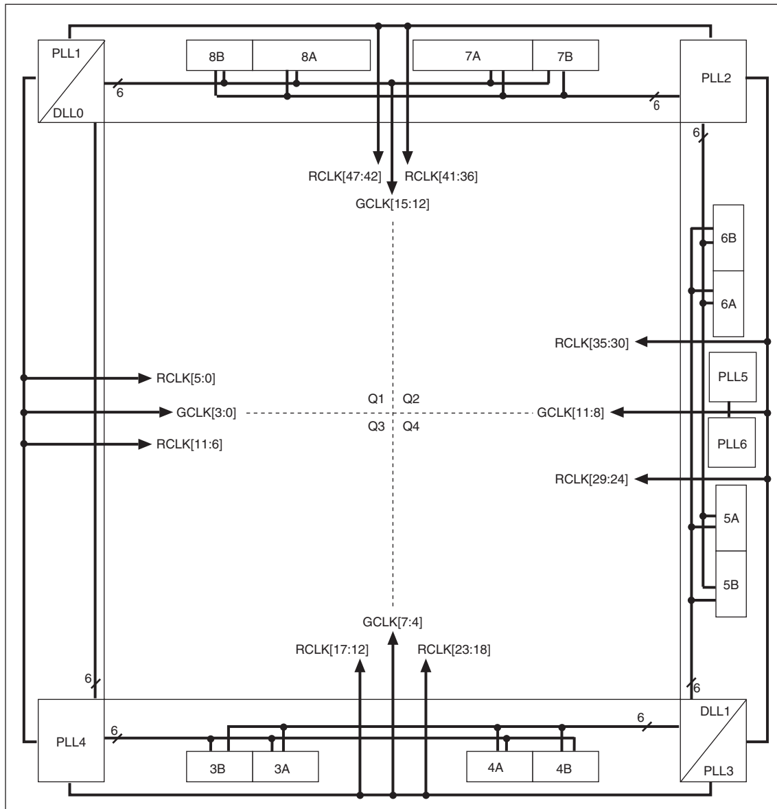
Figure 1-1. PLL and DLL Locations in Arria II GX Devices
