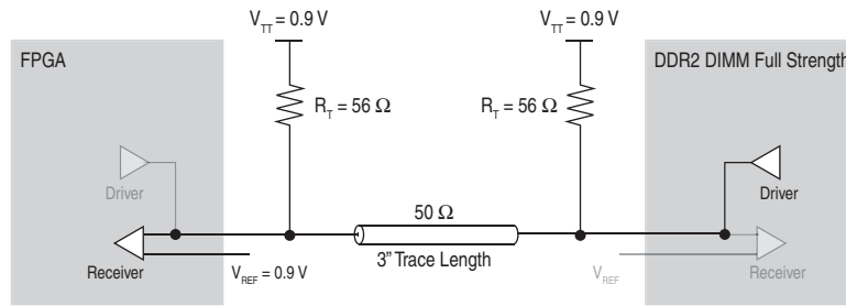
Figure 1-20. Class II Termination Scheme with Memory-Side Series Resistor
