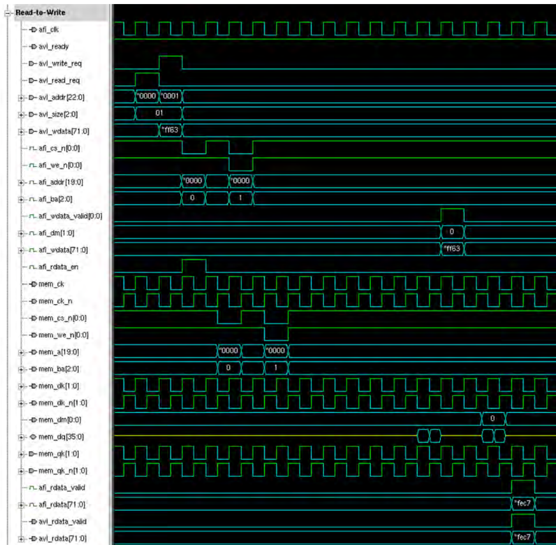
Figure 8-4. Read-to-Write Signals
