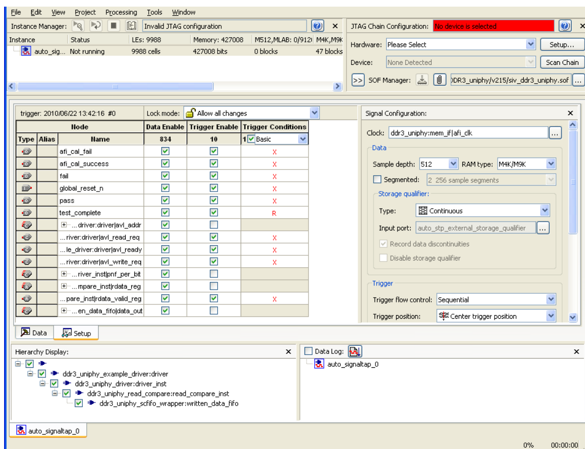
Figure 3-5. SignalTap II Embedded Logic Analyzer
