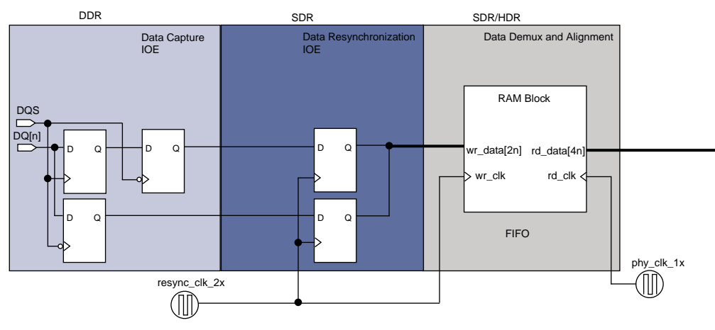
Figure 5-9. DDR3 SDRAM Read Datapath in Arria II GX Devices
