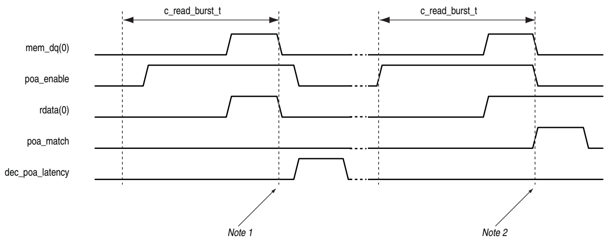
Figure 3-3. Calibration Timing
