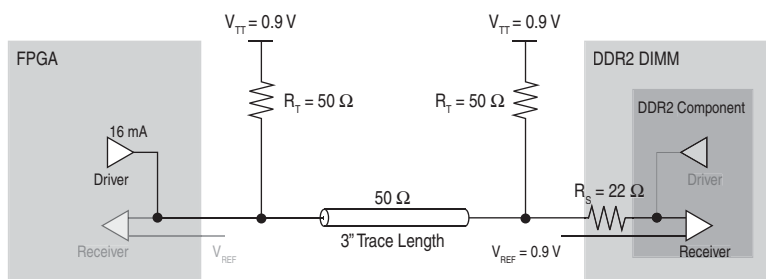
Figure 1-17. Class-II Termination Scheme with Memory-Side Series Resistor
