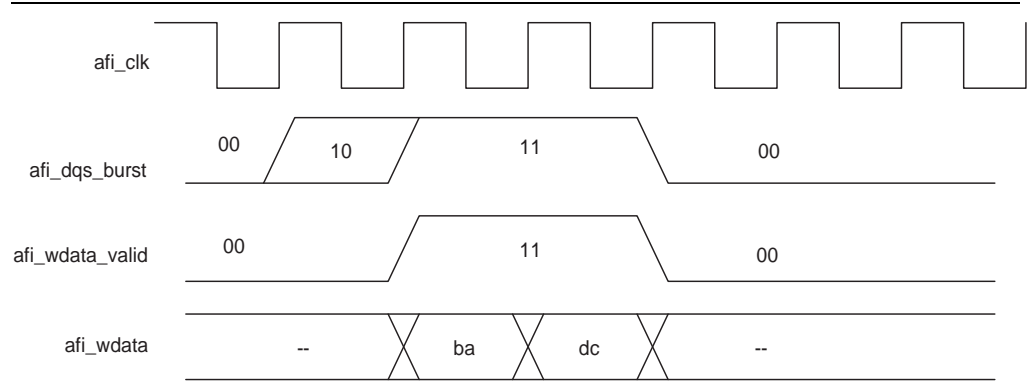
Figure 5-6. Half-Rate Write with Word-Aligned Data
