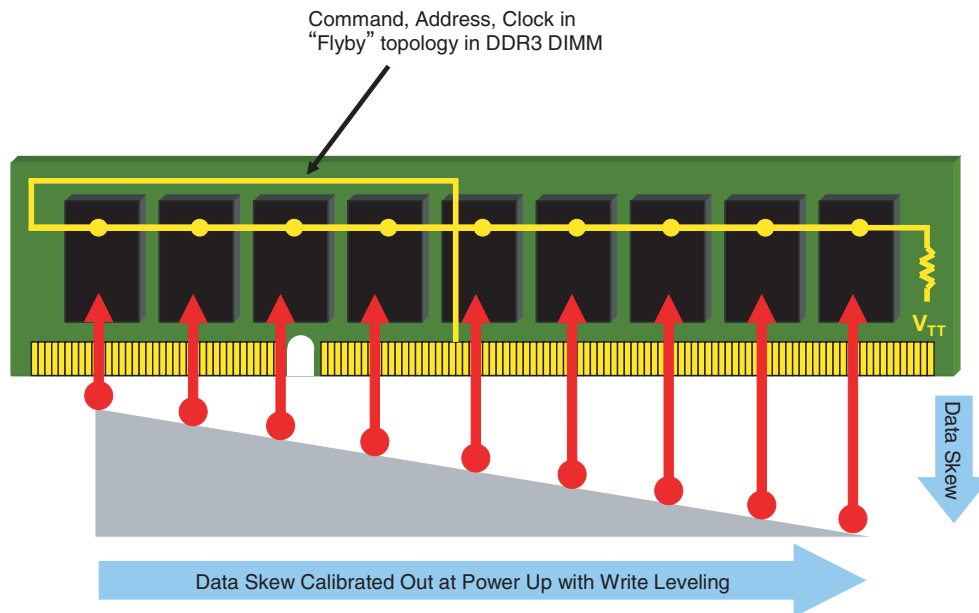
Figure 2-1. DDR3 DIMM Fly-By Topology Requiring Write Leveling (Note 1)
