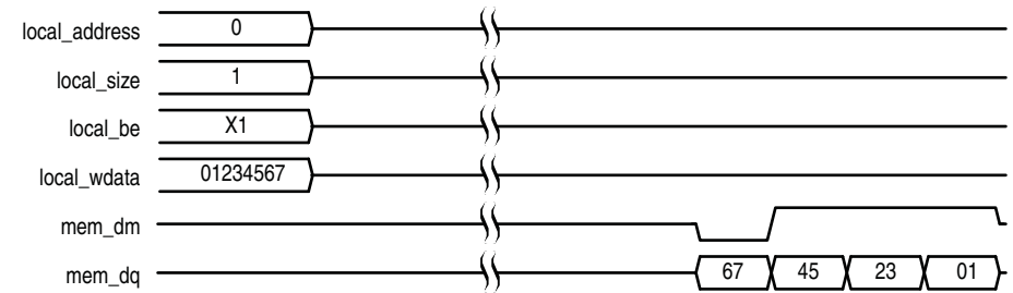
Figure 5-5. Partial Burst for Controller
