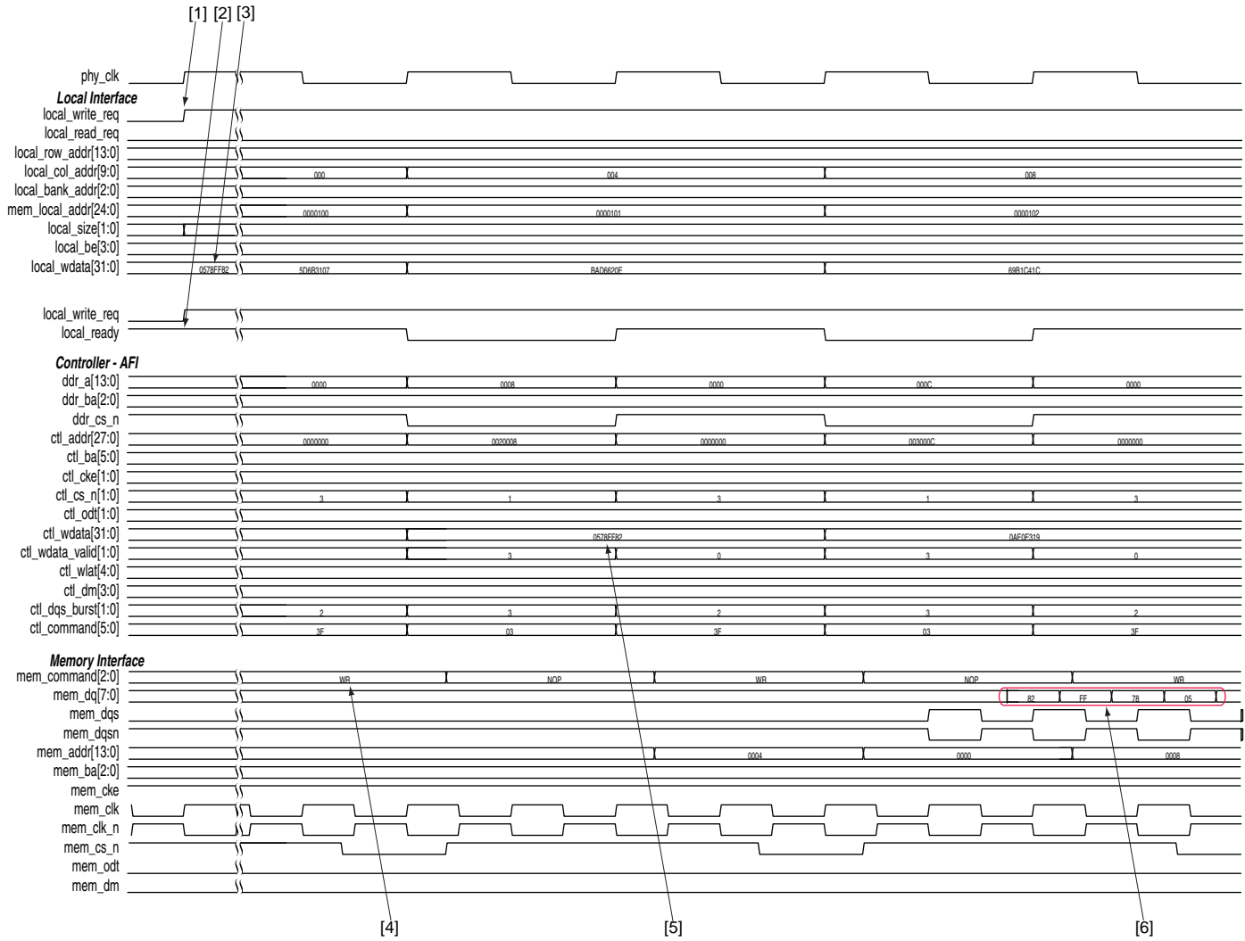
Figure 9-4. Half-Rate Write Operation for HPC Using Avalon Interface
