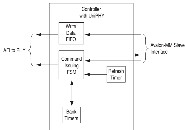
Figure 4-1. RLDRAM II Controller Architecture Block Diagram
