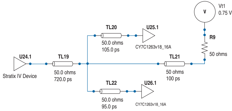
Figure 4-8. Address for QDR II SRAM Burst Length of 2 in Width Expansion Mode Topology
