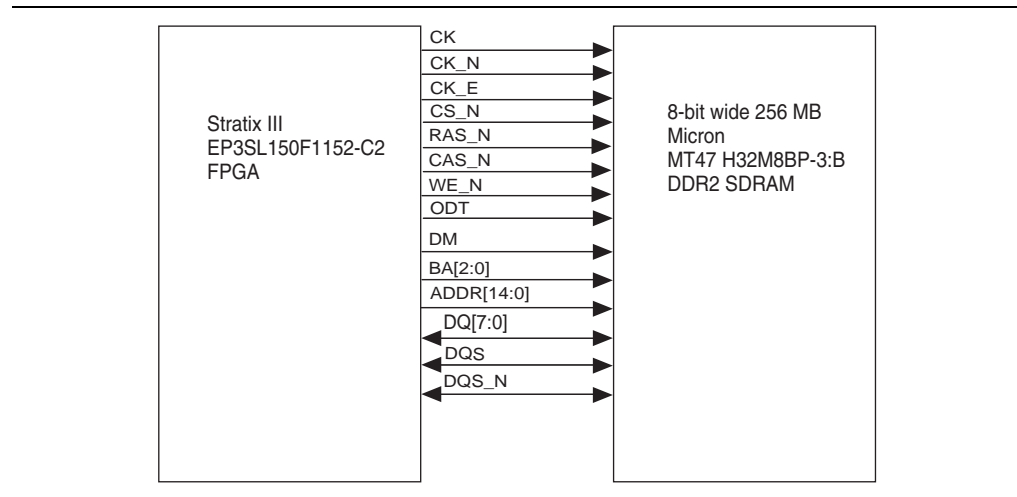
Figure 2-1. Interface Between a Stratix III Device and a DDR2 SDRAM Component
