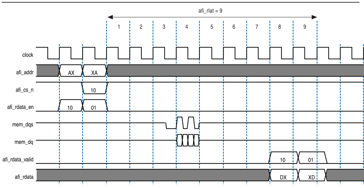
Figure 5-9. Half-Rate Reads
