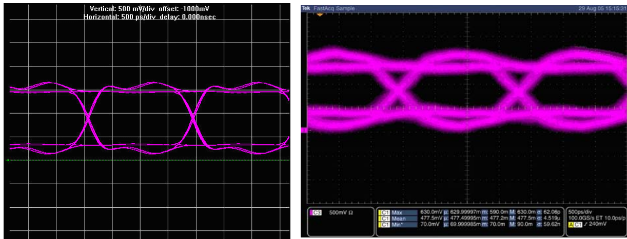
Figure 1-39. HyperLynx Simulation and Measurement, FPGA Reading from the DDR2 SDRAM Component
