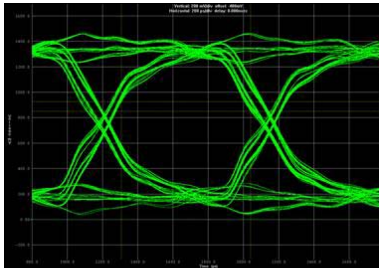
Figure 2-16. Write-Eye Diagram of a DDR3 SDRAM Component Using a 120-Ω ODT Setting
