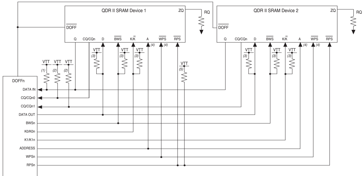
Figure 4–2. Configuration With Two QDR II SRAM Components In A Width Expansion Configuration
