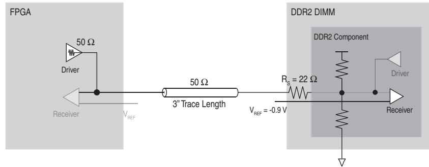
Figure 1-13. Class I Termination Using ODT with 50-ΩOCT
