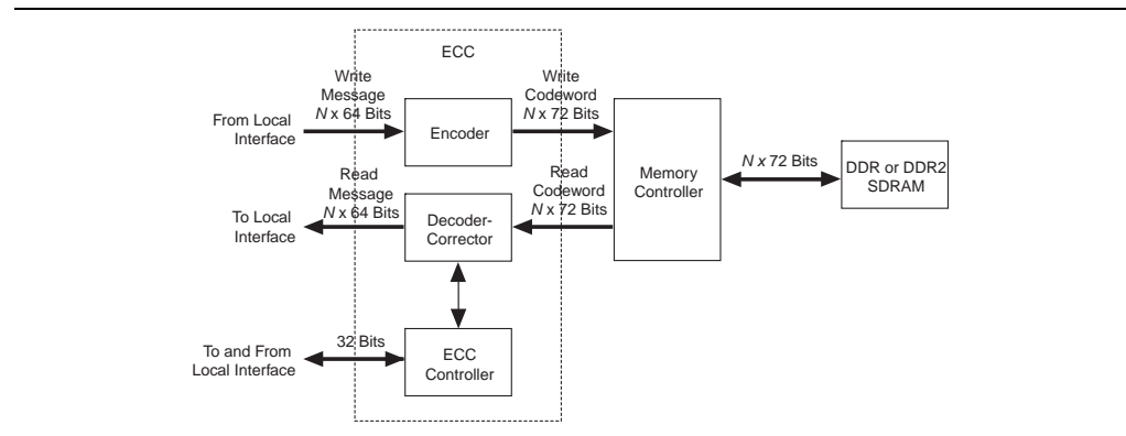
Figure 6-3. ECC Block Diagram
