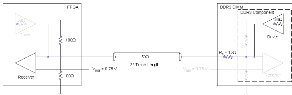
Figure 2-13. DDR3 SDRAM Component Driving the Stratix III and Stratix IV FPGA Device with Parallel 50- \Omega OCT Turned On
