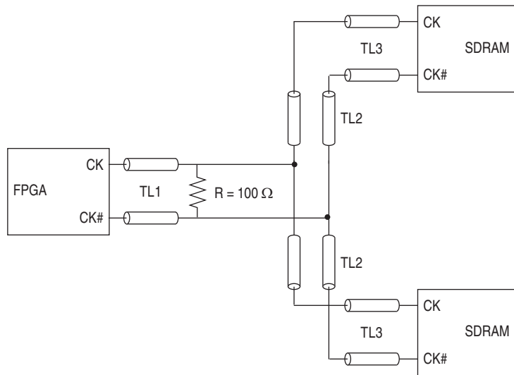
Figure 2-25. Placement of the Termination Resistor—at First Split
