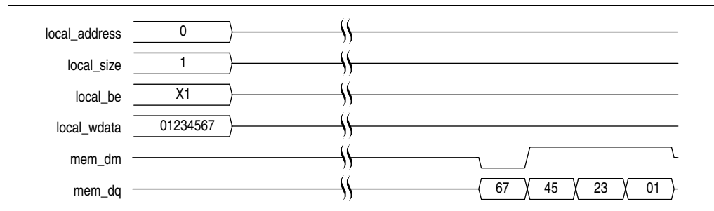
Figure 7-5. Partial Burst for HPC II
