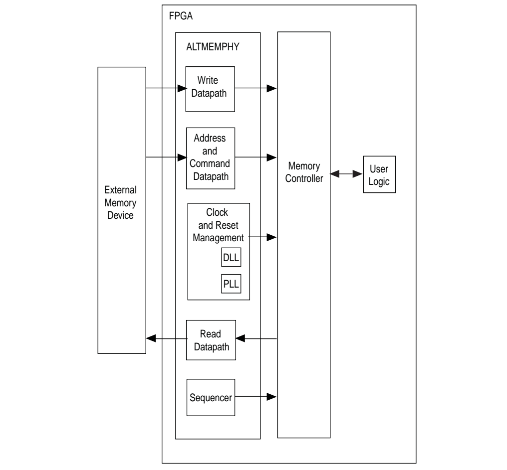
Figure 5-1. ALTMEMPHY Megafunction Interfacing with the Controller and the External Memory
