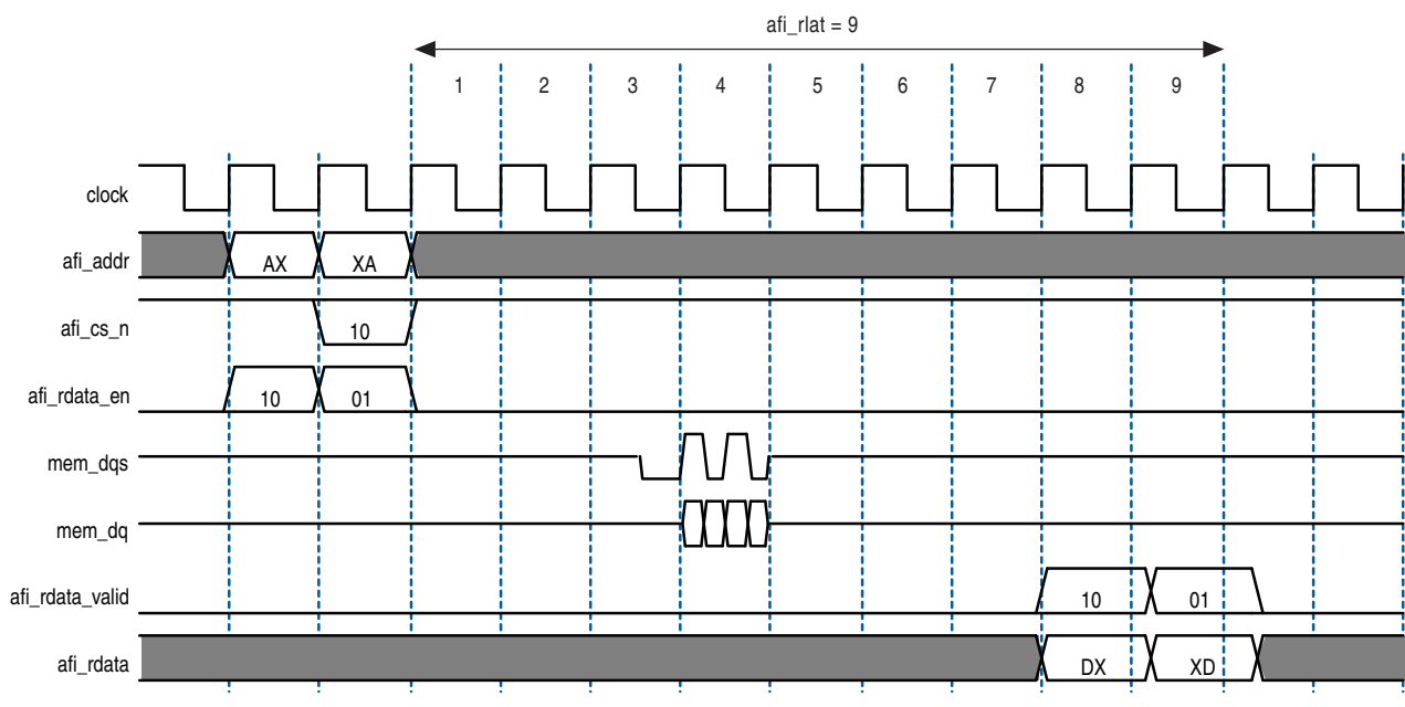
Figure 5-9. Half-Rate Reads
