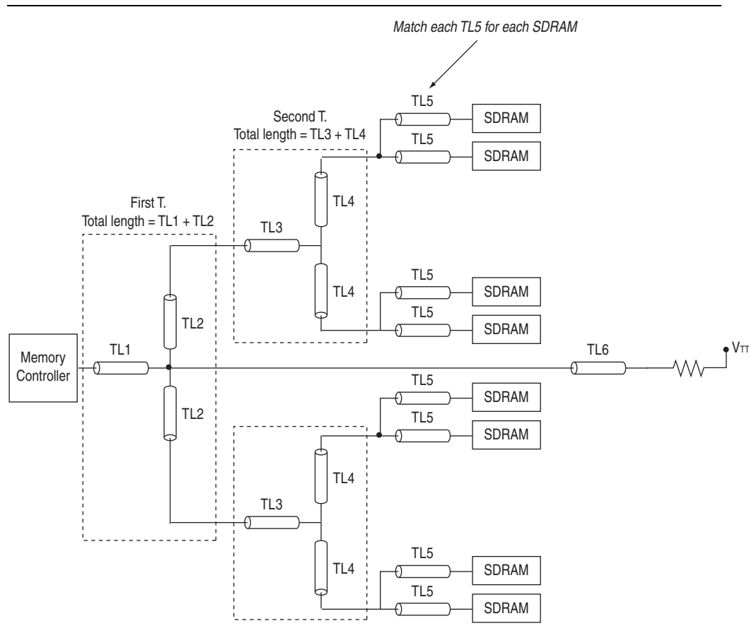
Figure 2-27. Placing the 50-Ω Resistor
