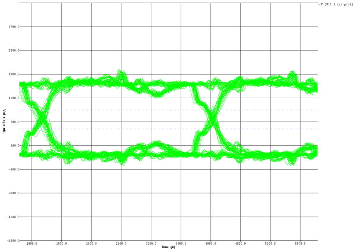
Figure 4-7. Address Simulation for QDR II SRAM Burst Length of 4 at 175 MHz with No Far-End Termination
