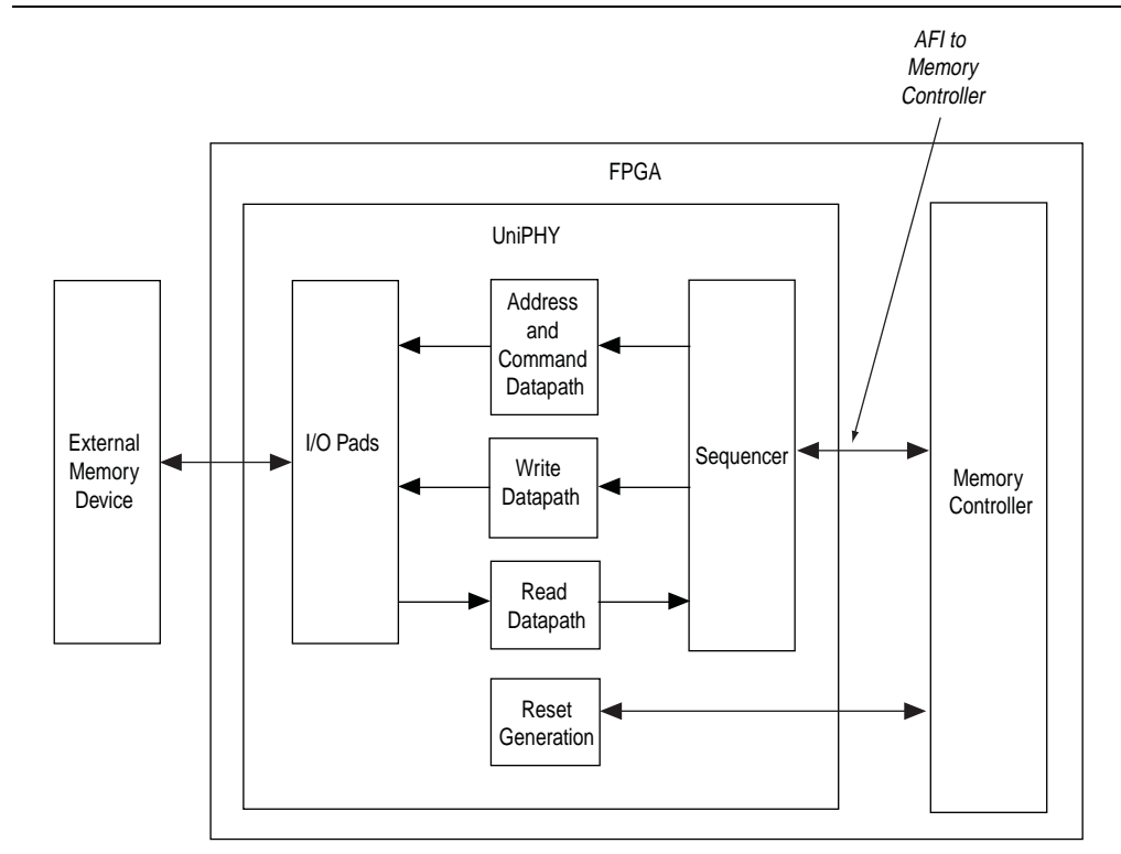
Figure 5–1. PHY Block Diagram
