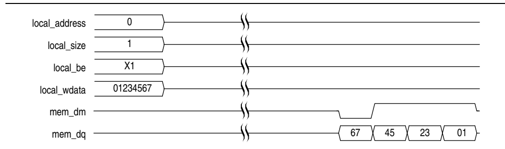
Figure 6-6. Partial Burst for HPC
