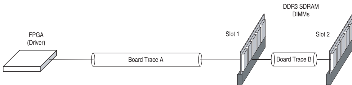
Figure 3-20. Multi DIMM DDR3 DQS, DQ, and DM, and Address and Command Termination Topology
