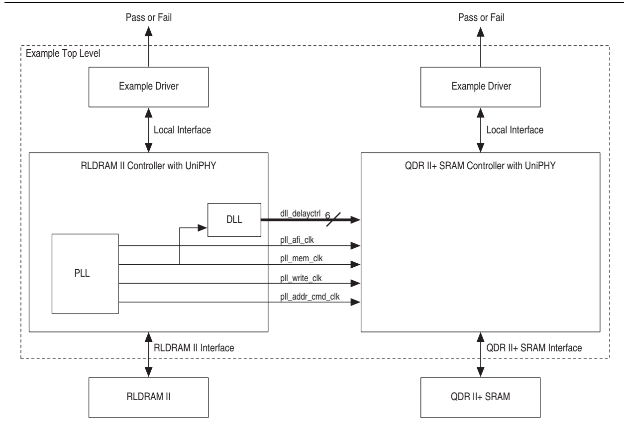
Figure 4-2. Multiple Memory-Controller Top-Level Diagram
