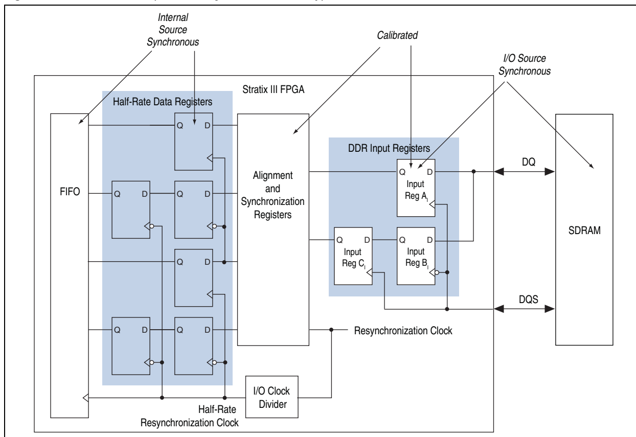
Figure 1-2. Stratix IV and Input Path Registers and Circuit Types in SDRAM Interface
