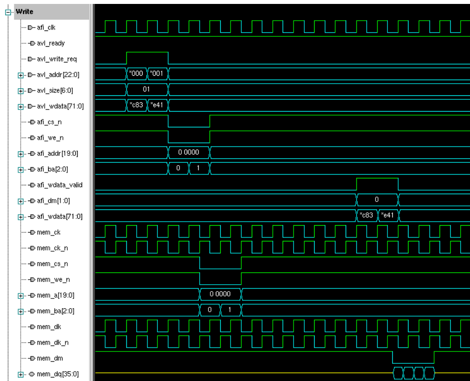
Figure 8–1. Back-to-Back Writes
