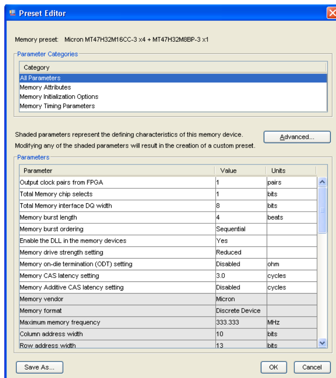
Figure 6-8. Preset Editor
