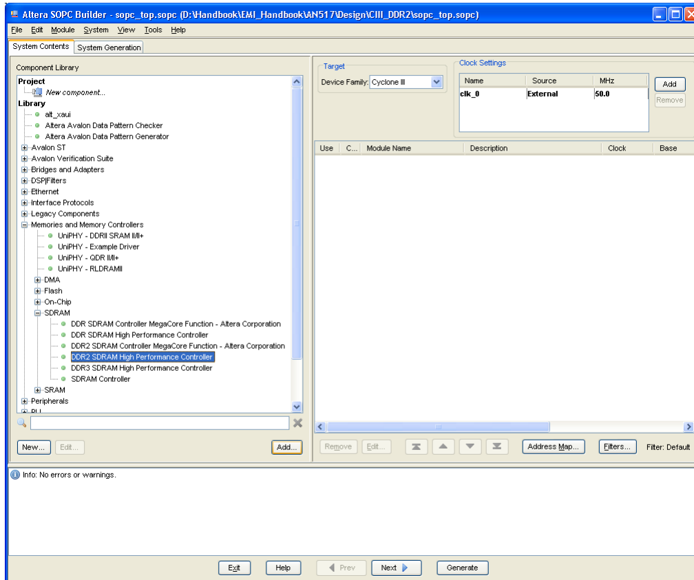
Figure 6-6. System Content
