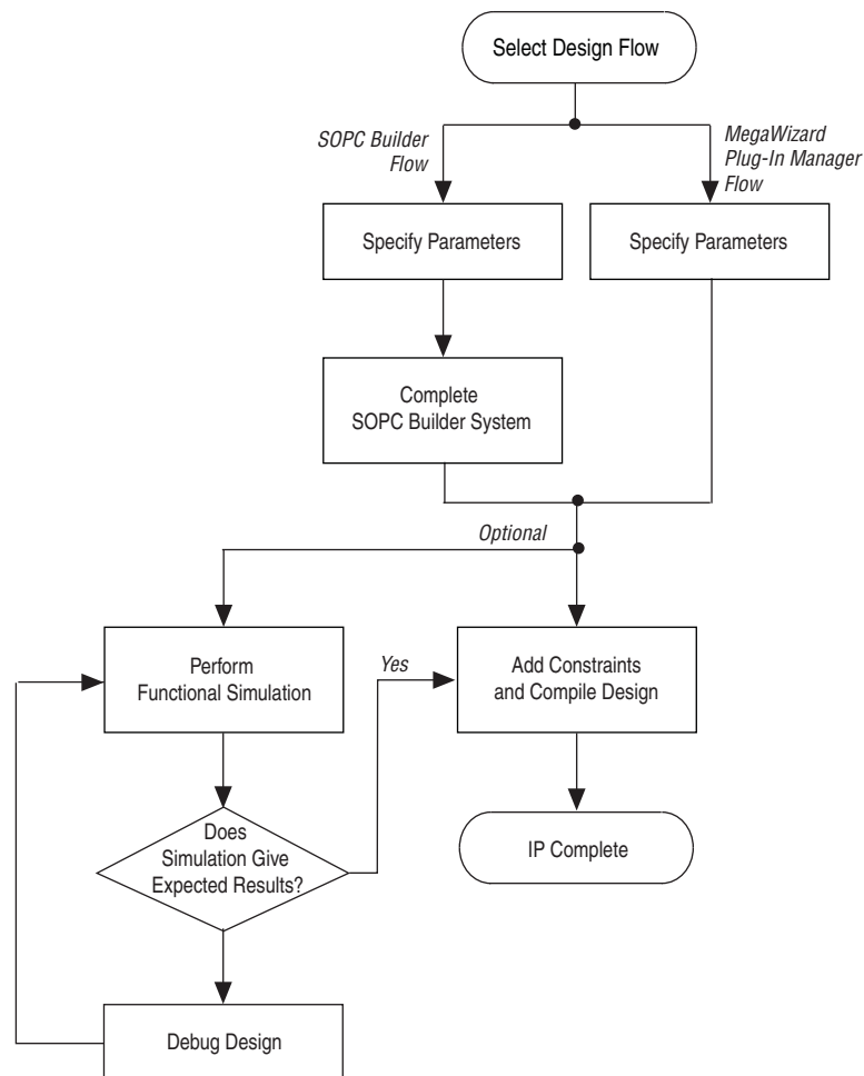
Figure 2-1. Design Flows
