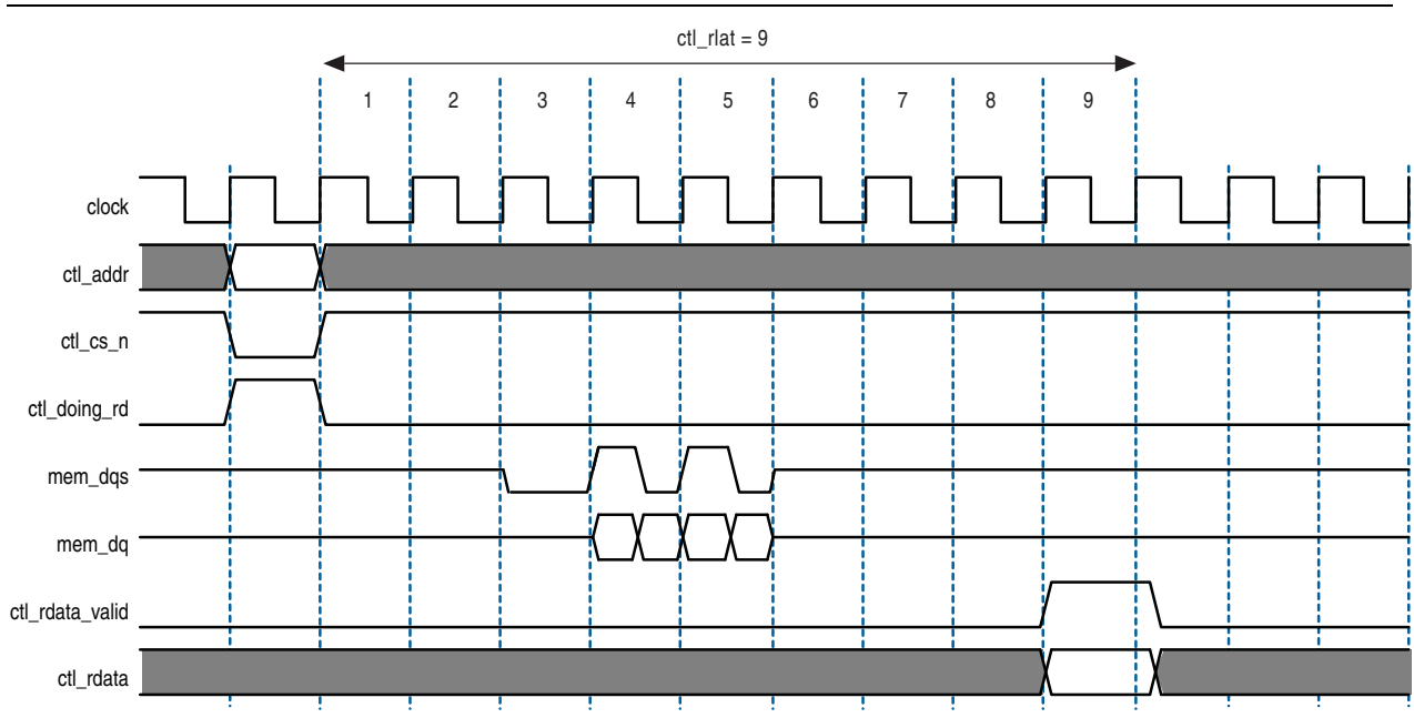
Figure 5-17. Full-Rate Reads
