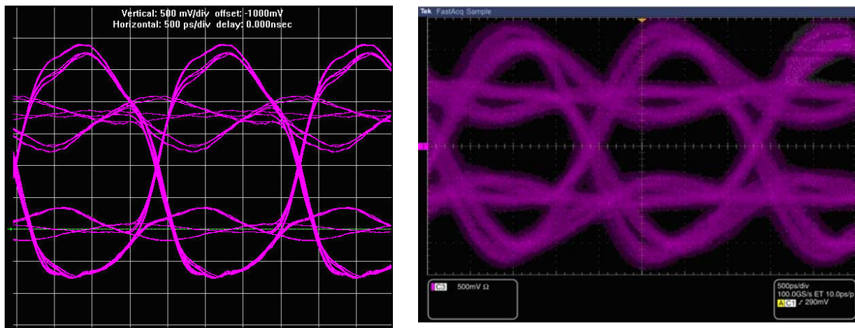
Figure 1-34. HyperLynx Simulation and Measurement, FPGA Reading from Memory
