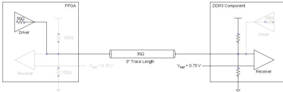
Figure 2-15. Stratix III and Stratix IV FPGA Writing to a DDR3 SDRAM Components
