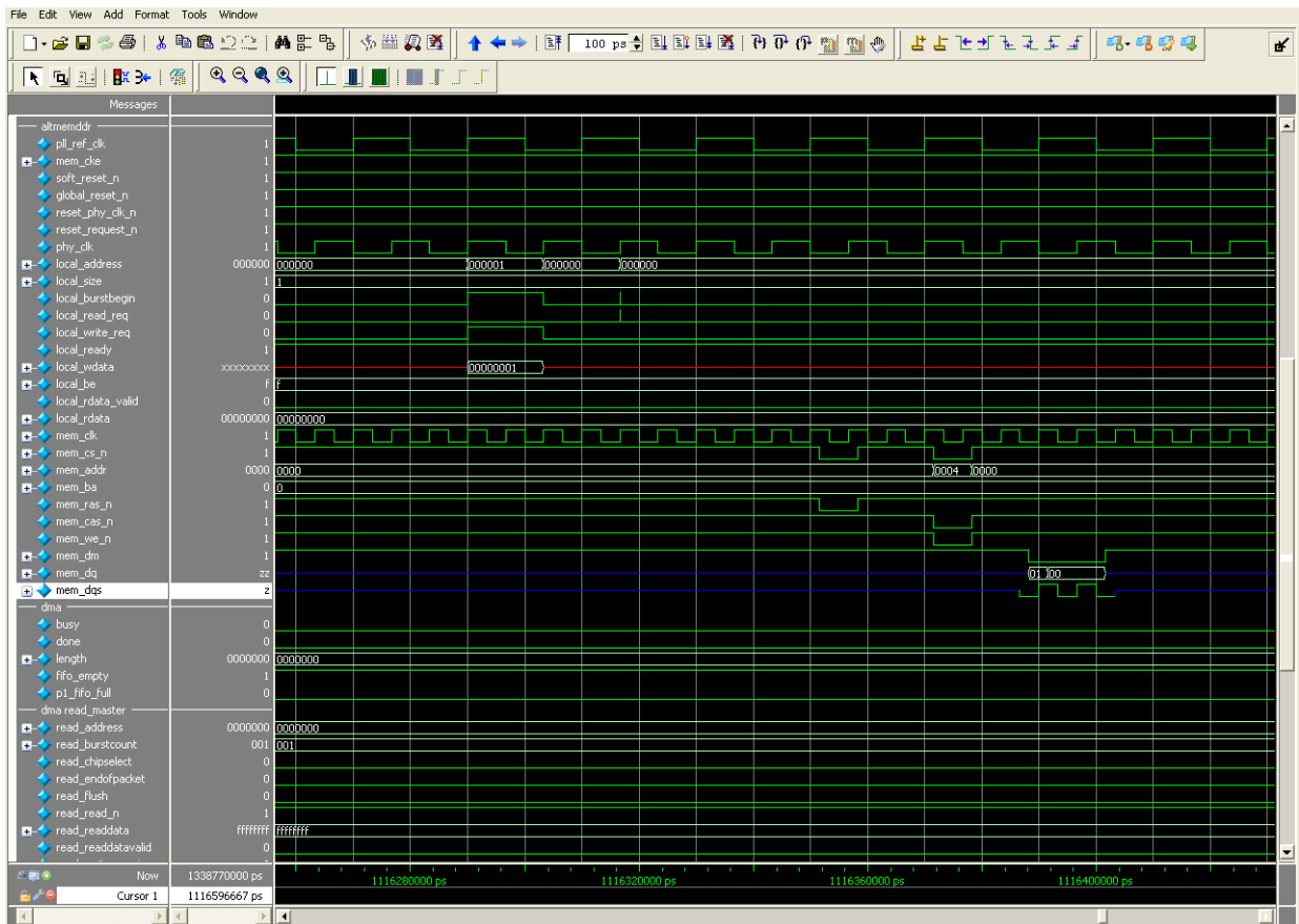
Figure 6-24. Waveform for Single Write Operation
