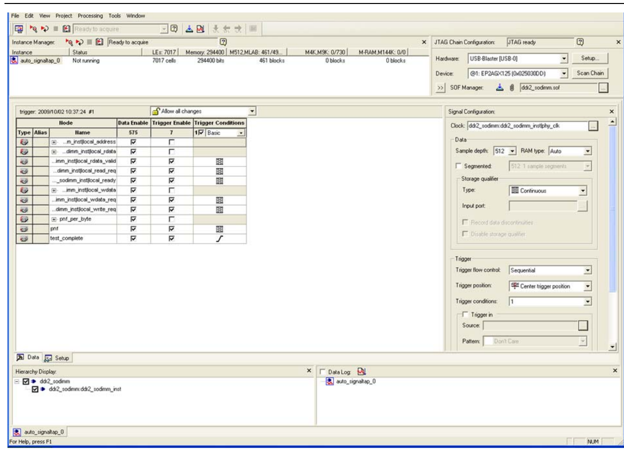
Figure 2-11. SignalTap II Embedded Logic Analyzer
