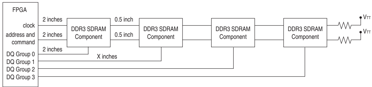
Figure 2-24. DDR3 SDRAM Components DQ, DQS, DM Routing Guidelines
