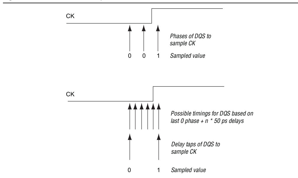
Figure 3-5. Determine Phase Tap
