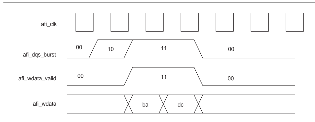
Figure 6-7. Half-Rate Write with Word-Aligned Data
