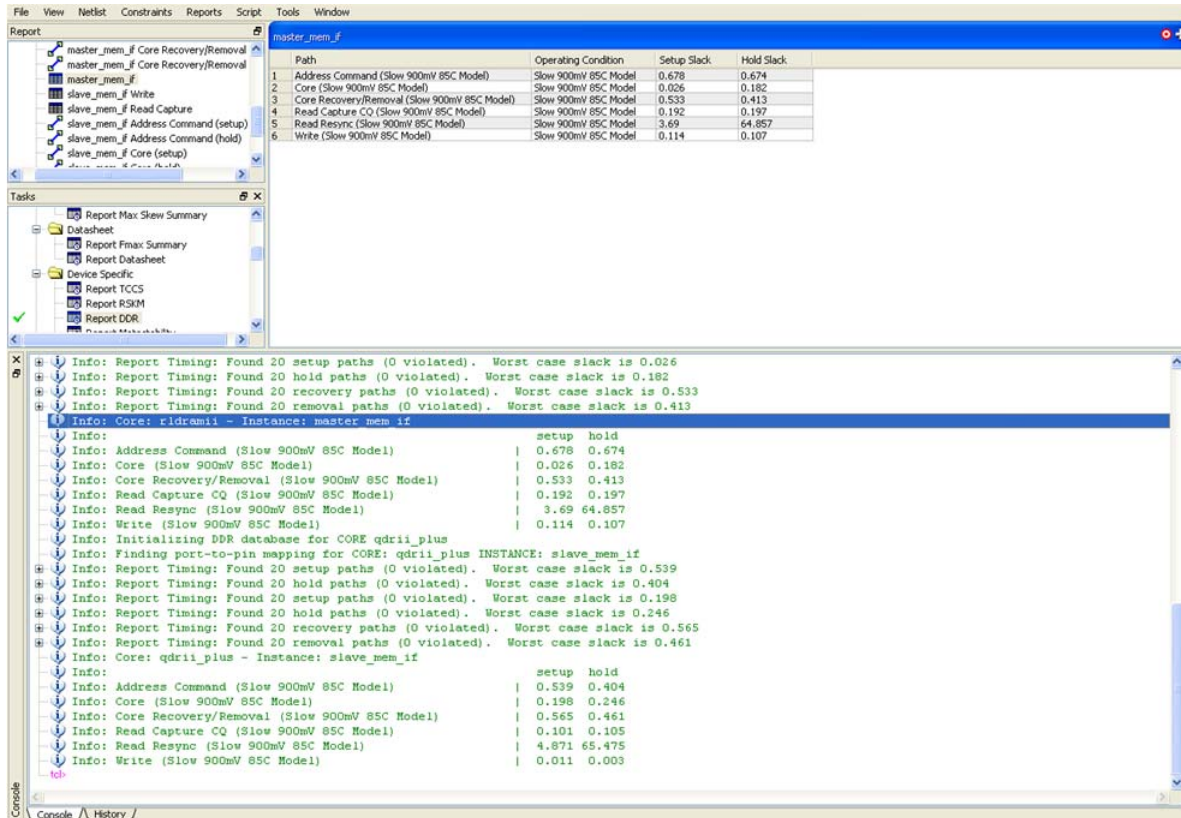
Figure 4-6. Timing Margin Report in TimeQuest Timing Analyzer
