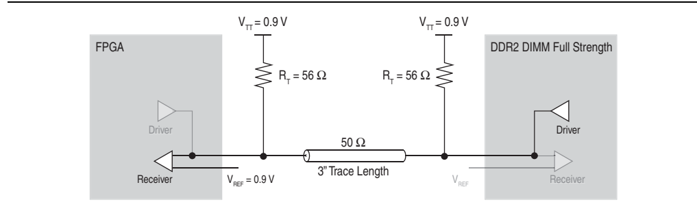
Figure 1-38. Class II Termination Scheme without Memory-Side Series Resistor
