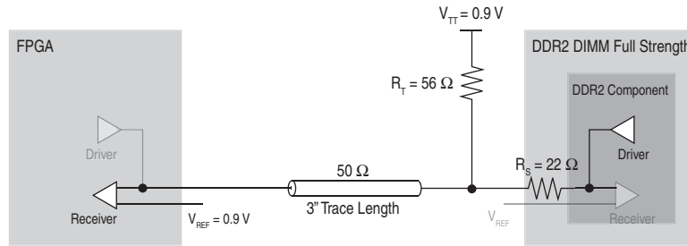
Figure 1-25. Class I Termination Scheme with Memory-Side Series Resistor
