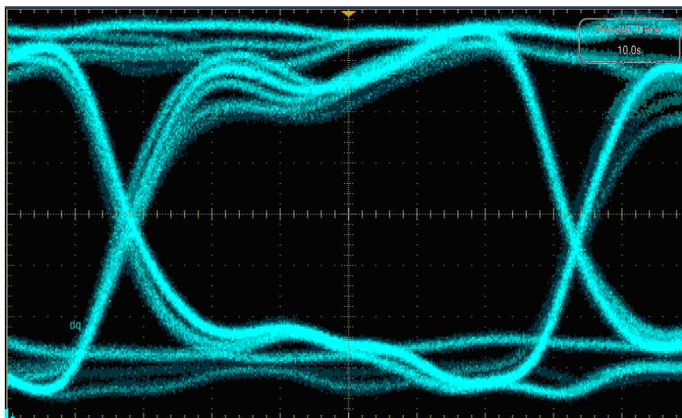
Figure 1-10. Board Measurement, FPGA Writing to Memory
