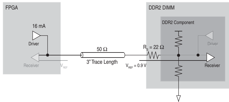
Figure 1-27. Class I Termination Scheme Using ODT
