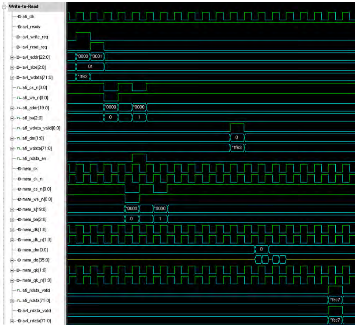
Figure 8-5. Write-to-Read Signals
