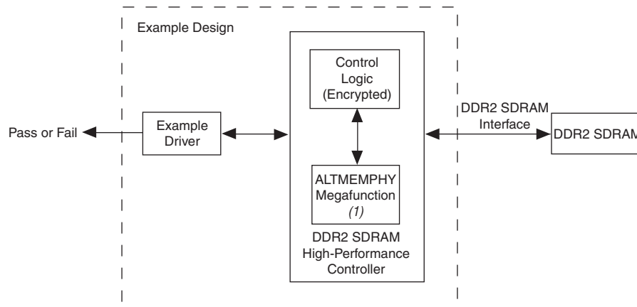
Figure 3-8. DDR2 SDRAM Controller with ALTMEMPHY IP System-Level Diagram
