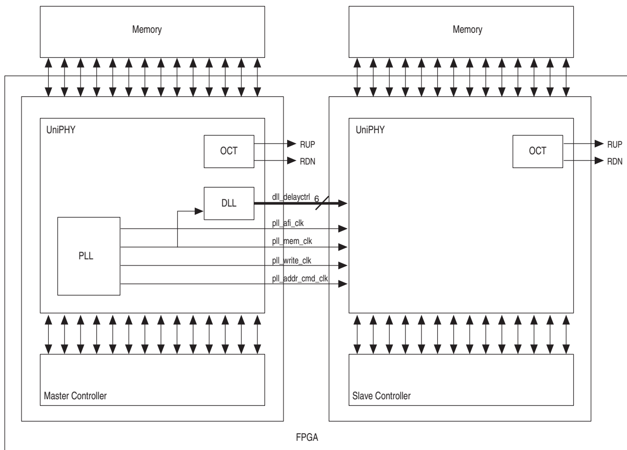
Figure 4-1. A Master-Slave Scenario Sharing DLL and PLL Clocks
