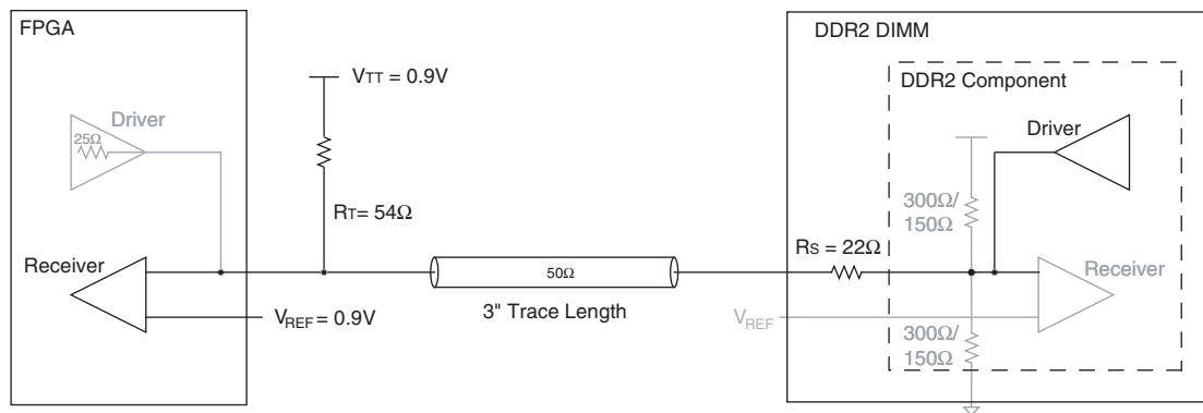
Figure 3-10. Single Parallel Termination Scheme (Class I) Using External Resistor and Memory-Side Series Resistor
