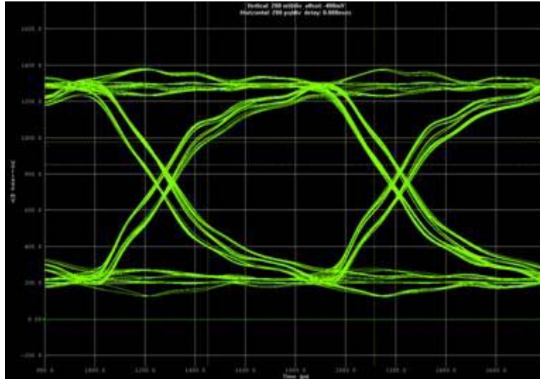
Figure 2-6. Simulated Write-Eye Diagram of a DDR3 SDRAM DIMM Using a 120- Ω ODT Setting
