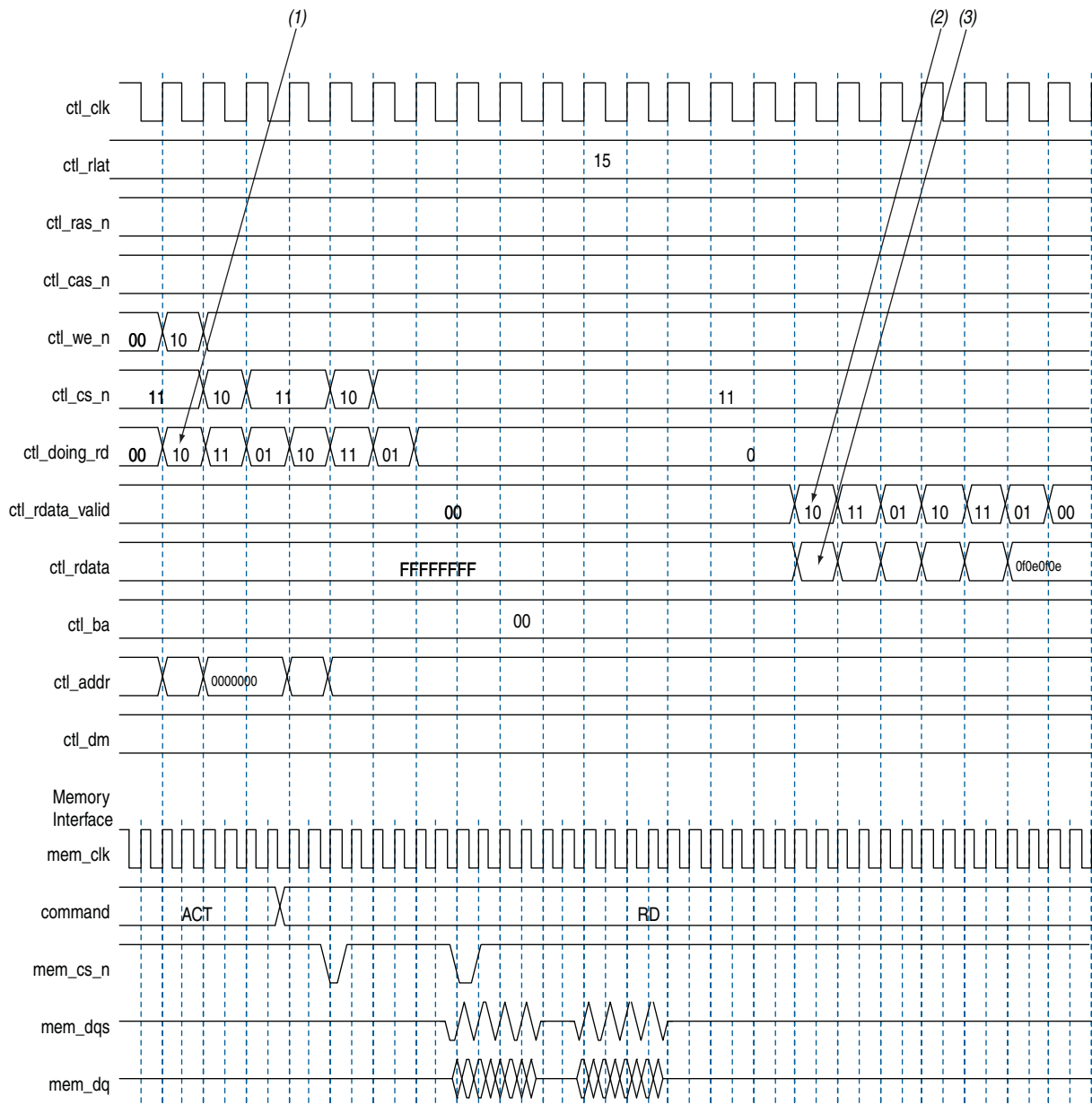
Figure 5-22. Word-Unaligned Reads
