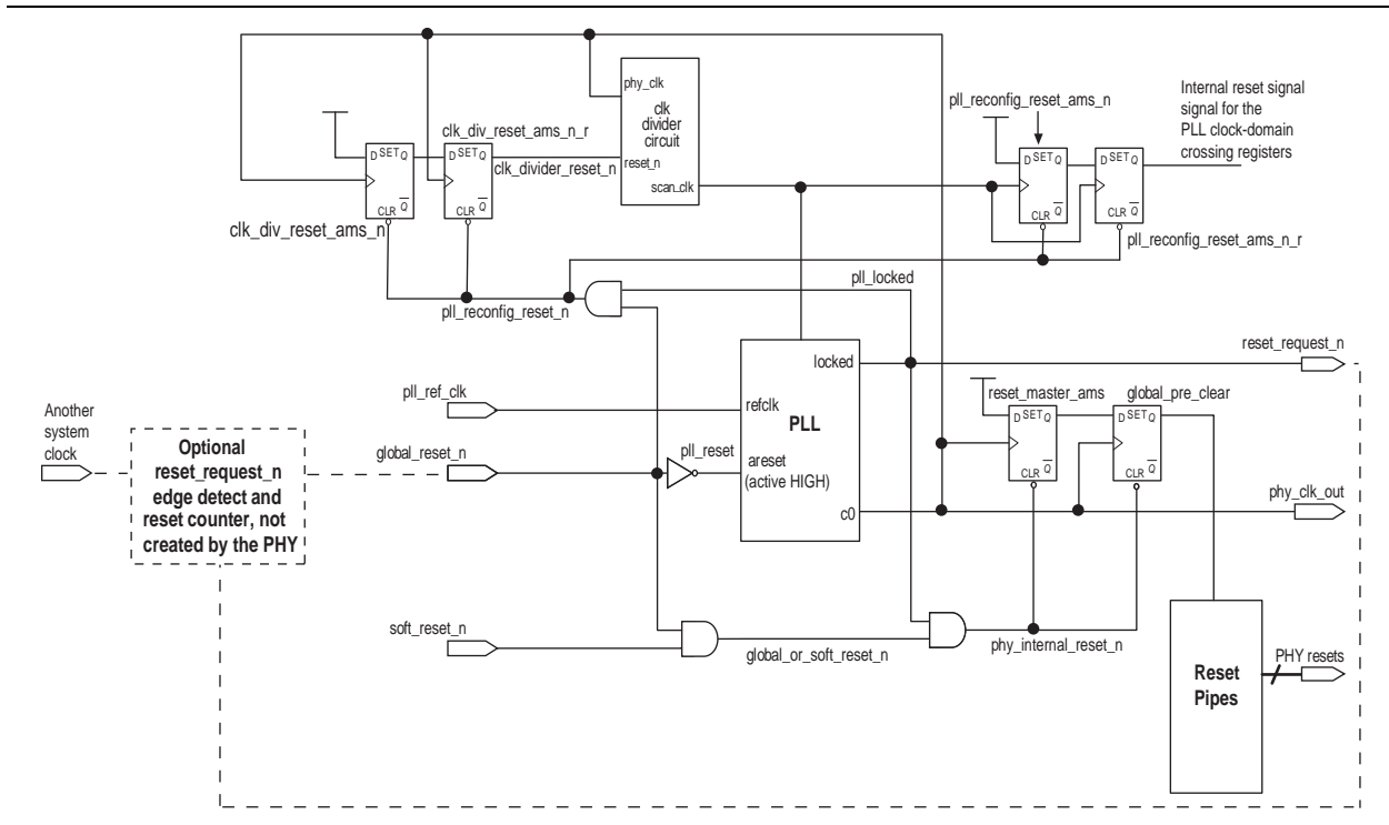
Figure 5-6. ALTMEMPHY Reset Management Block for Stratix IV and Stratix III Devices
