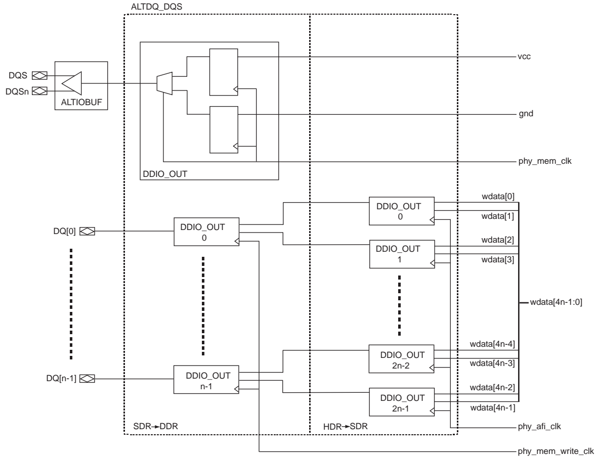
Figure 6-3. Write Datapath
