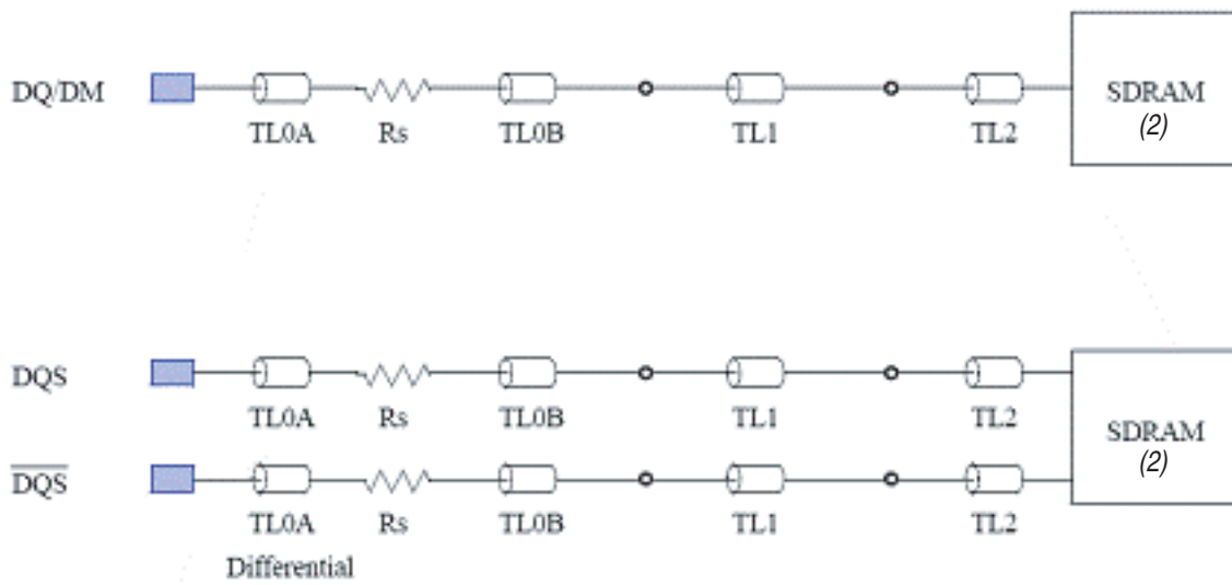
Figure 2-5. DQ and DQS Net Structure for 64-Bit DDR3 SDRAM Unbuffered DIMM (Note 1)
