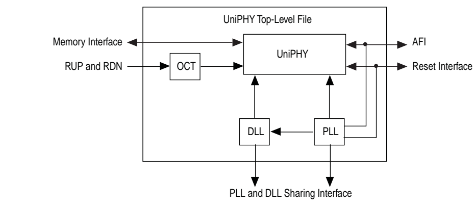
Figure 5-5. UniPHY Interfaces with the Controller and the External Memory
