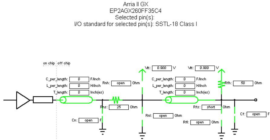
Figure 2-5. Board Trace Model
