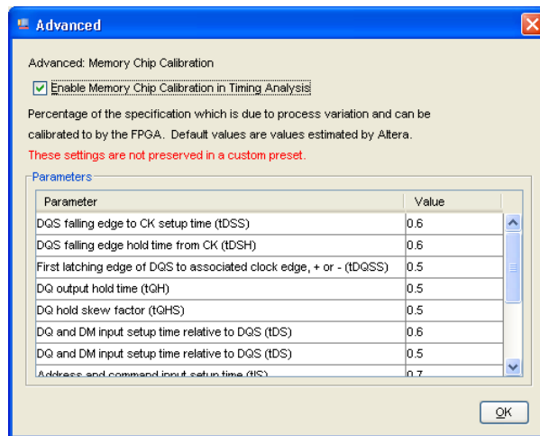
Figure 6-9. Advanced Memory Settings
