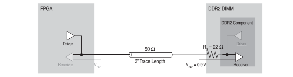
Figure 1-29. No-Parallel Termination Scheme
