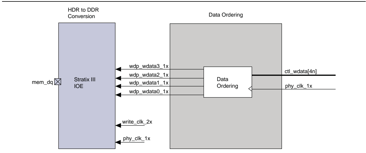
Figure 5-12. DDR and DDR2 SDRAM Write Datapath in Stratix IV and Stratix III Devices
