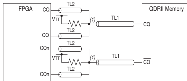
Figure 4-15. Emulated \times 36 Mode CQ/CQn Termination Topology
