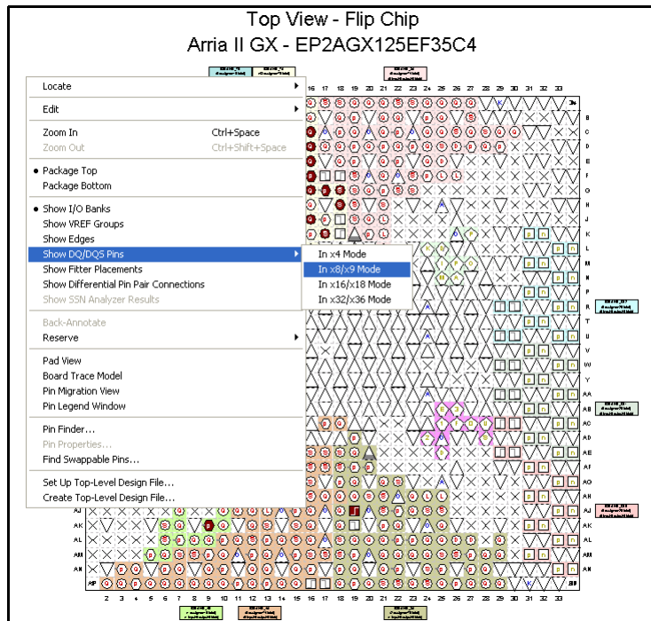
Figure 2-4. Quartus II Pin Planner, Show DQ/DQS Pins in x8/x9 Mode
