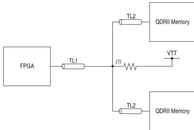
Figure 4-3. External Parallel Termination for Balanced Topology
