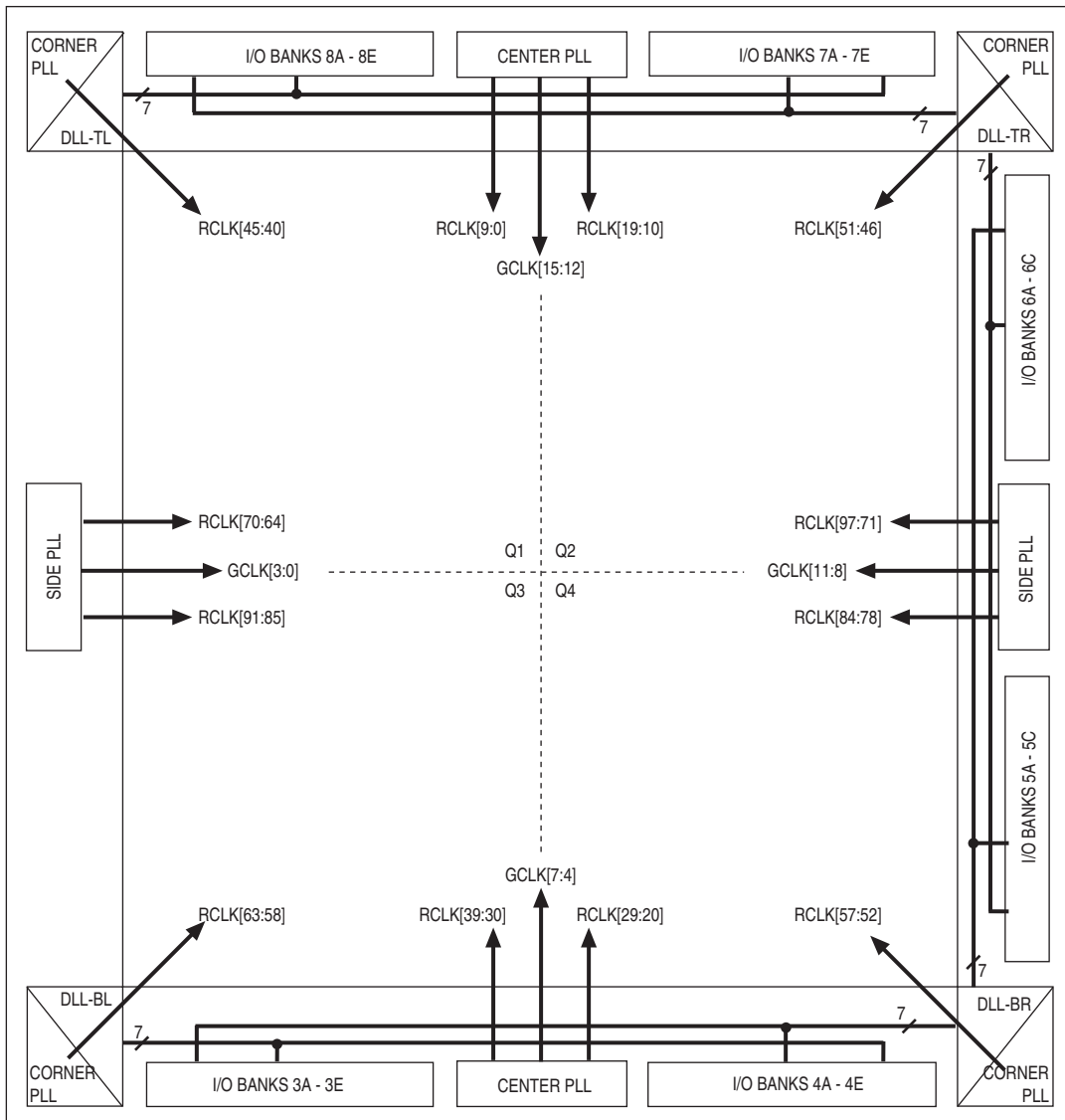
Figure 1-5. PLL and DLL Locations in Stratix V Devices
