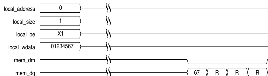
Figure 6-5. Partial Write for HPC—Half Rate
