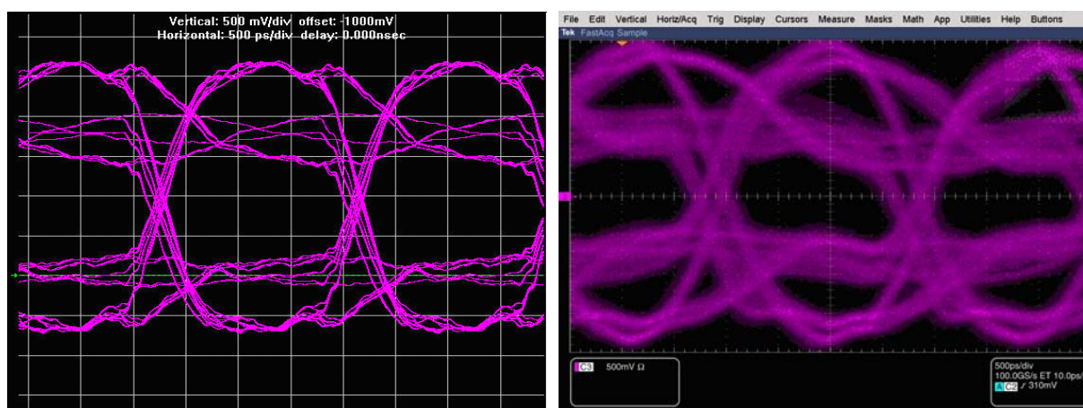
Figure 1-30. HyperLynx Simulation and Board Measurement, FPGA Writing to Memory
