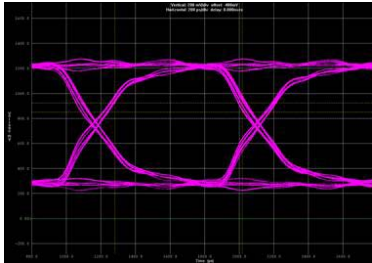
Figure 2-17. Write-Eye Diagram of a DDR3 SDRAM Component Using a 60-Ω ODT Setting
