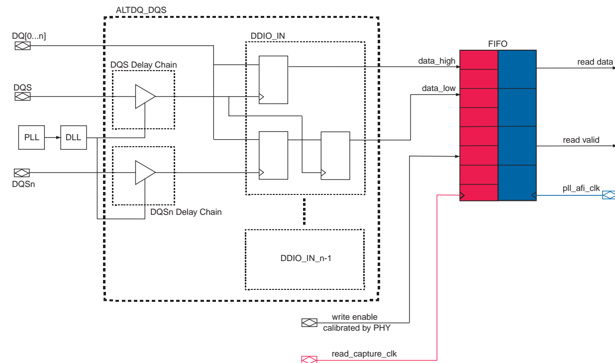
Figure 5-4. Read Datapath
