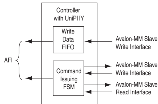
Figure 4-1. QDR II and QDR II+ SRAM Controller Architecture Block Diagram
