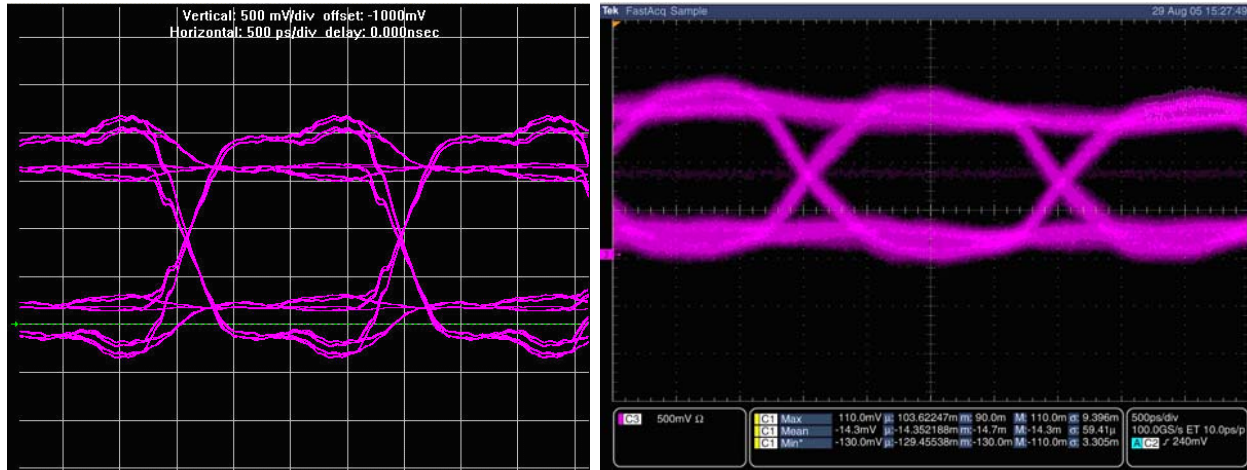
Figure 1-37. HyperLynx Simulation and Measurement of the Signal, FPGA Writing to Memory
