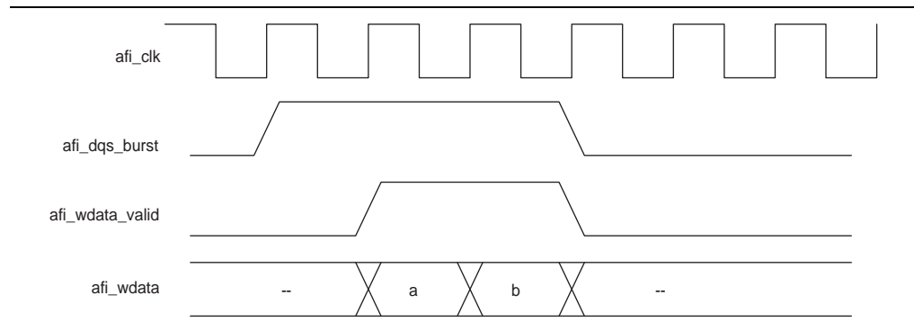
Figure 6-8. Full-Rate Write
