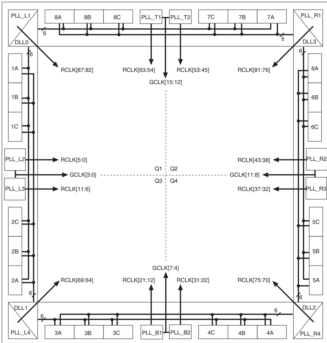
Figure 1-4. PLL and DLL Locations in Stratix III and Stratix IV Devices
