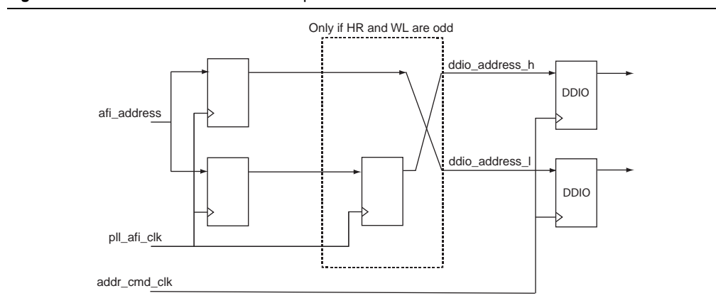
Figure 5-2. Address and Command Datapath
