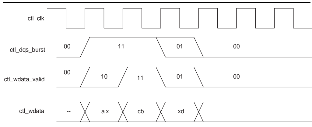
Figure 5-15. Half-Rate Write with Word-Unaligned Data
