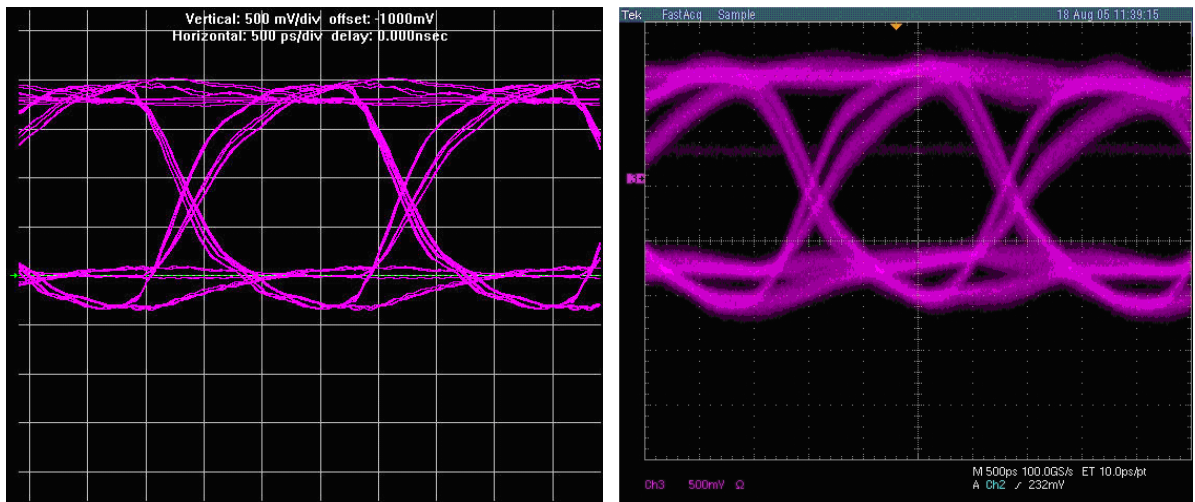
Figure 1-35. HyperLynx Simulation and Measurement, FPGA Writing to Memory
