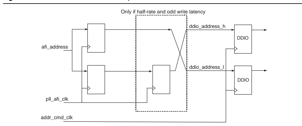
Figure 5-2. Address and Command Datapath
