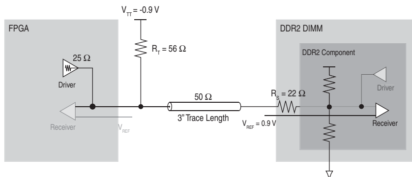
Figure 1-15. Class II Termination Using ODT with 25-Ω OCT
