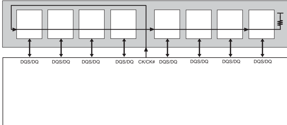
Figure 5-4. DDR3 SDRAM Unbuffered Module Clock Topology
