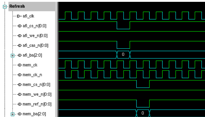
Figure 8-3. Refresh to Bank 0
