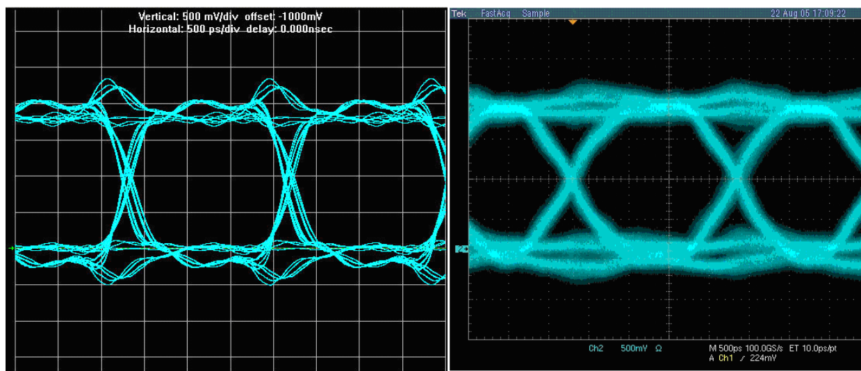
Figure 1-32. HyperLynx Simulation and Board Measurement, FPGA Reading from Memory
