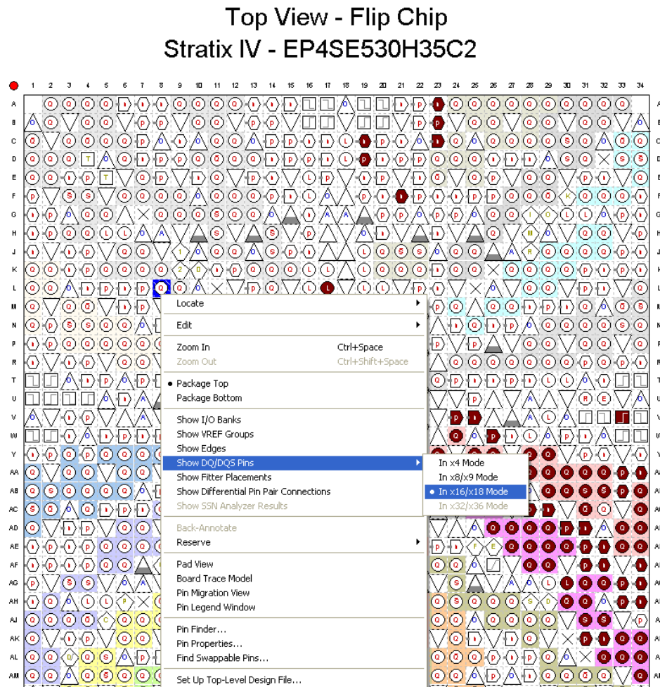
Figure 2-1. Quartus II Pin Planner, Show DQ/DQS Pins, In x16/x18 Mode
