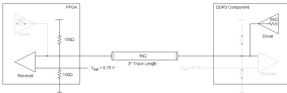
Figure 2-21. DDR3 SDRAM Component Driving the Stratix III and Stratix IV FPGA Device with Parallel 50- \Omega OCT Turned On
