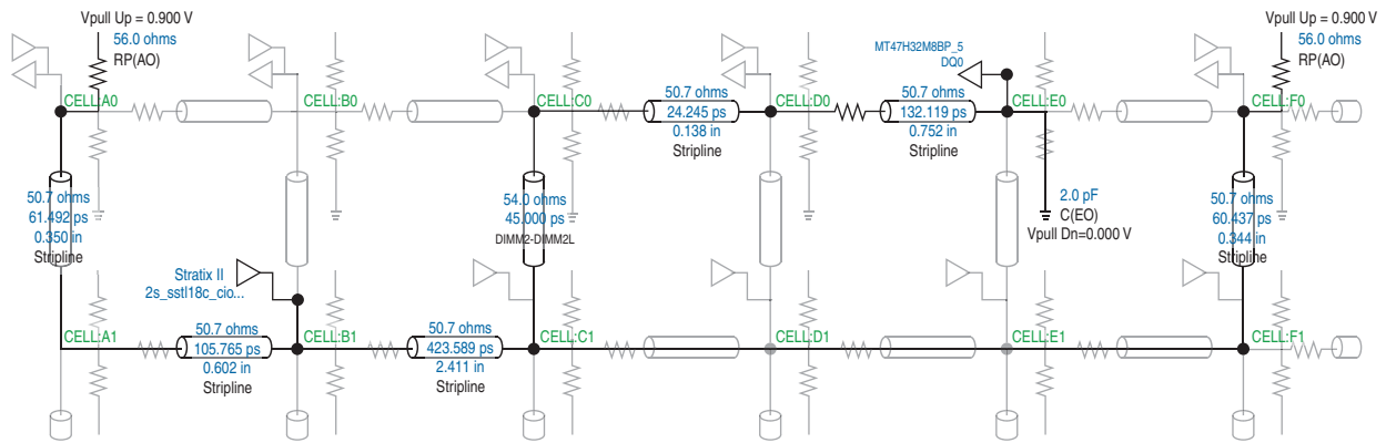
Figure 1-8. HyperLynx Setup for Stratix II Memory Board 2 with DDR2 SDRAM DIMM Interface Simulation
