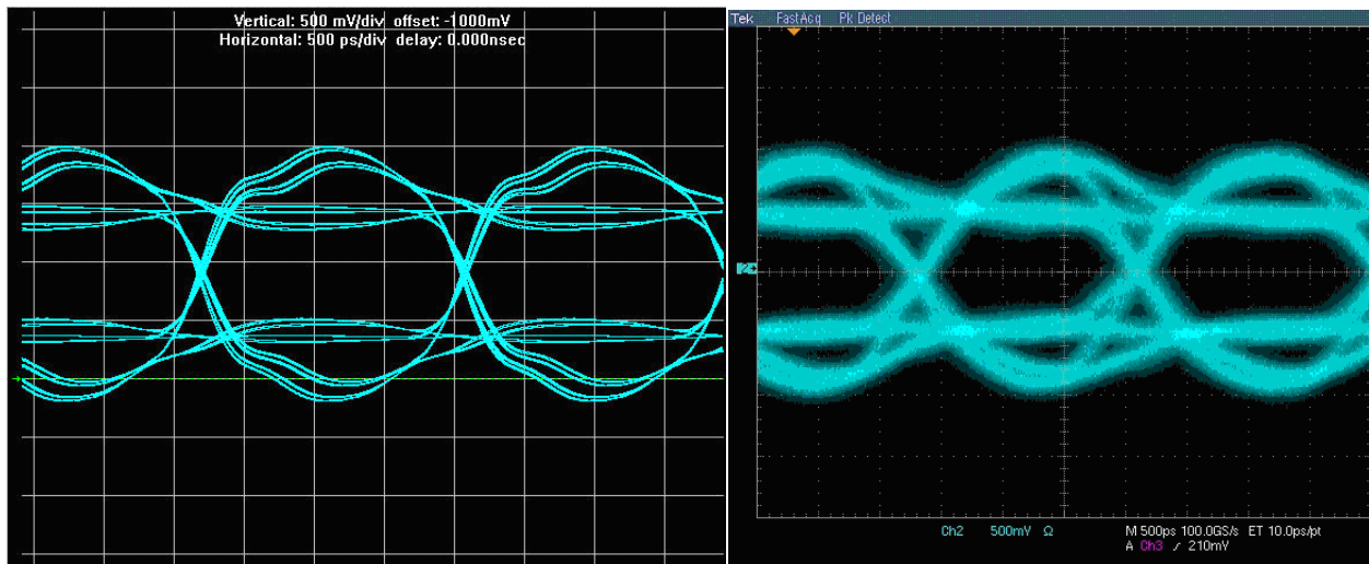
Figure 1-26. HyperLynx Simulation and Board Measurement, FPGA Reading from Memory
