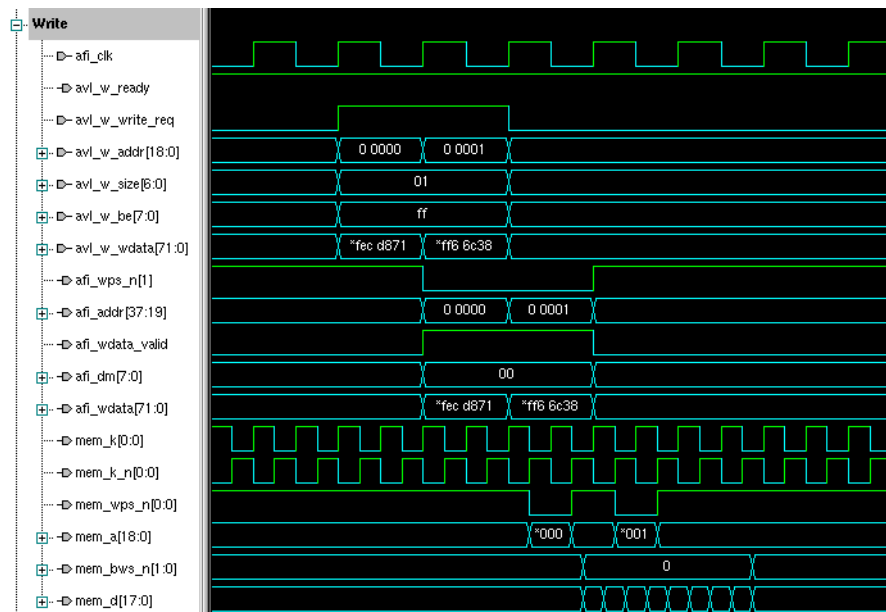
Figure 8–1. Back-to-Back Writes
