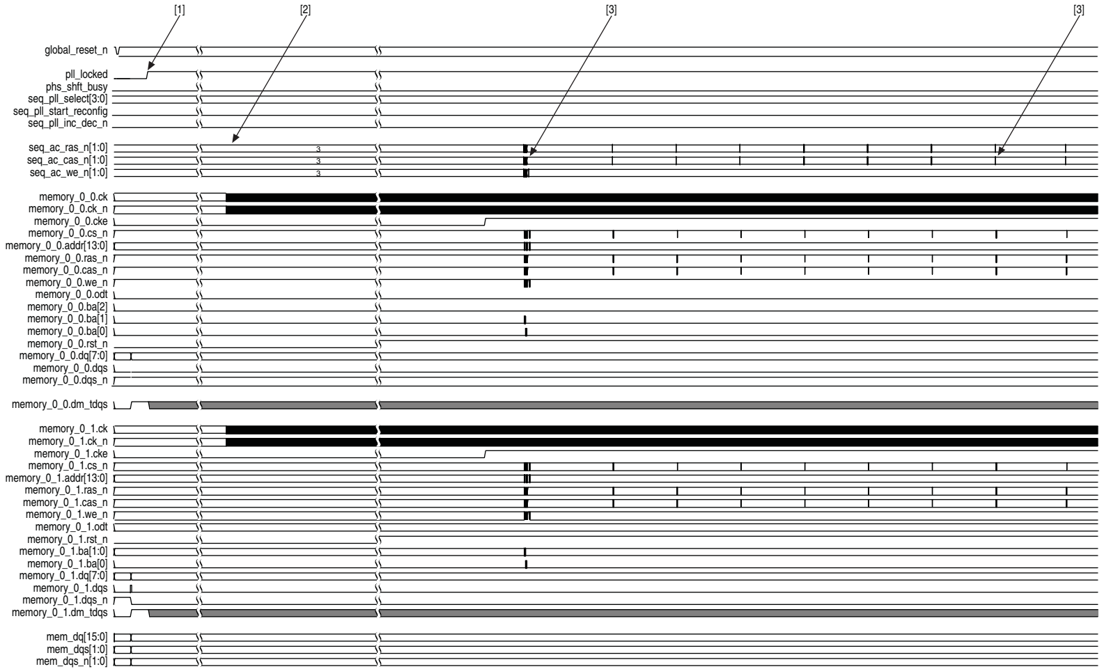
Figure 9-6. Initialization Timing for HPC
