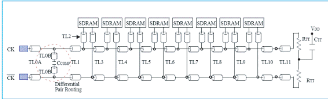
Figure 2-9. Clock Net Structure for a 64-Bit DDR3 SDRAM Unbuffered DIMM (Note 1)
