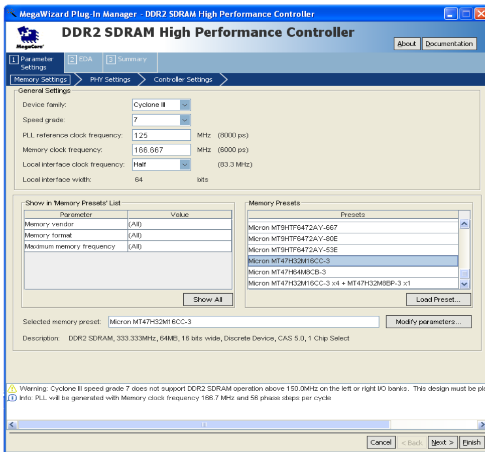
Figure 3-2. Configuring the DDR2 SDRAM Controller with ALTMEMPHY IP for the DDR2 Memory Interface
