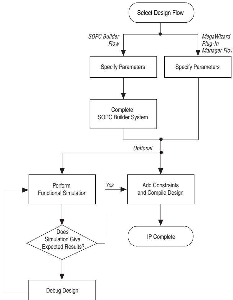
Figure 2-1. Design Flows
