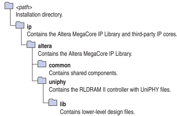
Figure 1-1. Directory Structure
