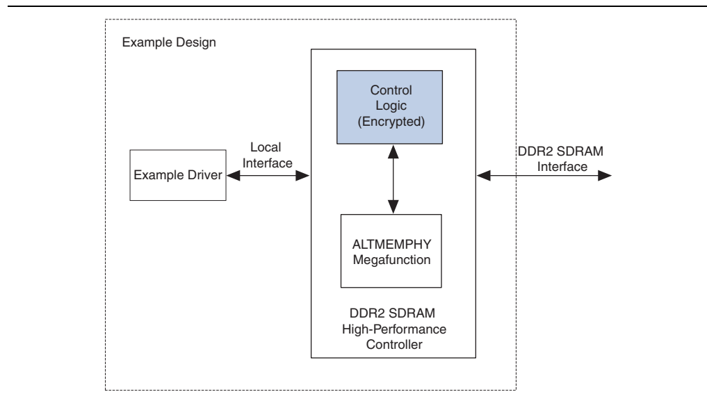
Figure 6-13. Design Example
