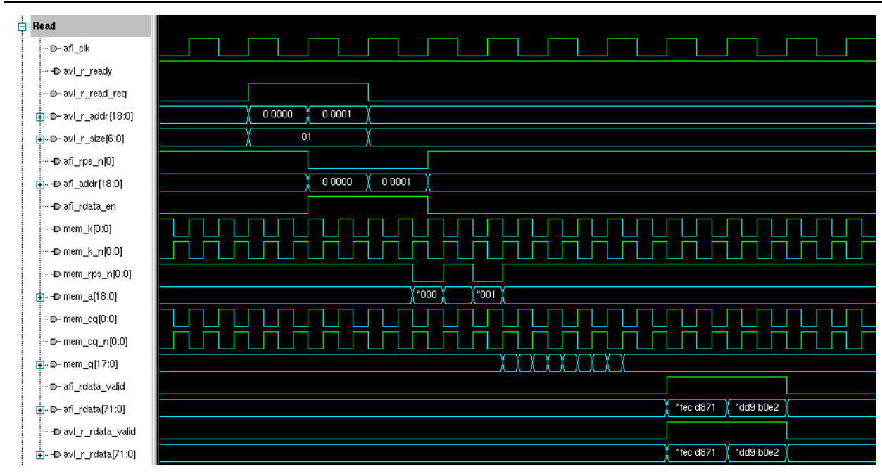
Figure 8-2. Back-to-Back Reads
