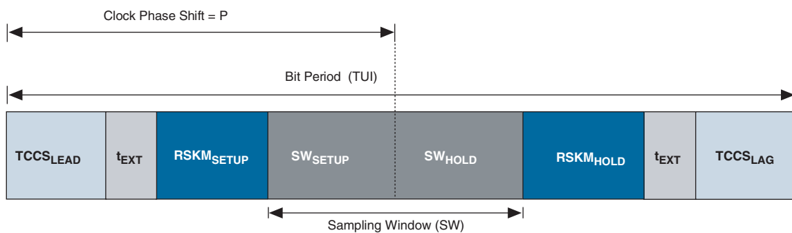
Figure 1-5. Sample Timing Budget with Unbalanced (TCCS and SW) Timing Parameters
