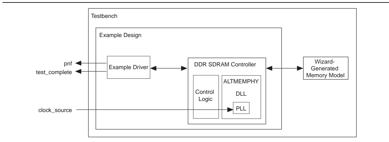
Figure 6-7. Testbench and Example Top-Level File
