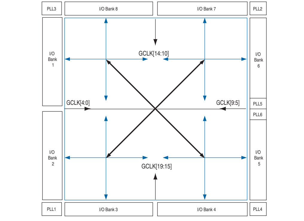
Figure 1-2. PLL Locations in Cyclone III and Cyclone IV E Devices
