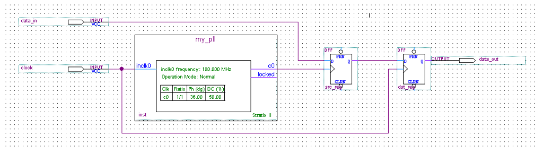
Figure 35. Register-To-Register Path
