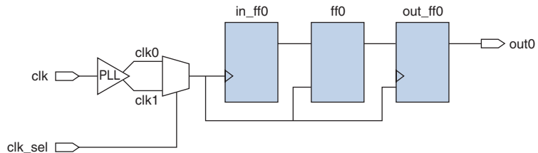
Figure 46. Clock Multiplexer Design
