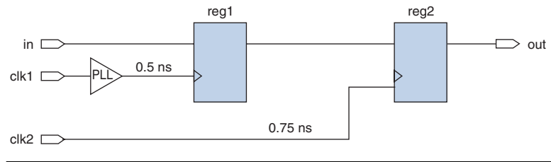
Figure 7. Register-to-Register Path with a PLL
