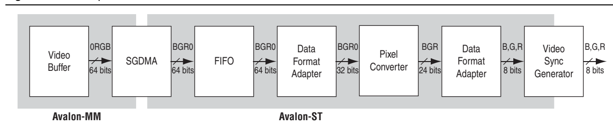
Figure 2. Video Pipeline
