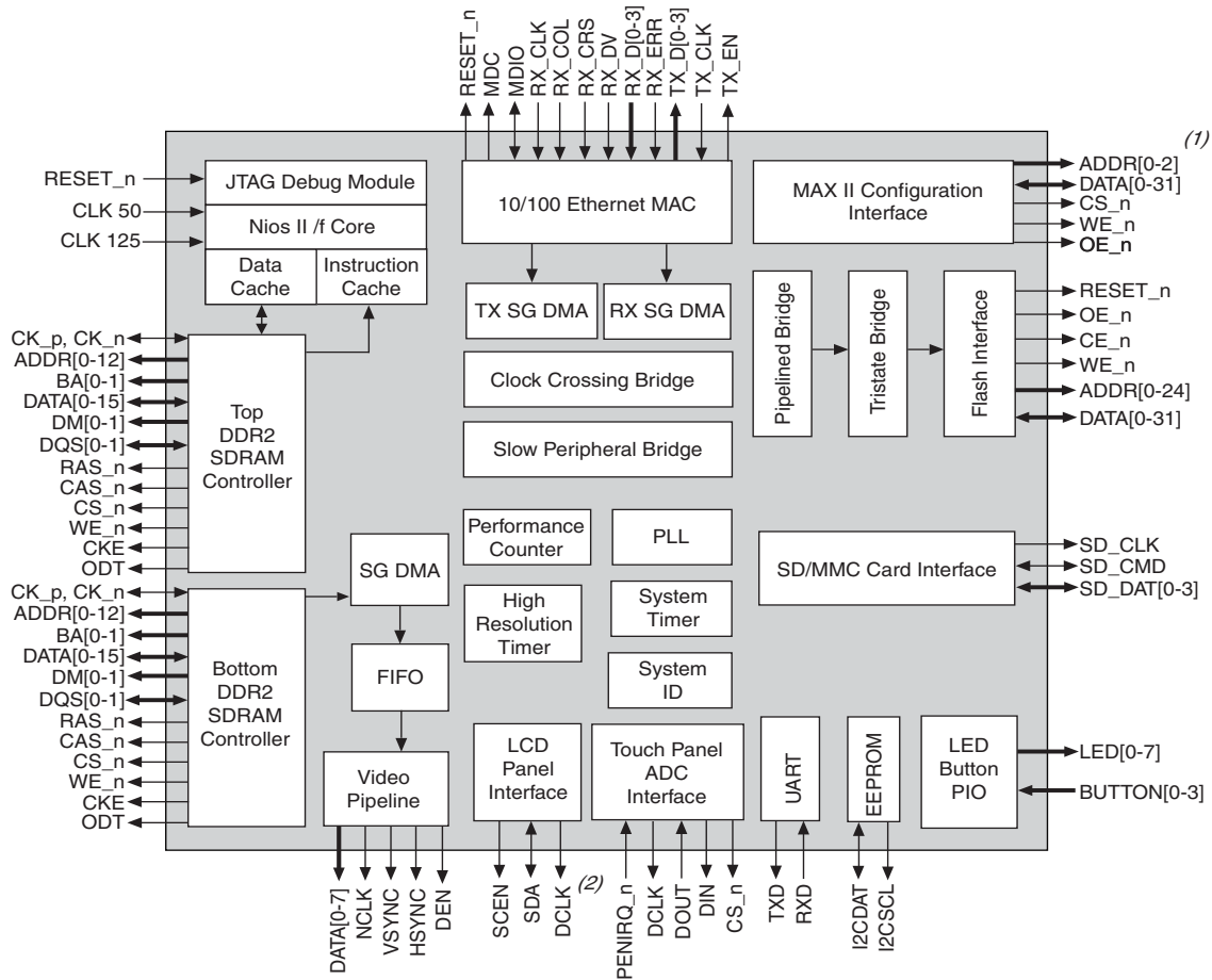
Figure 1. Block Diagram
