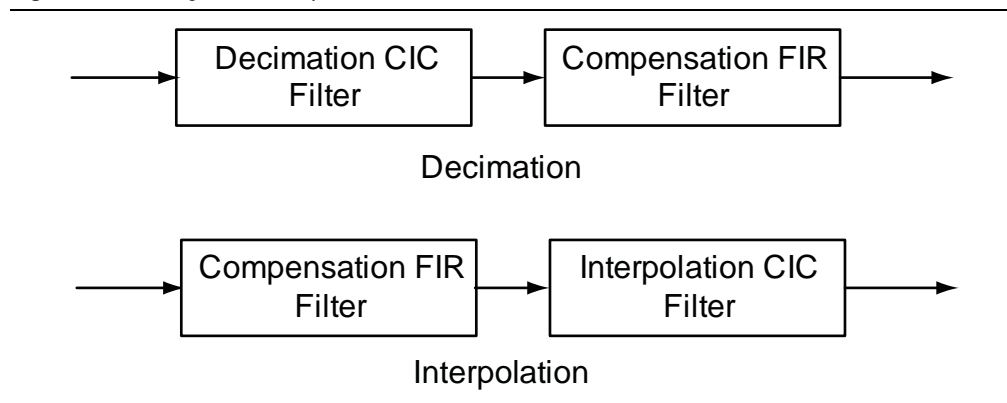
Figure 4-9. Using a CIC Compensation FIR Filter
