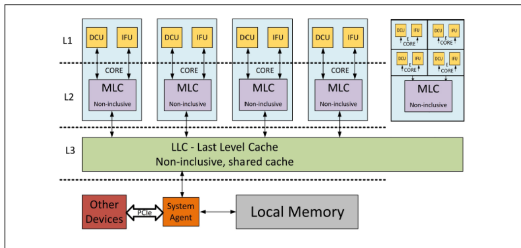
Figure 9. Hybrid Cache
