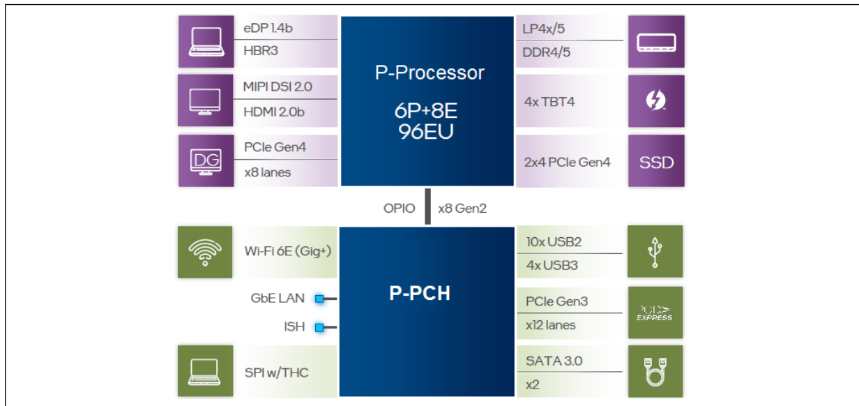
Figure 2. H/P Processor Line Platform Diagram
