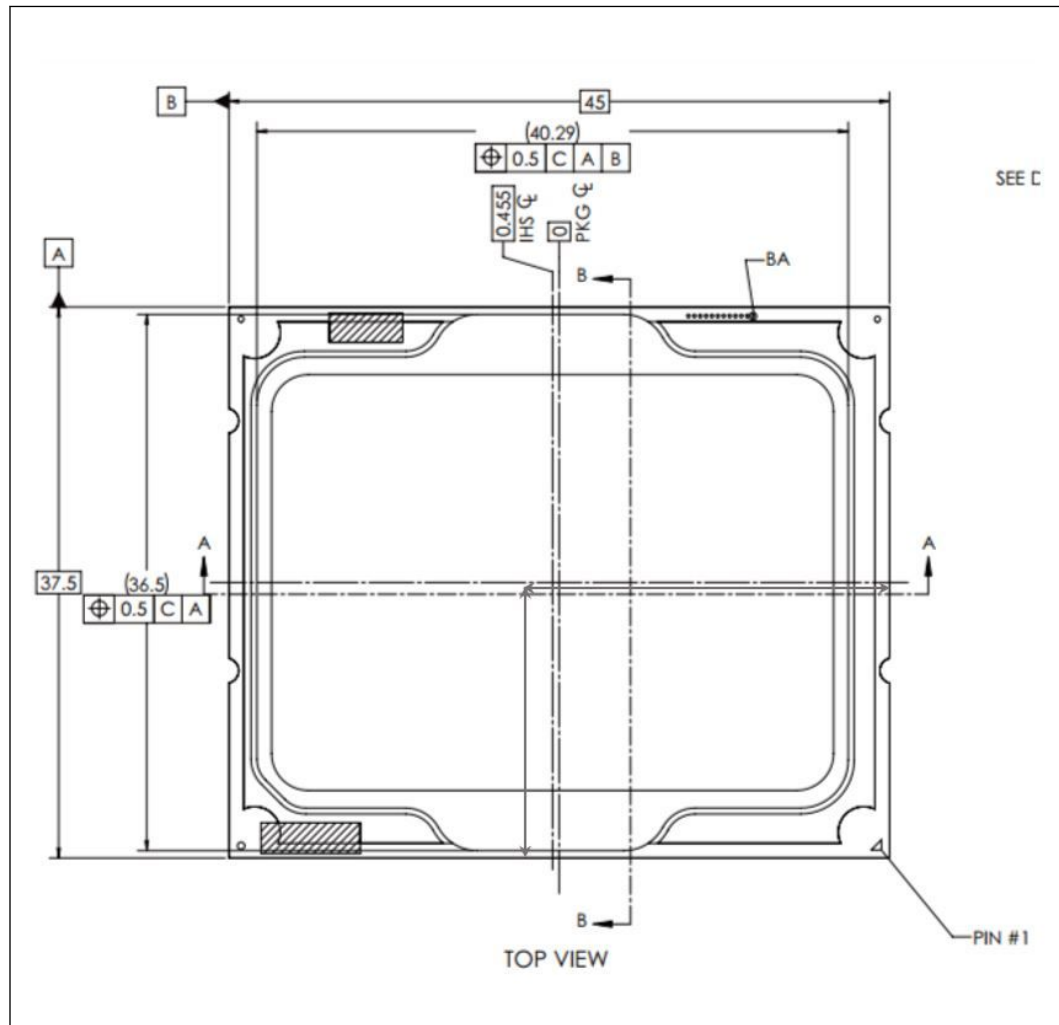
Figure 22. Thermal Test Vehicle (TTV) Case Temperature ( T_{CASE} ) Measurement Location
