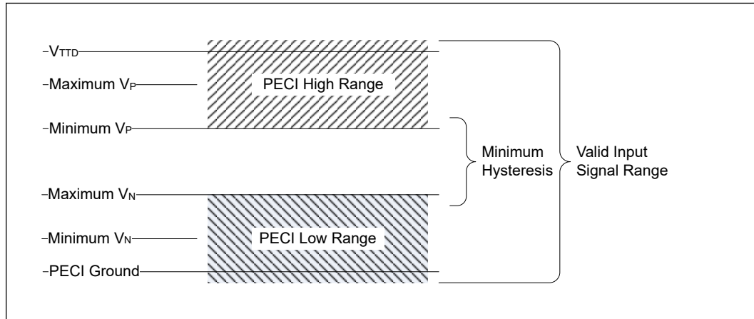
Figure 34. Input Device Hysteresis
