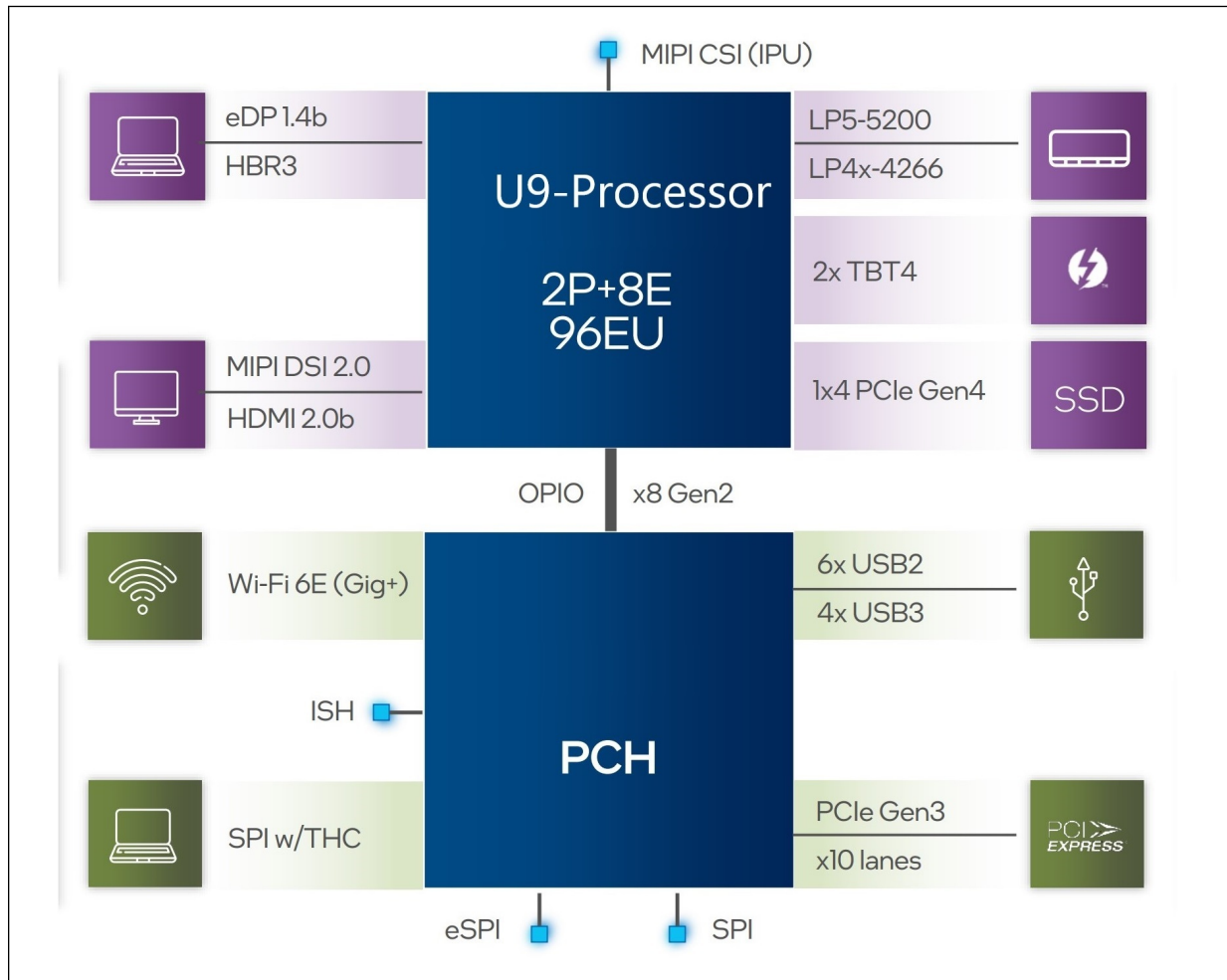
Figure 4. U9 Processor Line Platform Diagram
