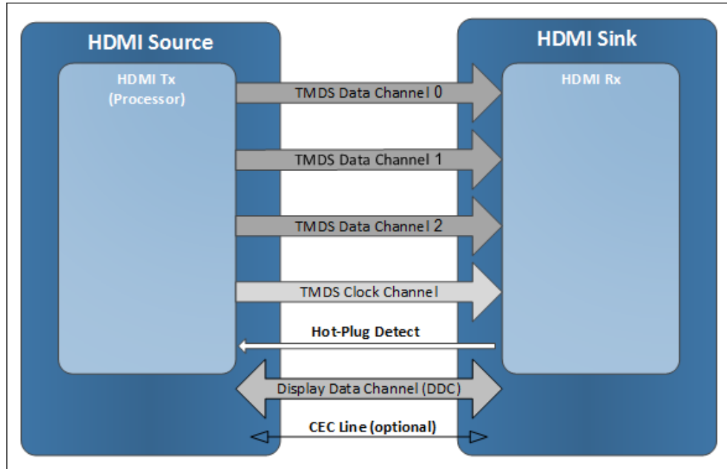
Figure 32. HDMI* Overview
