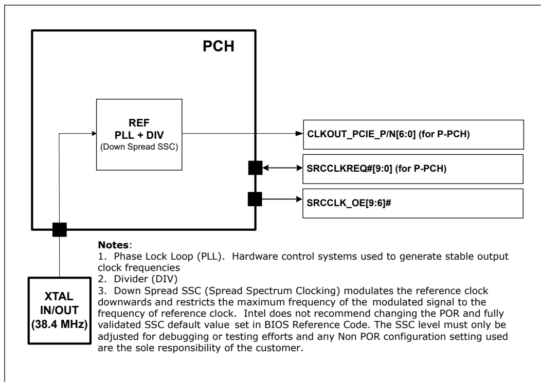
Figure 11. Integrated Clock Controller (ICC) Diagram
