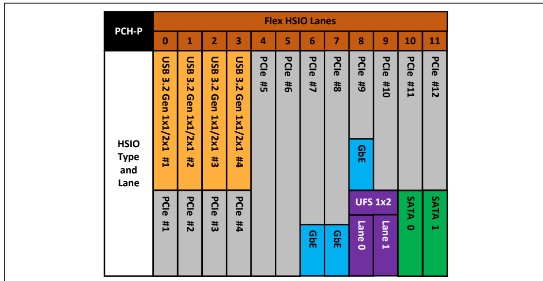
Figure 1. Flexible HSIO Lane Multiplexing in PCH-P
