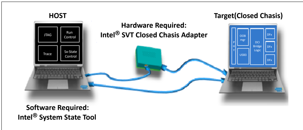
Figure 20. Platform Setup with Intel® Trace Hub
