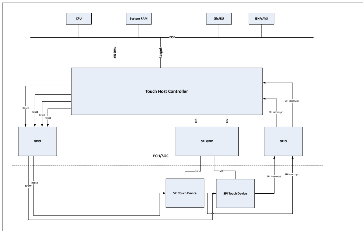
Figure 19. THC Block Diagram
