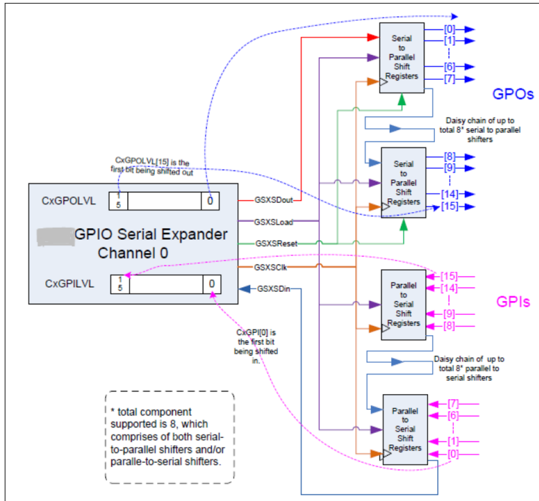
Figure 26. Example of GSX Topology
