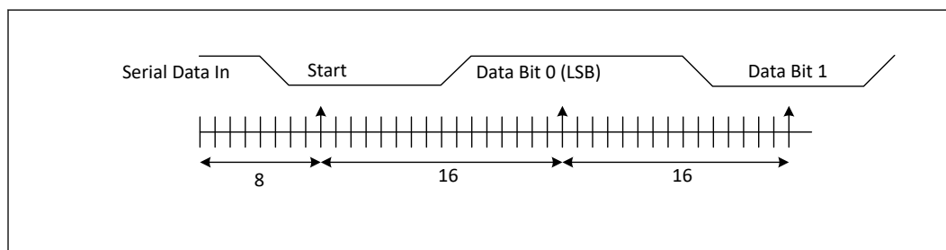
Figure 23. UART Receiver Serial Data Sample Points
