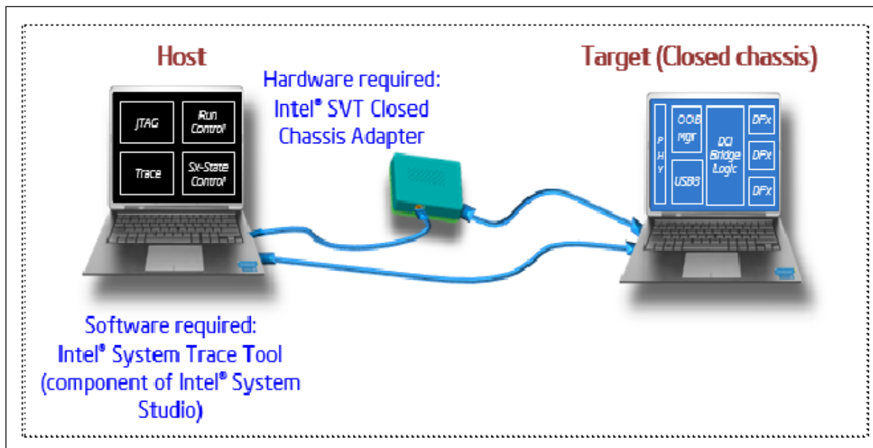
Figure 21. Platform Setup with DCI Connection
