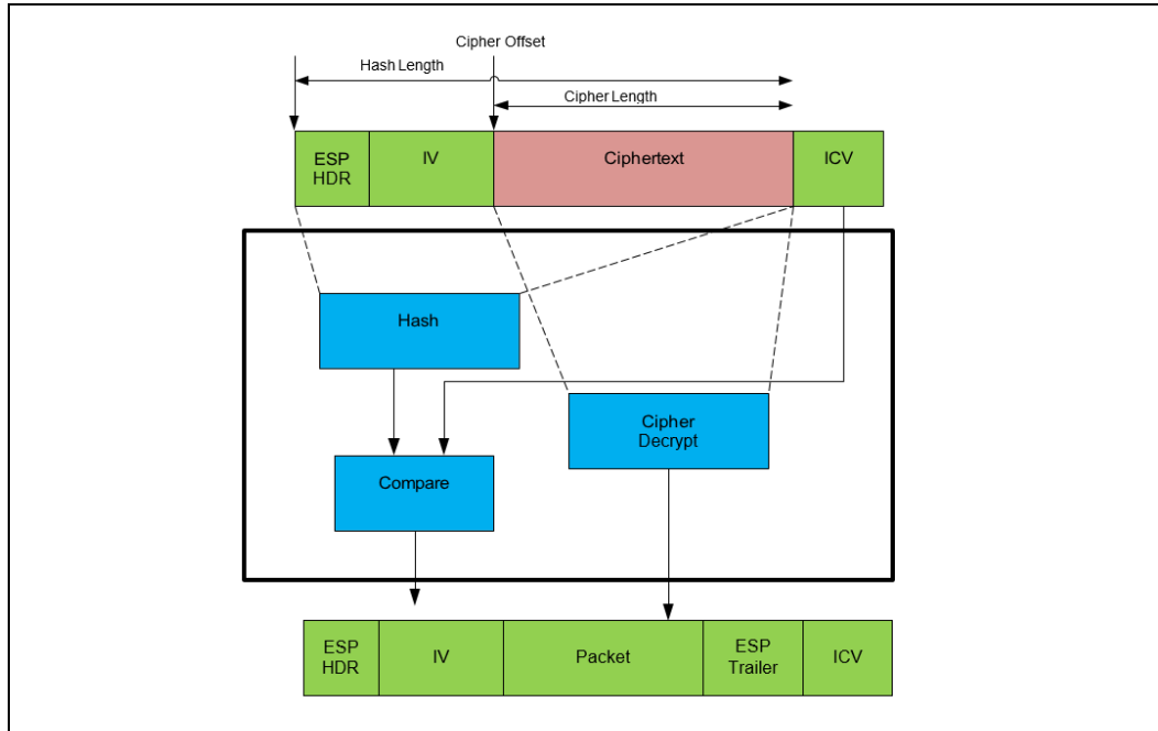
Figure 6. IPSec Inbound
