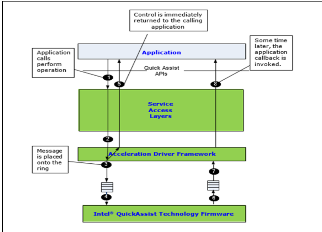
Figure 3. Asynchronous Operation
