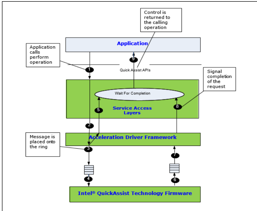
Figure 4. Synchronous Operation
