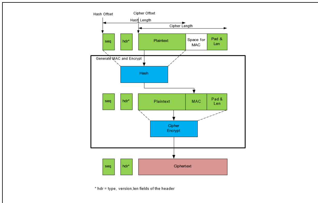
Figure 7. SSL Outbound
