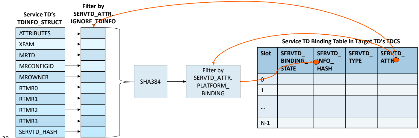
Figure 13.2: SERVTD_INFO_HASH Calculation
