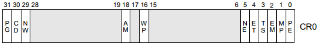
Figure 11.2: CR0
