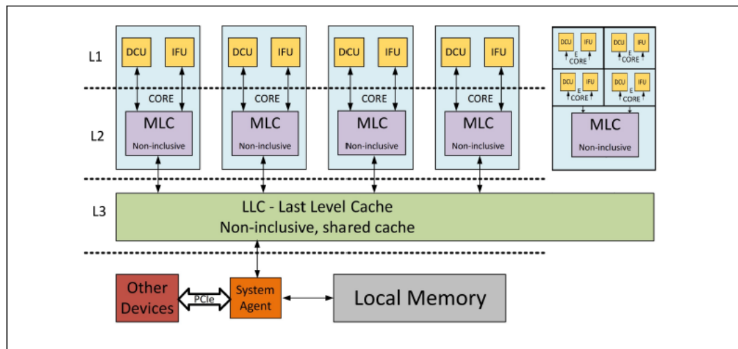
Figure 11. Hybrid Cache
