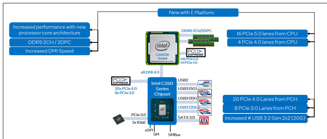
Figure 2. E/E Refresh Processor Line Platform Diagram
