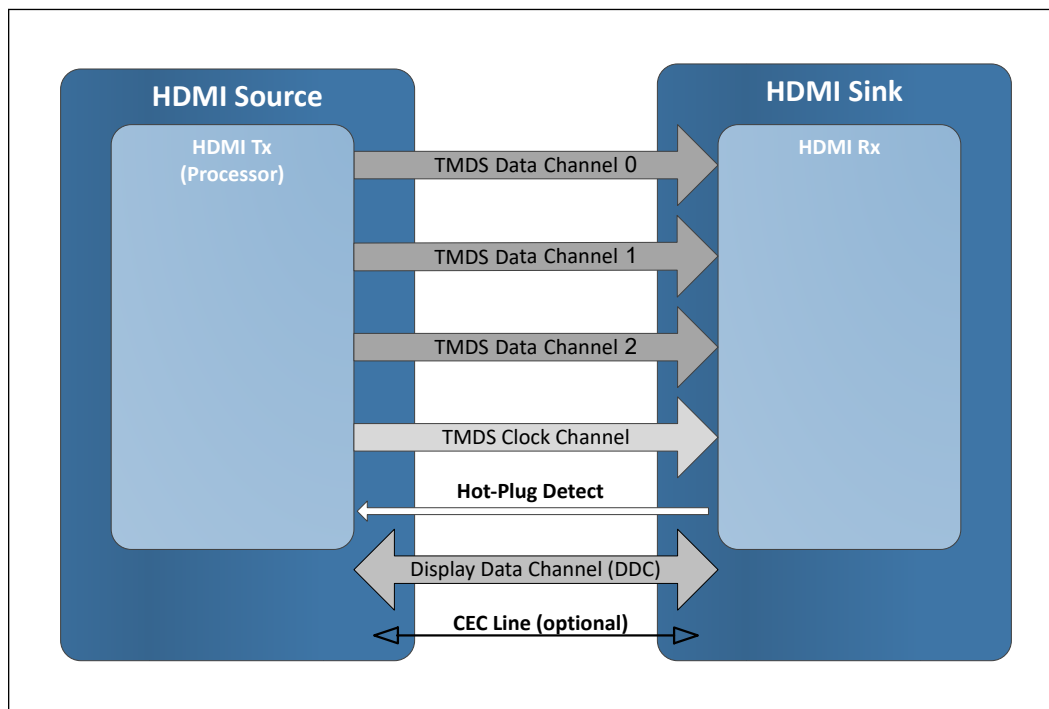
Figure 25. HDMI* Overview
