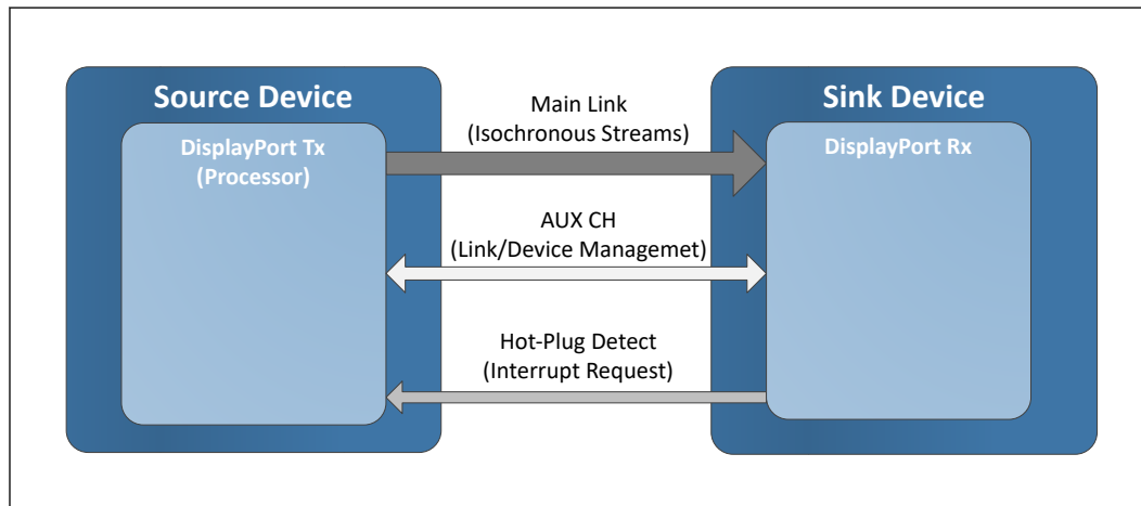
Figure 24. DisplayPort* Overview
