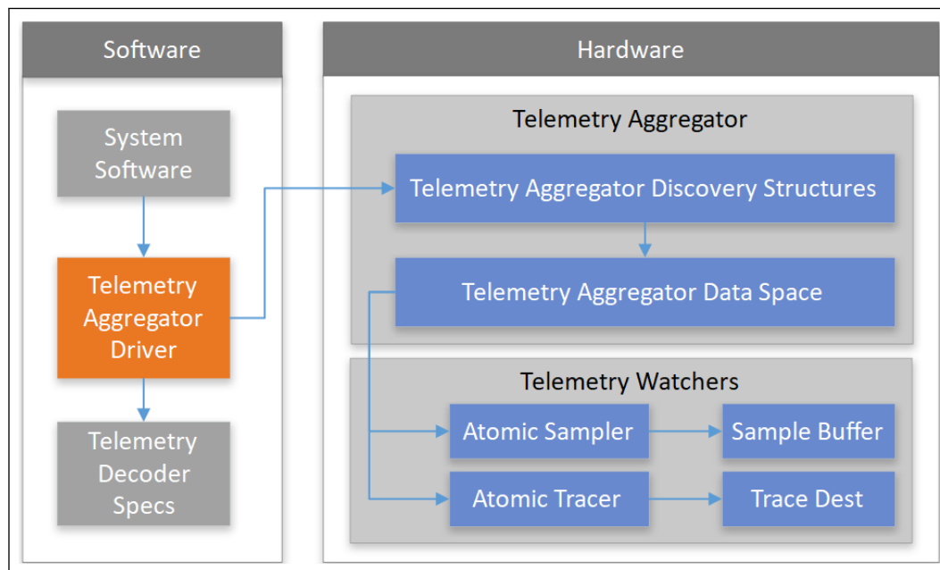
Figure 13. Telemetry Aggregator
