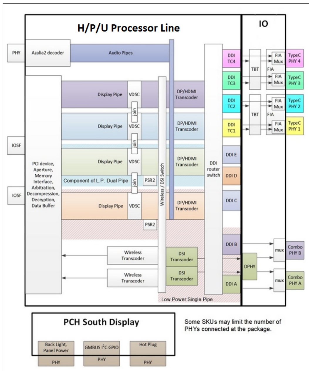
Figure 23. P, PX/U/U Refresh/H/H Refresh Processor Display Architecture
