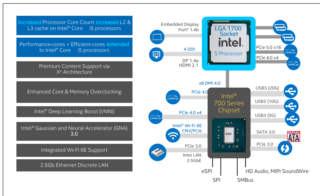
Figure 2. E/E Refresh Processor Line Platform Diagram
