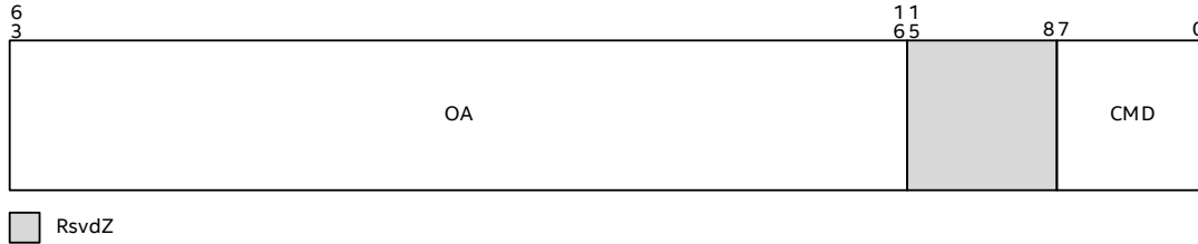
Figure 11-72. Virtual Command Register
