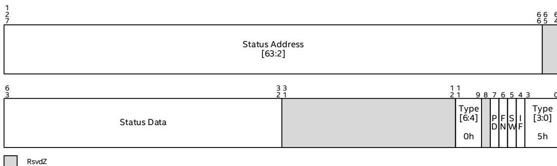
Figure 6-8. Invalidation Wait Descriptor (128-bit Version)
