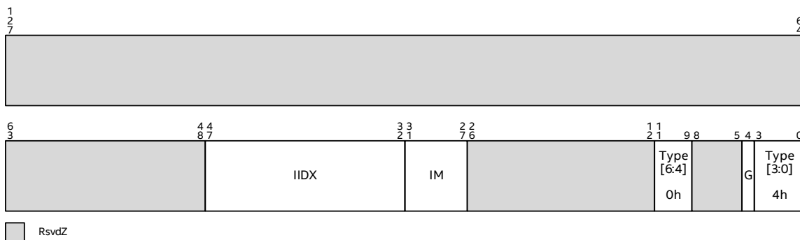
Figure 6-7. Interrupt Entry Cache Invalidate Descriptor (128-bit Version)
