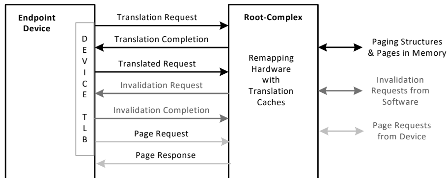
Figure 4-1. Device-TLB Operation
