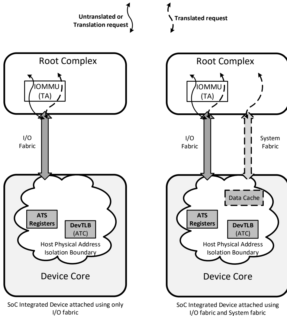
Figure 4-2. DevTLB in SoC Integrated Devices
