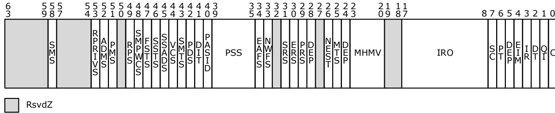
Figure 11-3. Extended Capability Register
