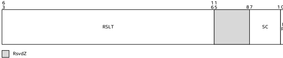
Figure 11-74. Virtual Command Response Register
