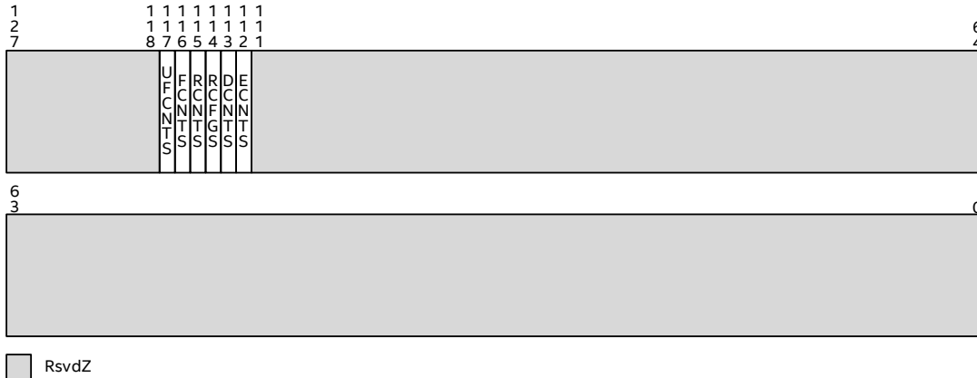
Figure 11-71. Enhanced Command Capability Register 1
