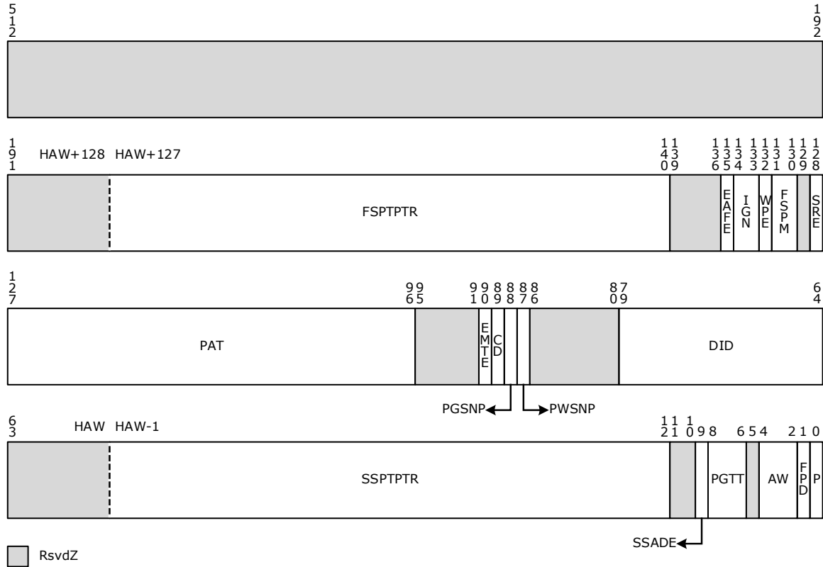
Figure 9-6. Scalable-Mode PASID Table Entry Format
