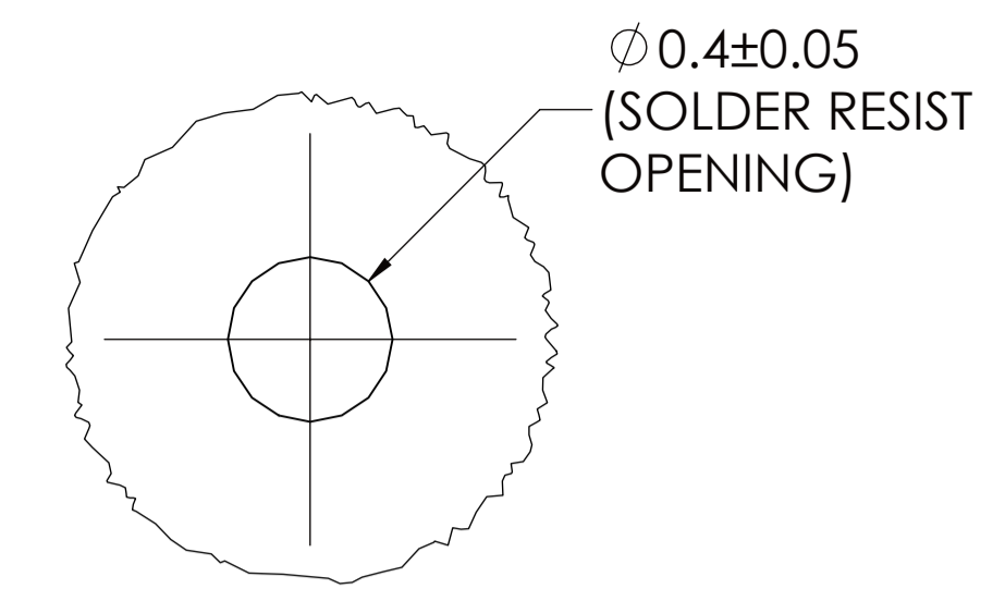
DETAIL C SCALE 50 : 1 SURFACE ALIGNMENT FIDUCIAL 2
