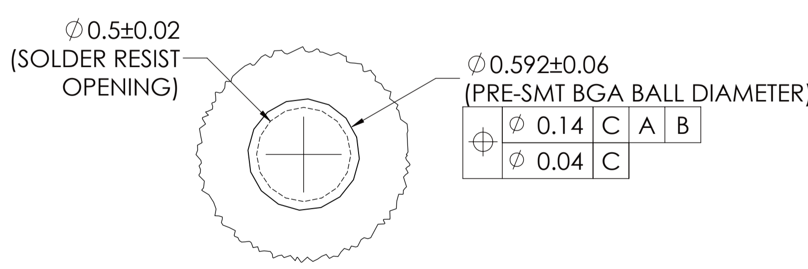
DETAIL D SCALE 50 : 1 3184X
