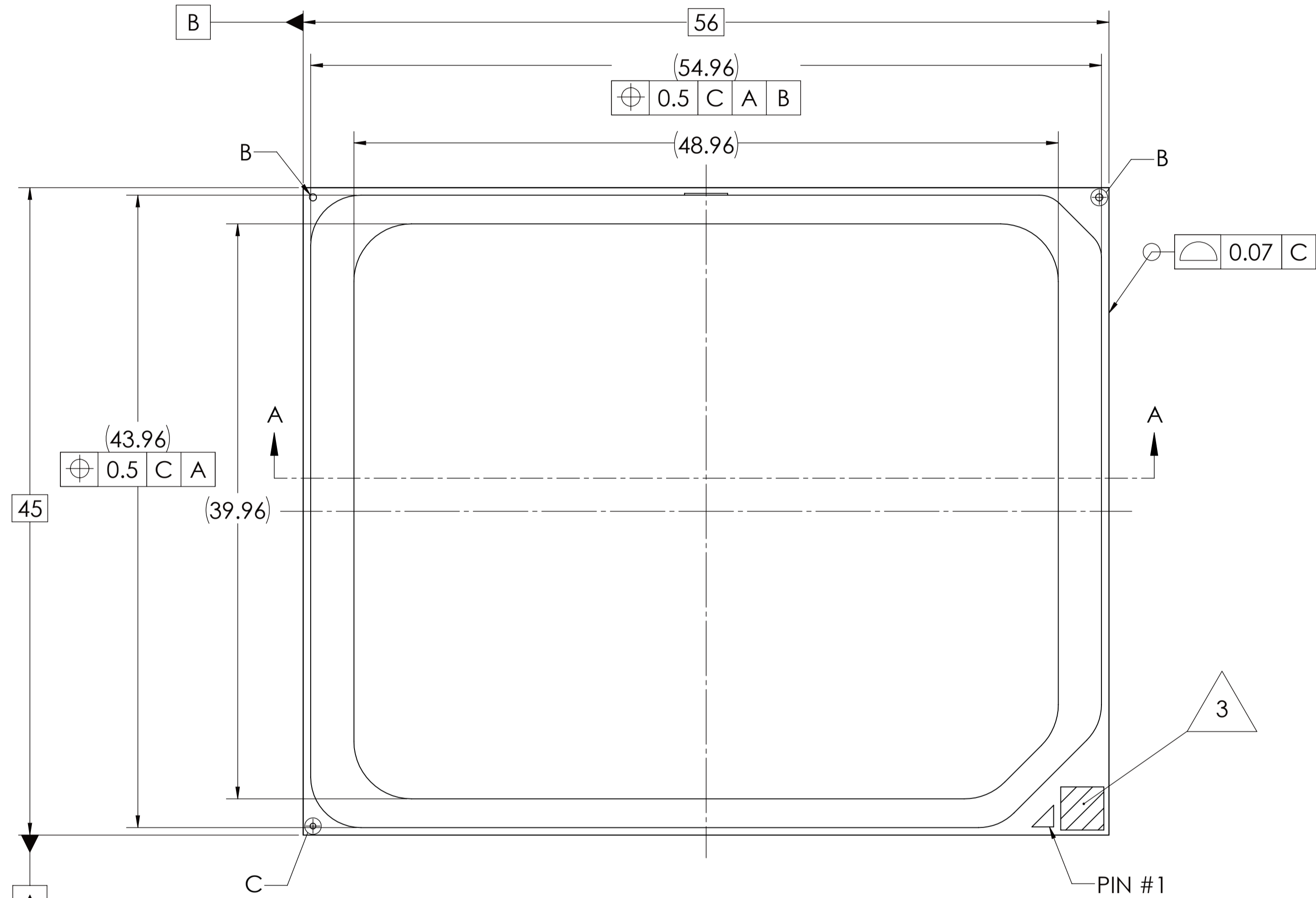
TOP VIEW
