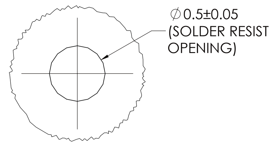
DETAIL B SCALE 50 : 1 SURFACE ALIGNMENT FIDUCIAL 1 2X
