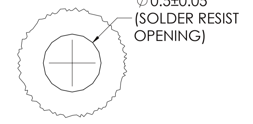
DETAIL E SCALE 50 : 1 LSC FIDUCIAL 2X
