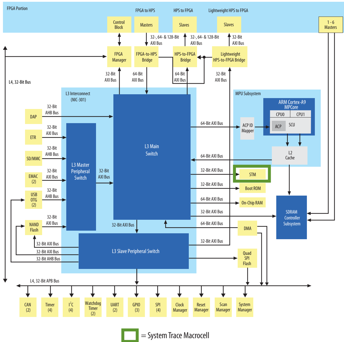
Figure 1: Altera Cyclone® V SoC Block Diagram With The System Trace Macrocell Highlighted
