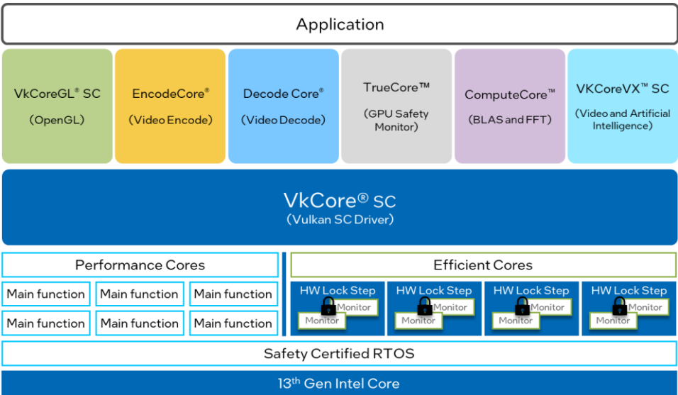
Figure 3: Native Software Architecture
