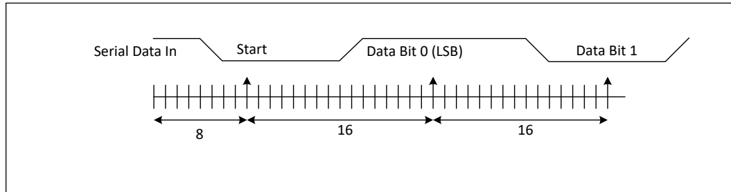
Figure 41. UART Receiver Serial Data Sample Points
