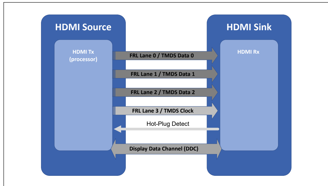
Figure 28. HDMI* Overview
