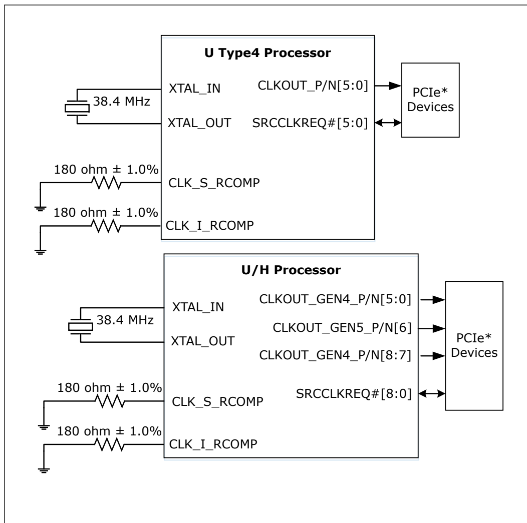
Figure 17. ICC Diagram
