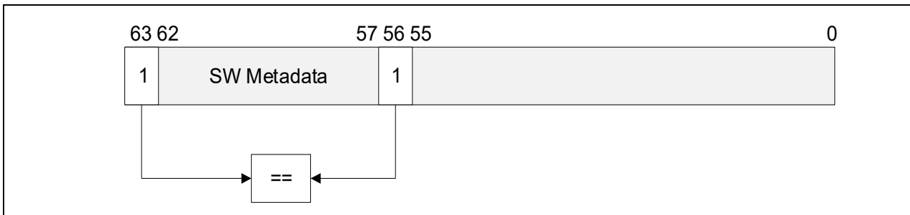
Figure 6-4. Canonicity Check When LAM57 is Enabled for Supervisor Pointers with 5-Level Paging
