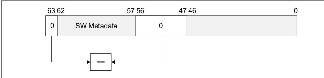
Figure 6-3. Canonicity Check When LAM57 is Enabled for User Pointers with 4-Level Paging
