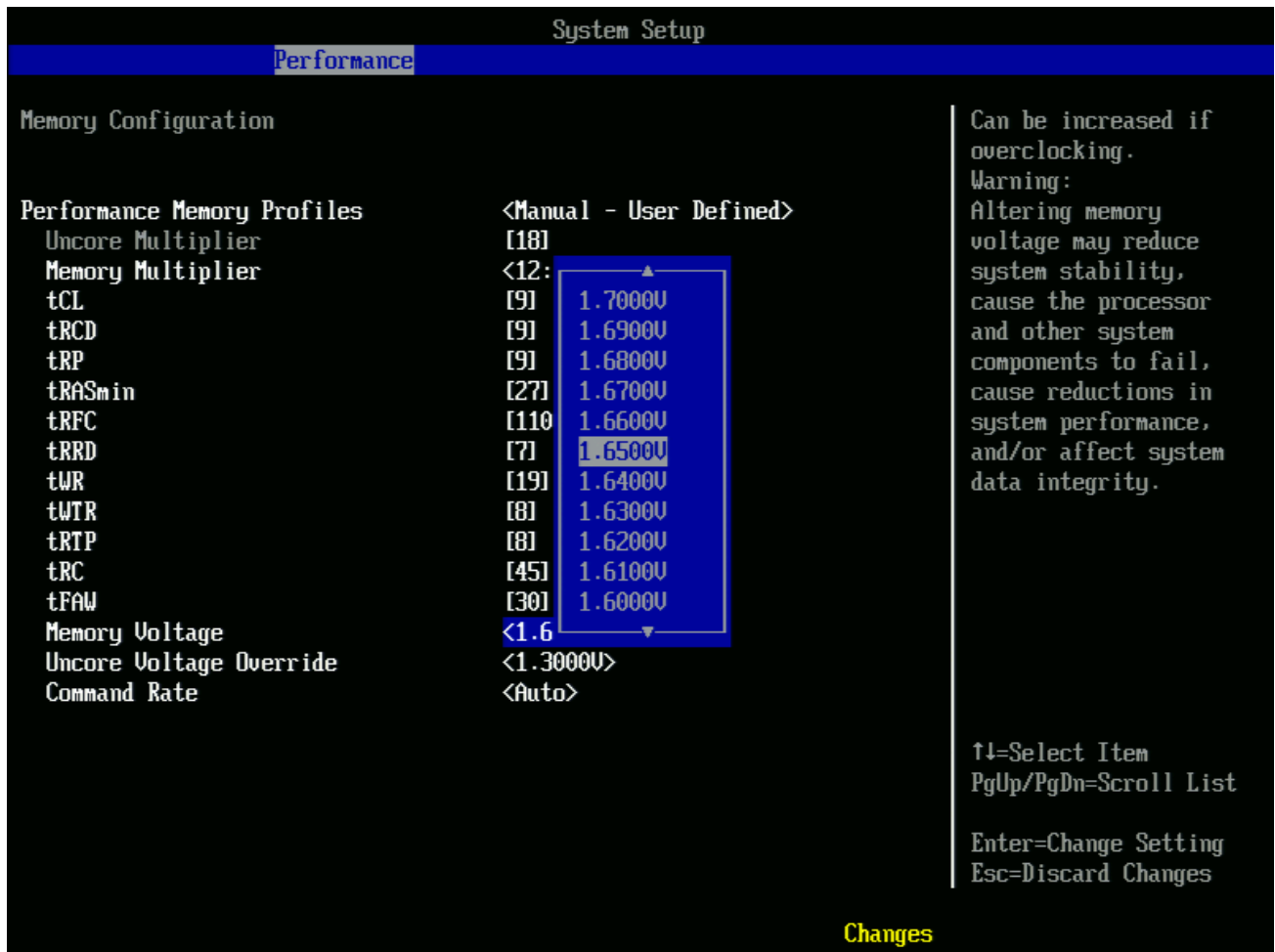
Figure 16. Memory Configuration with Uncore Voltage Adjusted in Manual Mode
