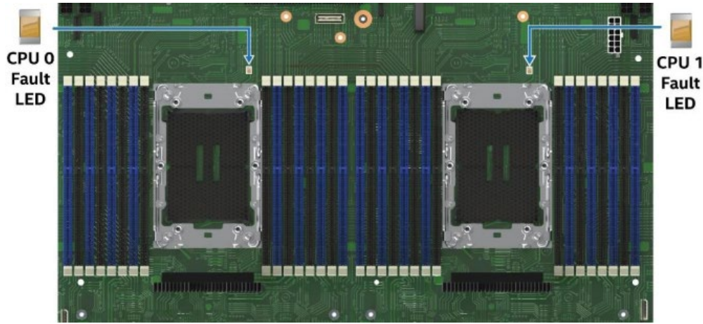
Figure 102. Processor Fault LEDs
