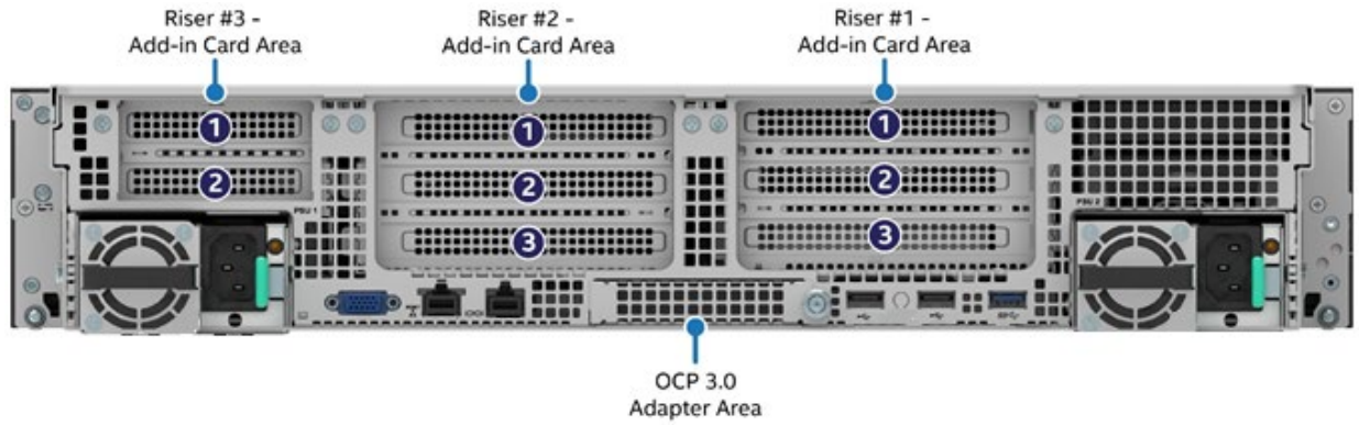
Figure 42. Server System Back Panel Add-In Card Areas
