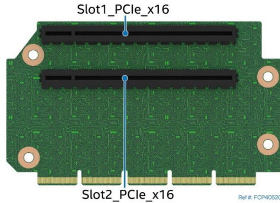
Figure 52. Two-slot PCIe* Riser Card for Riser Slot #2
