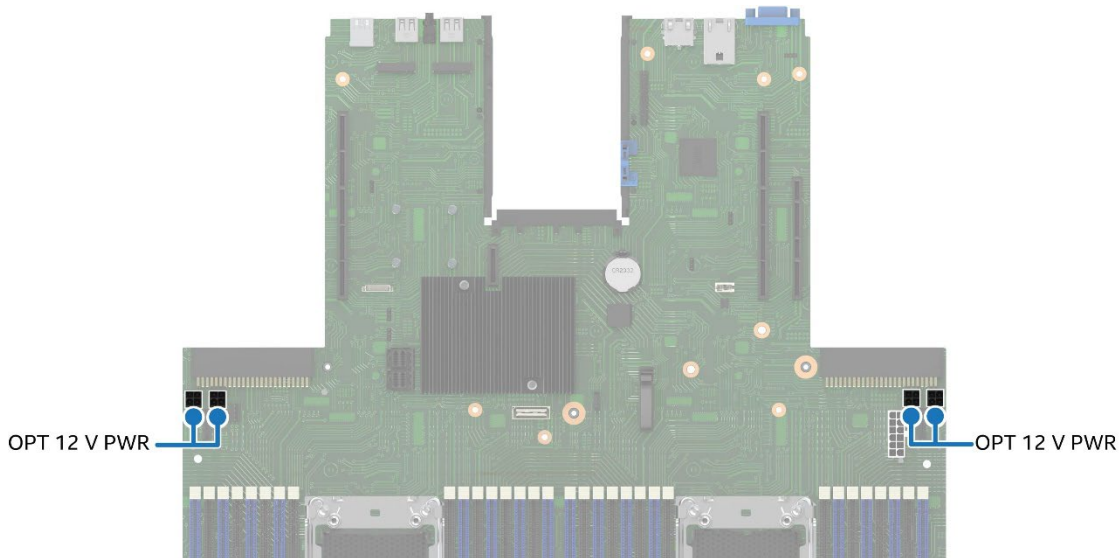
Figure 55. Auxiliary 12-Volt Power Connectors
