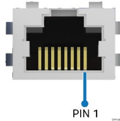
Figure 98. RJ45 Serial Port A Connector Pin Orientation
