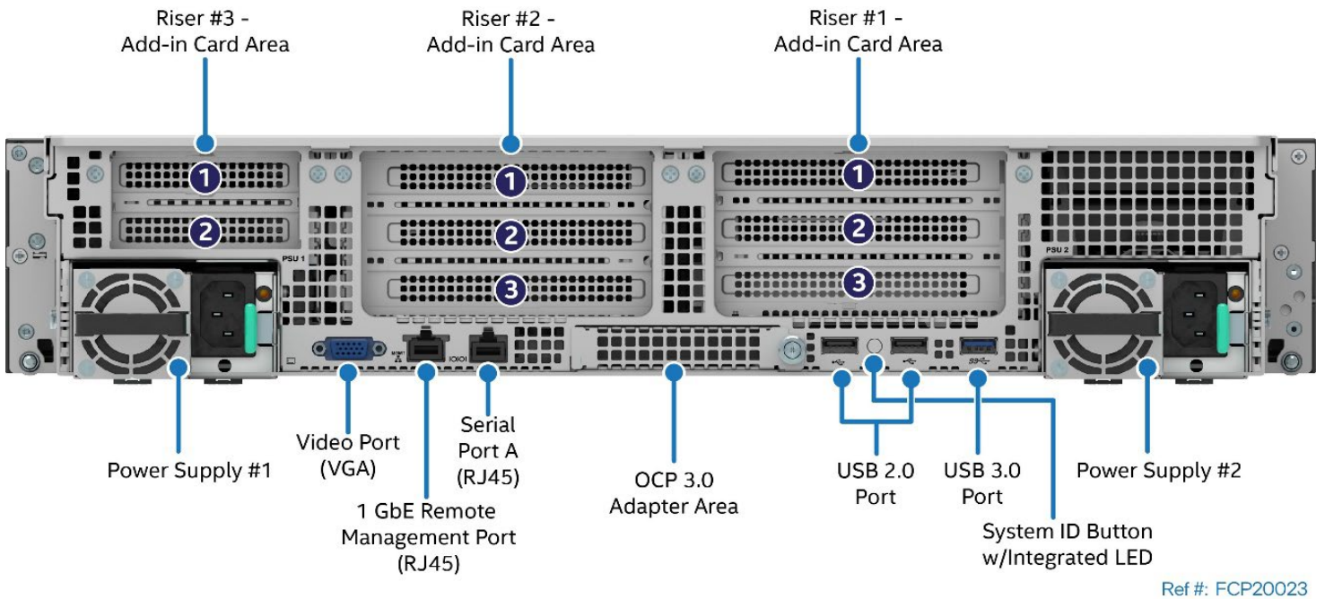
Figure 5. Back Panel Feature Identification
