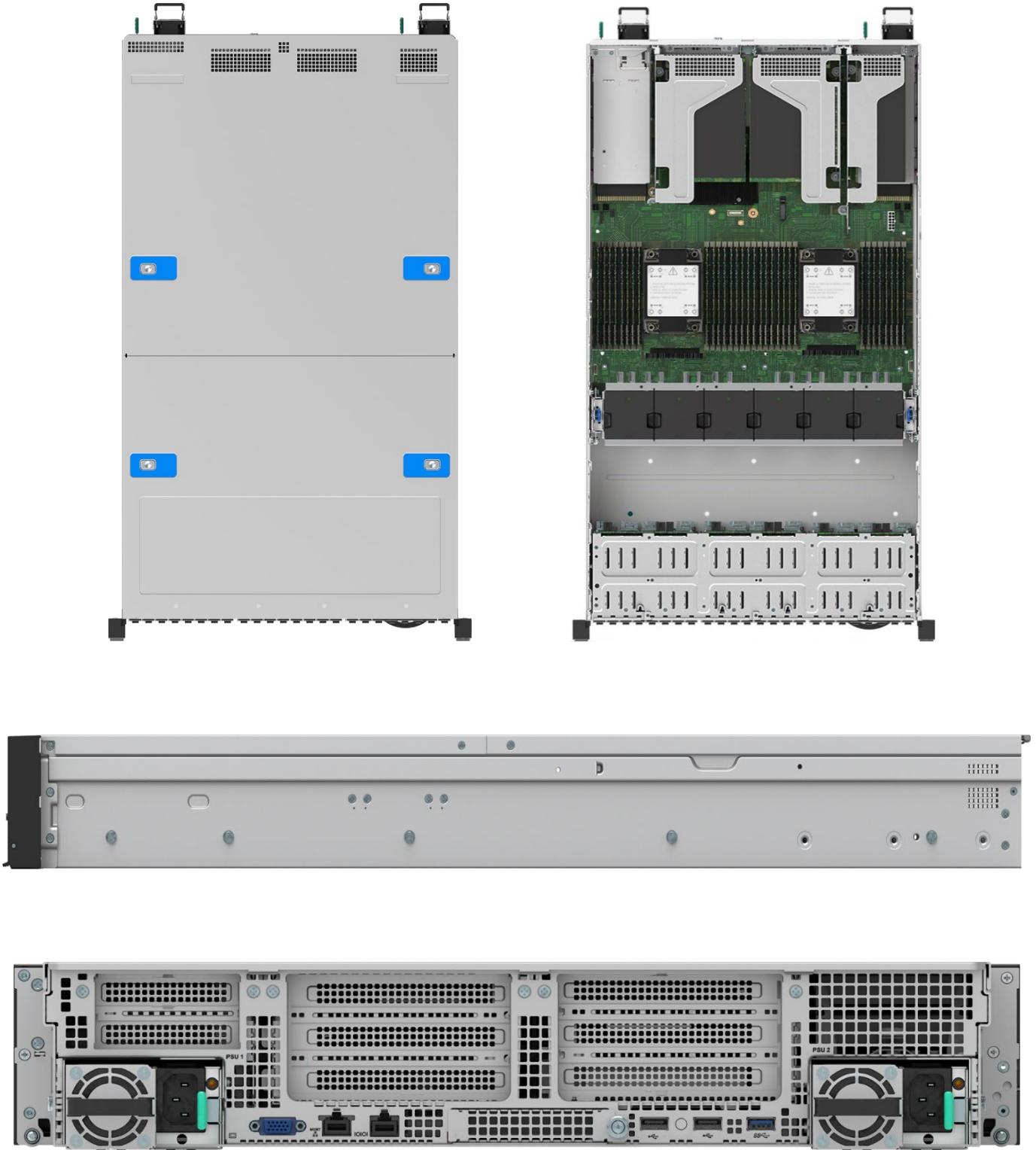
Figure 2. Intel® Server M50FCP2UR System Views (Top, Side, and Back)
