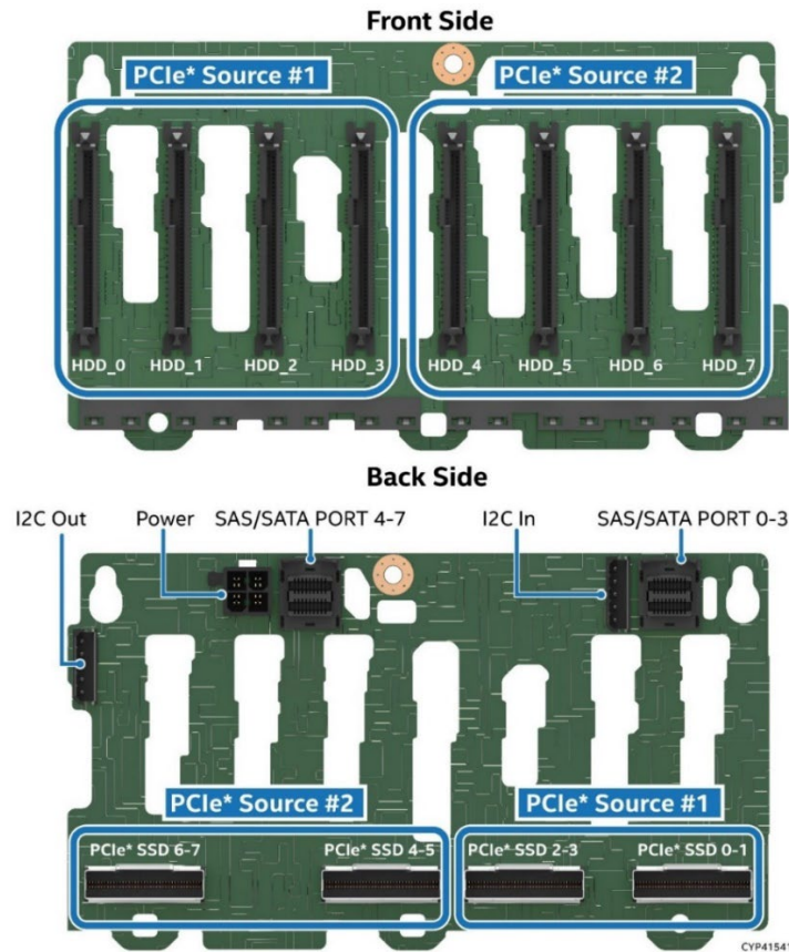
Figure 85. Backplane Cabling from Two Backplane Sources
