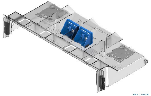
Air Duct option (iPN - FCPDUCTCMN) (1U processor heat sink configurations)
