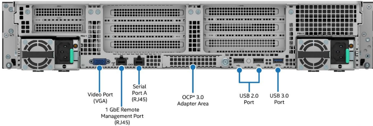
Figure 95. Rear I/O Features
