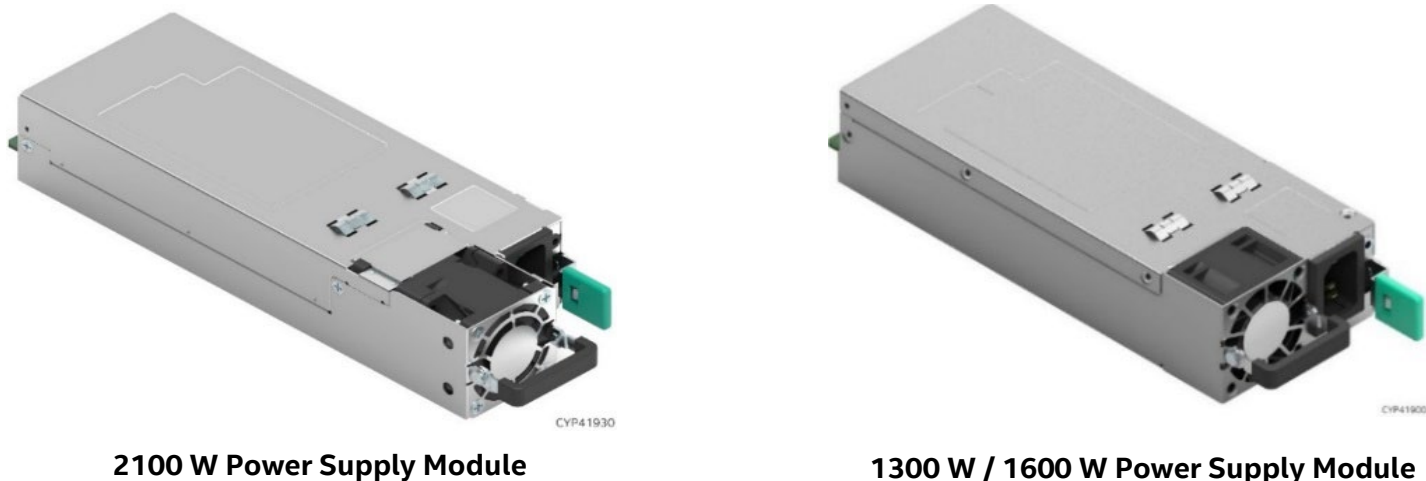
Figure 30. Power Supply Modules
