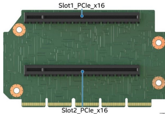
Figure 51. Two-slot PCIe* Riser Card for Riser Slot #2
