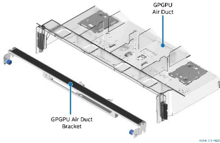
GPGPU Air Duct option (iPN - FCPGPGPUKit) (1U processor heat sink + GPGPU configurations)
