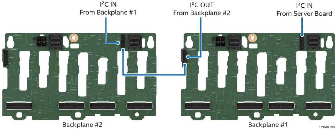
Figure 75. Connecting Two x8 Backplanes
