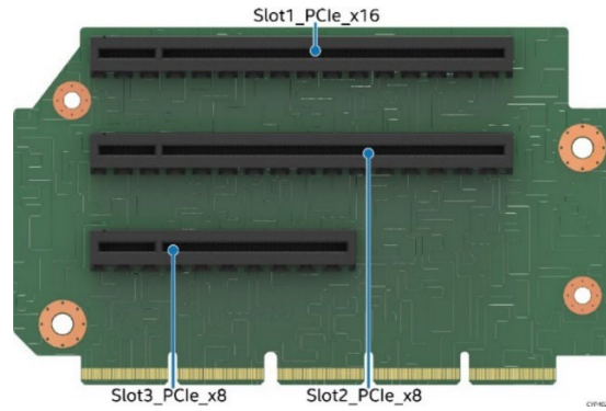
Figure 50. Three-slot PCIe* Riser Card for Riser Slot #2
