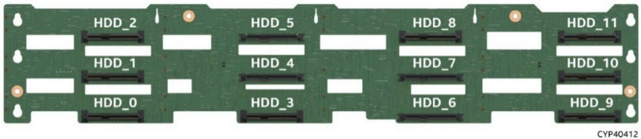
Figure 78. 12 x 3.5" HSBP Connector Identification – Front Side
