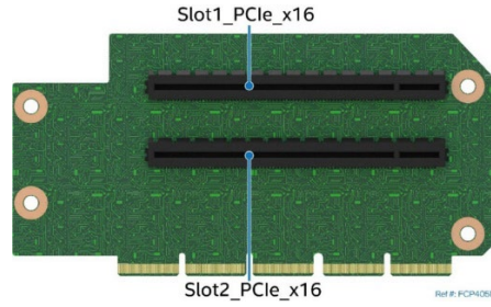
Figure 48. Two-Slot PCIe* Riser Card for Riser Slot #1
