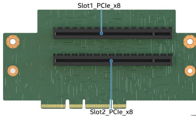
Figure 53. Two-slot PCIe* Riser Card for Riser Slot #3
