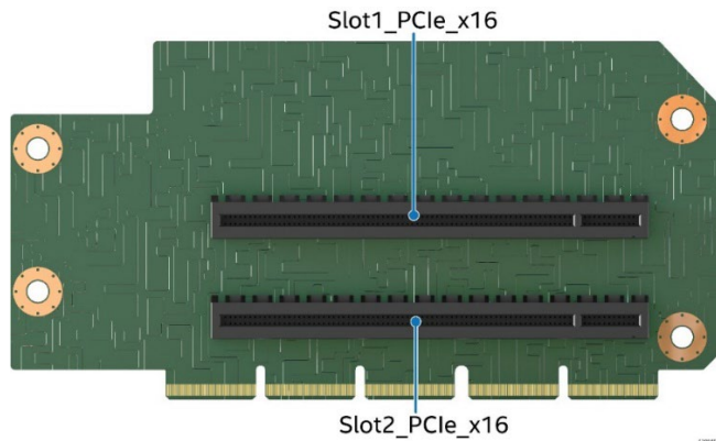
Figure 47. Two-Slot PCIe* Riser Card for Riser Slot #1
