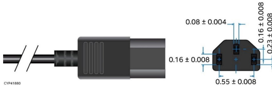
Figure 32. AC Power Cord Specification
