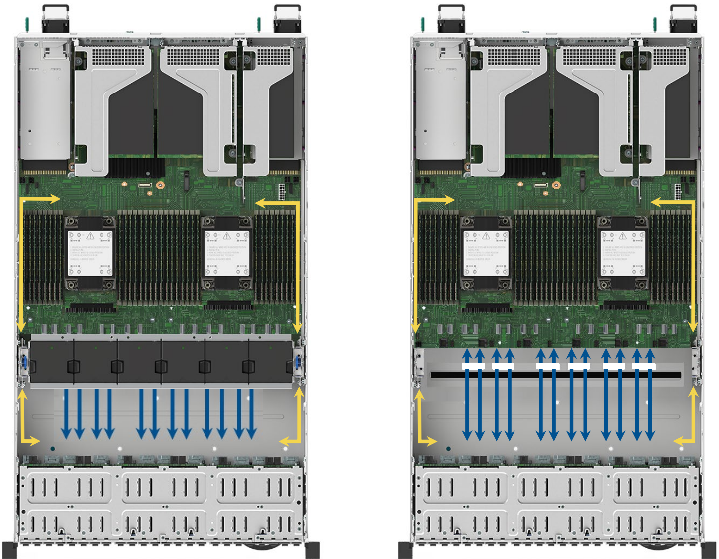
Figure 26. System Cable Routing Channels
