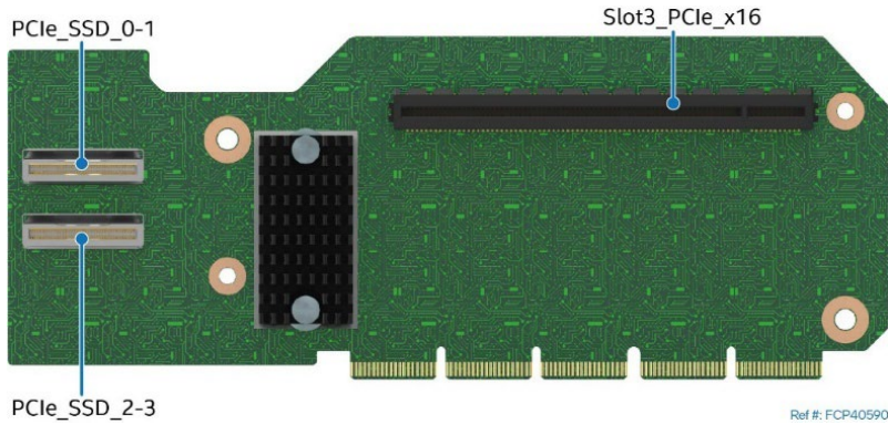
Figure 82. PCIe* NVMe* Riser Card for Riser Slot #1
