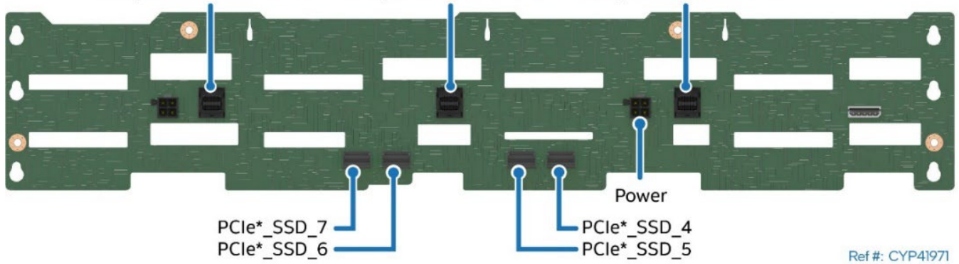
Figure 79. 12 x 3.5" HSBP Connector Identification – Back Side
