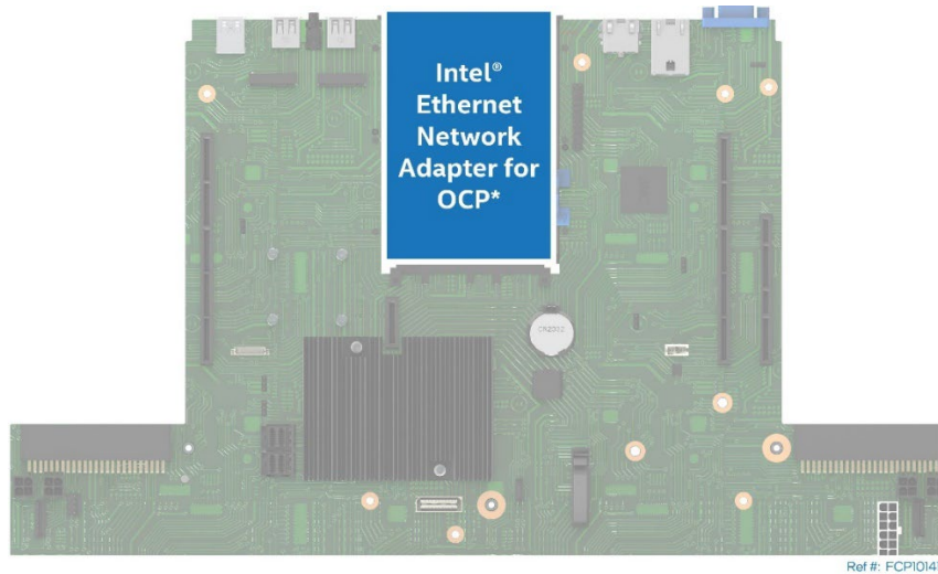
Figure 56. Intel® Ethernet Network Adapter for OCP* Placement
