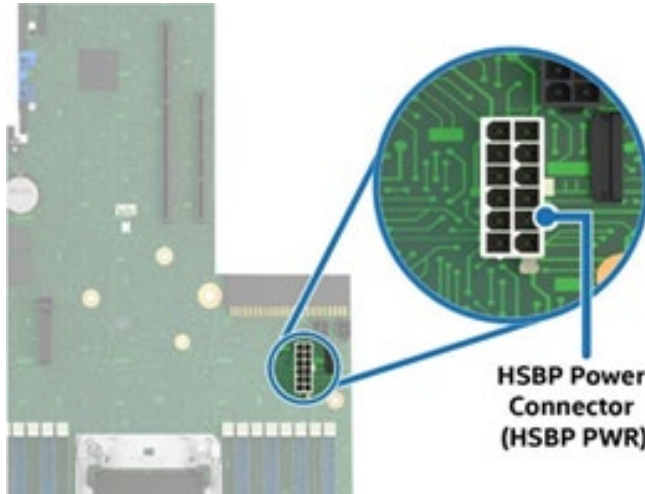
Figure 68. Server Board HSBP Power Connector
