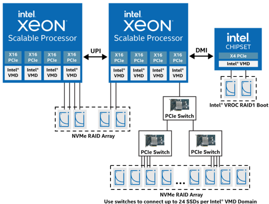
Figure 84. Supported NVMe* Configurations – Windows* and Linux*
