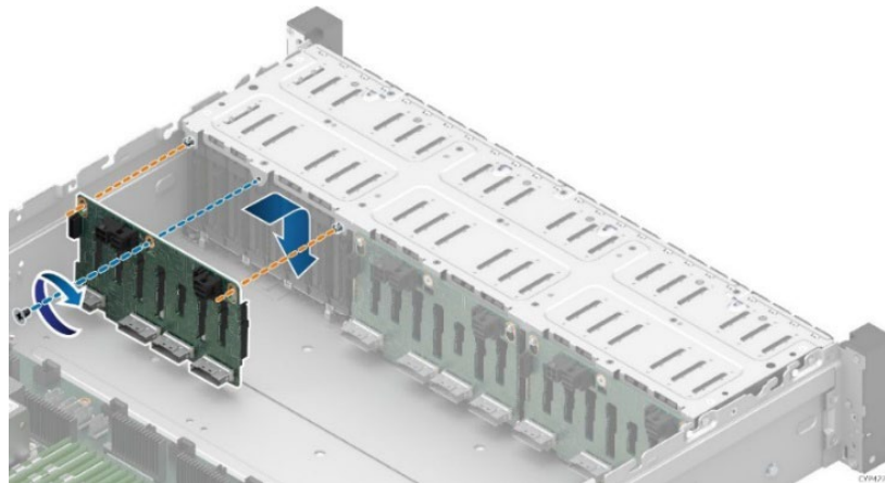
Figure 69. 2.5" Backplane Placement
