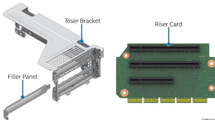
Figure 44. Riser Card Assembly Components
