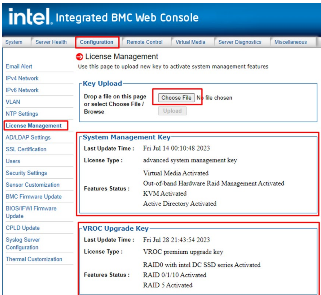
Figure 109. Integrated BMC Web Console Advanced System Management Key Page
