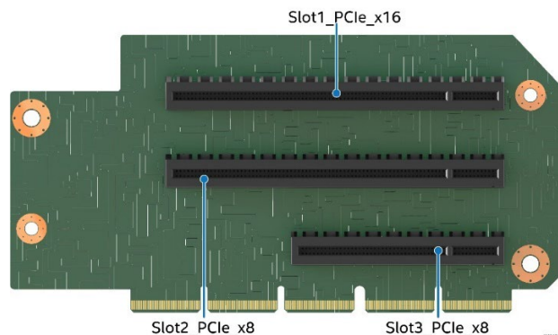
Figure 46. 3-Slot PCIe* Riser Card for Riser Slot #1
