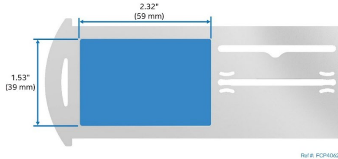
Figure 22. Pull-Out Tab Label Emboss Dimensions
