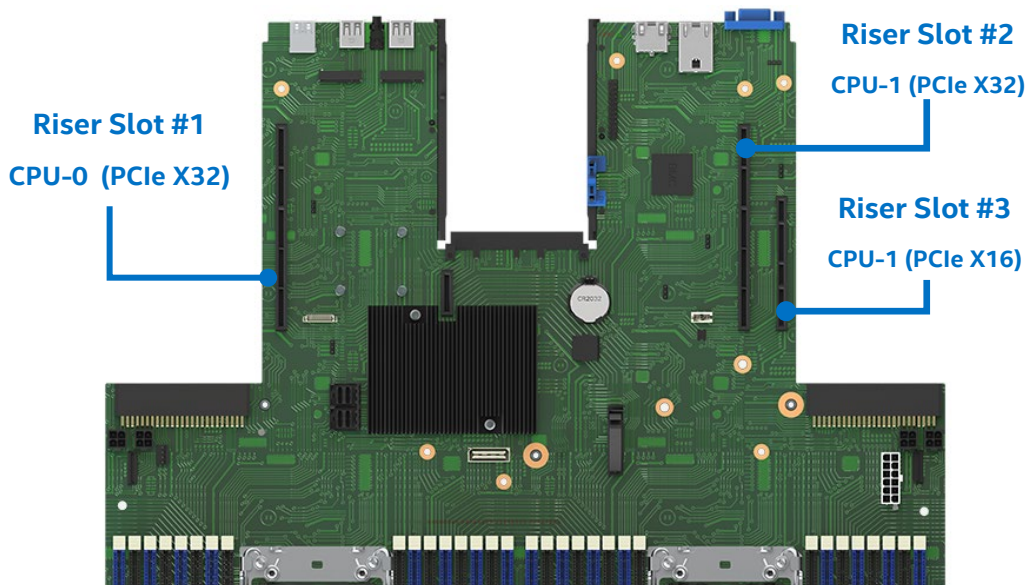
Figure 41. Riser Card Slots
