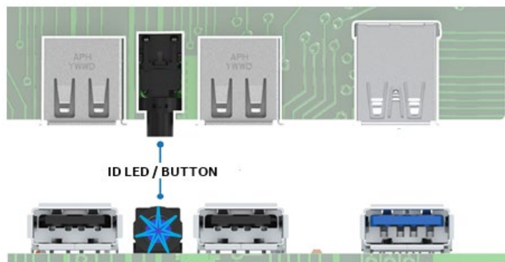
Figure 101. System ID LED / Button
