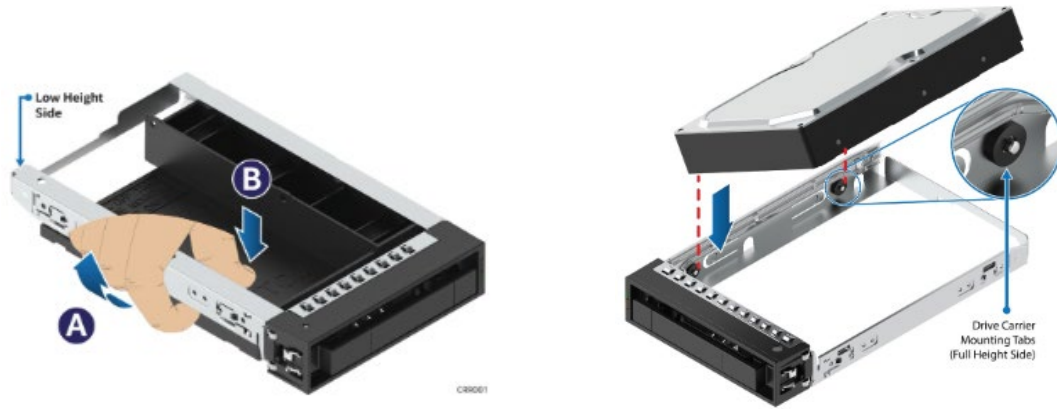
Figure 65. 3.5" Drive Assembly
