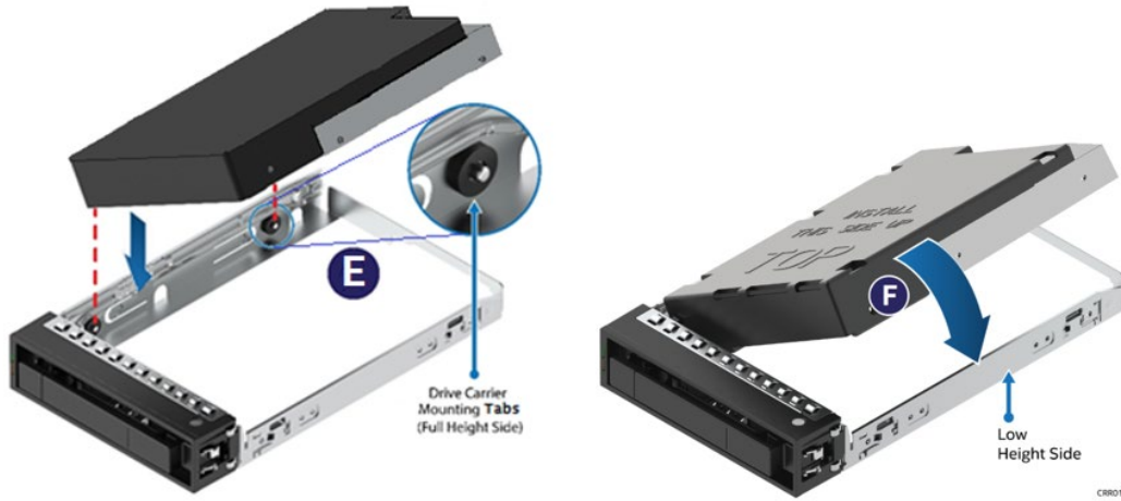
Figure 66. 2.5" SSD Assembly into Drive Rail – Alignment and SSD Installation
