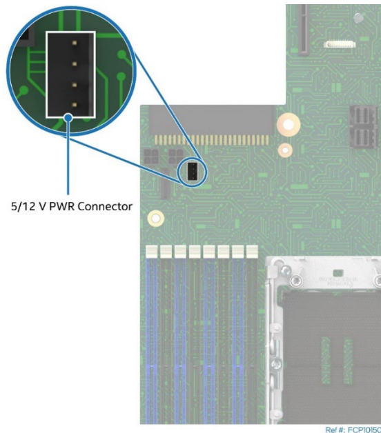
Figure 91. Peripheral Power Connector Identification
