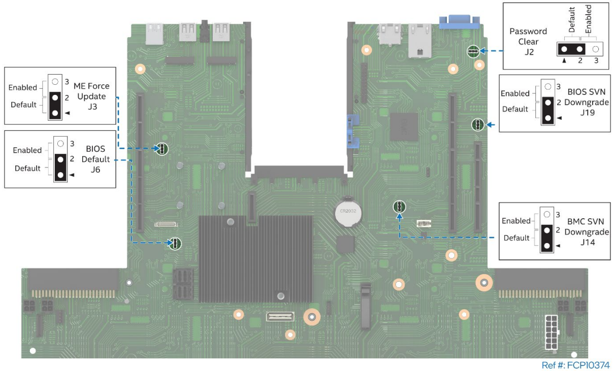
Figure 17. System Configuration and Recovery Jumpers
