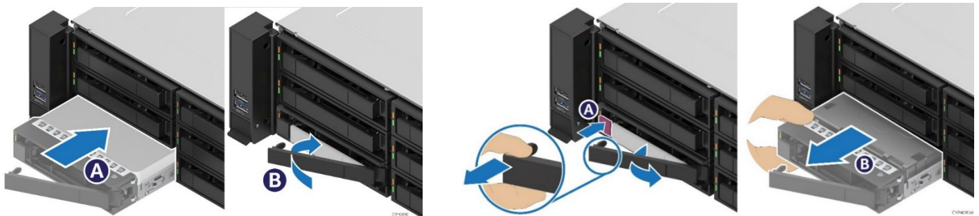
Figure 64. 3.5" Drive Insertion / Extraction
