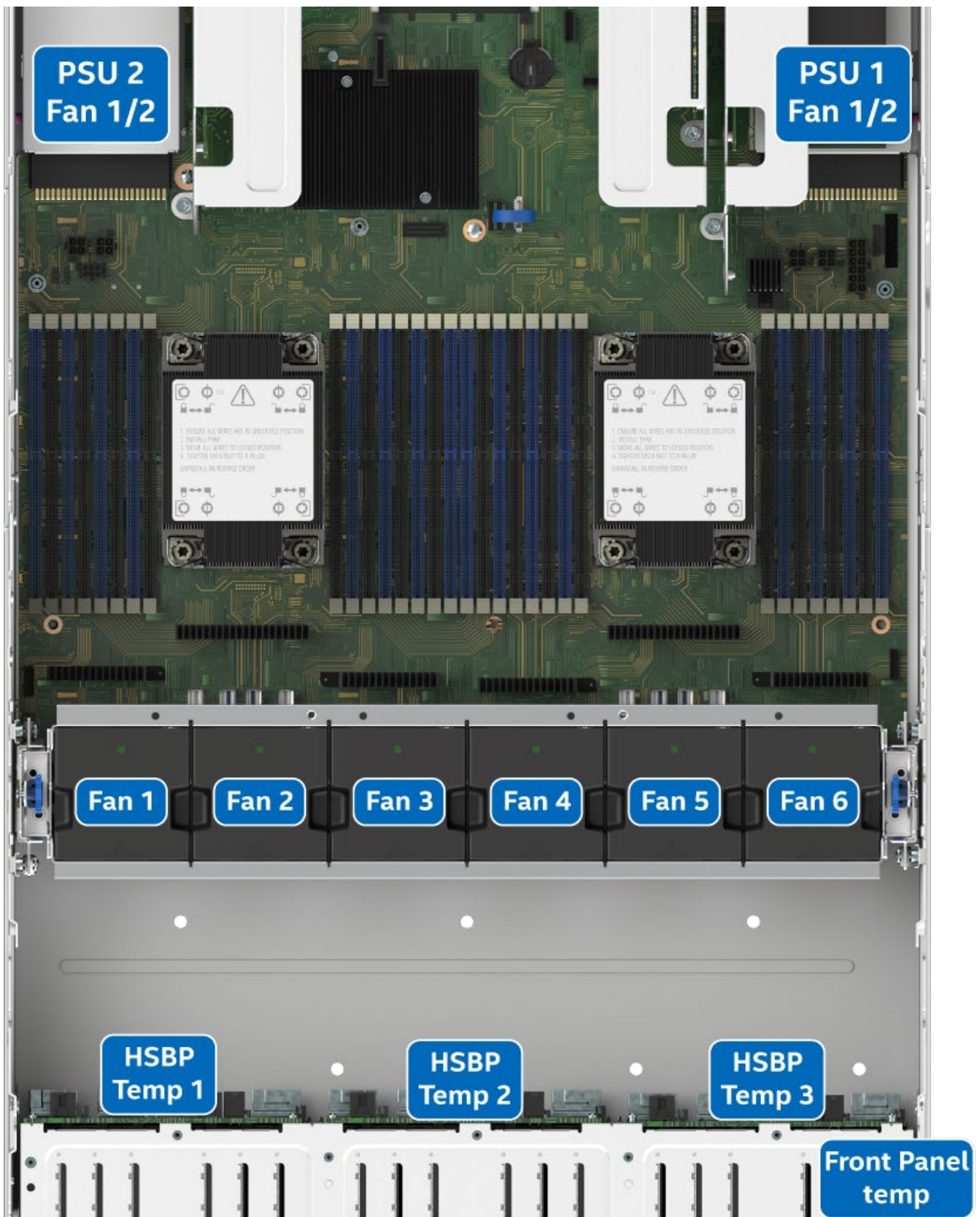
Figure 117. Server System Sensor Map
