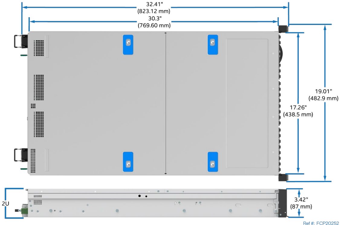
Figure 18. System Dimensions with 2100 Watt Power Supply Option
