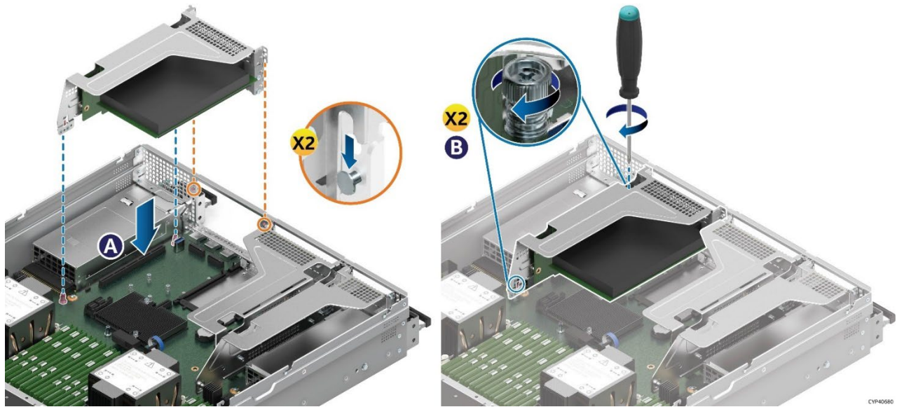
Figure 45. Riser Card Assembly Installation
