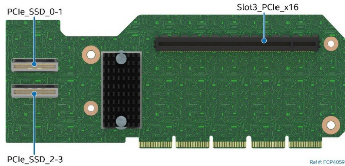
Figure 49. PCIe* NVMe* Riser Card for Riser Slot #1
