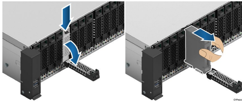
Figure 61. 7-mm Drive Removal from 2.5" Drive Bay
