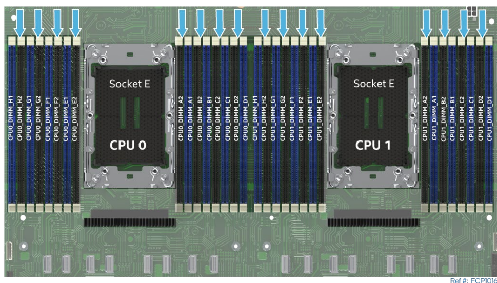
Figure 34. System Memory Modules / DIMM Blanks Configuration
