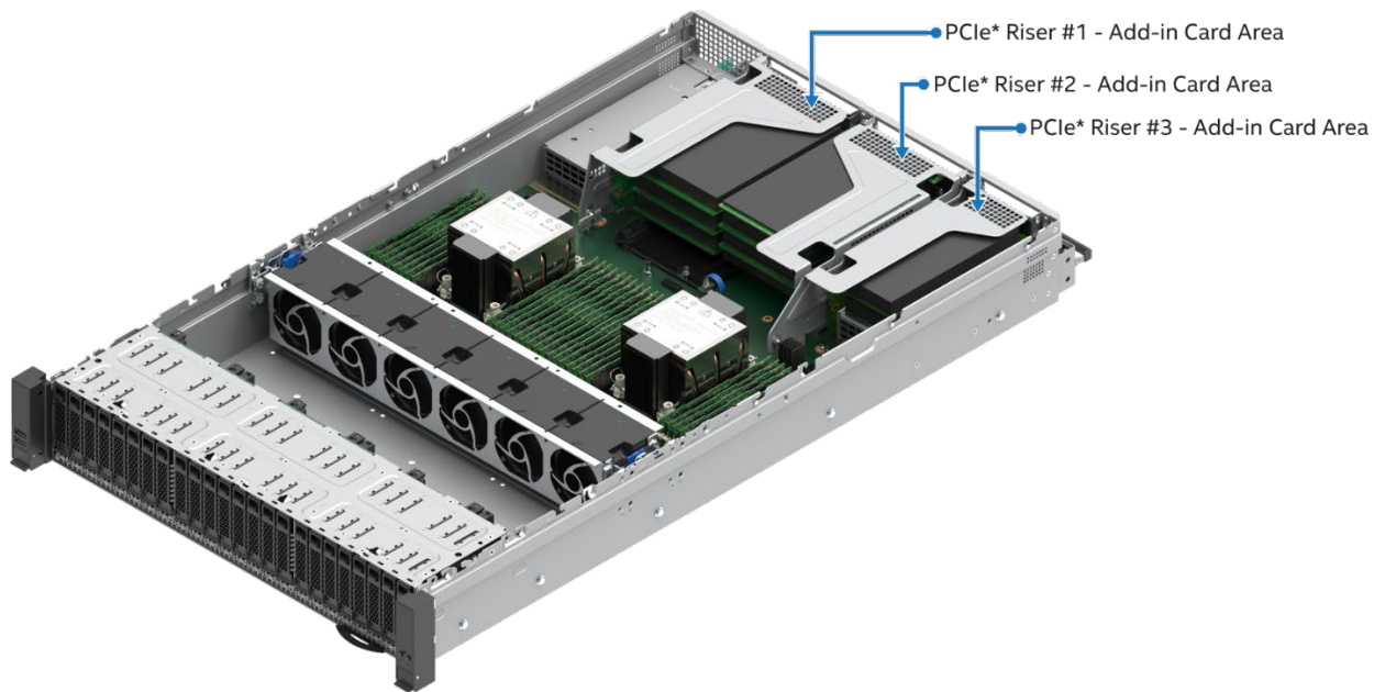
Figure 43. Server System PCIe* Riser Add-In Card Areas
