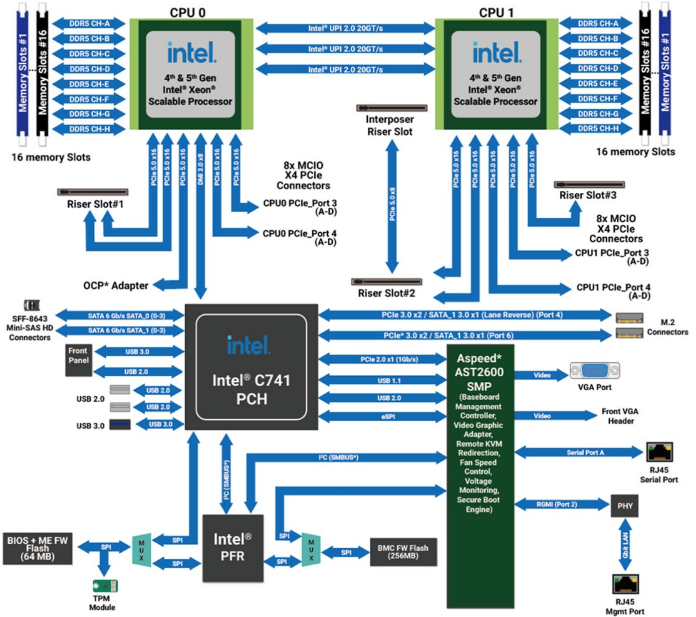
Figure 13. Intel® Server Board M50FCP2SBSTD Architectural Block Diagram
