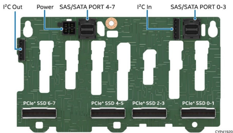
Figure 74. 8 x 2.5" SAS/SATA/NVMe* Hot-Swap Backplane – Back Side
