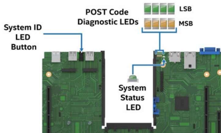
Figure 100. Exploded View of POST Code Diagnostic, System ID, and System Status LEDs
