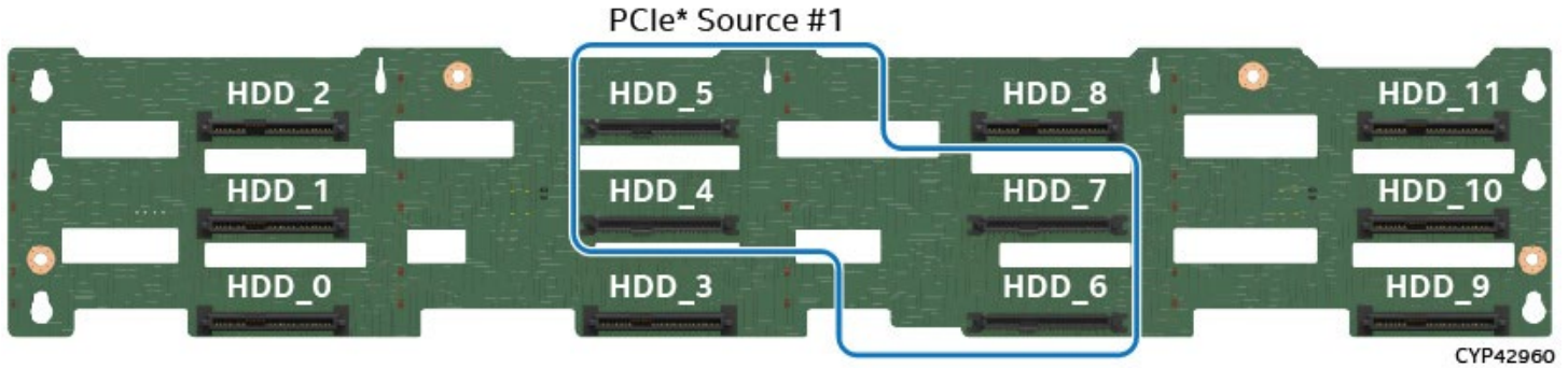
Figure 87. 12 x 3.5" HSBP NVMe* Connector Identification – Front Side
