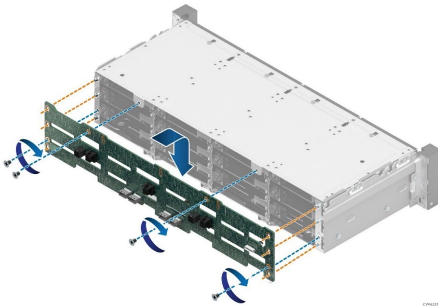
Figure 76. 3.5" Backplane Placement
