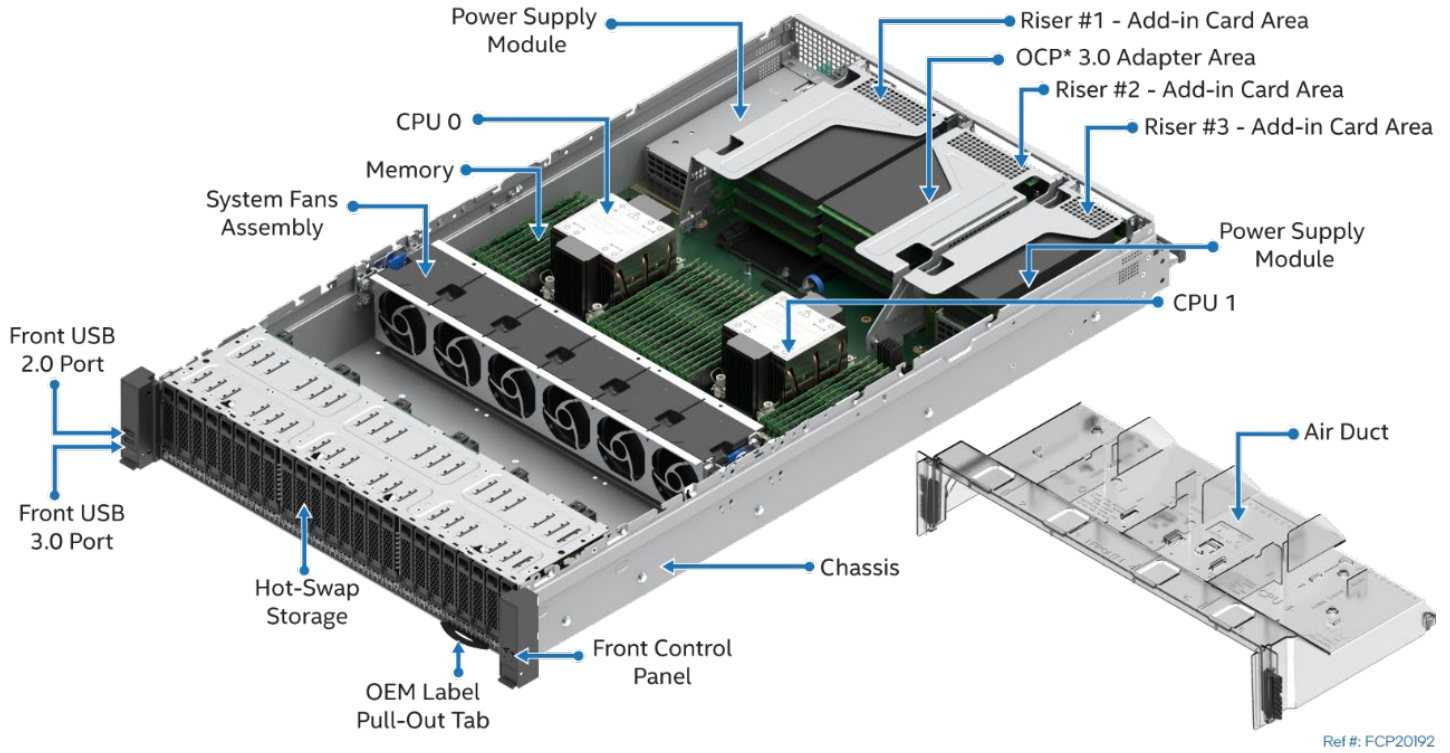
Figure 4. Server System Components Overview
