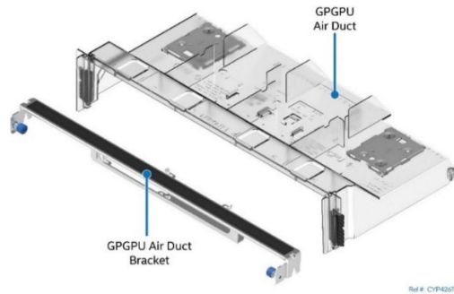
Figure 39. Optional GPGPU Air Duct for 1U Height Processor Heat Sink and GPGPU Add-In Cards
