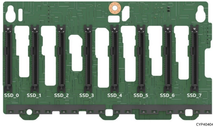
Figure 73. 8 x 2.5" SAS/SATA/NVMe* Hot-Swap Backplane – Front Side
