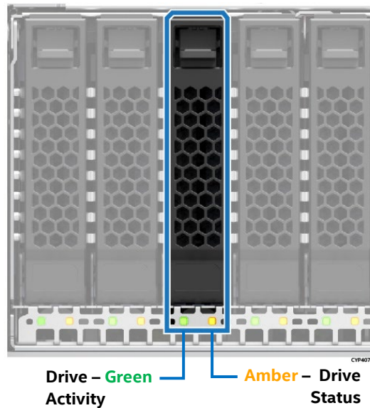
Figure 62. 2.5" Front Drive LED Identification
