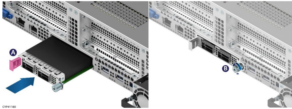
Figure 58. OCP* Adapter with Pull Tab Installation
