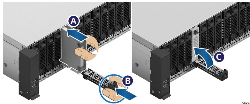
Figure 60. 7-mm Drive Insertion into 2.5" Drive Bay
