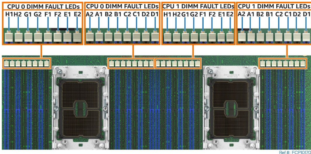
Figure 103. Memory Fault LED Location
