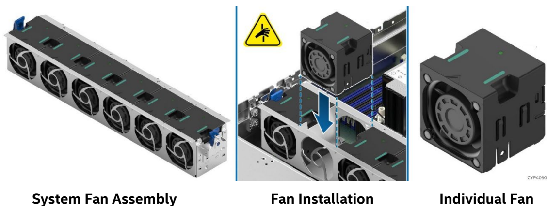
Figure 35. System Fan Assembly
