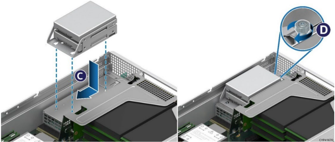
Figure 90. 2.5" Solid State Drive (SSD) Mounting Option
