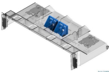
Figure 38. Optional Air Duct for 1U Height Processor Heat Sinks
