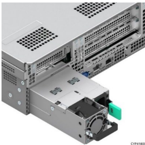
Figure 29. 2100 W Power Supply Module Partially Out of Chassis
