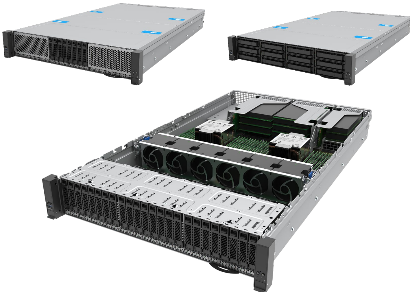
Figure 1. Intel® Server System M50FCP2UR Family
