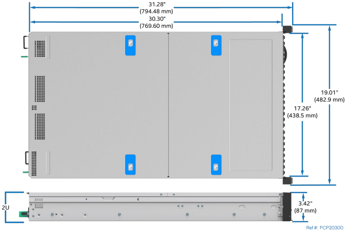
Figure 19. System Dimensions with 1300 Watt or 1600 Watt Power Supply Options
