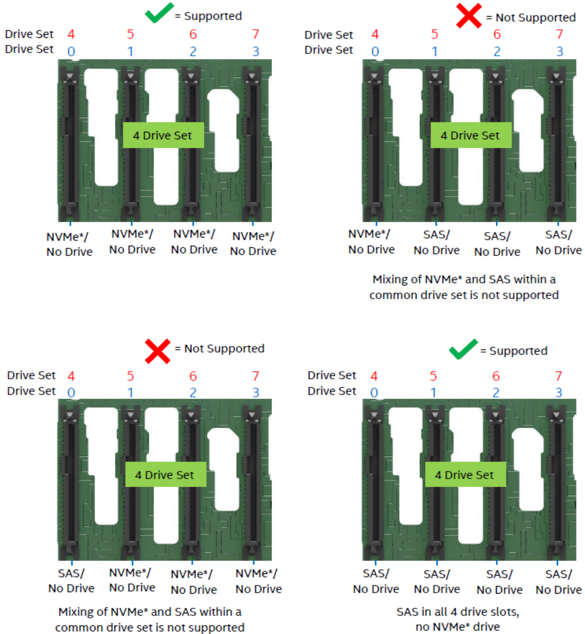
Figure 86. Supported Drive Population for Server Board MCIO Connectors or Tri-Mode Intel® RAID Module
