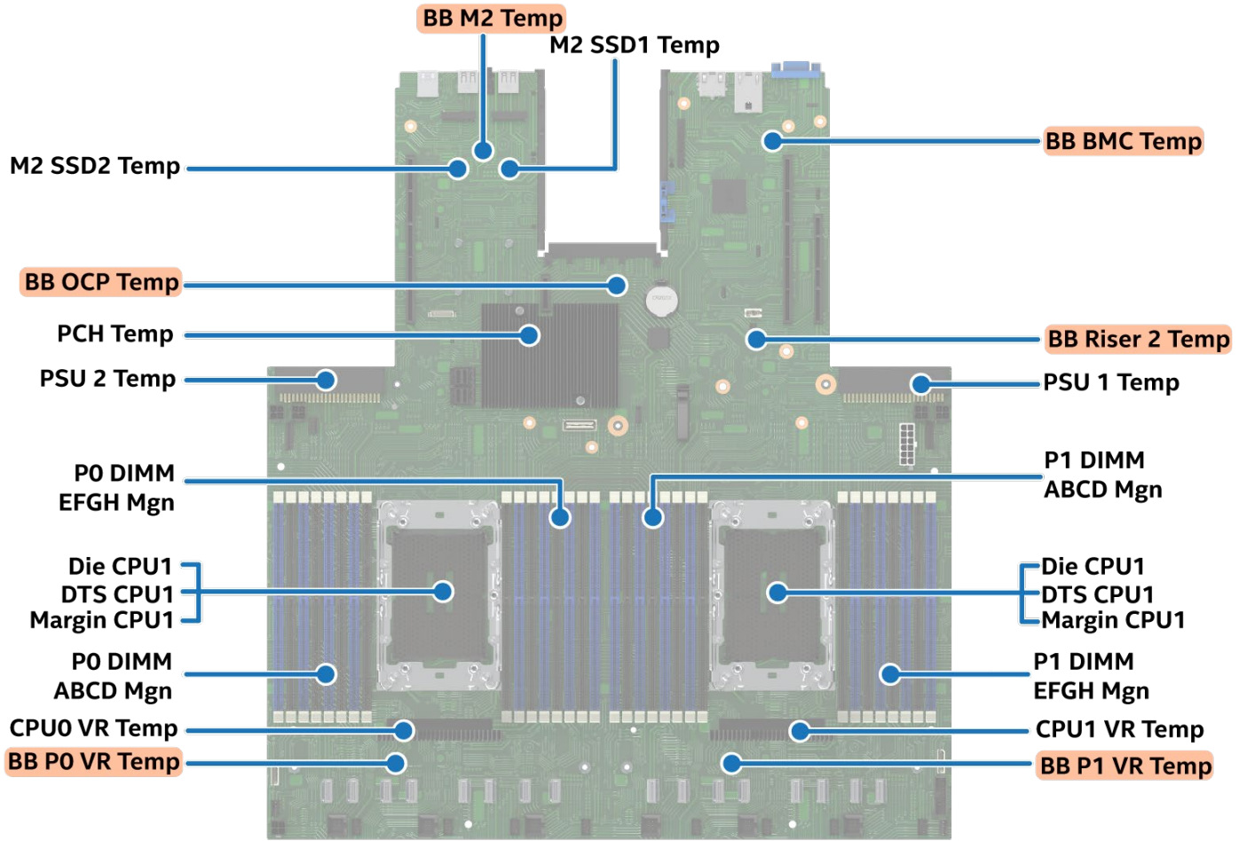
Figure 116. Server Board Sensor Map
