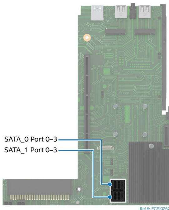
Figure 92. Onboard SATA Port Connectors
