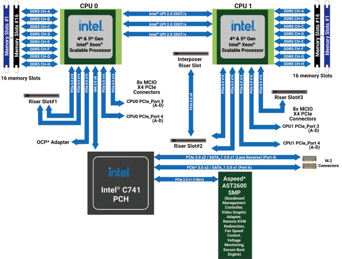
Figure 40. PCIe Subsystem Architecture
