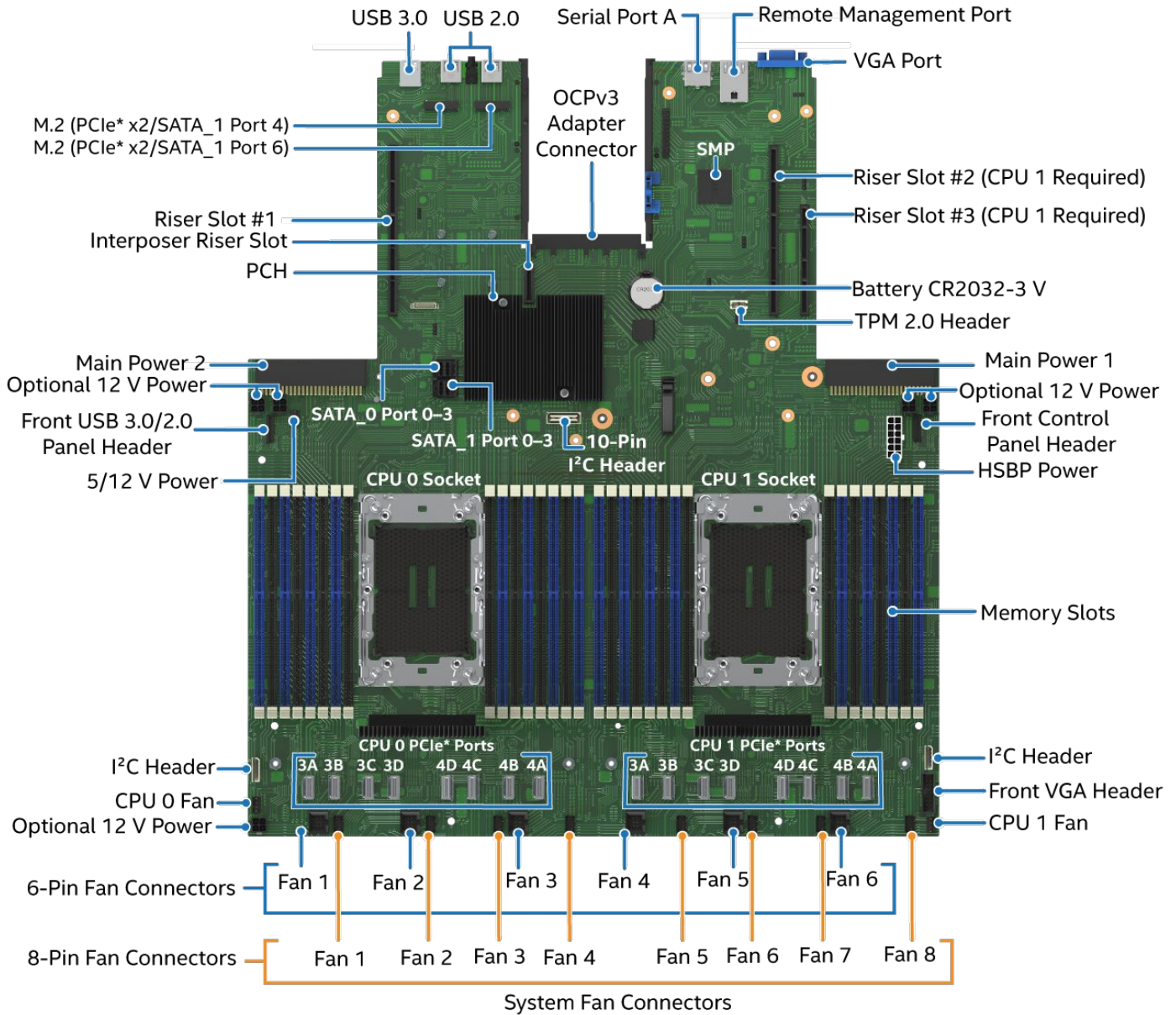
Figure 14. Intel® Server Board M50FCP2SBSTD Component / Feature Identification
