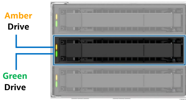
Figure 67. 3.5" Front Drive LED Identification
