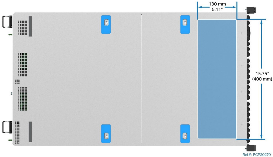
Figure 20. Label Emboss Dimensions
