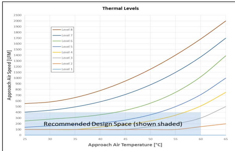
Figure 115. PCIe SIG Add-in cards thermal level
