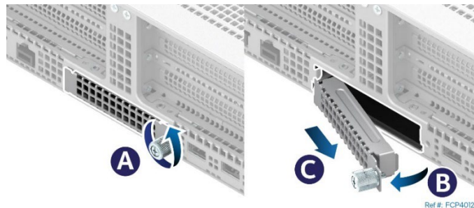
Figure 57. OCP* Adapter Bay Filler Removal
