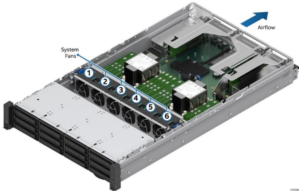
Figure 33. System Airflow and Fan Identification
