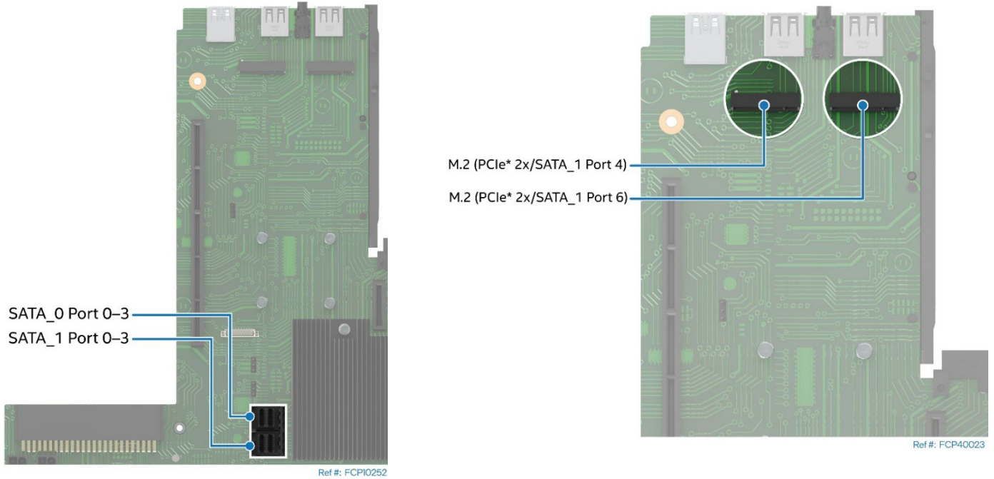
Figure 89. Onboard SATA Cable Connectors and M.2 SSD Connectors
