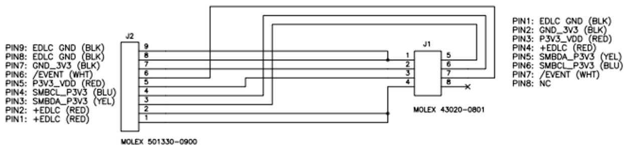
Figure 20. Extender cable pinout
