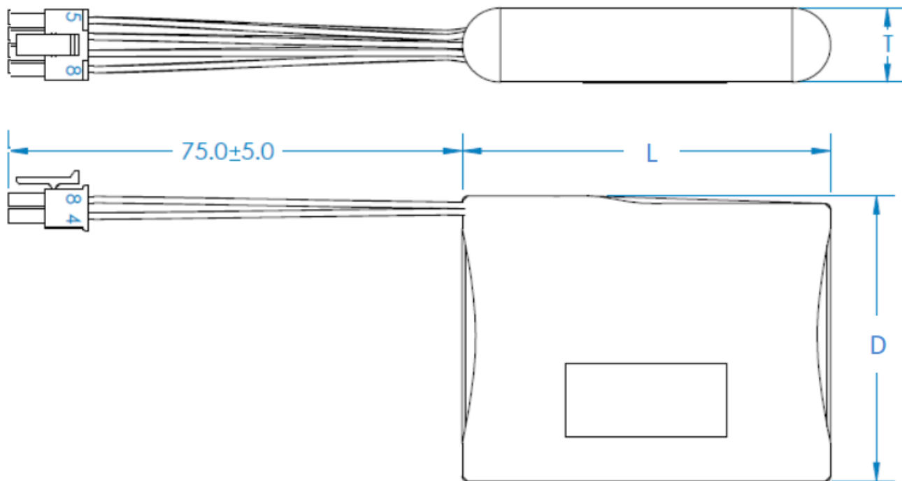
Figure 19. FBU345 layout
