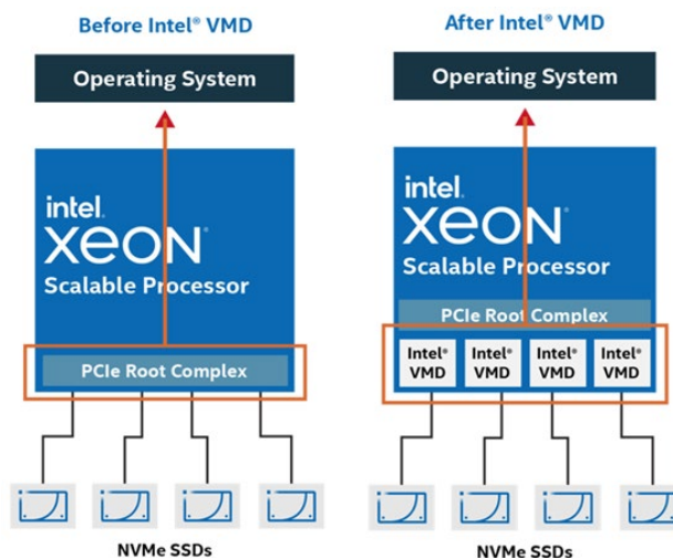
Figure 61. NVMe* Storage Bus Event / Error Handling
