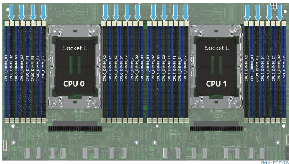
Figure 27. System Memory Module / DIMM Blanks Configuration
