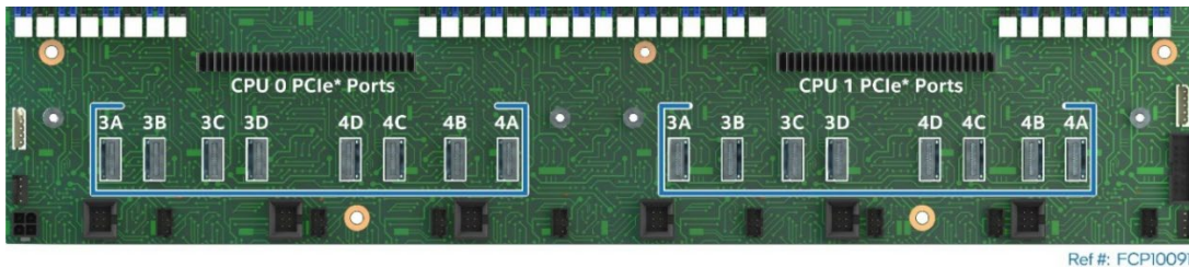
Figure 60. PCIe* MCIO Connectors
