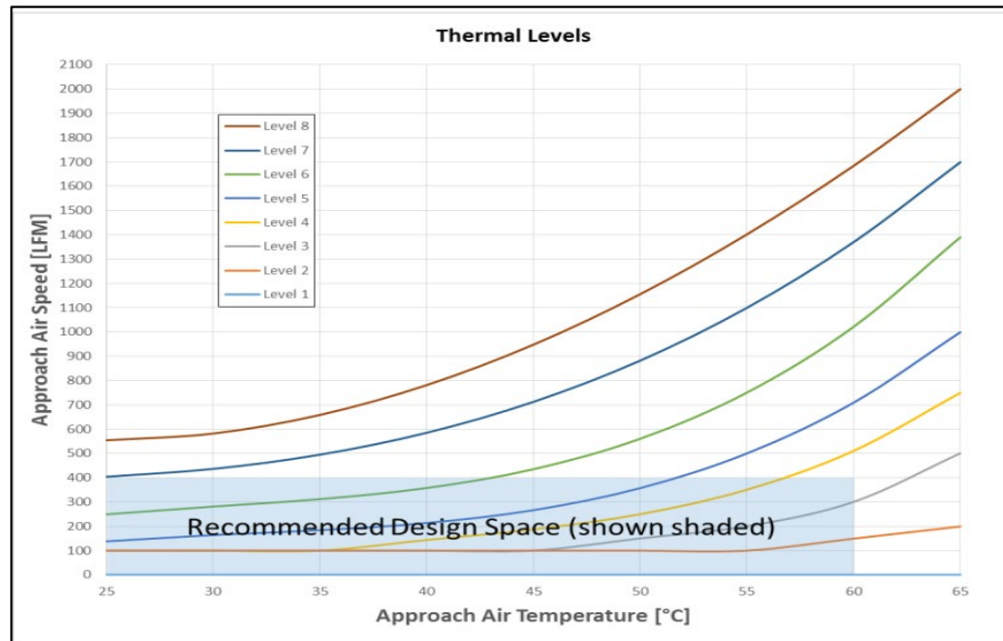
Figure 90. PCIe SIG Add-in cards thermal levels
