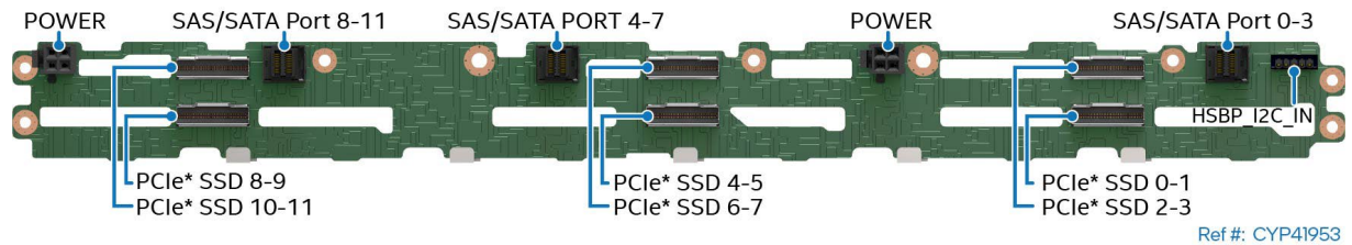
Figure 59. 12 x 2.5" SAS/SATA/NVMe* Hot Swap Backplane – Back Side
