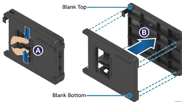
Figure 48. Separating a drive blank
