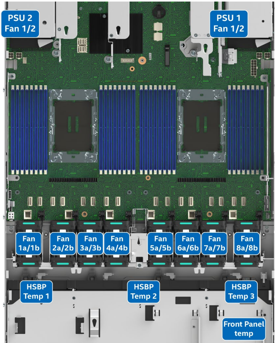
Figure 92. Server System Sensor Map
