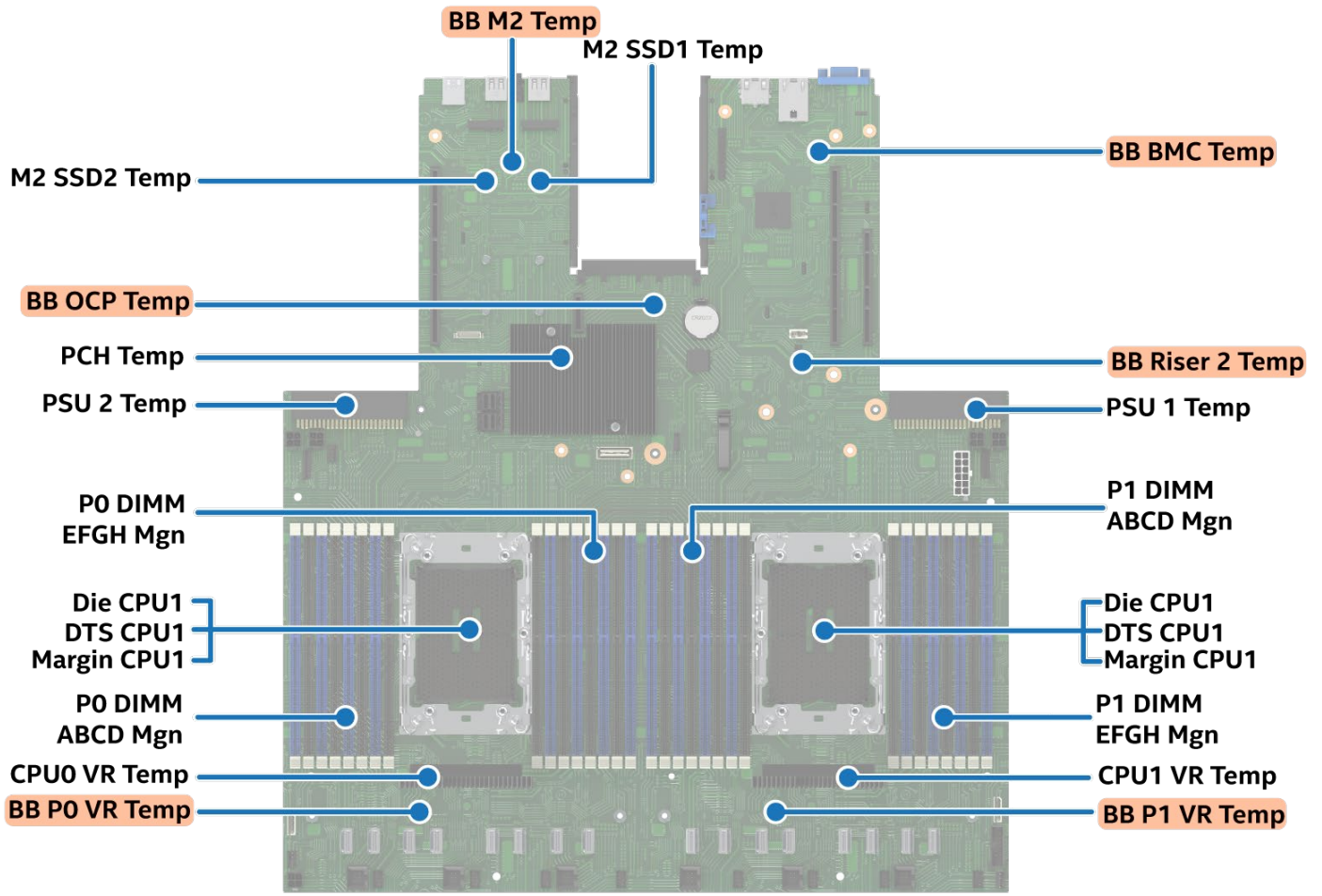
Figure 91. Server Board Sensor Map
