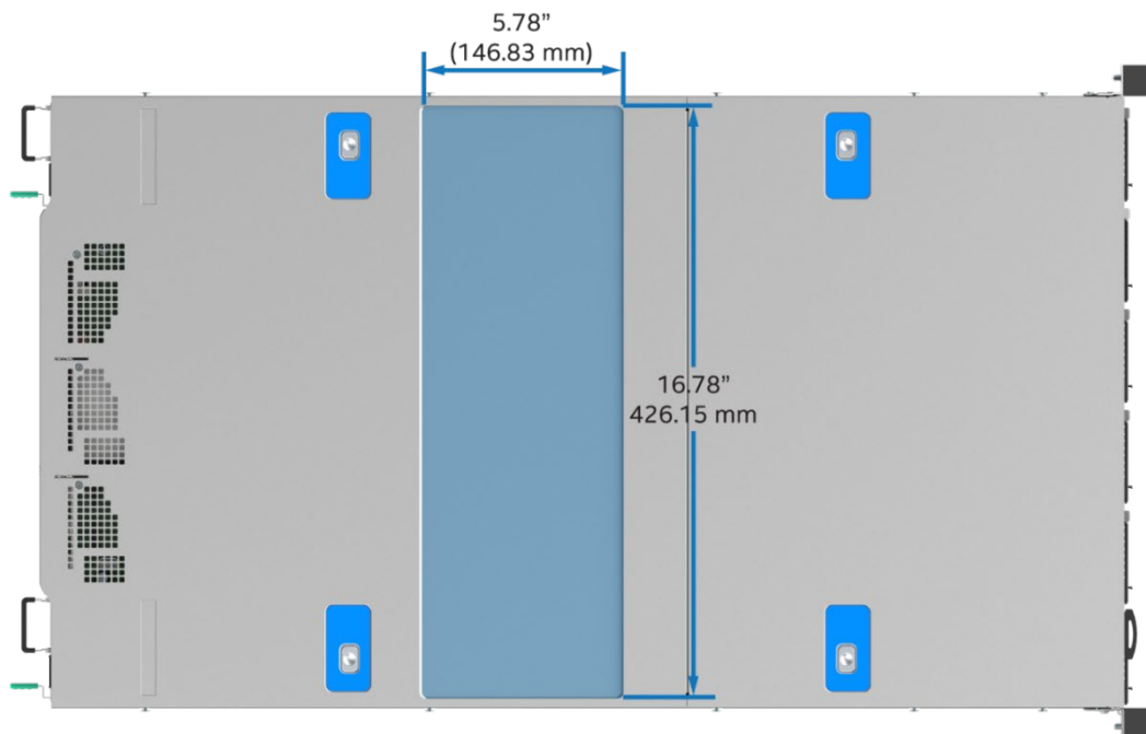
Figure 13. Label Emboss Dimensions
