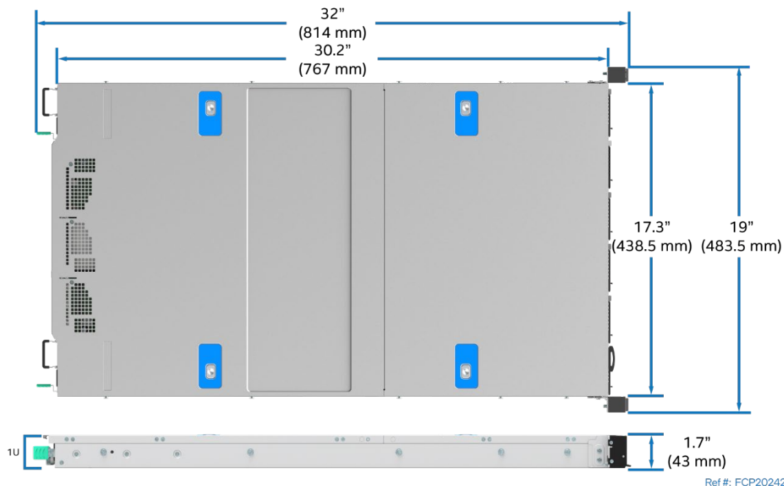
Figure 12. System Dimensions
