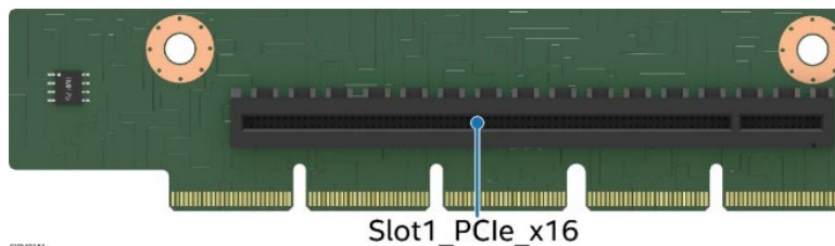
Figure 35. PCIe* Riser Card for Riser Slot #1
