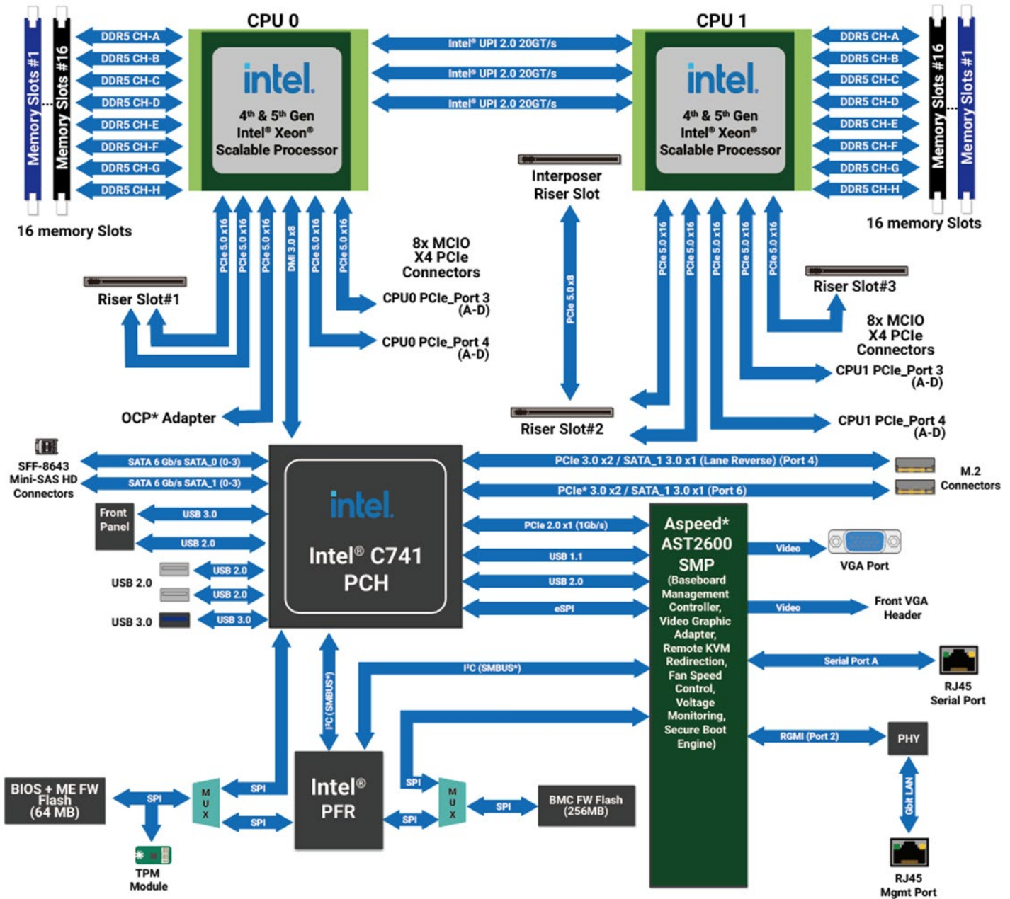
Figure 7. Intel® Server Board M50FCP2SBSTD Architectural Block Diagram
