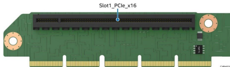
Figure 36. PCIe* Riser Card for Riser Slot #2
