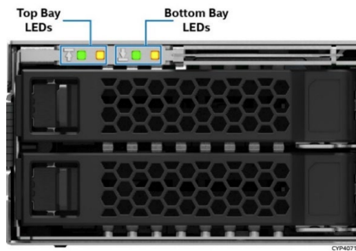
Figure 52. Drive Bay LED Identification
