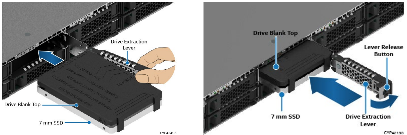
Figure 50. Drive Installation
