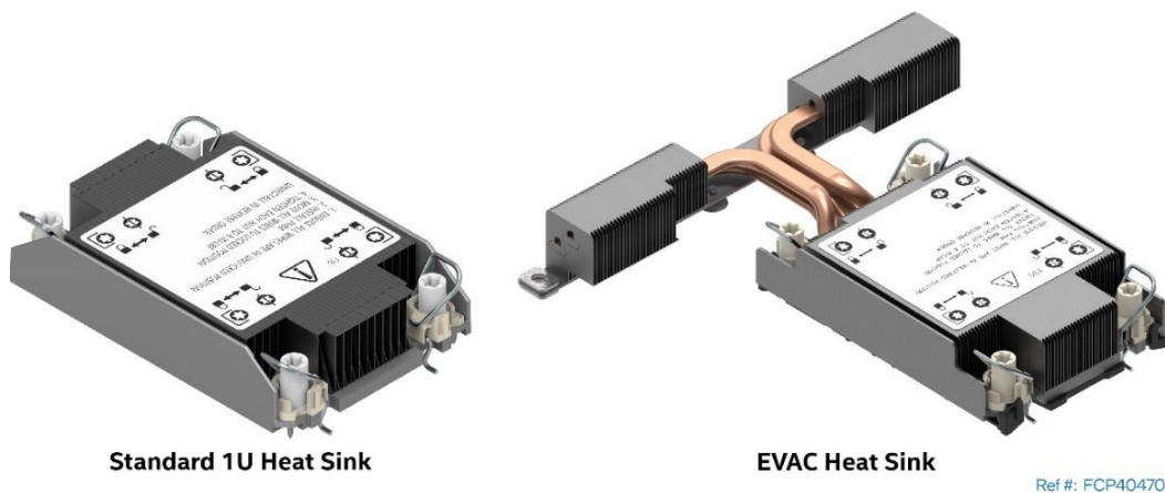
Figure 29. Supported Processor Heat Sinks
