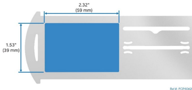
Figure 15. Pull-out Tab Label Emboss Dimensions
