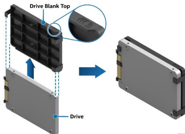
Figure 49. 7mm SSD Support
